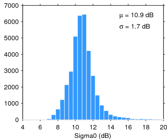
Figure 28. Histogram of science-valid sigma0 over oceans and lakes for 07/10/2015. The mean ( \mu ) and standard deviation ( \sigma ) are also shown. Note that values outside [4 20] dB are excluded from the histogram for the sake of readability but not from the computation of \mu and \sigma .
