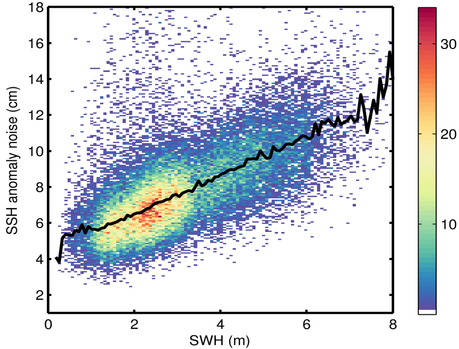
Figure 9. 2D histogram showing flag-valid SSH anomaly noise as a function of SWH for 07/10/2015. The black line denotes the median SSH anomaly noise as a function of SWH.
