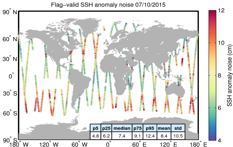
Figure 8. Geographical distribution of flag-valid 20-Hz SSH anomaly measurement noise over oceans and lakes for 07/10/2015. The statistical values shown in the table refer to the SSH anomaly noise and are calculated over all measurements shown in the figure.
