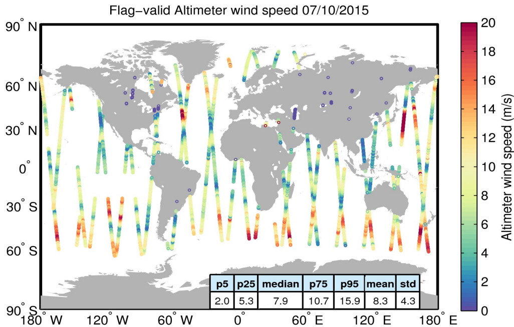
Figure 31. Geographical distribution of flag-valid wind data over oceans and lakes for 07/10/2015. The statistical values shown in the table refer to the wind in m/s and are calculated over all measurements shown in the figure.
