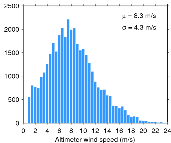
Figure 35. Histogram of science-valid wind over oceans and lakes for 07/10/2015. The mean ( \mu ) and standard deviation ( \sigma ) are also shown. Note that values larger than 24 m/s are excluded from the histogram for the sake of readability but not from the computation of \mu and \sigma .
