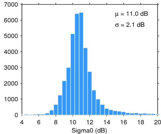
Figure 25. Histogram of flag-valid sigma0 over oceans and lakes for 07/10/2015. The mean ( \mu ) and standard deviation ( \sigma ) are also shown. Note that values outside [4 20] dB are excluded from the histogram for the sake of readability but not from the computation of \mu and \sigma .
