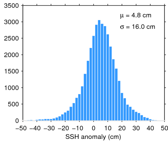
Figure 7. Histogram of flag-valid SSH anomaly over oceans and lakes for 07/10/2015. The mean ( \mu ) and standard deviation ( \sigma ) are also shown. Note that values outside [-50\ 50] cm are excluded from the histogram for the sake of readability but not from the computation of \mu and \sigma .
