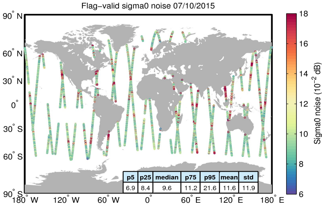
Figure 26. Geographical distribution of flag-valid 20-Hz sigma0 measurement noise over oceans and lakes for 07/10/2015. The statistical values shown in the table refer to the sigma0 noise and are calculated over all measurements shown in the figure.
