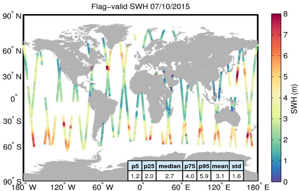
Figure 15. Geographical distribution of flag-valid SWH data over oceans and lakes for 07/10/2015. The statistical values shown in the table refer to the SWH in m and are calculated over all measurements shown in the figure.
