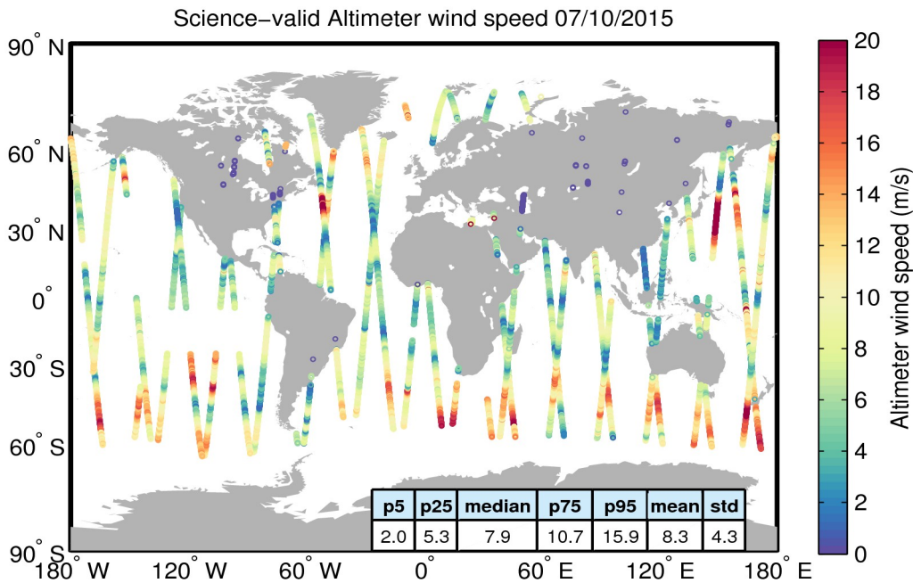
Figure 34. Geographical distribution of science-valid wind data over oceans and lakes for 07/10/2015. The statistical values shown in the table refer to the wind in m/s and are calculated over all measurements shown in the figure. Gray circles denote records that have been rejected based on the editing criteria described in Table 5.
