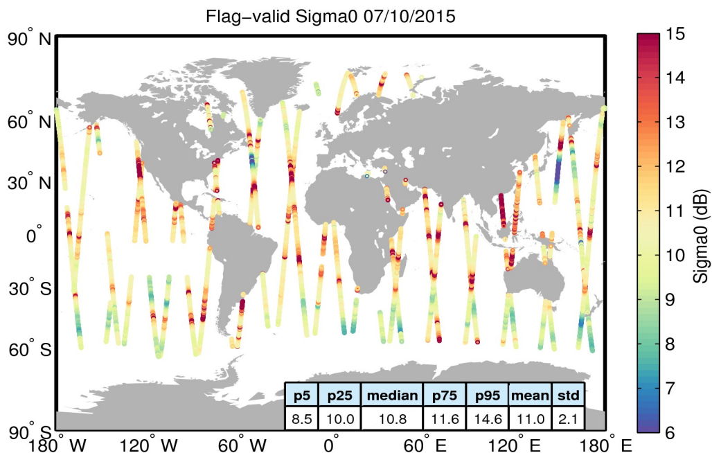
Figure 23. Geographical distribution of flag-valid sigma0 data over oceans and lakes for 07/10/2015. The statistical values shown in the table refer to the sigma0 in dB and are calculated over all measurements shown in the figure.
