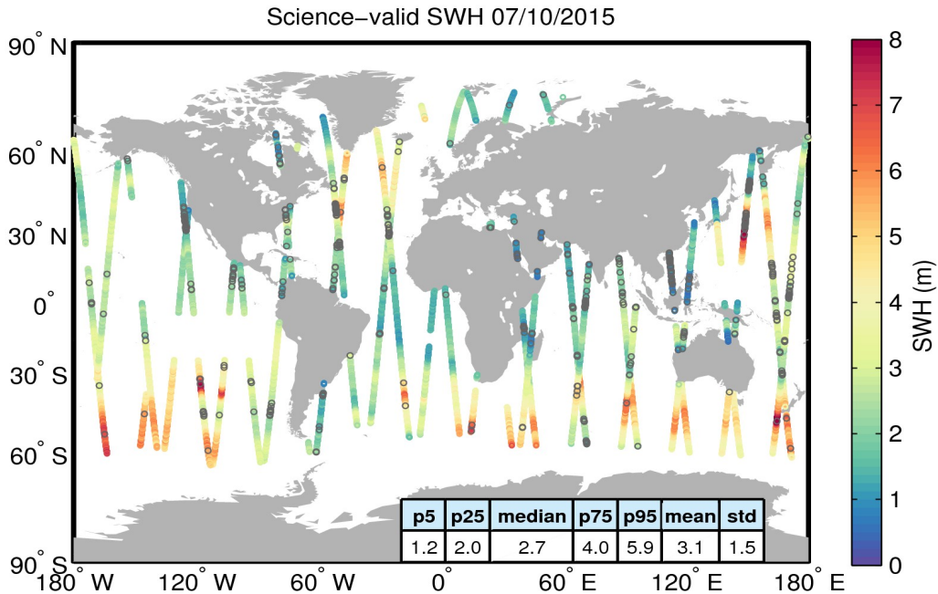
Figure 19. Geographical distribution of science-valid SWH data over oceans and lakes for 07/10/2015. The statistical values shown in the table refer to the SWH in m and are calculated over all measurements shown in the figure. Gray circles denote records that have been rejected based on the editing criteria described in Table 3.
