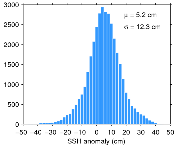
Figure 11. Histogram of science-valid SSH anomaly over oceans and lakes for 07/10/2015. The mean ( \mu ) and standard deviation ( \sigma ) are also shown. Note that values outside [-50 50] cm are excluded from the histogram for the sake of readability but not from the computation of \mu and \sigma .
