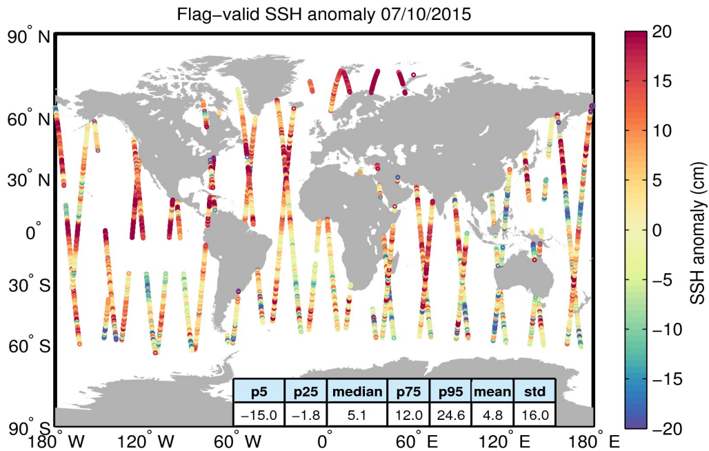
Figure 5. Geographical distribution of flag-valid 1-Hz SSH anomaly data over oceans and lakes for 07/10/2015. The statistical values shown in the table refer to the SSH anomaly in cm and are calculated over all measurements shown in the figure.
