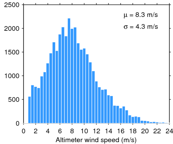
Figure 33. Histogram of flag-valid wind over oceans and lakes for 07/10/2015. The mean ( \mu ) and standard deviation ( \sigma ) are also shown. Note that values larger than 24 m/s are excluded from the histogram for the sake of readability but not from the computation of \mu and \sigma .
