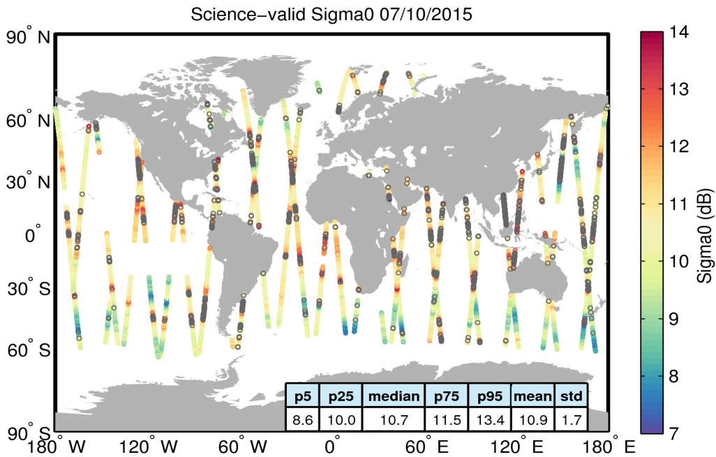
Figure 27. Geographical distribution of science-valid sigma0 data over oceans and lakes for 07/10/2015. The statistical values shown in the table refer to the sigma0 in dB and are calculated over all measurements shown in the figure. Gray circles denote records that have been rejected based on the editing criteria described in Table 4.
