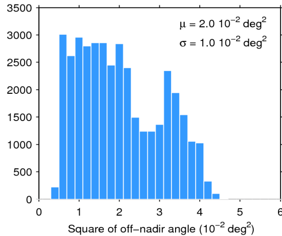
Figure 39. Histogram of flag-valid mispointing over oceans and lakes for 07/10/2015. The mean ( \mu ) and standard deviation ( \sigma ) are also shown. Note that values larger than 6 \cdot 10^{-2} \text{ deg}^2 are excluded from the histogram for the sake of readability but not from the computation of \mu and \sigma .
