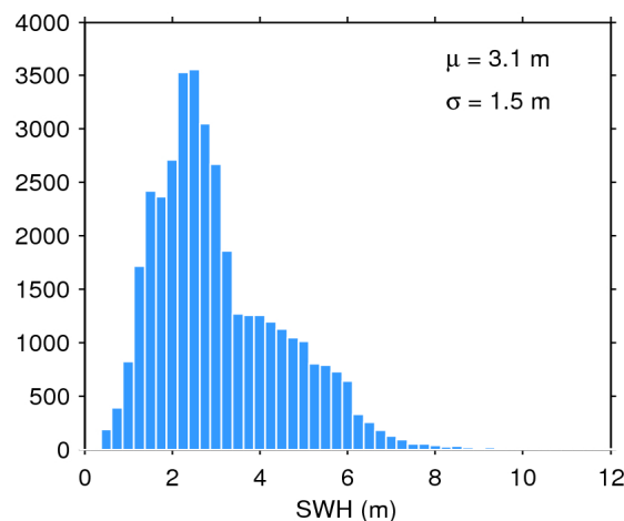
Figure 20. Histogram of science-valid SWH over oceans and lakes for 07/10/2015. The mean ( \mu ) and standard deviation ( \sigma ) are also shown. Note that values larger than 12 m are excluded from the histogram for the sake of readability but not from the computation of \mu and \sigma .
