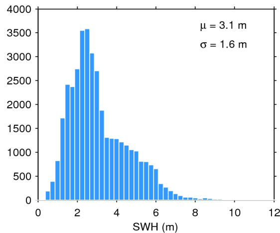
Figure 17. Histogram of flag-valid SWH over oceans and lakes for 07/10/2015. The mean ( \mu ) and standard deviation ( \sigma ) are also shown. Note that values larger than 12 m are excluded from the histogram for the sake of readability but not from the computation of \mu and \sigma .
