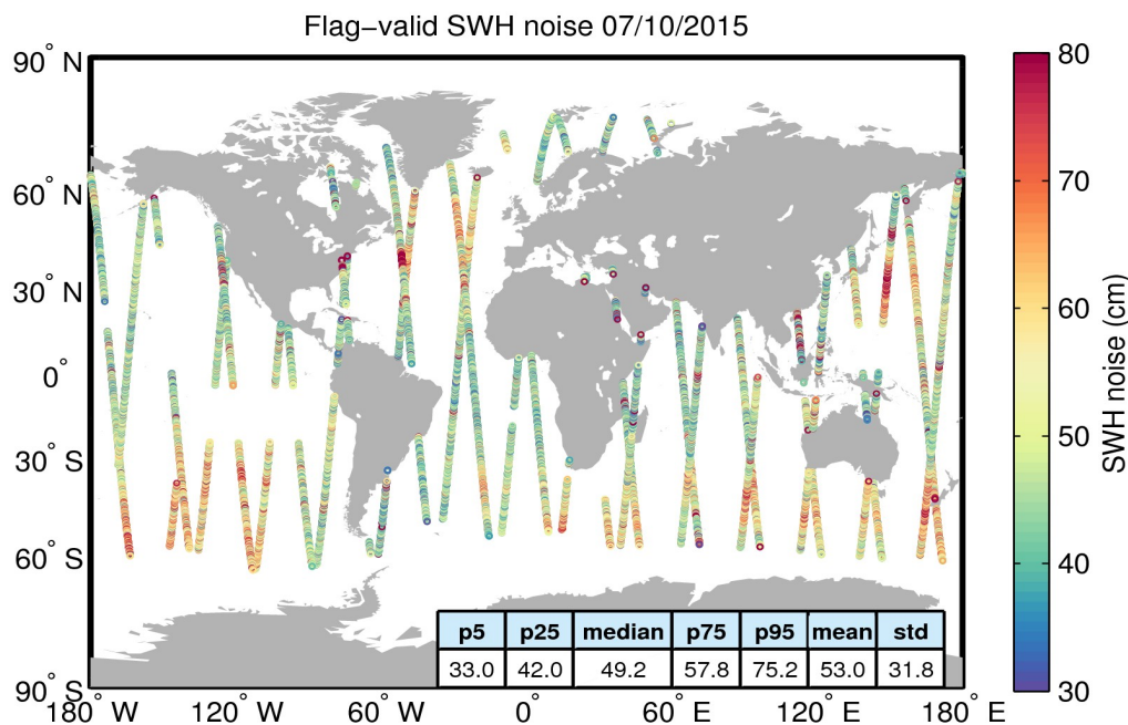
Figure 18. Geographical distribution of flag-valid 20-Hz SWH measurement noise over oceans and lakes for 07/10/2015. The statistical values shown in the figure refer to the SWH noise and are calculated over all measurements shown in the figure.
