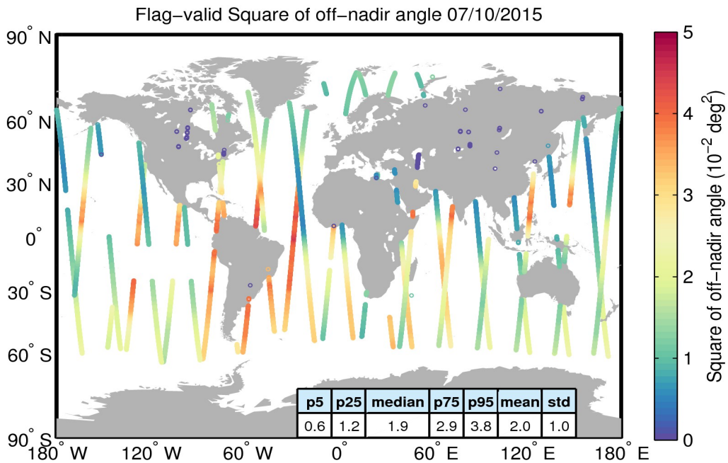
Figure 37. Geographical distribution of flag-valid mispointing data over oceans and lakes for 07/10/2015. The statistical values shown in the table refer to the mispointing in 10^{-2} \text{ deg}^2 and are calculated over all measurements shown in the figure.
