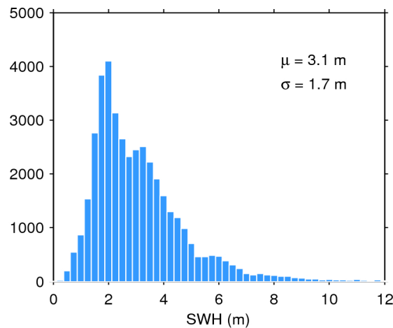
Figure 17. Histogram of flag-valid SWH over oceans and lakes for 04/10/2015. The mean ( \mu ) and standard deviation ( \sigma ) are also shown. Note that values larger than 12 m are excluded from the histogram for the sake of readability but not from the computation of \mu and \sigma .
