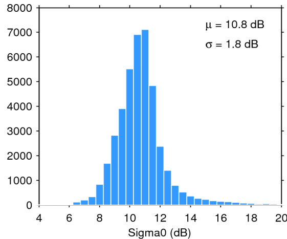
Figure 25. Histogram of flag-valid sigma0 over oceans and lakes for 04/10/2015. The mean ( \mu ) and standard deviation ( \sigma ) are also shown. Note that values outside [4 20] dB are excluded from the histogram for the sake of readability but not from the computation of \mu and \sigma .
