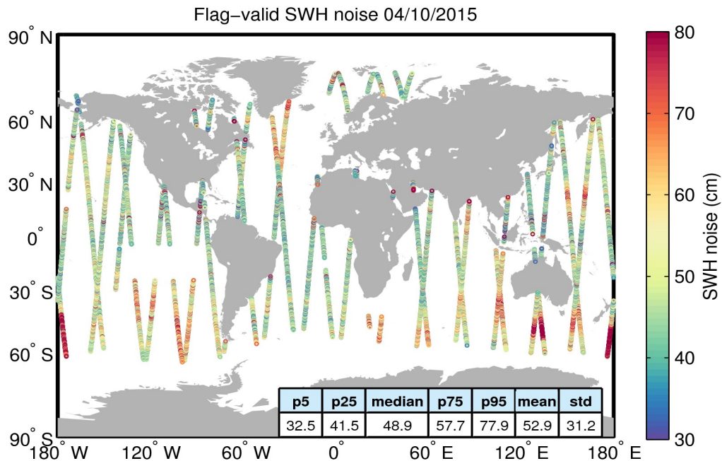
Figure 18. Geographical distribution of flag-valid 20-Hz SWH measurement noise over oceans and lakes for 04/10/2015. The statistical values shown in the table refer to the SWH noise and are calculated over all measurements shown in the figure.
