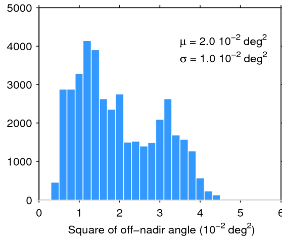
Figure 39. Histogram of flag-valid mispointing over oceans and lakes for 04/10/2015. The mean ( \mu ) and standard deviation ( \sigma ) are also shown. Note that values larger than 6 \cdot 10^{-2} \text{ deg}^2 are excluded from the histogram for the sake of readability but not from the computation of \mu and \sigma .
