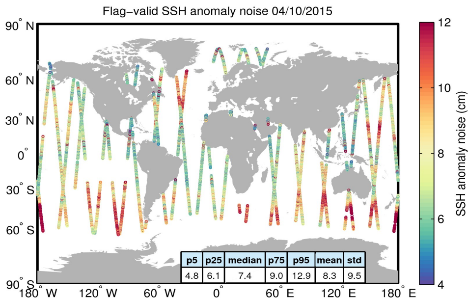
Figure 8. Geographical distribution of flag-valid 20-Hz SSH anomaly measurement noise over oceans and lakes for 04/10/2015. The statistical values shown in the table refer to the SSH anomaly noise and are calculated over all measurements shown in the figure.
