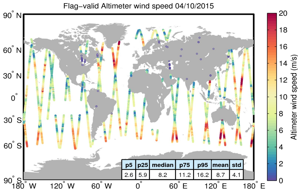
Figure 31. Geographical distribution of flag-valid wind data over oceans and lakes for 04/10/2015. The statistical values shown in the table refer to the wind in m/s and are calculated over all measurements shown in the figure.
