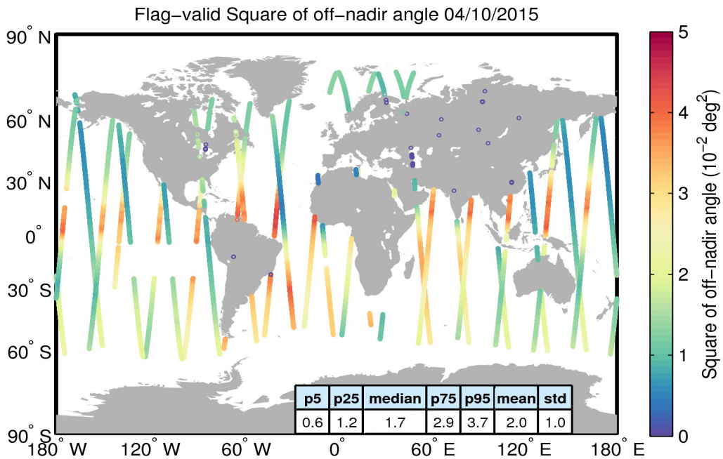
Figure 37. Geographical distribution of flag-valid mispointing data over oceans and lakes for 04/10/2015. The statistical values shown in the table refer to the mispointing in 10^{-2} deg 2 and are calculated over all measurements shown in the figure.
