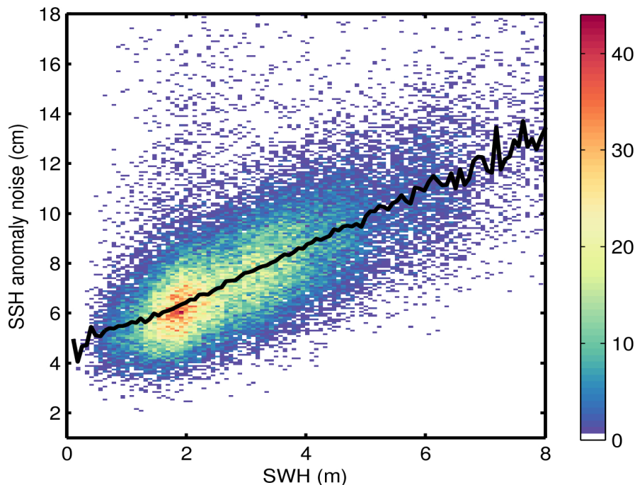
Figure 9. 2D histogram showing flag-valid SSH anomaly noise as a function of SWH for 04/10/2015. The black line denotes the median SSH anomaly noise as a function of SWH.
