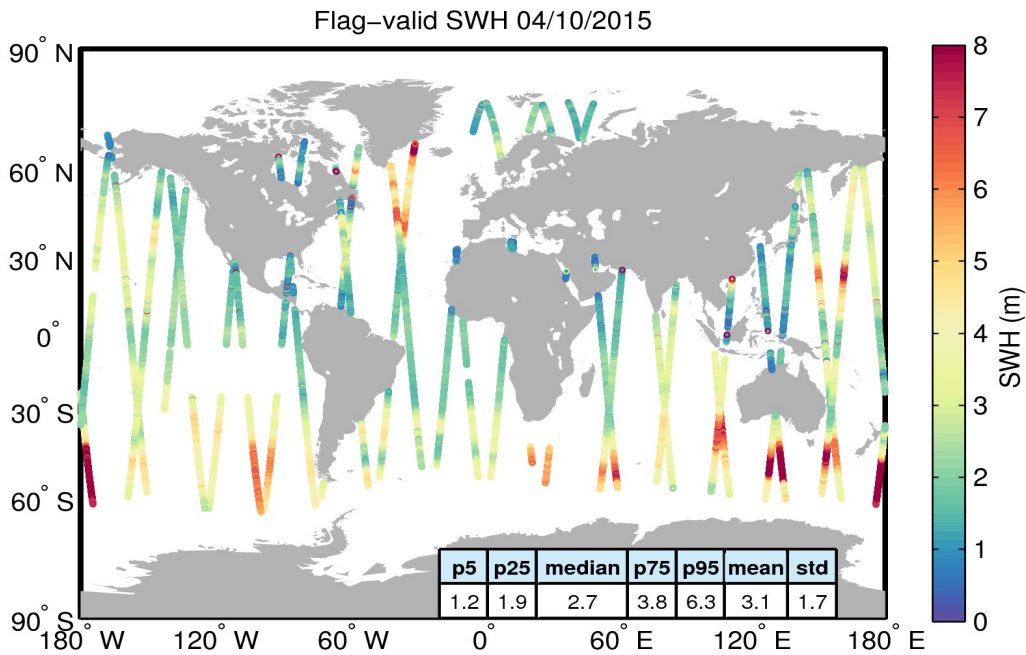
Figure 15. Geographical distribution of flag-valid SWH data over oceans and lakes for 04/10/2015. The statistical values shown in the table refer to the SWH in m and are calculated over all measurements shown in the figure.
