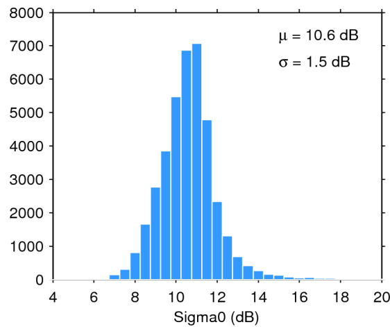
Figure 28. Histogram of science-valid sigma0 over oceans and lakes for 04/10/2015. The mean ( \mu ) and standard deviation ( \sigma ) are also shown. Note that values outside [4 20] dB are excluded from the histogram for the sake of readability but not from the computation of \mu and \sigma .
