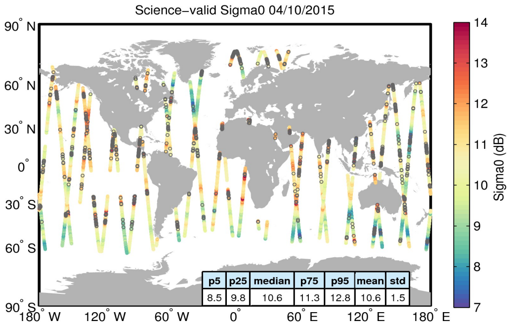
Figure 27. Geographical distribution of science-valid sigma0 data over oceans and lakes for 04/10/2015. The statistical values shown in the table refer to the sigma0 in dB and are calculated over all measurements shown in the figure. Gray circles denote records that have been rejected based on the editing criteria described in Table 4.
