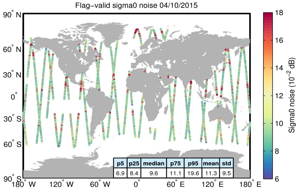
Figure 26. Geographical distribution of flag-valid 20-Hz sigma0 measurement noise over oceans and lakes for 04/10/2015. The statistical values shown in the table refer to the sigma0 noise and are calculated over all measurements shown in the figure.
