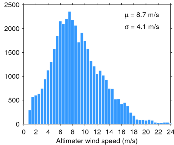
Figure 33. Histogram of flag-valid wind over oceans and lakes for 04/10/2015. The mean ( \mu ) and standard deviation ( \sigma ) are also shown. Note that values larger than 24 m/s are excluded from the histogram for the sake of readability but not from the computation of \mu and \sigma .
