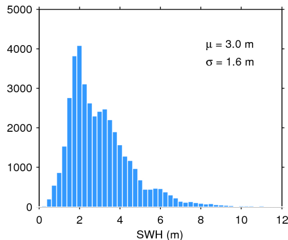
Figure 20. Histogram of science-valid SWH over oceans and lakes for 04/10/2015. The mean ( \mu ) and standard deviation ( \sigma ) are also shown. Note that values larger than 12 m are excluded from the histogram for the sake of readability but not from the computation of \mu and \sigma .
