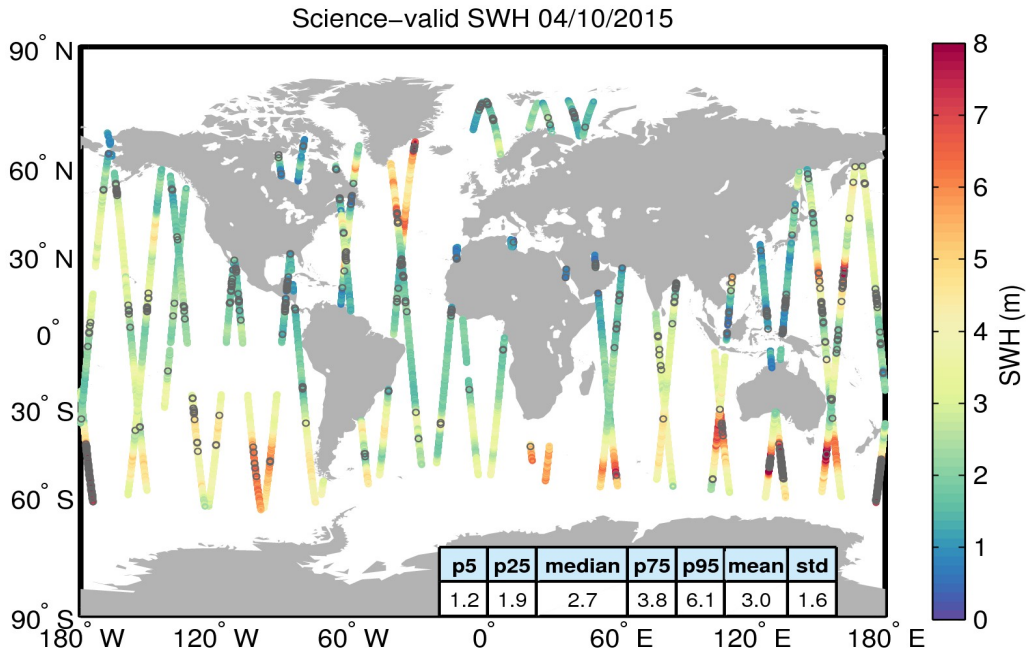
Figure 19. Geographical distribution of science-valid SWH data over oceans and lakes for 04/10/2015. The statistical values shown in the table refer to the SWH in m and are calculated over all measurements shown in the figure. Gray circles denote records that have been rejected based on the editing criteria described in Table 3.
