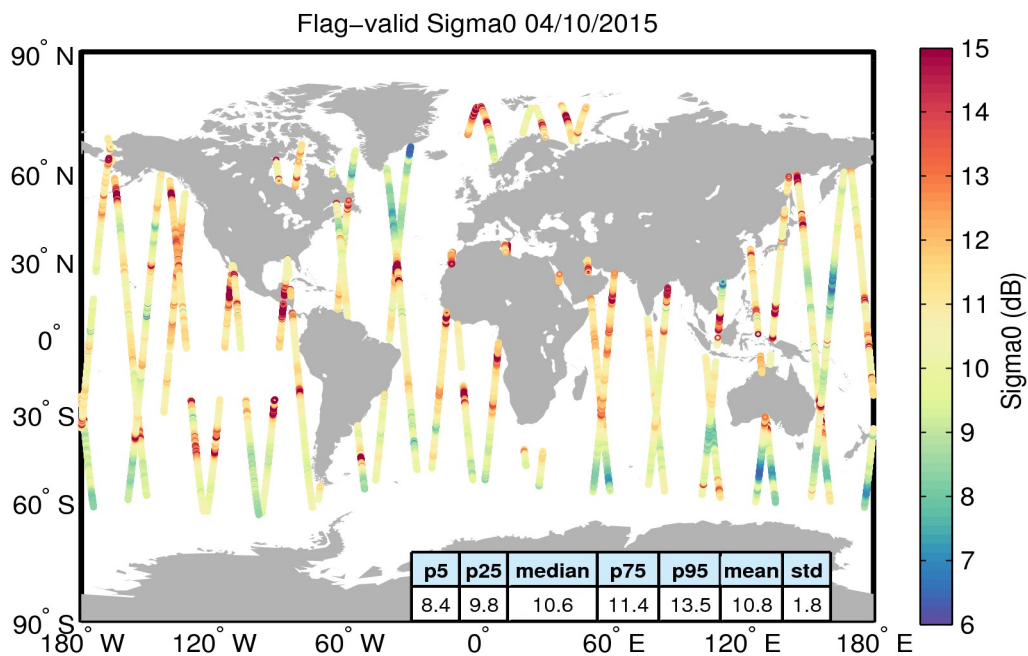
Figure 23. Geographical distribution of flag-valid sigma0 data over oceans and lakes for 04/10/2015. The statistical values shown in the table refer to the sigma0 in dB and are calculated over all measurements shown in the figure.
