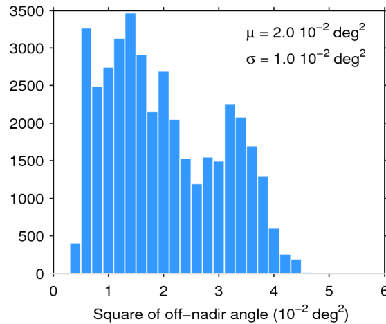
Figure 39. Histogram of flag-valid mispointing over oceans and lakes for 03/10/2015. The mean ( \mu ) and standard deviation ( \sigma ) are also shown. Note that values larger than 6 \cdot 10^{-2} \text{ deg}^2 are excluded from the histogram for the sake of readability but not from the computation of \mu and \sigma .
