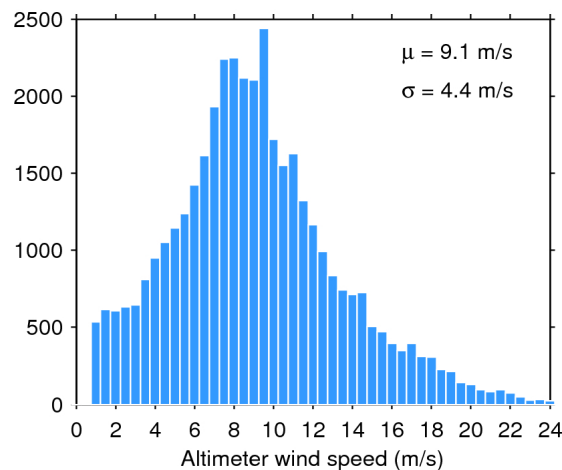
Figure 35. Histogram of science-valid wind over oceans and lakes for 03/10/2015. The mean ( \mu ) and standard deviation ( \sigma ) are also shown. Note that values larger than 24 m/s are excluded from the histogram for the sake of readability but not from the computation of \mu and \sigma .
