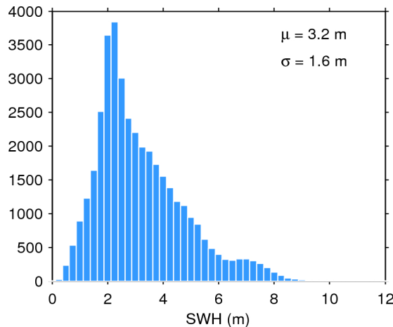
Figure 20. Histogram of science-valid SWH over oceans and lakes for 03/10/2015. The mean ( \mu ) and standard deviation ( \sigma ) are also shown. Note that values larger than 12 m are excluded from the histogram for the sake of readability but not from the computation of \mu and \sigma .
