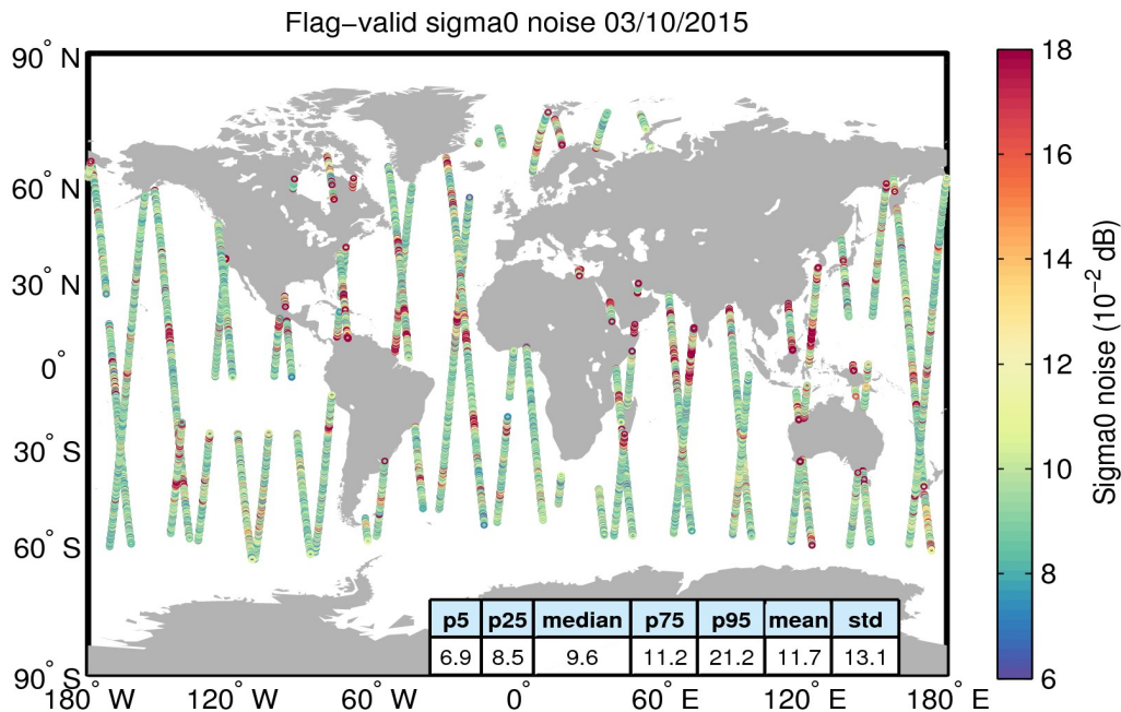
Figure 26. Geographical distribution of flag-valid 20-Hz sigma0 measurement noise over oceans and lakes for 03/10/2015. The statistical values shown in the table refer to the sigma0 noise and are calculated over all measurements shown in the figure.
