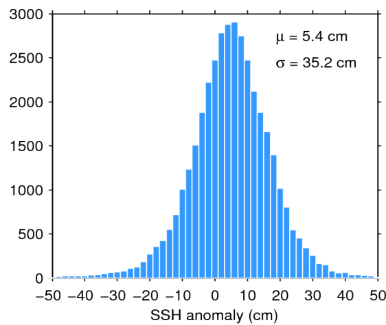
Figure 7. Histogram of flag-valid SSH anomaly over oceans and lakes for 03/10/2015. The mean ( \mu ) and standard deviation ( \sigma ) are also shown. Note that values outside [-50\ 50] cm are excluded from the histogram for the sake of readability but not from the computation of \mu and \sigma .
