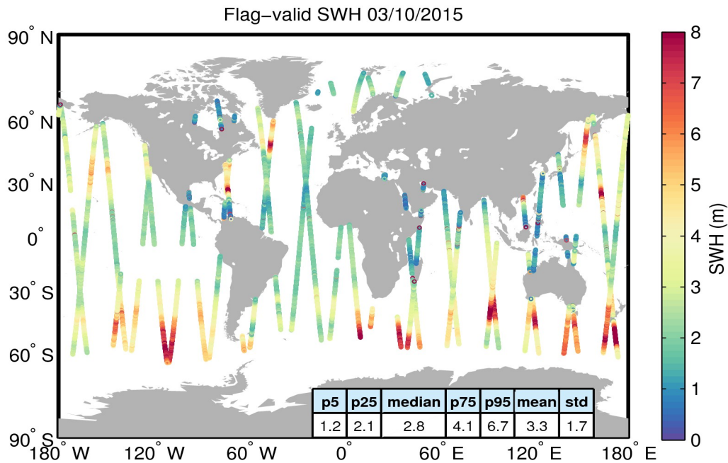
Figure 15. Geographical distribution of flag-valid SWH data over oceans and lakes for 03/10/2015. The statistical values shown in the table refer to the SWH in m and are calculated over all measurements shown in the figure.
