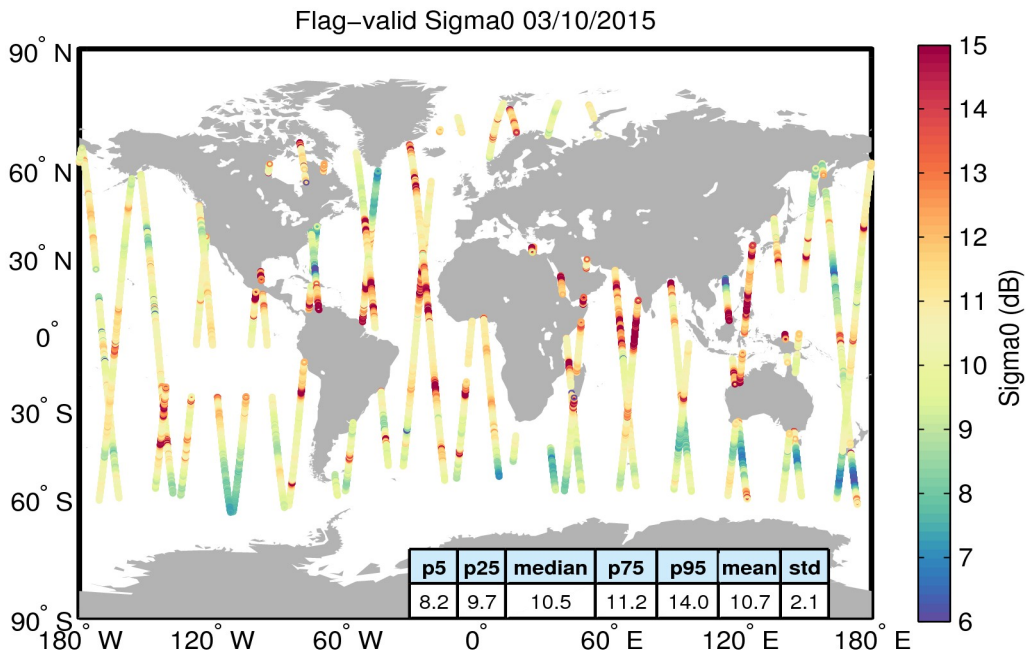
Figure 23. Geographical distribution of flag-valid sigma0 data over oceans and lakes for 03/10/2015. The statistical values shown in the table refer to the sigma0 in dB and are calculated over all measurements shown in the figure.
