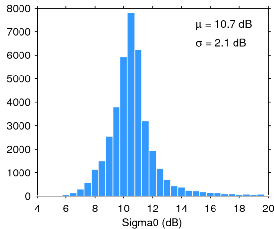
Figure 25. Histogram of flag-valid sigma0 over oceans and lakes for 03/10/2015. The mean ( \mu ) and standard deviation ( \sigma ) are also shown. Note that values outside [4 20] dB are excluded from the histogram for the sake of readability but not from the computation of \mu and \sigma .
