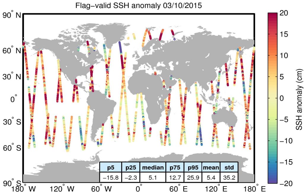
Figure 5. Geographical distribution of flag-valid 1-Hz SSH anomaly data over oceans and lakes for 03/10/2015. The statistical values shown in the table refer to the SSH anomaly in cm and are calculated over all measurements shown in the figure.
