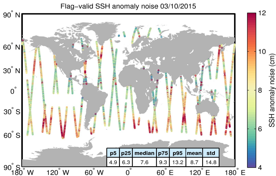
Figure 8. Geographical distribution of flag-valid 20-Hz SSH anomaly measurement noise over oceans and lakes for 03/10/2015. The statistical values shown in the table refer to the SSH anomaly noise and are calculated over all measurements shown in the figure.
