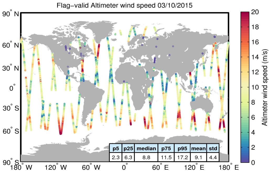
Figure 31. Geographical distribution of flag-valid wind data over oceans and lakes for 03/10/2015. The statistical values shown in the table refer to the wind in m/s and are calculated over all measurements shown in the figure.
