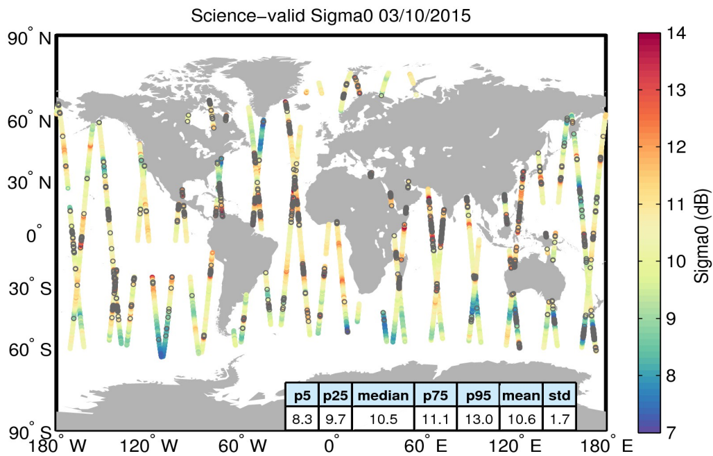
Figure 27. Geographical distribution of science-valid sigma0 data over oceans and lakes for 03/10/2015. The statistical values shown in the table refer to the sigma0 in dB and are calculated over all measurements shown in the figure. Gray circles denote records that have been rejected based on the editing criteria described in Table 4.
