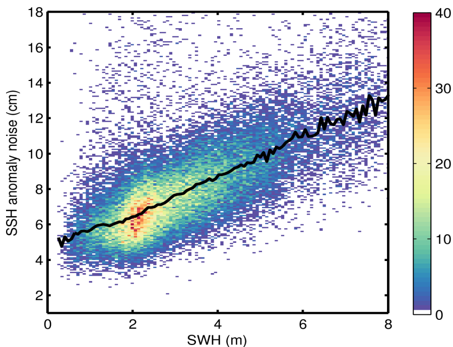
Figure 9. 2D histogram showing flag-valid SSH anomaly noise as a function of SWH for 03/10/2015. The black line denotes the median SSH anomaly noise as a function of SWH.
