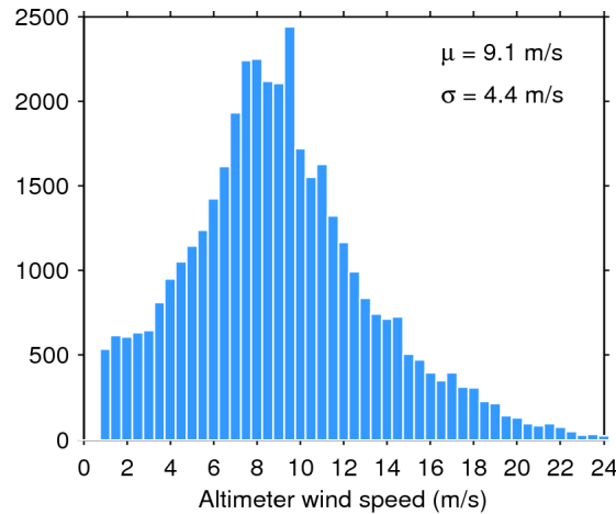
Figure 33. Histogram of flag-valid wind over oceans and lakes for 03/10/2015. The mean ( \mu ) and standard deviation ( \sigma ) are also shown. Note that values larger than 24 m/s are excluded from the histogram for the sake of readability but not from the computation of \mu and \sigma .
