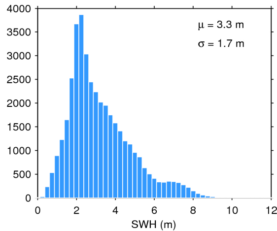
Figure 17. Histogram of flag-valid SWH over oceans and lakes for 03/10/2015. The mean ( \mu ) and standard deviation ( \sigma ) are also shown. Note that values larger than 12 m are excluded from the histogram for the sake of readability but not from the computation of \mu and \sigma .
