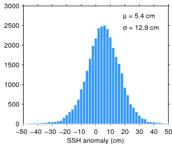
Figure 11. Histogram of science-valid SSH anomaly over oceans and lakes for 03/10/2015. The mean ( \mu ) and standard deviation ( \sigma ) are also shown. Note that values outside [-50 50] cm are excluded from the histogram for the sake of readability but not from the computation of \mu and \sigma .
