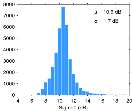
Figure 28. Histogram of science-valid sigma0 over oceans and lakes for 03/10/2015. The mean ( \mu ) and standard deviation ( \sigma ) are also shown. Note that values outside [4 20] dB are excluded from the histogram for the sake of readability but not from the computation of \mu and \sigma .
