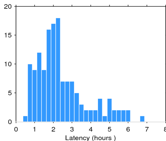
Figure 2. Histogram of the data latency for 03/10/2015. The y-axis denotes the number of files that are made available with a delay of x-hours with respect to the mean time of the records stored in the file.
