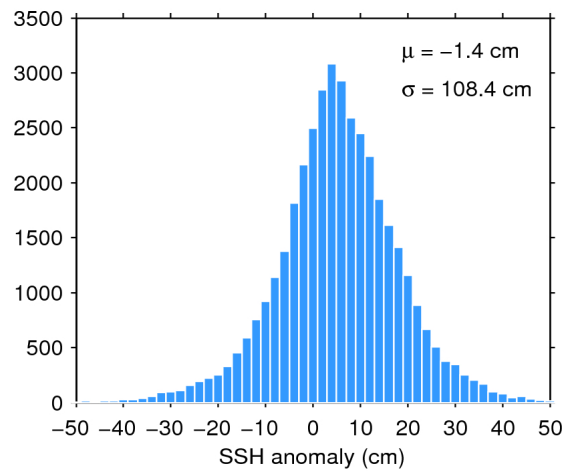
Figure 7. Histogram of flag-valid SSH anomaly over oceans and lakes for 02/10/2015. The mean ( \mu ) and standard deviation ( \sigma ) are also shown. Note that values outside [-50\ 50] cm are excluded from the histogram for the sake of readability but not from the computation of \mu and \sigma .
