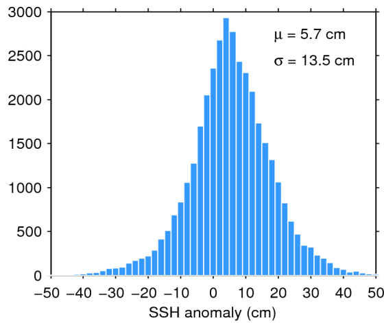
Figure 11. Histogram of science-valid SSH anomaly over oceans and lakes for 02/10/2015. The mean ( \mu ) and standard deviation ( \sigma ) are also shown. Note that values outside [-50 50] cm are excluded from the histogram for the sake of readability but not from the computation of \mu and \sigma .
