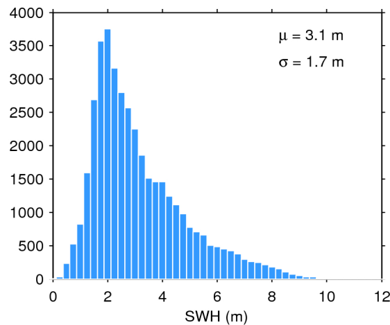
Figure 17. Histogram of flag-valid SWH over oceans and lakes for 02/10/2015. The mean ( \mu ) and standard deviation ( \sigma ) are also shown. Note that values larger than 12 m are excluded from the histogram for the sake of readability but not from the computation of \mu and \sigma .
