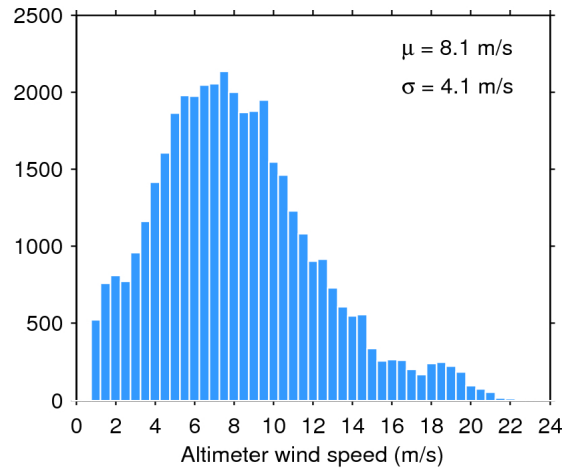
Figure 33. Histogram of flag-valid wind over oceans and lakes for 02/10/2015. The mean ( \mu ) and standard deviation ( \sigma ) are also shown. Note that values larger than 24 m/s are excluded from the histogram for the sake of readability but not from the computation of \mu and \sigma .
