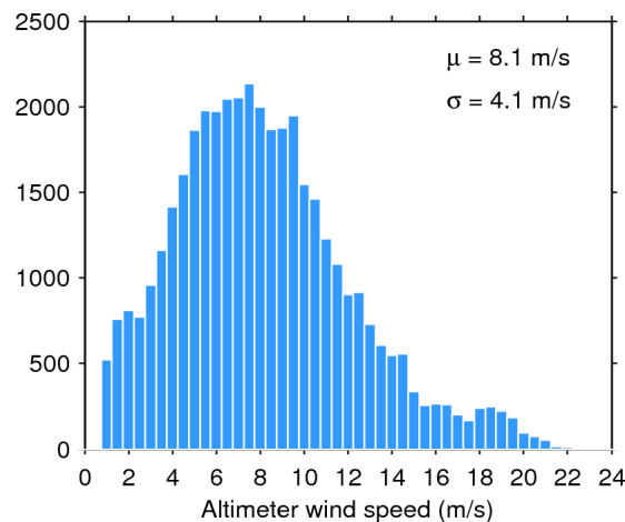
Figure 35. Histogram of science-valid wind over oceans and lakes for 02/10/2015. The mean ( \mu ) and standard deviation ( \sigma ) are also shown. Note that values larger than 24 m/s are excluded from the histogram for the sake of readability but not from the computation of \mu and \sigma .
