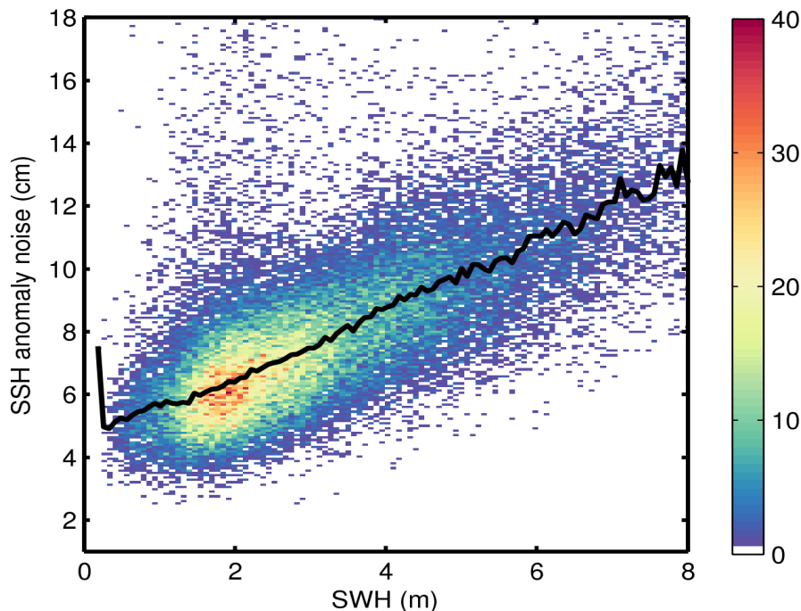
Figure 9. 2D histogram showing flag-valid SSH anomaly noise as a function of SWH for 02/10/2015. The black line denotes the median SSH anomaly noise as a function of SWH.
