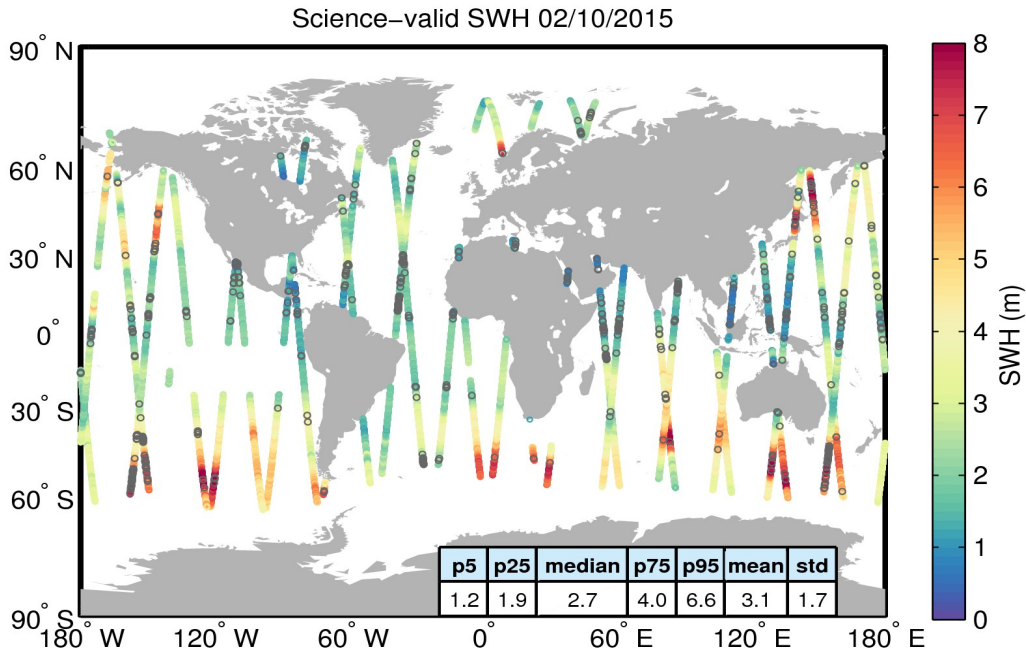
Figure 19. Geographical distribution of science-valid SWH data over oceans and lakes for 02/10/2015. The statistical values shown in the table refer to the SWH in m and are calculated over all measurements shown in the figure. Gray circles denote records that have been rejected based on the editing criteria described in Table 3.
