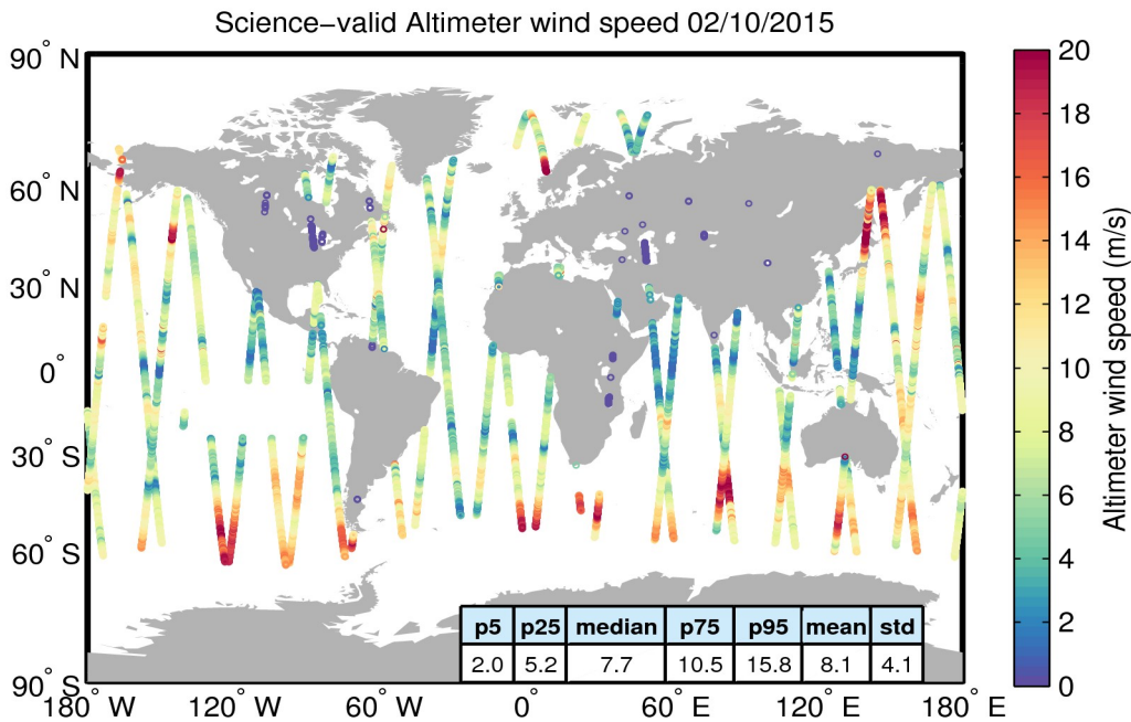
Figure 34. Geographical distribution of science-valid wind data over oceans and lakes for 02/10/2015. The statistical values shown in the table refer to the wind in m/s and are calculated over all measurements shown in the figure. Gray circles denote records that have been rejected based on the editing criteria described in Table 5.
