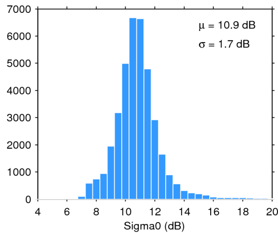
Figure 28. Histogram of science-valid sigma0 over oceans and lakes for 02/10/2015. The mean ( \mu ) and standard deviation ( \sigma ) are also shown. Note that values outside [4 20] dB are excluded from the histogram for the sake of readability but not from the computation of \mu and \sigma .
