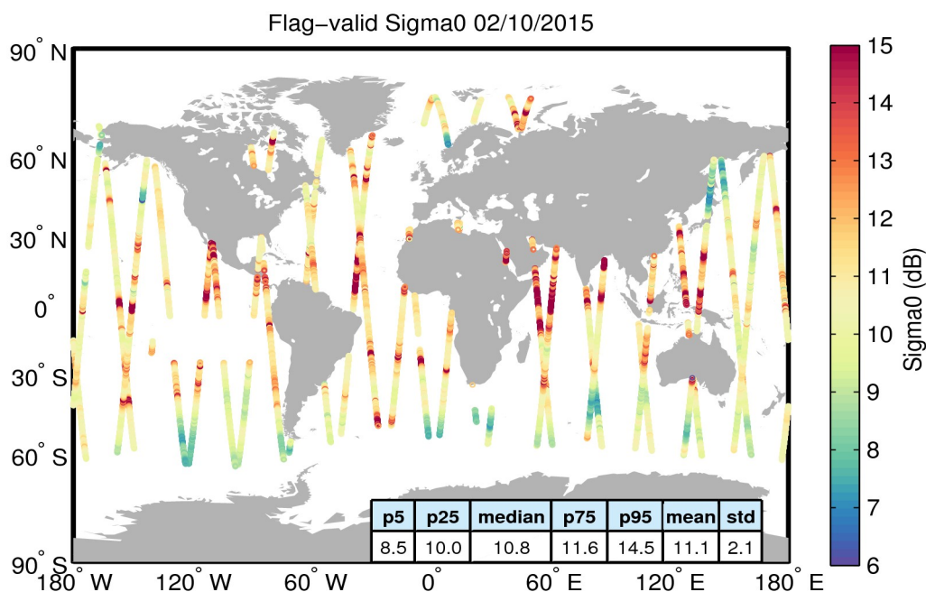
Figure 23. Geographical distribution of flag-valid sigma0 data over oceans and lakes for 02/10/2015. The statistical values shown in the table refer to the sigma0 in dB and are calculated over all measurements shown in the figure.
