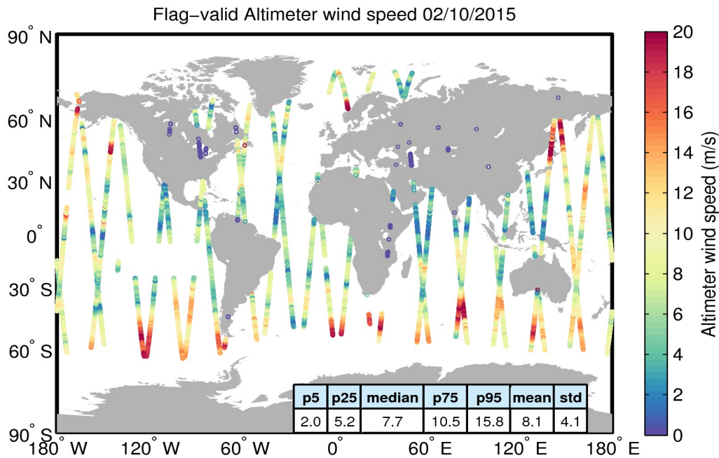
Figure 31. Geographical distribution of flag-valid wind data over oceans and lakes for 02/10/2015. The statistical values shown in the table refer to the wind in m/s and are calculated over all measurements shown in the figure.
