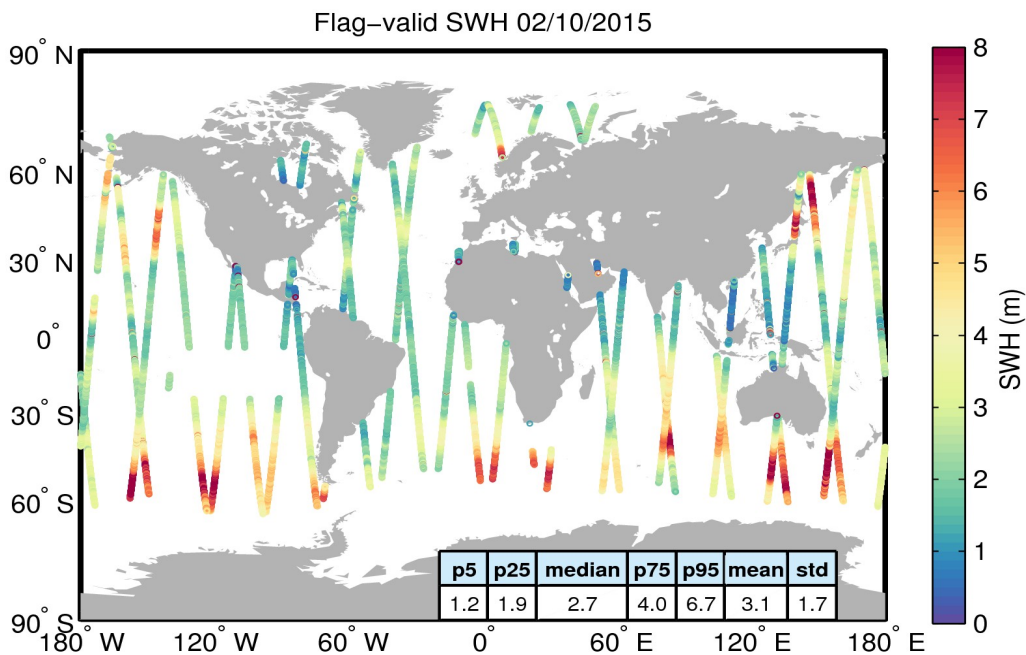
Figure 15. Geographical distribution of flag-valid SWH data over oceans and lakes for 02/10/2015. The statistical values shown in the table refer to the SWH in m and are calculated over all measurements shown in the figure.
