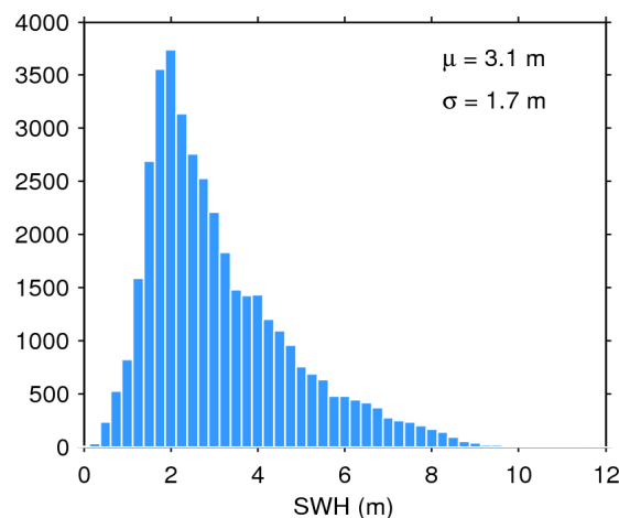
Figure 20. Histogram of science-valid SWH over oceans and lakes for 02/10/2015. The mean ( \mu ) and standard deviation ( \sigma ) are also shown. Note that values larger than 12 m are excluded from the histogram for the sake of readability but not from the computation of \mu and \sigma .
