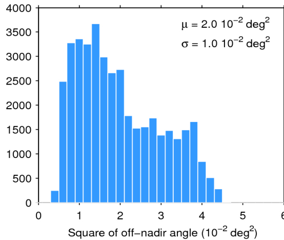
Figure 39. Histogram of flag-valid mispointing over oceans and lakes for 02/10/2015. The mean ( \mu ) and standard deviation ( \sigma ) are also shown. Note that values larger than 6 \cdot 10^{-2} \text{ deg}^2 are excluded from the histogram for the sake of readability but not from the computation of \mu and \sigma .
