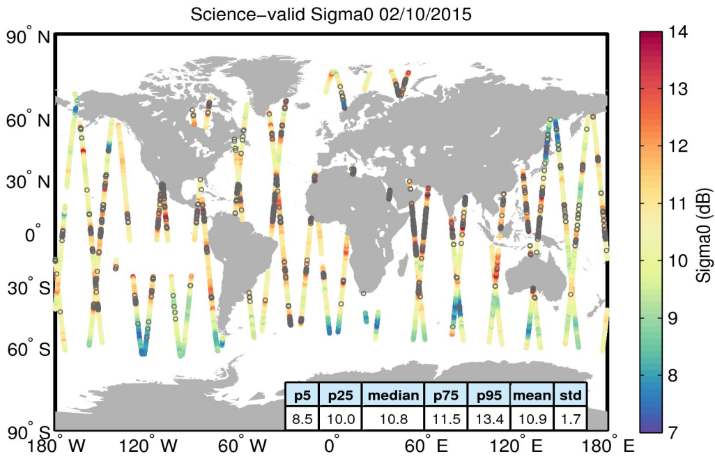
Figure 27. Geographical distribution of science-valid sigma0 data over oceans and lakes for 02/10/2015. The statistical values shown in the table refer to the sigma0 in dB and are calculated over all measurements shown in the figure. Gray circles denote records that have been rejected based on the editing criteria described in Table 4.
