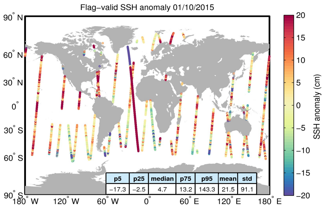
Figure 5. Geographical distribution of flag-valid 1-Hz SSH anomaly data over oceans and lakes for 01/10/2015. The statistical values shown in the table refer to the SSH anomaly in cm and are calculated over all measurements shown in the figure.
