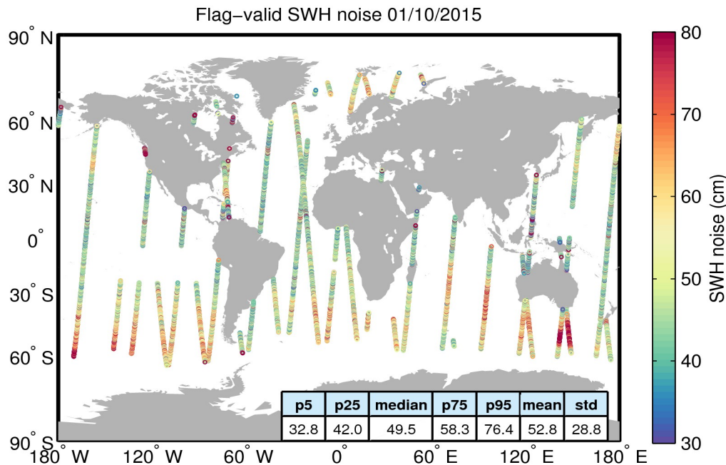
Figure 18. Geographical distribution of flag-valid 20-Hz SWH measurement noise over oceans and lakes for 01/10/2015. The statistical values shown in the table refer to the SWH noise and are calculated over all measurements shown in the figure.
