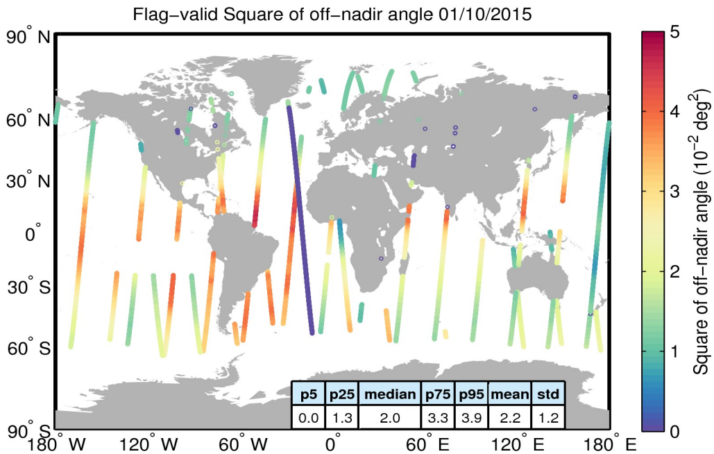
Figure 37. Geographical distribution of flag-valid mispointing data over oceans and lakes for 01/10/2015. The statistical values shown in the table refer to the mispointing in 10^{-2} \text{ deg}^2 and are calculated over all measurements shown in the figure.
