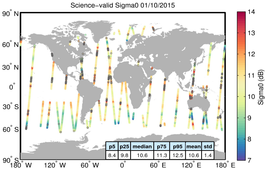
Figure 27. Geographical distribution of science-valid sigma0 data over oceans and lakes for 01/10/2015. The statistical values shown in the table refer to the sigma0 in dB and are calculated over all measurements shown in the figure. Gray circles denote records that have been rejected based on the editing criteria described in Table 4.
