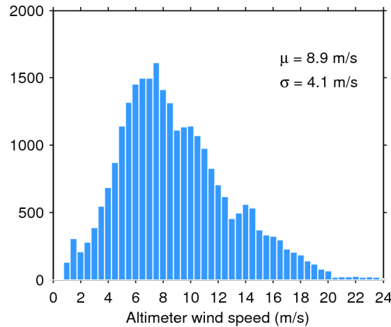
Figure 33. Histogram of flag-valid wind over oceans and lakes for 01/10/2015. The mean ( \mu ) and standard deviation ( \sigma ) are also shown. Note that values larger than 24 m/s are excluded from the histogram for the sake of readability but not from the computation of \mu and \sigma .
