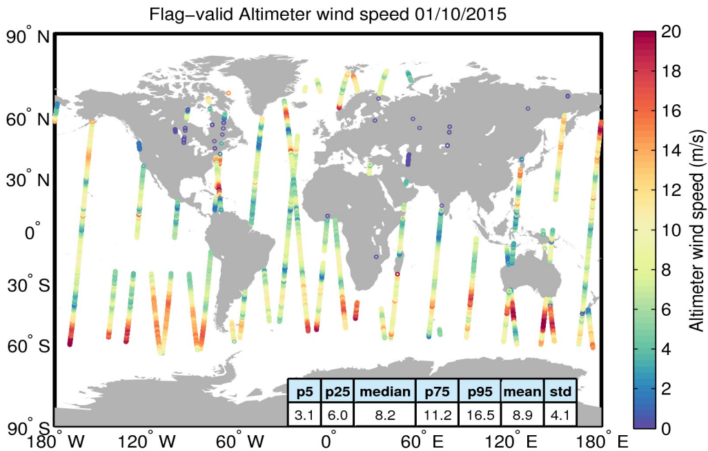
Figure 31. Geographical distribution of flag-valid wind data over oceans and lakes for 01/10/2015. The statistical values shown in the table refer to the wind in m/s and are calculated over all measurements shown in the figure.
