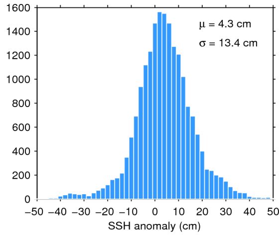
Figure 11. Histogram of science-valid SSH anomaly over oceans and lakes for 01/10/2015. The mean ( \mu ) and standard deviation ( \sigma ) are also shown. Note that values outside [-50 50] cm are excluded from the histogram for the sake of readability but not from the computation of \mu and \sigma .
