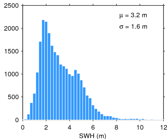
Figure 20. Histogram of science-valid SWH over oceans and lakes for 01/10/2015. The mean ( \mu ) and standard deviation ( \sigma ) are also shown. Note that values larger than 12 m are excluded from the histogram for the sake of readability but not from the computation of \mu and \sigma .
