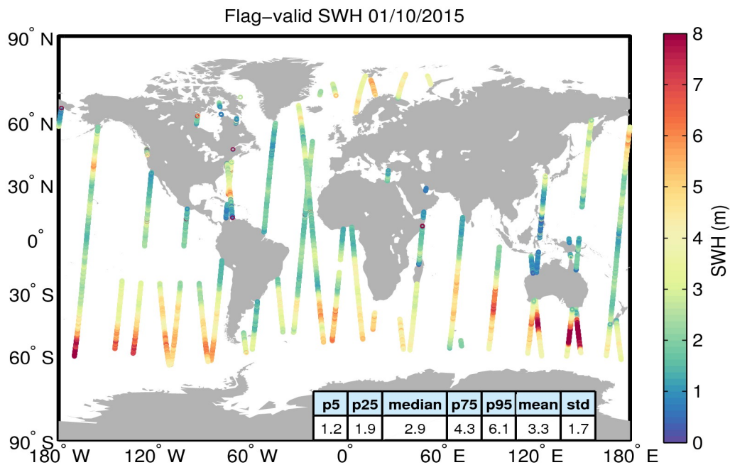
Figure 15. Geographical distribution of flag-valid SWH data over oceans and lakes for 01/10/2015. The statistical values shown in the table refer to the SWH in m and are calculated over all measurements shown in the figure.
