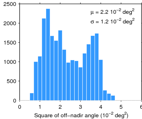
Figure 39. Histogram of flag-valid mispointing over oceans and lakes for 01/10/2015. The mean ( \mu ) and standard deviation ( \sigma ) are also shown. Note that values larger than 6 \cdot 10^{-2} \text{ deg}^2 are excluded from the histogram for the sake of readability but not from the computation of \mu and \sigma .
