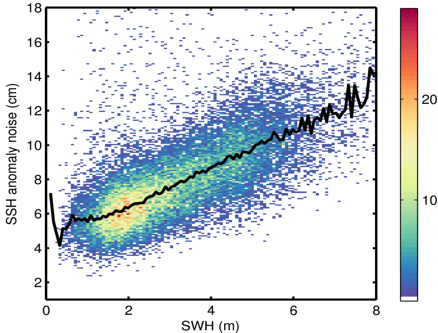
Figure 9. 2D histogram showing flag-valid SSH anomaly noise as a function of SWH for 01/10/2015. The black line denotes the median SSH anomaly noise as a function of SWH.
