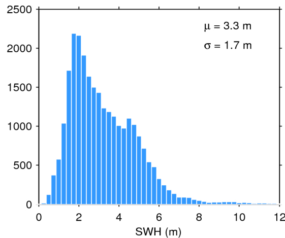
Figure 17. Histogram of flag-valid SWH over oceans and lakes for 01/10/2015. The mean ( \mu ) and standard deviation ( \sigma ) are also shown. Note that values larger than 12 m are excluded from the histogram for the sake of readability but not from the computation of \mu and \sigma .
