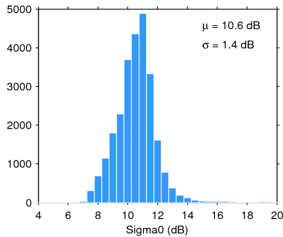
Figure 28. Histogram of science-valid sigma0 over oceans and lakes for 01/10/2015. The mean ( \mu ) and standard deviation ( \sigma ) are also shown. Note that values outside [4 20] dB are excluded from the histogram for the sake of readability but not from the computation of \mu and \sigma .
