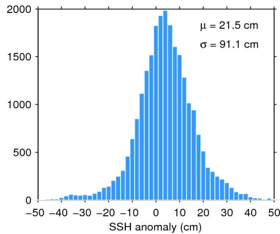
Figure 7. Histogram of flag-valid SSH anomaly over oceans and lakes for 01/10/2015. The mean ( \mu ) and standard deviation ( \sigma ) are also shown. Note that values outside [-50\ 50] cm are excluded from the histogram for the sake of readability but not from the computation of \mu and \sigma .
