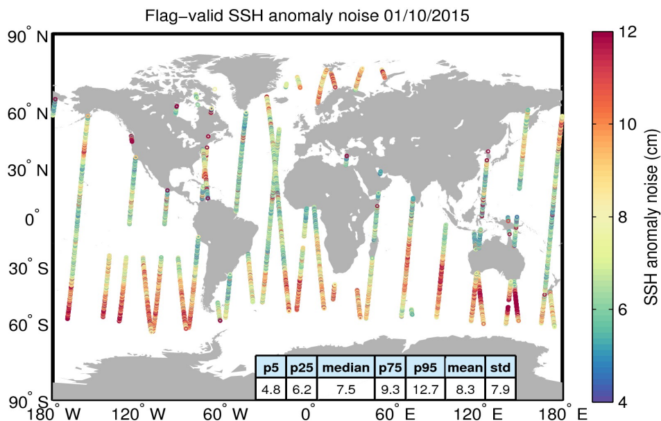
Figure 8. Geographical distribution of flag-valid 20-Hz SSH anomaly measurement noise over oceans and lakes for 01/10/2015. The statistical values shown in the table refer to the SSH anomaly noise and are calculated over all measurements shown in the figure.
