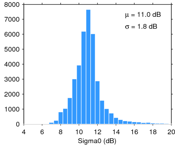
Figure 25. Histogram of flag-valid sigma0 over oceans and lakes for 30/09/2015. The mean ( \mu ) and standard deviation ( \sigma ) are also shown. Note that values outside [4 20] dB are excluded from the histogram for the sake of readability but not from the computation of \mu and \sigma .
