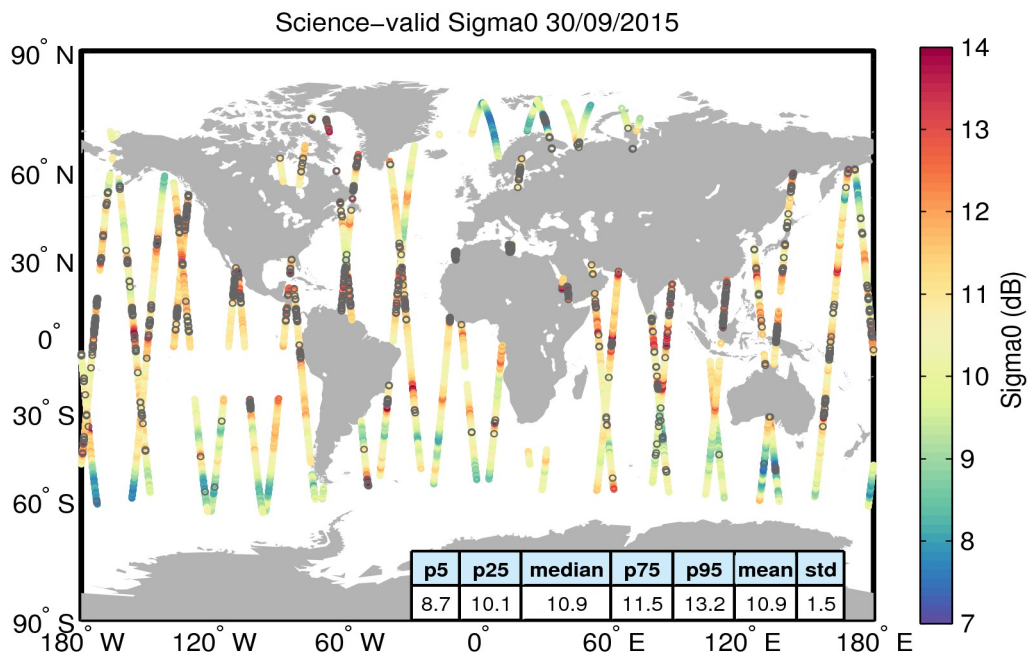
Figure 27. Geographical distribution of science-valid sigma0 data over oceans and lakes for 30/09/2015. The statistical values shown in the table refer to the sigma0 in dB and are calculated over all measurements shown in the figure. Gray circles denote records that have been rejected based on the editing criteria described in Table 4.
