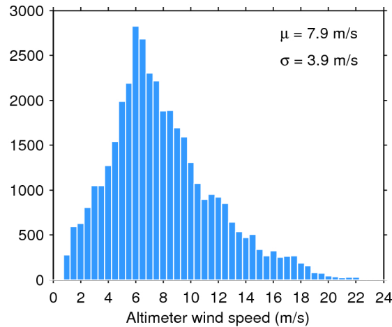
Figure 33. Histogram of flag-valid wind over oceans and lakes for 30/09/2015. The mean ( \mu ) and standard deviation ( \sigma ) are also shown. Note that values larger than 24 m/s are excluded from the histogram for the sake of readability but not from the computation of \mu and \sigma .
