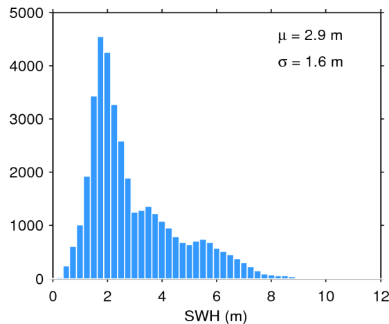
Figure 20. Histogram of science-valid SWH over oceans and lakes for 30/09/2015. The mean ( \mu ) and standard deviation ( \sigma ) are also shown. Note that values larger than 12 m are excluded from the histogram for the sake of readability but not from the computation of \mu and \sigma .
