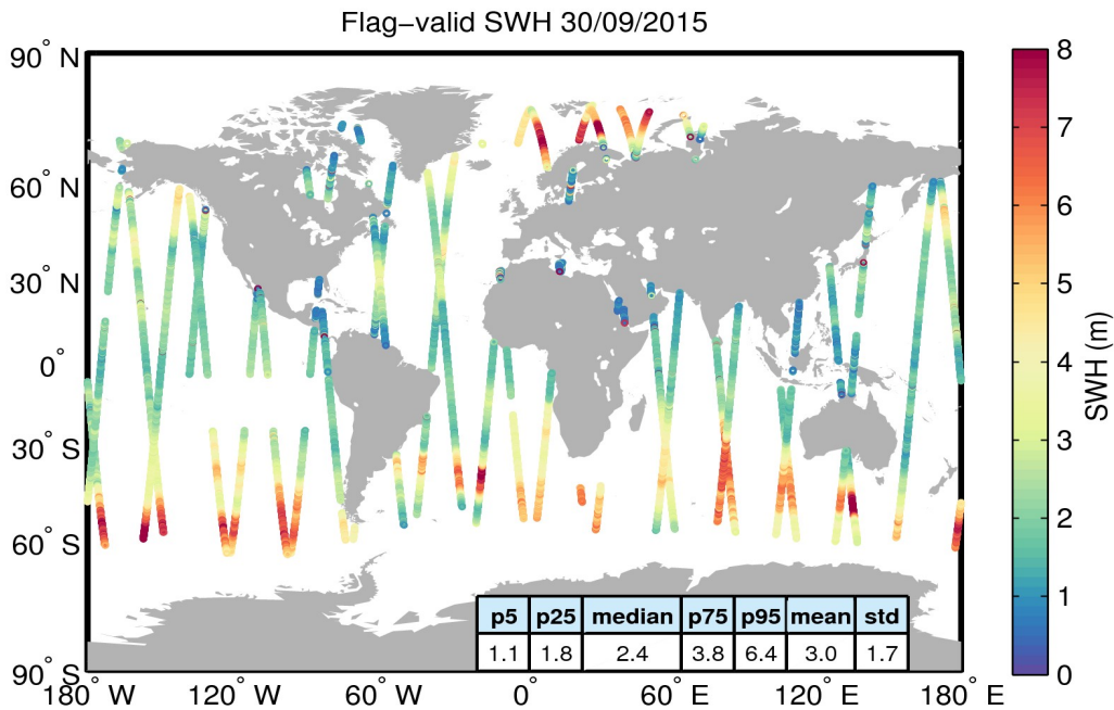
Figure 15. Geographical distribution of flag-valid SWH data over oceans and lakes for 30/09/2015. The statistical values shown in the table refer to the SWH in m and are calculated over all measurements shown in the figure.
