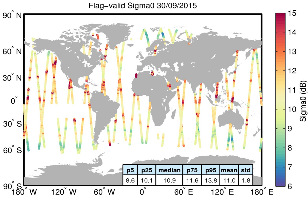
Figure 23. Geographical distribution of flag-valid sigma0 data over oceans and lakes for 30/09/2015. The statistical values shown in the table refer to the sigma0 in dB and are calculated over all measurements shown in the figure.
