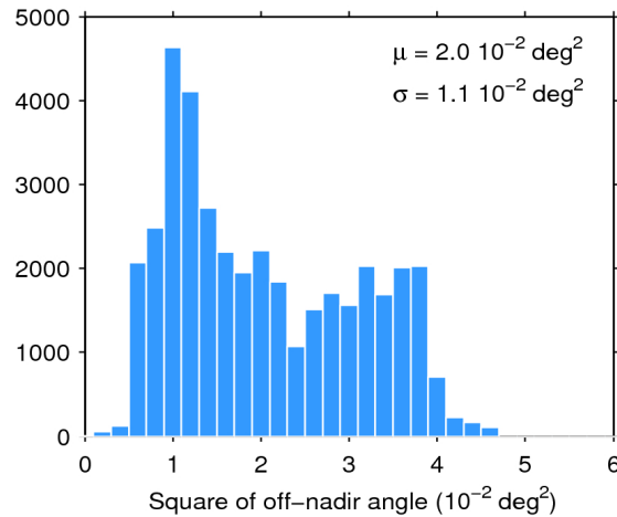
Figure 39. Histogram of flag-valid mispointing over oceans and lakes for 30/09/2015. The mean ( \mu ) and standard deviation ( \sigma ) are also shown. Note that values larger than 6 \cdot 10^{-2} \text{ deg}^2 are excluded from the histogram for the sake of readability but not from the computation of \mu and \sigma .
