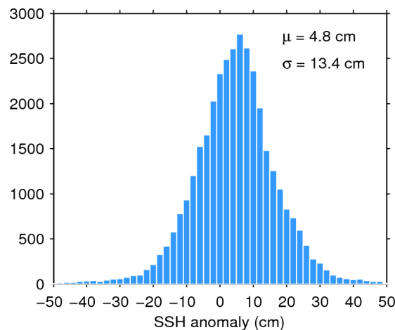
Figure 11. Histogram of science-valid SSH anomaly over oceans and lakes for 30/09/2015. The mean ( \mu ) and standard deviation ( \sigma ) are also shown. Note that values outside [-50 50] cm are excluded from the histogram for the sake of readability but not from the computation of \mu and \sigma .
