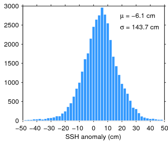
Figure 7. Histogram of flag-valid SSH anomaly over oceans and lakes for 30/09/2015. The mean ( \mu ) and standard deviation ( \sigma ) are also shown. Note that values outside [-50 50] cm are excluded from the histogram for the sake of readability but not from the computation of \mu and \sigma .
