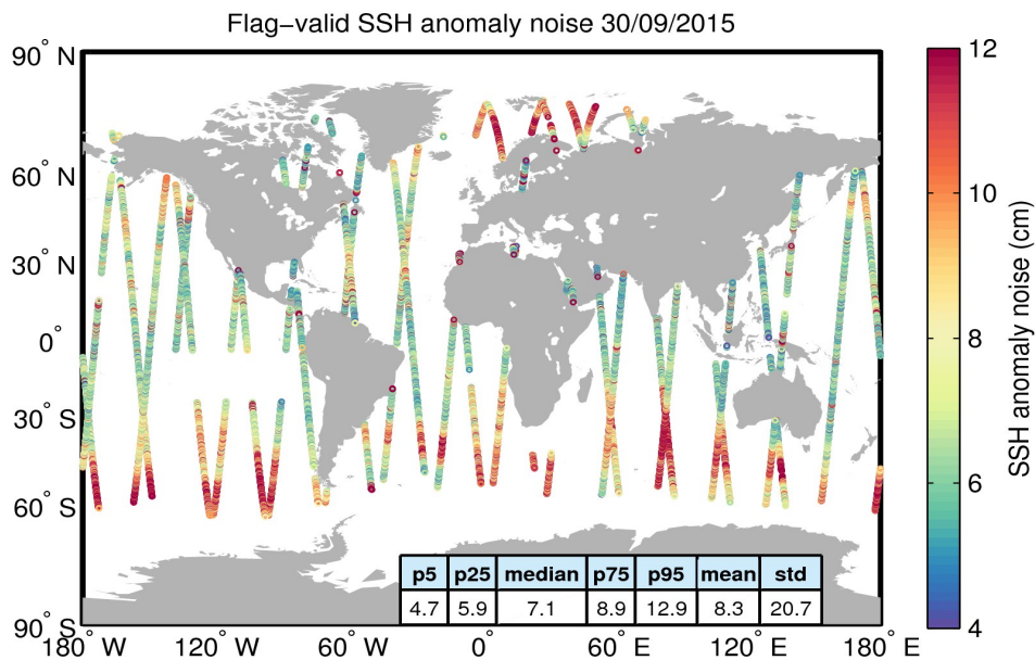
Figure 8. Geographical distribution of flag-valid 20-Hz SSH anomaly measurement noise over oceans and lakes for 30/09/2015. The statistical values shown in the table refer to the SSH anomaly noise and are calculated over all measurements shown in the figure.
