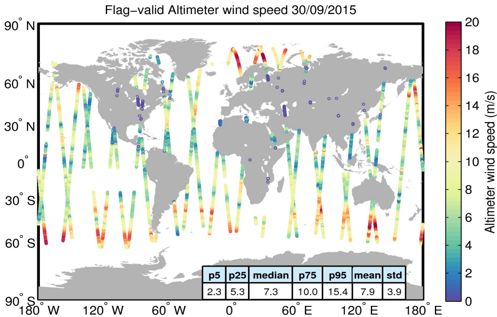
Figure 31. Geographical distribution of flag-valid wind data over oceans and lakes for 30/09/2015. The statistical values shown in the table refer to the wind in m/s and are calculated over all measurements shown in the figure.
