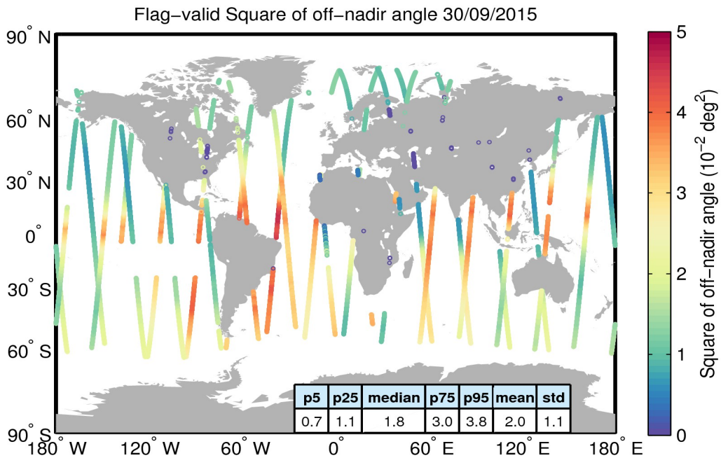
Figure 37. Geographical distribution of flag-valid mispointing data over oceans and lakes for 30/09/2015. The statistical values shown in the table refer to the mispointing in 10^{-2} deg 2 and are calculated over all measurements shown in the figure.
