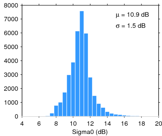
Figure 28. Histogram of science-valid sigma0 over oceans and lakes for 30/09/2015. The mean ( \mu ) and standard deviation ( \sigma ) are also shown. Note that values outside [4 20] dB are excluded from the histogram for the sake of readability but not from the computation of \mu and \sigma .
