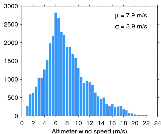
Figure 35. Histogram of science-valid wind over oceans and lakes for 30/09/2015. The mean ( \mu ) and standard deviation ( \sigma ) are also shown. Note that values larger than 24 m/s are excluded from the histogram for the sake of readability but not from the computation of \mu and \sigma .
