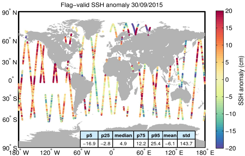
Figure 5. Geographical distribution of flag-valid 1-Hz SSH anomaly data over oceans and lakes for 30/09/2015. The statistical values shown in the table refer to the SSH anomaly in cm and are calculated over all measurements shown in the figure.
