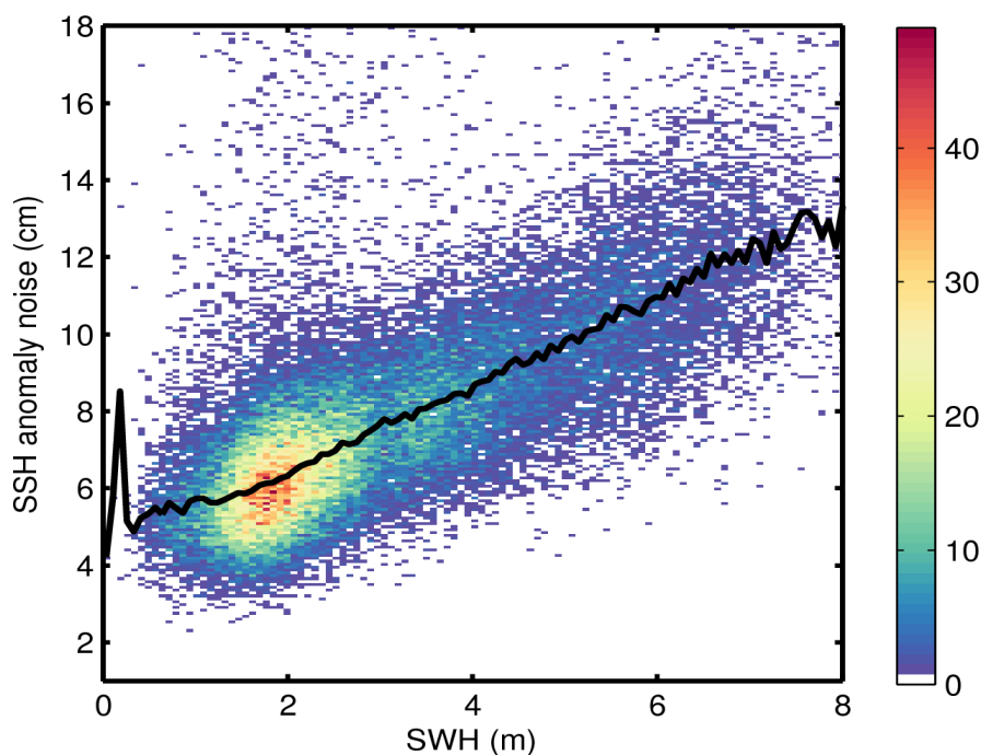
Figure 9. 2D histogram showing flag-valid SSH anomaly noise as a function of SWH for 30/09/2015. The black line denotes the median SSH anomaly noise as a function of SWH.
