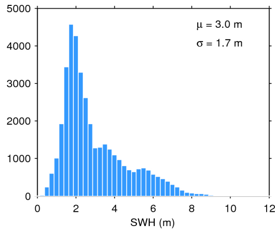
Figure 17. Histogram of flag-valid SWH over oceans and lakes for 30/09/2015. The mean ( \mu ) and standard deviation ( \sigma ) are also shown. Note that values larger than 12 m are excluded from the histogram for the sake of readability but not from the computation of \mu and \sigma .
