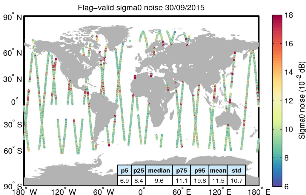
Figure 26. Geographical distribution of flag-valid 20-Hz sigma0 measurement noise over oceans and lakes for 30/09/2015. The statistical values shown in the table refer to the sigma0 noise and are calculated over all measurements shown in the figure.
