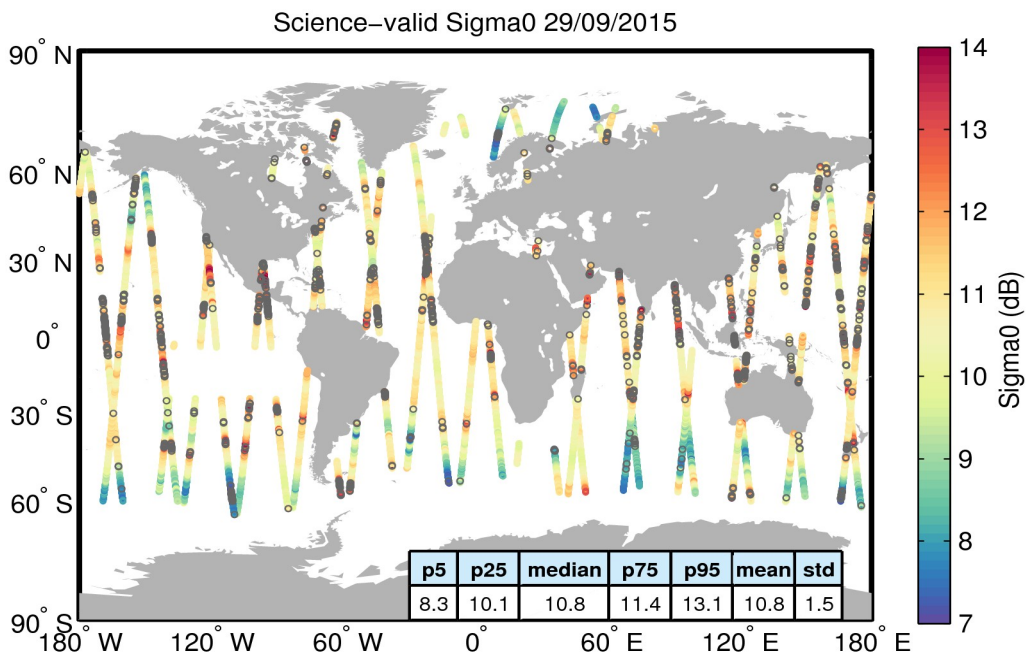
Figure 27. Geographical distribution of science-valid sigma0 data over oceans and lakes for 29/09/2015. The statistical values shown in the table refer to the sigma0 in dB and are calculated over all measurements shown in the figure. Gray circles denote records that have been rejected based on the editing criteria described in Table 4.
