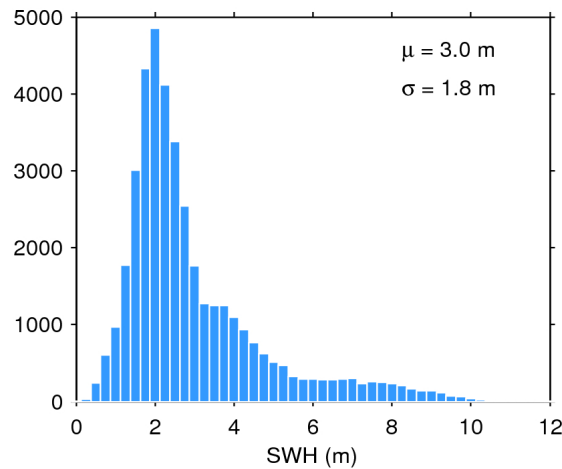
Figure 17. Histogram of flag-valid SWH over oceans and lakes for 29/09/2015. The mean ( \mu ) and standard deviation ( \sigma ) are also shown. Note that values larger than 12 m are excluded from the histogram for the sake of readability but not from the computation of \mu and \sigma .
