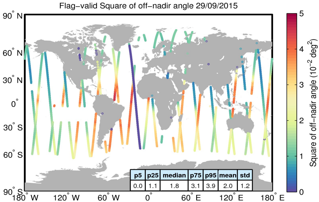
Figure 37. Geographical distribution of flag-valid mispointing data over oceans and lakes for 29/09/2015. The statistical values shown in the table refer to the mispointing in 10^{-2} \text{ deg}^2 and are calculated over all measurements shown in the figure.
