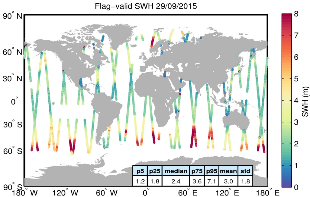
Figure 15. Geographical distribution of flag-valid SWH data over oceans and lakes for 29/09/2015. The statistical values shown in the table refer to the SWH in m and are calculated over all measurements shown in the figure.
