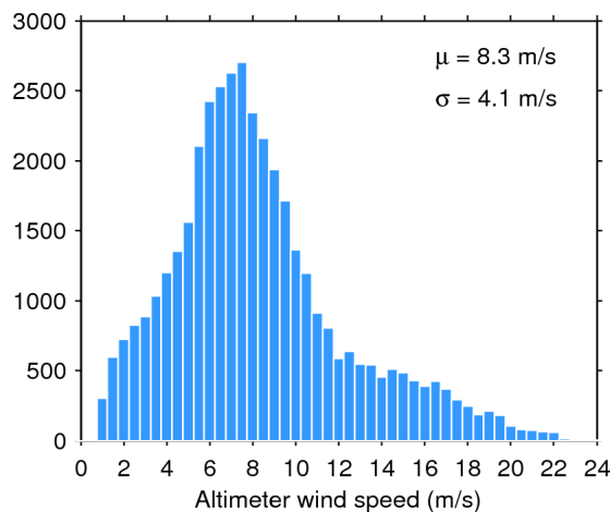
Figure 35. Histogram of science-valid wind over oceans and lakes for 29/09/2015. The mean ( \mu ) and standard deviation ( \sigma ) are also shown. Note that values larger than 24 m/s are excluded from the histogram for the sake of readability but not from the computation of \mu and \sigma .
