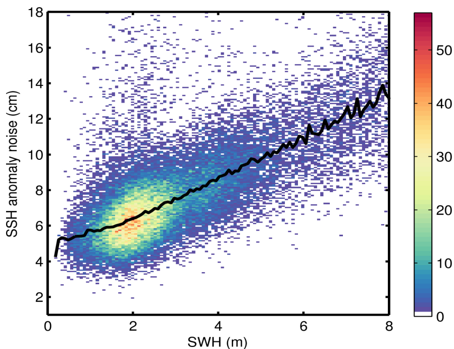
Figure 9. 2D histogram showing flag-valid SSH anomaly noise as a function of SWH for 29/09/2015. The black line denotes the median SSH anomaly noise as a function of SWH.
