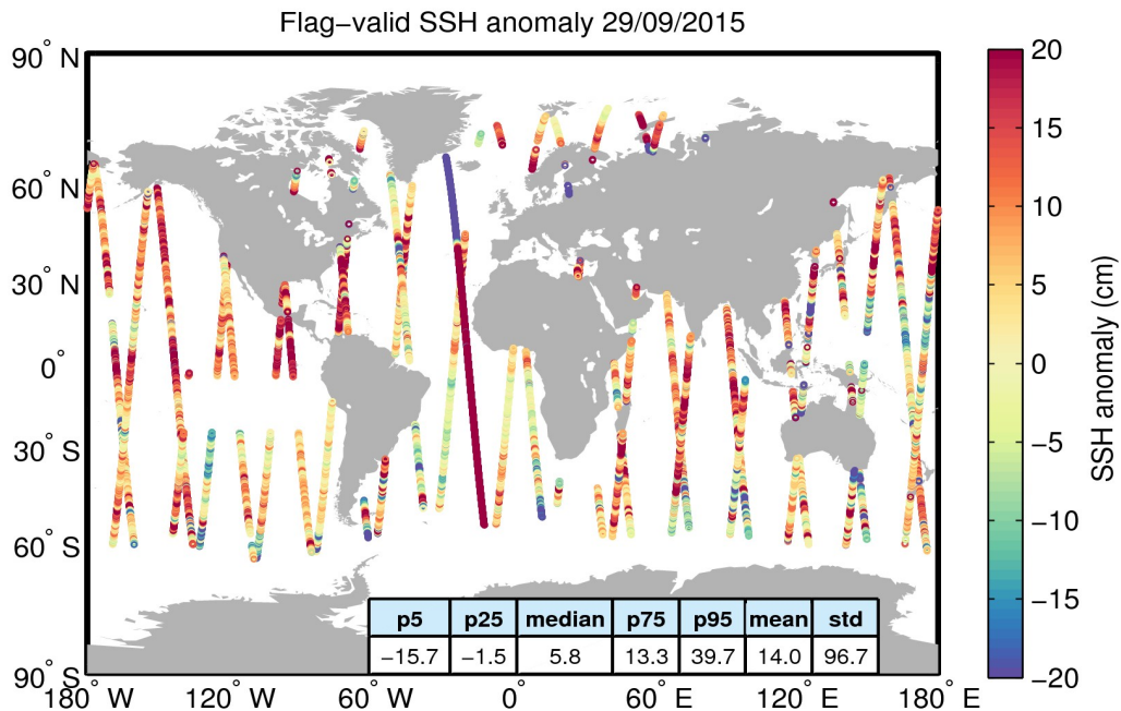
Figure 5. Geographical distribution of flag-valid 1-Hz SSH anomaly data over oceans and lakes for 29/09/2015. The statistical values shown in the table refer to the SSH anomaly in cm and are calculated over all measurements shown in the figure.
