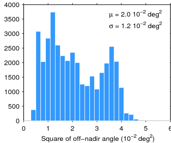
Figure 39. Histogram of flag-valid mispointing over oceans and lakes for 29/09/2015. The mean ( \mu ) and standard deviation ( \sigma ) are also shown. Note that values larger than 6 \cdot 10^{-2} \text{ deg}^2 are excluded from the histogram for the sake of readability but not from the computation of \mu and \sigma .
