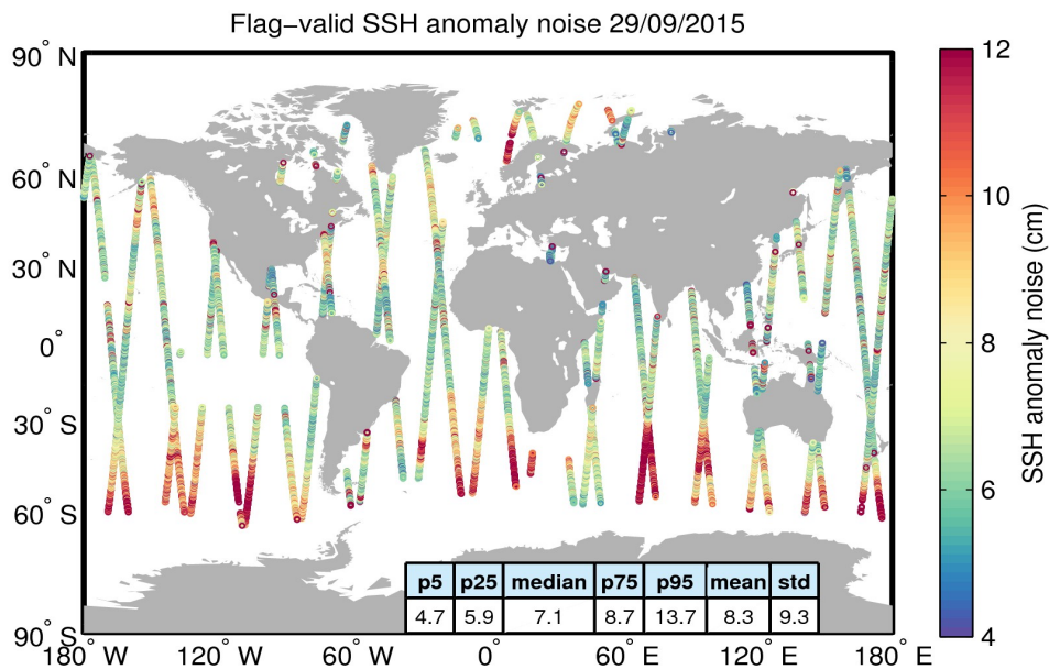
Figure 8. Geographical distribution of flag-valid 20-Hz SSH anomaly measurement noise over oceans and lakes for 29/09/2015. The statistical values shown in the table refer to the SSH anomaly noise and are calculated over all measurements shown in the figure.
