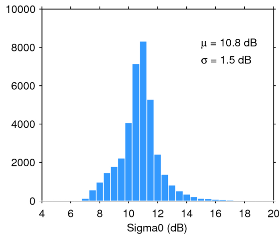
Figure 28. Histogram of science-valid sigma0 over oceans and lakes for 29/09/2015. The mean ( \mu ) and standard deviation ( \sigma ) are also shown. Note that values outside [4 20] dB are excluded from the histogram for the sake of readability but not from the computation of \mu and \sigma .
