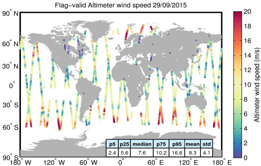
Figure 31. Geographical distribution of flag-valid wind data over oceans and lakes for 29/09/2015. The statistical values shown in the table refer to the wind in m/s and are calculated over all measurements shown in the figure.
