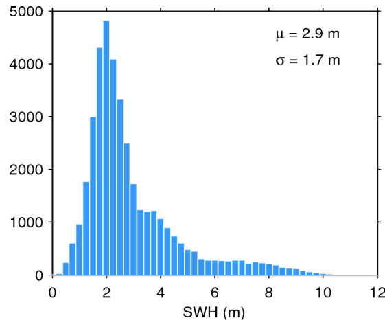
Figure 20. Histogram of science-valid SWH over oceans and lakes for 29/09/2015. The mean ( \mu ) and standard deviation ( \sigma ) are also shown. Note that values larger than 12 m are excluded from the histogram for the sake of readability but not from the computation of \mu and \sigma .
