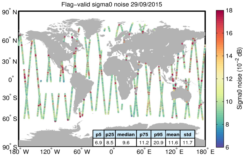
Figure 26. Geographical distribution of flag-valid 20-Hz sigma0 measurement noise over oceans and lakes for 29/09/2015. The statistical values shown in the table refer to the sigma0 noise and are calculated over all measurements shown in the figure.
