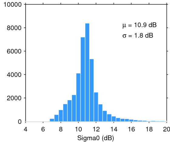
Figure 25. Histogram of flag-valid sigma0 over oceans and lakes for 29/09/2015. The mean ( \mu ) and standard deviation ( \sigma ) are also shown. Note that values outside [4 20] dB are excluded from the histogram for the sake of readability but not from the computation of \mu and \sigma .
