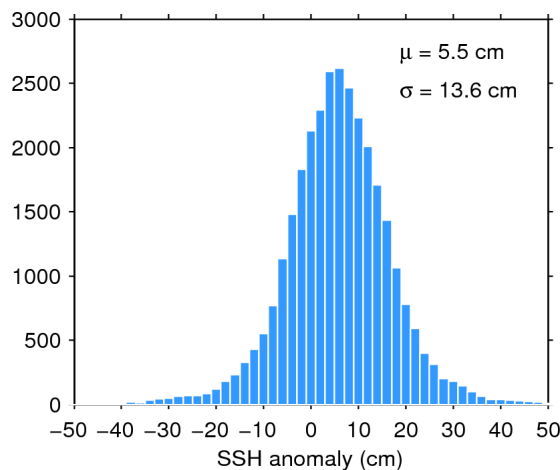
Figure 11. Histogram of science-valid SSH anomaly over oceans and lakes for 29/09/2015. The mean ( \mu ) and standard deviation ( \sigma ) are also shown. Note that values outside [-50 50] cm are excluded from the histogram for the sake of readability but not from the computation of \mu and \sigma .
