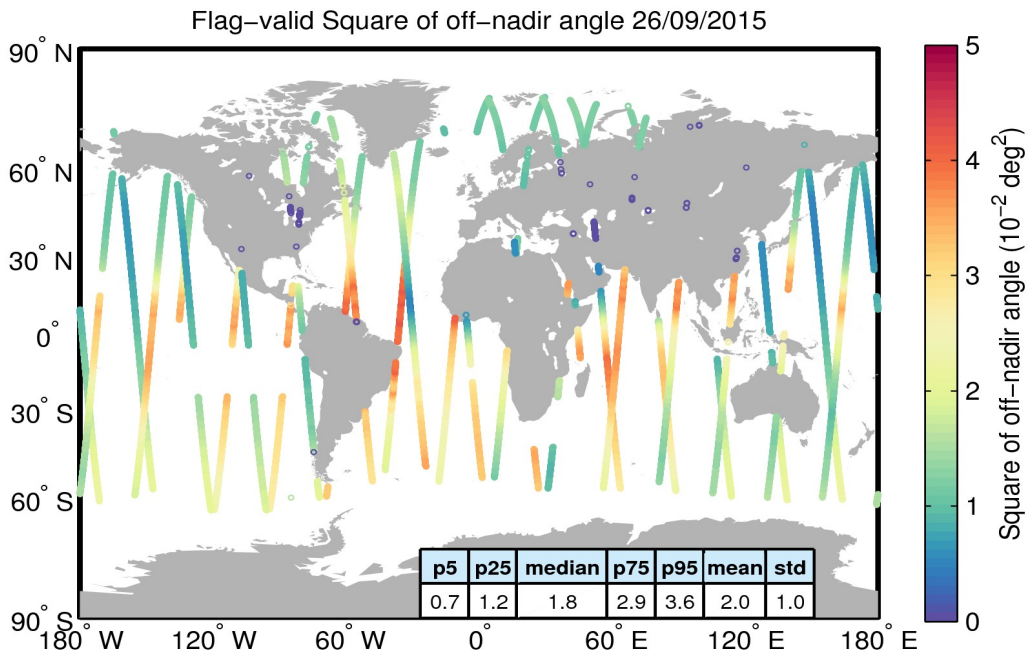
Figure 37. Geographical distribution of flag-valid mispointing data over oceans and lakes for 26/09/2015. The statistical values shown in the table refer to the mispointing in 10^{-2} \text{ deg}^2 and are calculated over all measurements shown in the figure.
