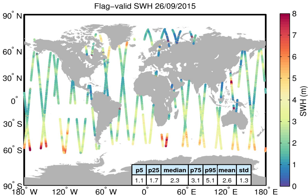
Figure 15. Geographical distribution of flag-valid SWH data over oceans and lakes for 26/09/2015. The statistical values shown in the table refer to the SWH in m and are calculated over all measurements shown in the figure.
