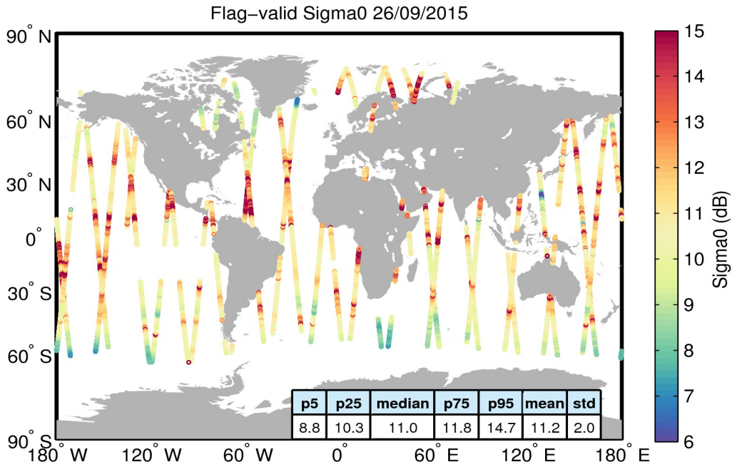
Figure 23. Geographical distribution of flag-valid sigma0 data over oceans and lakes for 26/09/2015. The statistical values shown in the table refer to the sigma0 in dB and are calculated over all measurements shown in the figure.
