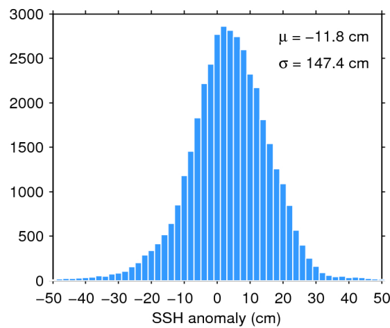
Figure 7. Histogram of flag-valid SSH anomaly over oceans and lakes for 26/09/2015. The mean ( \mu ) and standard deviation ( \sigma ) are also shown. Note that values outside [-50 50] cm are excluded from the histogram for the sake of readability but not from the computation of \mu and \sigma .
