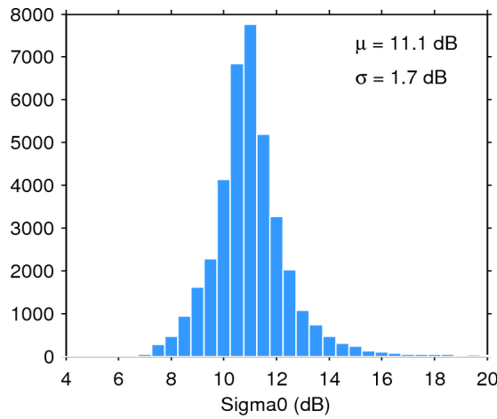
Figure 28. Histogram of science-valid sigma0 over oceans and lakes for 26/09/2015. The mean ( \mu ) and standard deviation ( \sigma ) are also shown. Note that values outside [4 20] dB are excluded from the histogram for the sake of readability but not from the computation of \mu and \sigma .
