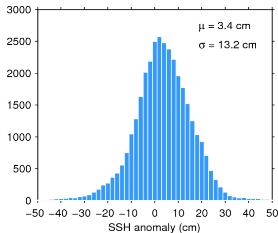
Figure 11. Histogram of science-valid SSH anomaly over oceans and lakes for 26/09/2015. The mean ( \mu ) and standard deviation ( \sigma ) are also shown. Note that values outside [-50 50] cm are excluded from the histogram for the sake of readability but not from the computation of \mu and \sigma .
