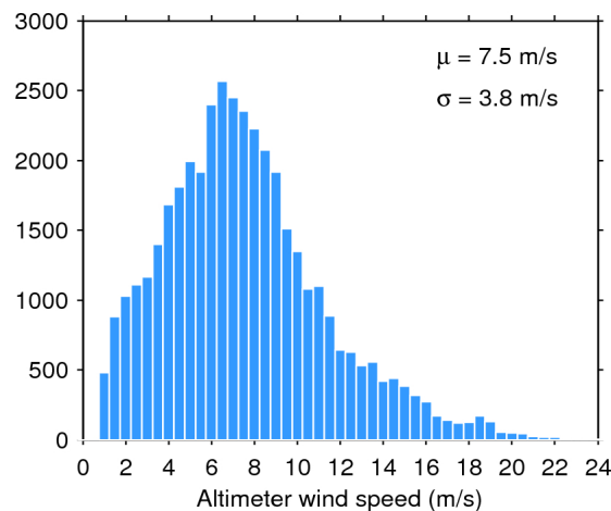
Figure 35. Histogram of science-valid wind over oceans and lakes for 26/09/2015. The mean ( \mu ) and standard deviation ( \sigma ) are also shown. Note that values larger than 24 m/s are excluded from the histogram for the sake of readability but not from the computation of \mu and \sigma .
