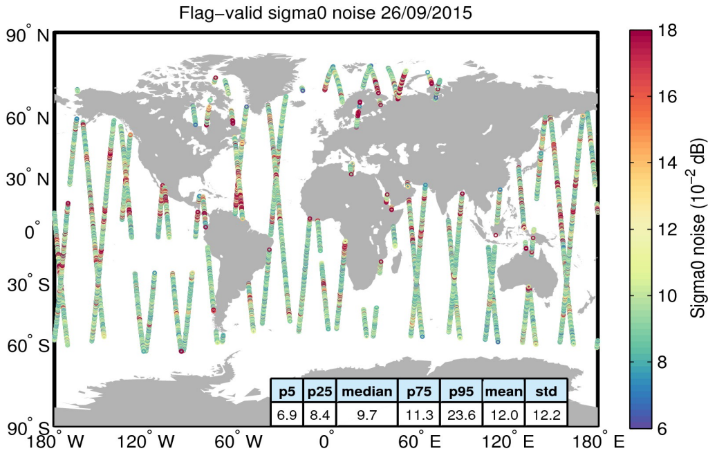
Figure 26. Geographical distribution of flag-valid 20-Hz sigma0 measurement noise over oceans and lakes for 26/09/2015. The statistical values shown in the table refer to the sigma0 noise and are calculated over all measurements shown in the figure.
