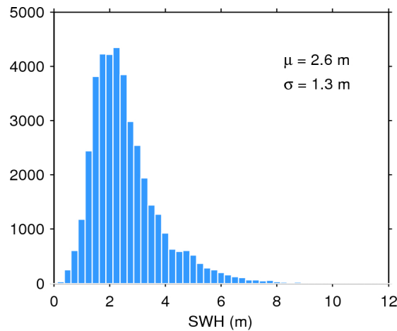
Figure 17. Histogram of flag-valid SWH over oceans and lakes for 26/09/2015. The mean ( \mu ) and standard deviation ( \sigma ) are also shown. Note that values larger than 12 m are excluded from the histogram for the sake of readability but not from the computation of \mu and \sigma .
