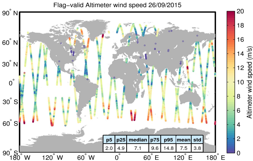
Figure 31. Geographical distribution of flag-valid wind data over oceans and lakes for 26/09/2015. The statistical values shown in the table refer to the wind in m/s and are calculated over all measurements shown in the figure.
