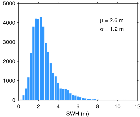
Figure 20. Histogram of science-valid SWH over oceans and lakes for 26/09/2015. The mean ( \mu ) and standard deviation ( \sigma ) are also shown. Note that values larger than 12 m are excluded from the histogram for the sake of readability but not from the computation of \mu and \sigma .
