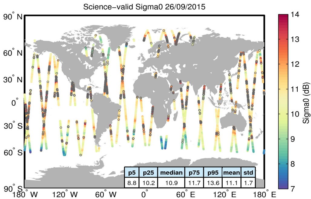
Figure 27. Geographical distribution of science-valid sigma0 data over oceans and lakes for 26/09/2015. The statistical values shown in the table refer to the sigma0 in dB and are calculated over all measurements shown in the figure. Gray circles denote records that have been rejected based on the editing criteria described in Table 4.
