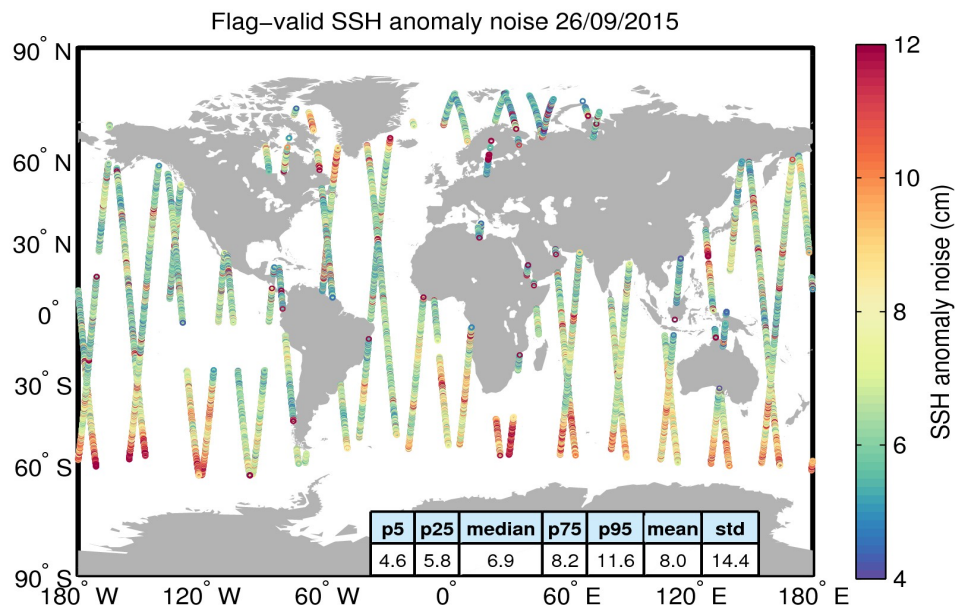
Figure 8. Geographical distribution of flag-valid 20-Hz SSH anomaly measurement noise over oceans and lakes for 26/09/2015. The statistical values shown in the table refer to the SSH anomaly noise and are calculated over all measurements shown in the figure.
