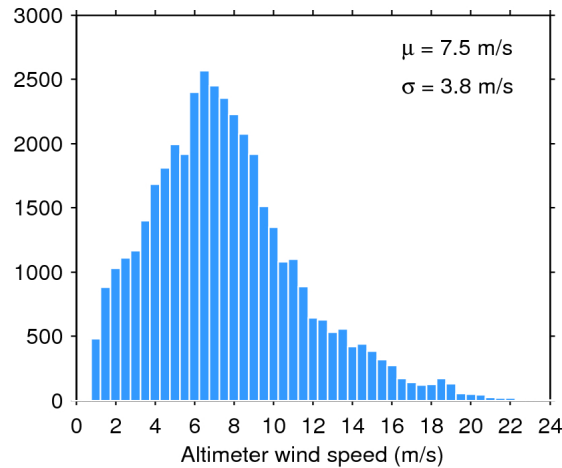
Figure 33. Histogram of flag-valid wind over oceans and lakes for 26/09/2015. The mean ( \mu ) and standard deviation ( \sigma ) are also shown. Note that values larger than 24 m/s are excluded from the histogram for the sake of readability but not from the computation of \mu and \sigma .
