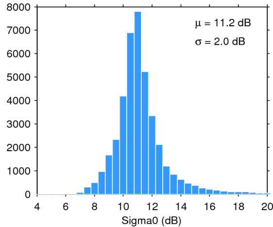
Figure 25. Histogram of flag-valid sigma0 over oceans and lakes for 26/09/2015. The mean ( \mu ) and standard deviation ( \sigma ) are also shown. Note that values outside [4 20] dB are excluded from the histogram for the sake of readability but not from the computation of \mu and \sigma .
