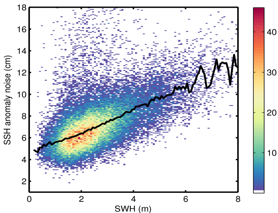
Figure 9. 2D histogram showing flag-valid SSH anomaly noise as a function of SWH for 26/09/2015. The black line denotes the median SSH anomaly noise as a function of SWH.
