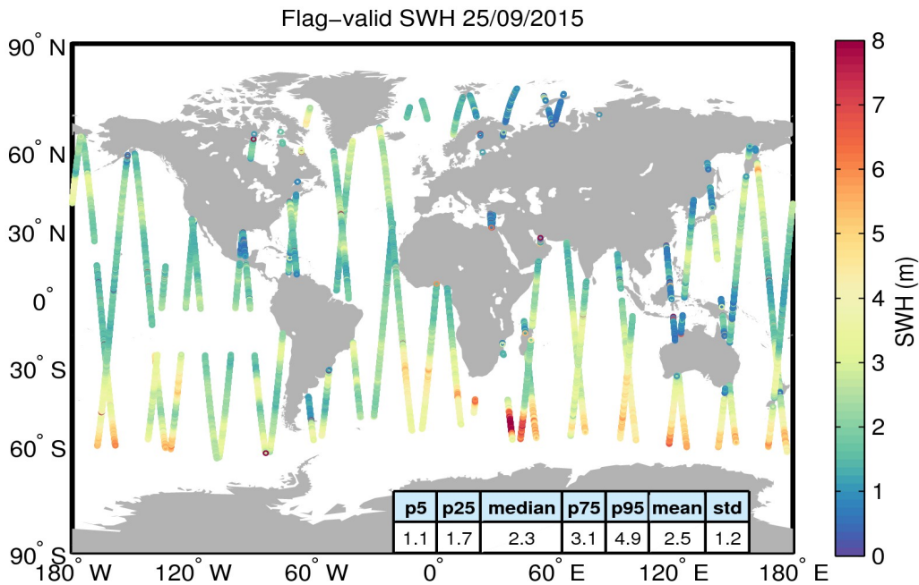
Figure 15. Geographical distribution of flag-valid SWH data over oceans and lakes for 25/09/2015. The statistical values shown in the table refer to the SWH in m and are calculated over all measurements shown in the figure.
