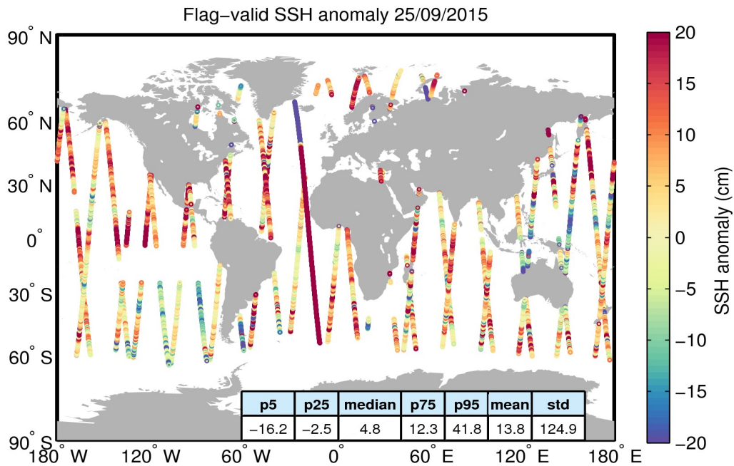
Figure 5. Geographical distribution of flag-valid 1-Hz SSH anomaly data over oceans and lakes for 25/09/2015. The statistical values shown in the table refer to the SSH anomaly in cm and are calculated over all measurements shown in the figure.
