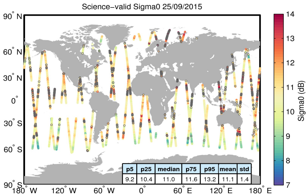
Figure 27. Geographical distribution of science-valid sigma0 data over oceans and lakes for 25/09/2015. The statistical values shown in the table refer to the sigma0 in dB and are calculated over all measurements shown in the figure. Gray circles denote records that have been rejected based on the editing criteria described in Table 4.
