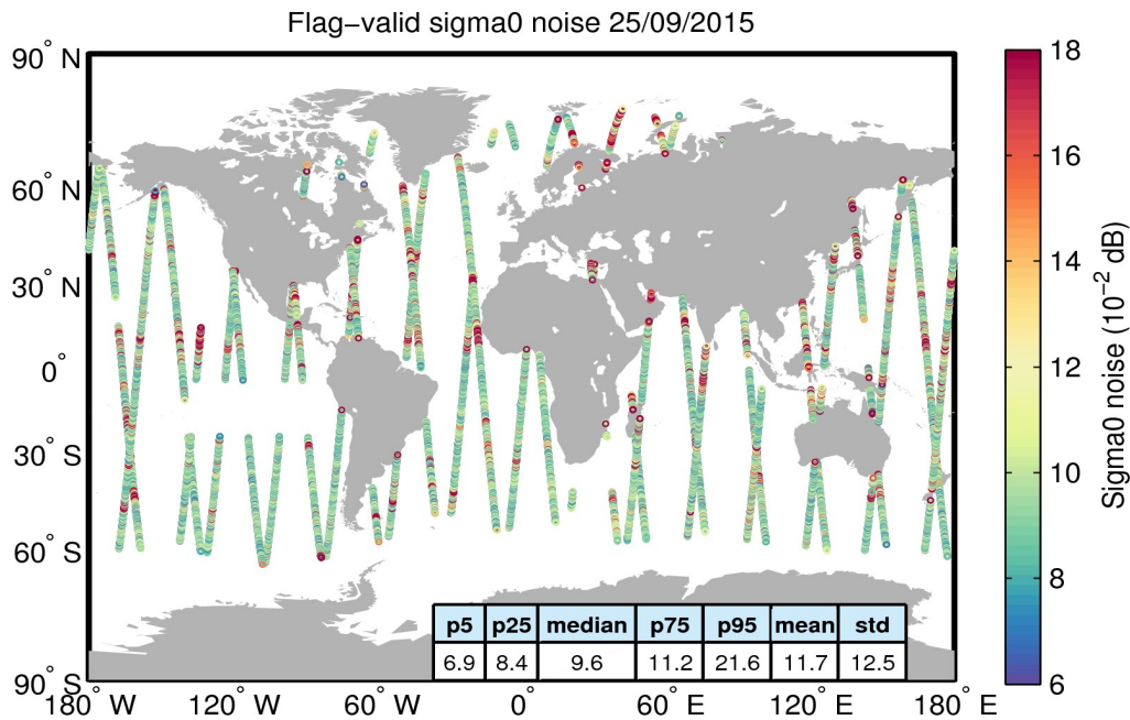
Figure 26. Geographical distribution of flag-valid 20-Hz sigma0 measurement noise over oceans and lakes for 25/09/2015. The statistical values shown in the table refer to the sigma0 noise and are calculated over all measurements shown in the figure.
