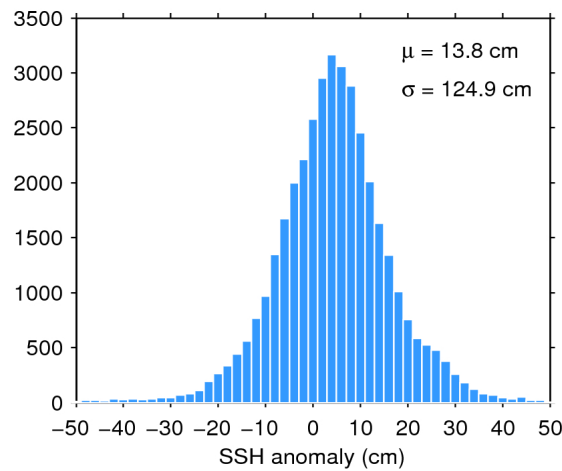
Figure 7. Histogram of flag-valid SSH anomaly over oceans and lakes for 25/09/2015. The mean ( \mu ) and standard deviation ( \sigma ) are also shown. Note that values outside [-50 50] cm are excluded from the histogram for the sake of readability but not from the computation of \mu and \sigma .
