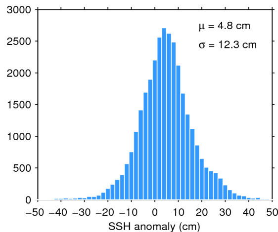
Figure 11. Histogram of science-valid SSH anomaly over oceans and lakes for 25/09/2015. The mean ( \mu ) and standard deviation ( \sigma ) are also shown. Note that values outside [-50 50] cm are excluded from the histogram for the sake of readability but not from the computation of \mu and \sigma .
