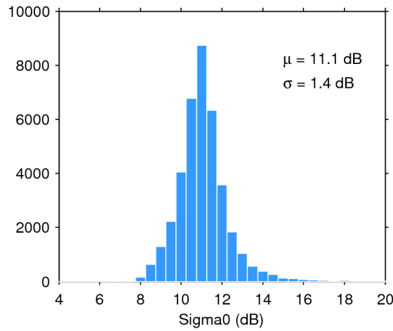
Figure 28. Histogram of science-valid sigma0 over oceans and lakes for 25/09/2015. The mean ( \mu ) and standard deviation ( \sigma ) are also shown. Note that values outside [4 20] dB are excluded from the histogram for the sake of readability but not from the computation of \mu and \sigma .
