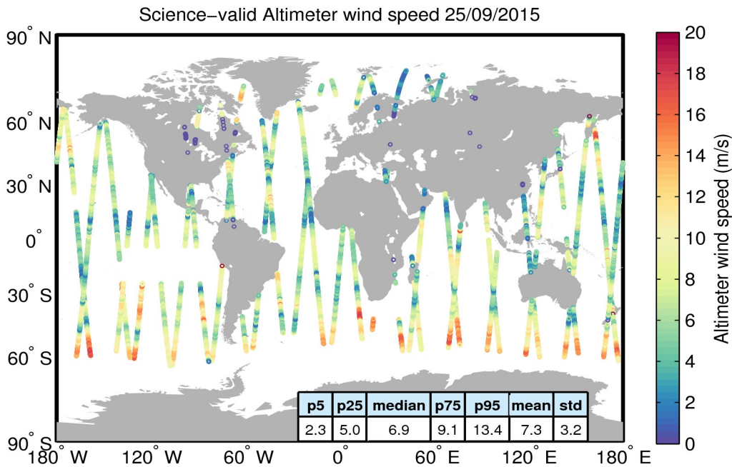
Figure 34. Geographical distribution of science-valid wind data over oceans and lakes for 25/09/2015. The statistical values shown in the table refer to the wind in m/s and are calculated over all measurements shown in the figure. Gray circles denote records that have been rejected based on the editing criteria described in Table 5.
