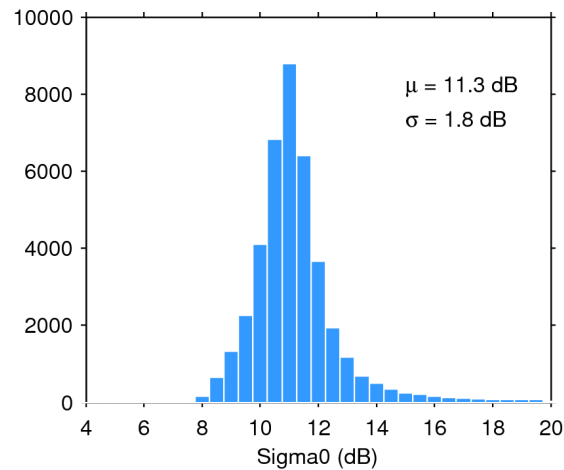
Figure 25. Histogram of flag-valid sigma0 over oceans and lakes for 25/09/2015. The mean ( \mu ) and standard deviation ( \sigma ) are also shown. Note that values outside [4 20] dB are excluded from the histogram for the sake of readability but not from the computation of \mu and \sigma .
