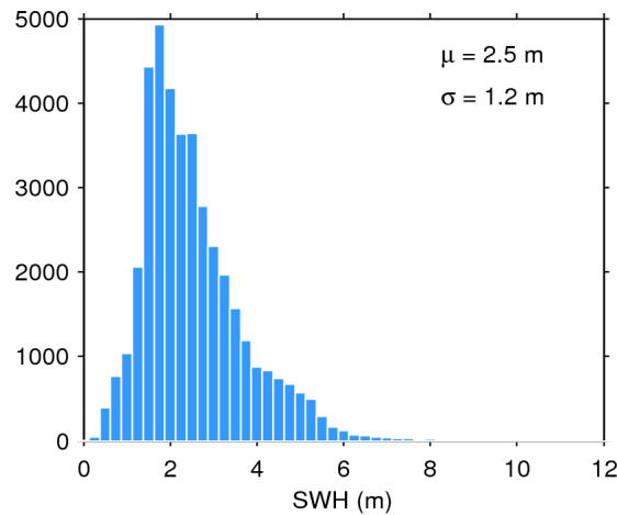
Figure 17. Histogram of flag-valid SWH over oceans and lakes for 25/09/2015. The mean ( \mu ) and standard deviation ( \sigma ) are also shown. Note that values larger than 12 m are excluded from the histogram for the sake of readability but not from the computation of \mu and \sigma .
