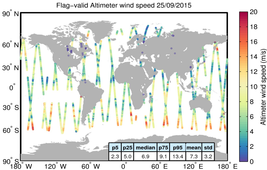
Figure 31. Geographical distribution of flag-valid wind data over oceans and lakes for 25/09/2015. The statistical values shown in the table refer to the wind in m/s and are calculated over all measurements shown in the figure.
