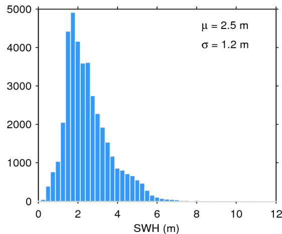
Figure 20. Histogram of science-valid SWH over oceans and lakes for 25/09/2015. The mean ( \mu ) and standard deviation ( \sigma ) are also shown. Note that values larger than 12 m are excluded from the histogram for the sake of readability but not from the computation of \mu and \sigma .
