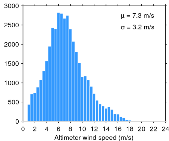
Figure 35. Histogram of science-valid wind over oceans and lakes for 25/09/2015. The mean ( \mu ) and standard deviation ( \sigma ) are also shown. Note that values larger than 24 m/s are excluded from the histogram for the sake of readability but not from the computation of \mu and \sigma .
