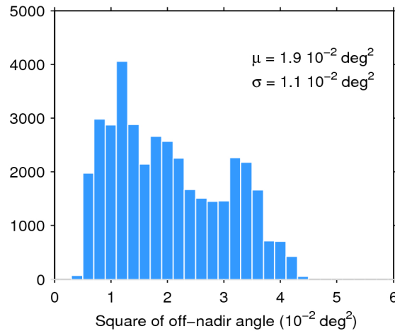
Figure 39. Histogram of flag-valid mispointing over oceans and lakes for 25/09/2015. The mean ( \mu ) and standard deviation ( \sigma ) are also shown. Note that values larger than 6 \cdot 10^{-2} \text{ deg}^2 are excluded from the histogram for the sake of readability but not from the computation of \mu and \sigma .
