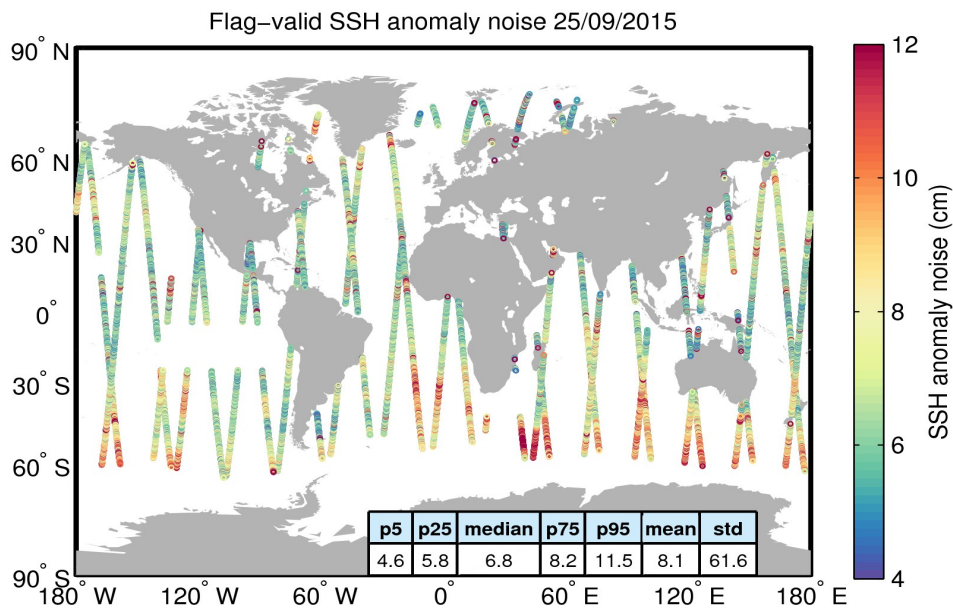
Figure 8. Geographical distribution of flag-valid 20-Hz SSH anomaly measurement noise over oceans and lakes for 25/09/2015. The statistical values shown in the table refer to the SSH anomaly noise and are calculated over all measurements shown in the figure.
