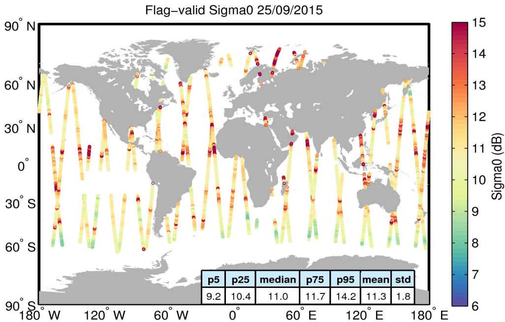
Figure 23. Geographical distribution of flag-valid sigma0 data over oceans and lakes for 25/09/2015. The statistical values shown in the table refer to the sigma0 in dB and are calculated over all measurements shown in the figure.
