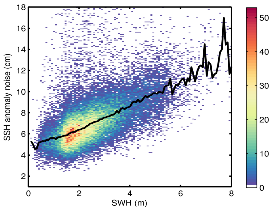
Figure 9. 2D histogram showing flag-valid SSH anomaly noise as a function of SWH for 25/09/2015. The black line denotes the median SSH anomaly noise as a function of SWH.
