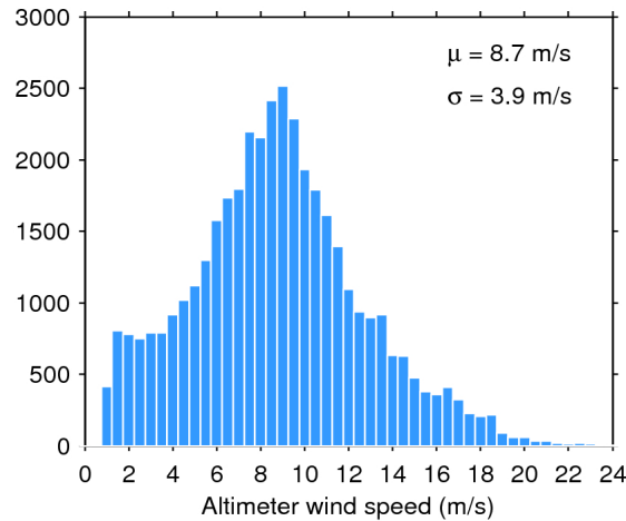
Figure 33. Histogram of flag-valid wind over oceans and lakes for 23/09/2015. The mean ( \mu ) and standard deviation ( \sigma ) are also shown. Note that values larger than 24 m/s are excluded from the histogram for the sake of readability but not from the computation of \mu and \sigma .
