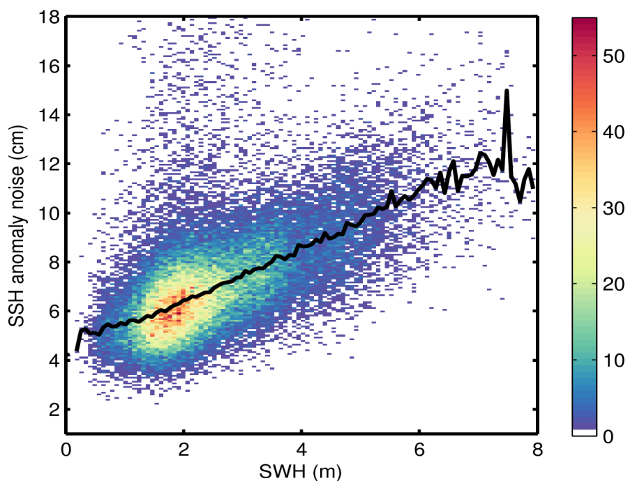
Figure 9. 2D histogram showing flag-valid SSH anomaly noise as a function of SWH for 23/09/2015. The black line denotes the median SSH anomaly noise as a function of SWH.
