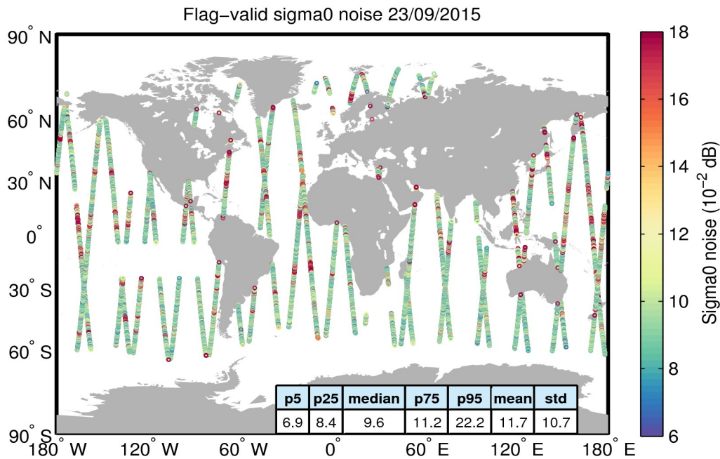
Figure 26. Geographical distribution of flag-valid 20-Hz sigma0 measurement noise over oceans and lakes for 23/09/2015. The statistical values shown in the table refer to the sigma0 noise and are calculated over all measurements shown in the figure.
