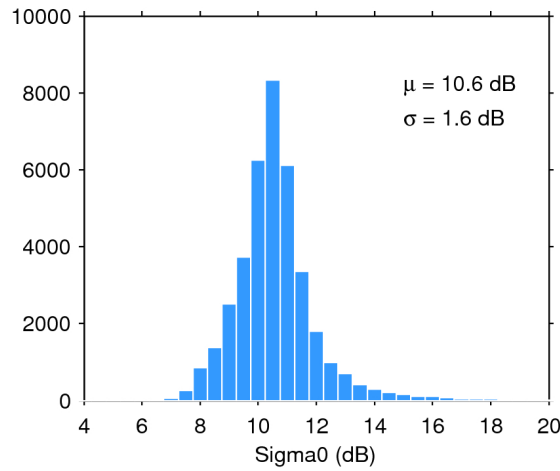
Figure 28. Histogram of science-valid sigma0 over oceans and lakes for 23/09/2015. The mean ( \mu ) and standard deviation ( \sigma ) are also shown. Note that values outside [4 20] dB are excluded from the histogram for the sake of readability but not from the computation of \mu and \sigma .
