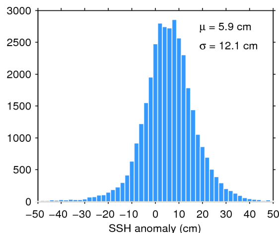
Figure 11. Histogram of science-valid SSH anomaly over oceans and lakes for 23/09/2015. The mean ( \mu ) and standard deviation ( \sigma ) are also shown. Note that values outside [-50 50] cm are excluded from the histogram for the sake of readability but not from the computation of \mu and \sigma .
