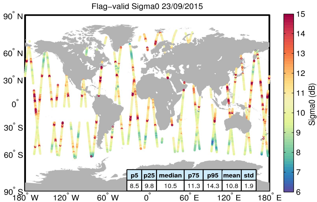
Figure 23. Geographical distribution of flag-valid sigma0 data over oceans and lakes for 23/09/2015. The statistical values shown in the table refer to the sigma0 in dB and are calculated over all measurements shown in the figure.
