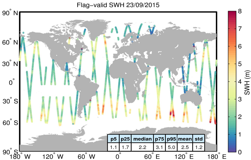
Figure 15. Geographical distribution of flag-valid SWH data over oceans and lakes for 23/09/2015. The statistical values shown in the table refer to the SWH in m and are calculated over all measurements shown in the figure.
