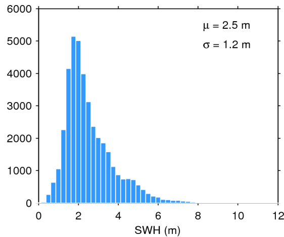
Figure 17. Histogram of flag-valid SWH over oceans and lakes for 23/09/2015. The mean ( \mu ) and standard deviation ( \sigma ) are also shown. Note that values larger than 12 m are excluded from the histogram for the sake of readability but not from the computation of \mu and \sigma .
