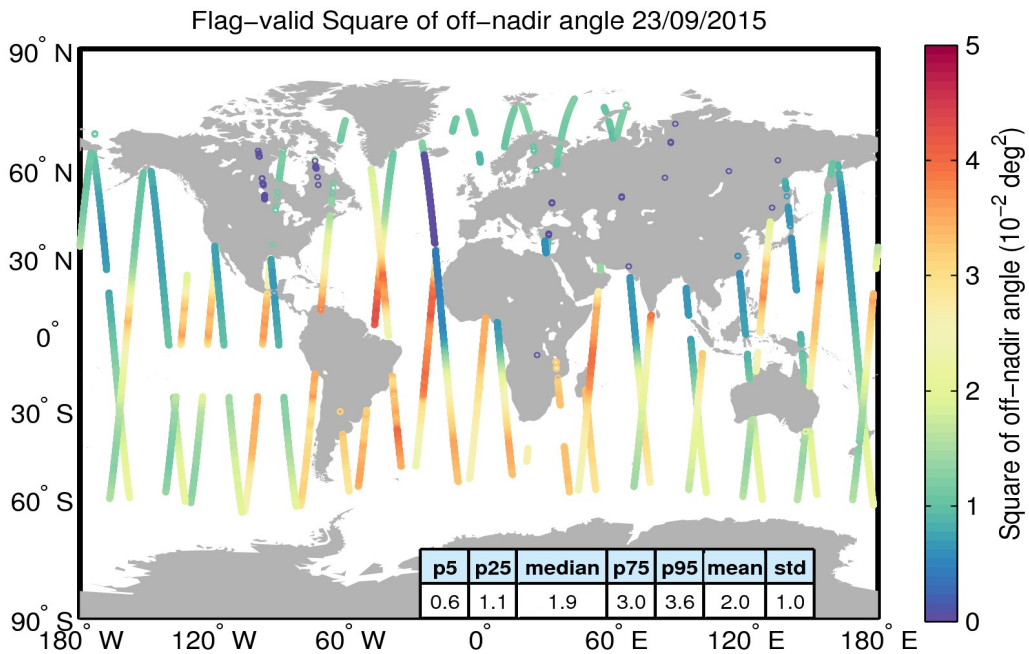
Figure 37. Geographical distribution of flag-valid mispointing data over oceans and lakes for 23/09/2015. The statistical values shown in the table refer to the mispointing in 10^{-2} deg 2 and are calculated over all measurements shown in the figure.
