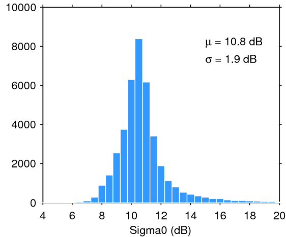
Figure 25. Histogram of flag-valid sigma0 over oceans and lakes for 23/09/2015. The mean ( \mu ) and standard deviation ( \sigma ) are also shown. Note that values outside [4 20] dB are excluded from the histogram for the sake of readability but not from the computation of \mu and \sigma .
