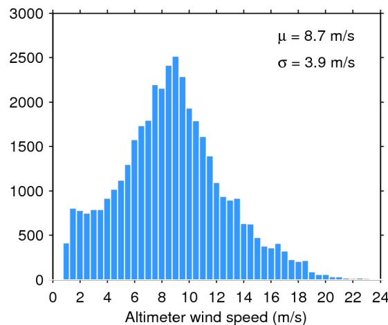
Figure 35. Histogram of science-valid wind over oceans and lakes for 23/09/2015. The mean ( \mu ) and standard deviation ( \sigma ) are also shown. Note that values larger than 24 m/s are excluded from the histogram for the sake of readability but not from the computation of \mu and \sigma .
