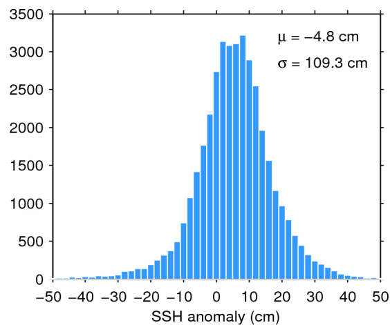
Figure 7. Histogram of flag-valid SSH anomaly over oceans and lakes for 23/09/2015. The mean ( \mu ) and standard deviation ( \sigma ) are also shown. Note that values outside [-50 50] cm are excluded from the histogram for the sake of readability but not from the computation of \mu and \sigma .
