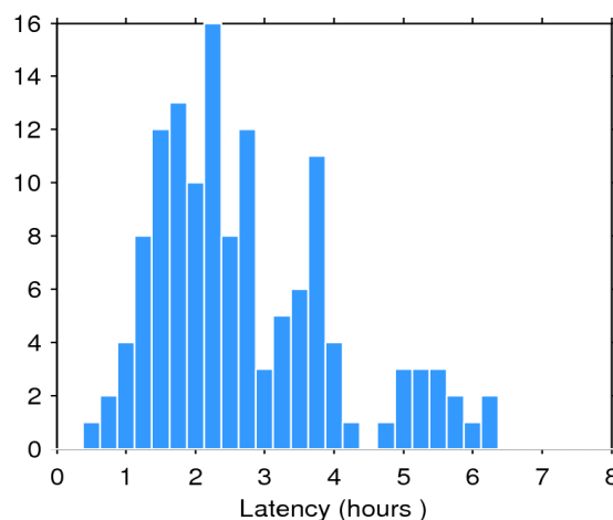
Figure 2. Histogram of the data latency for 23/09/2015. The y-axis denotes the number of files that are made available with a delay of x-hours with respect to the mean time of the records stored in the file.
