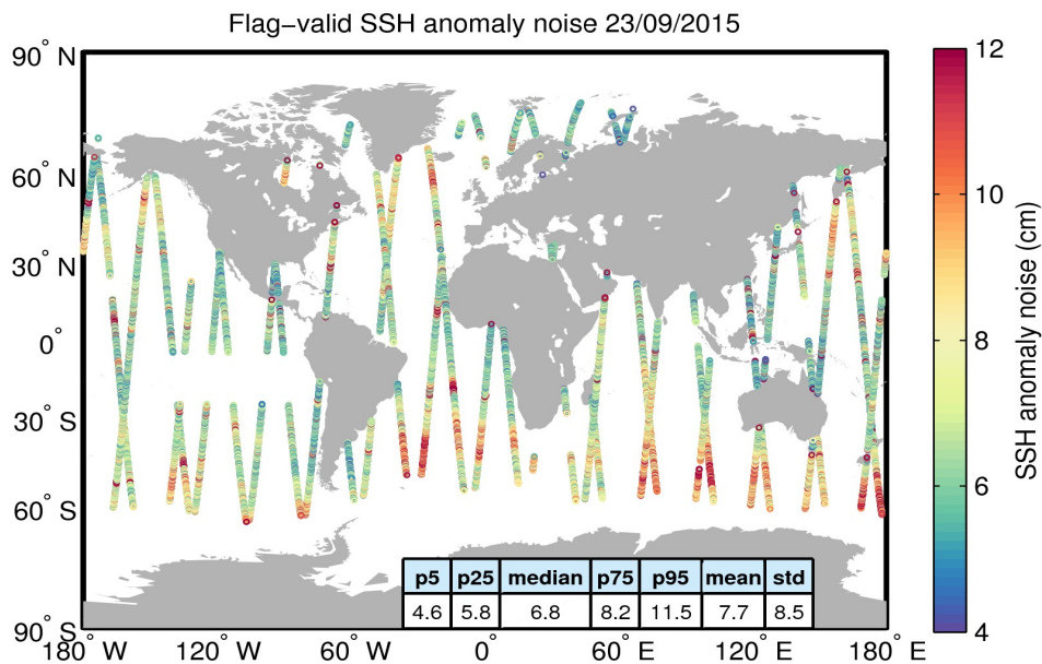
Figure 8. Geographical distribution of flag-valid 20-Hz SSH anomaly measurement noise over oceans and lakes for 23/09/2015. The statistical values shown in the table refer to the SSH anomaly noise and are calculated over all measurements shown in the figure.
