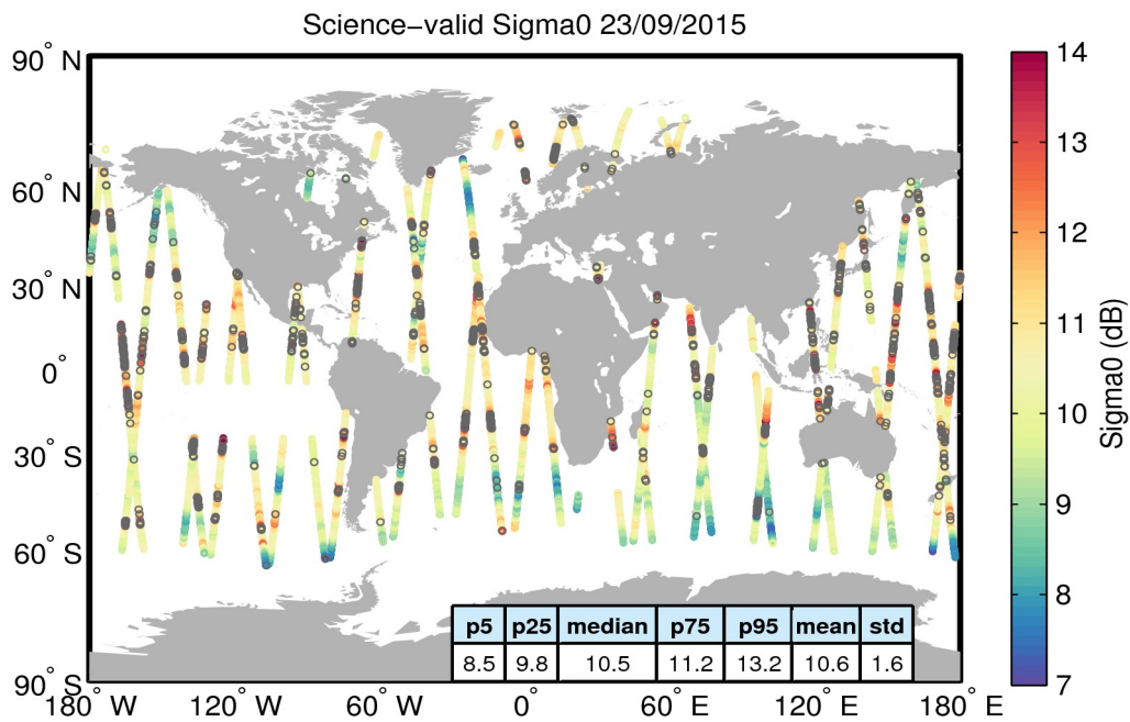
Figure 27. Geographical distribution of science-valid sigma0 data over oceans and lakes for 23/09/2015. The statistical values shown in the table refer to the sigma0 in dB and are calculated over all measurements shown in the figure. Gray circles denote records that have been rejected based on the editing criteria described in Table 4.
