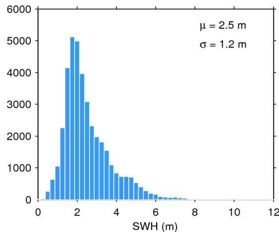
Figure 20. Histogram of science-valid SWH over oceans and lakes for 23/09/2015. The mean ( \mu ) and standard deviation ( \sigma ) are also shown. Note that values larger than 12 m are excluded from the histogram for the sake of readability but not from the computation of \mu and \sigma .
