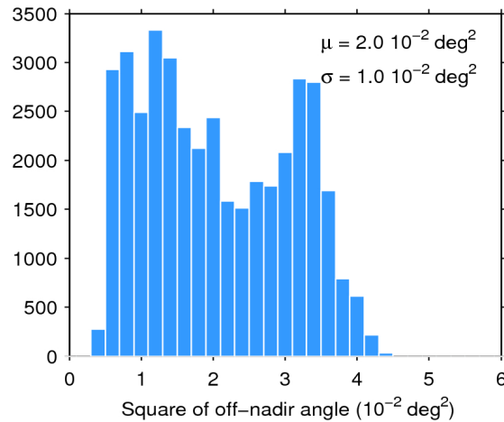
Figure 39. Histogram of flag-valid mispointing over oceans and lakes for 23/09/2015. The mean ( \mu ) and standard deviation ( \sigma ) are also shown. Note that values larger than 6 \cdot 10^{-2} \text{ deg}^2 are excluded from the histogram for the sake of readability but not from the computation of \mu and \sigma .
