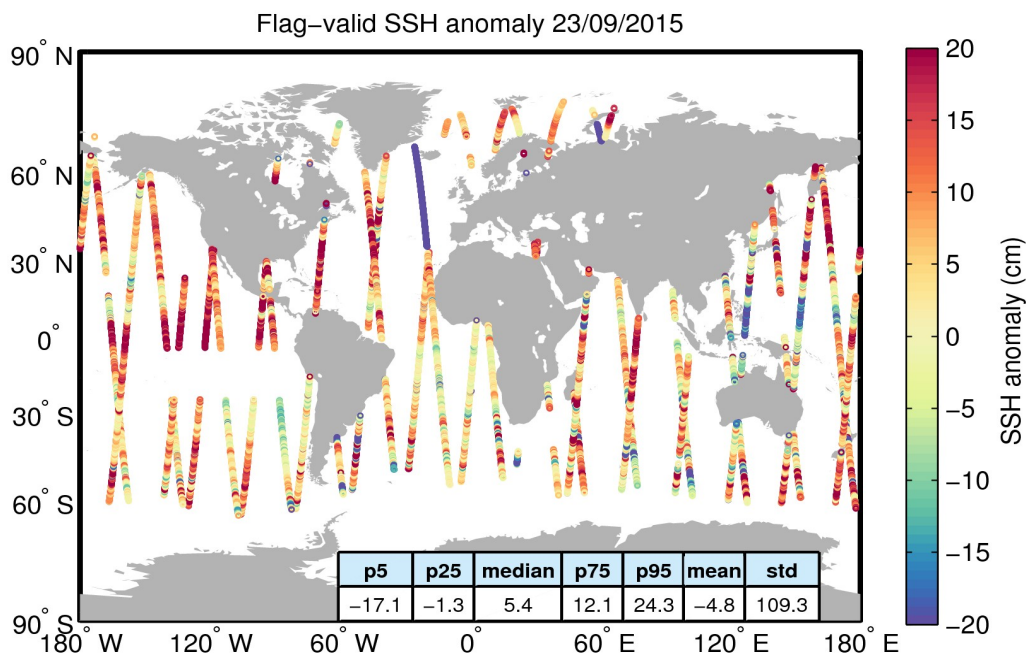
Figure 5. Geographical distribution of flag-valid 1-Hz SSH anomaly data over oceans and lakes for 23/09/2015. The statistical values shown in the table refer to the SSH anomaly in cm and are calculated over all measurements shown in the figure.
