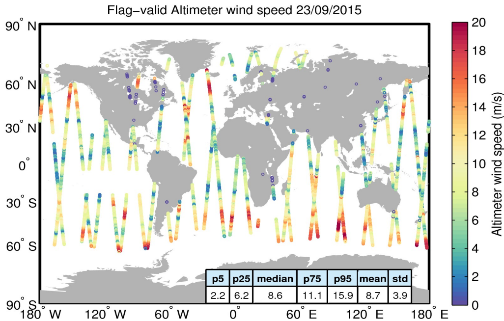
Figure 31. Geographical distribution of flag-valid wind data over oceans and lakes for 23/09/2015. The statistical values shown in the table refer to the wind in m/s and are calculated over all measurements shown in the figure.
