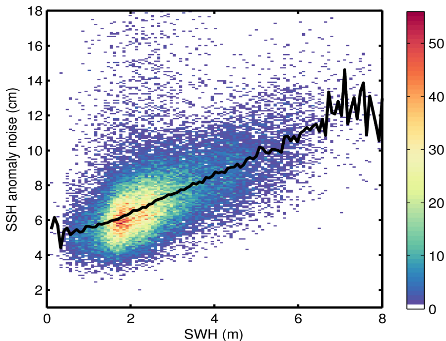
Figure 9. 2D histogram showing flag-valid SSH anomaly noise as a function of SWH for 22/09/2015. The black line denotes the median SSH anomaly noise as a function of SWH.
