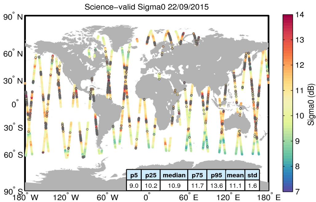
Figure 27. Geographical distribution of science-valid sigma0 data over oceans and lakes for 22/09/2015. The statistical values shown in the table refer to the sigma0 in dB and are calculated over all measurements shown in the figure. Gray circles denote records that have been rejected based on the editing criteria described in Table 4.
