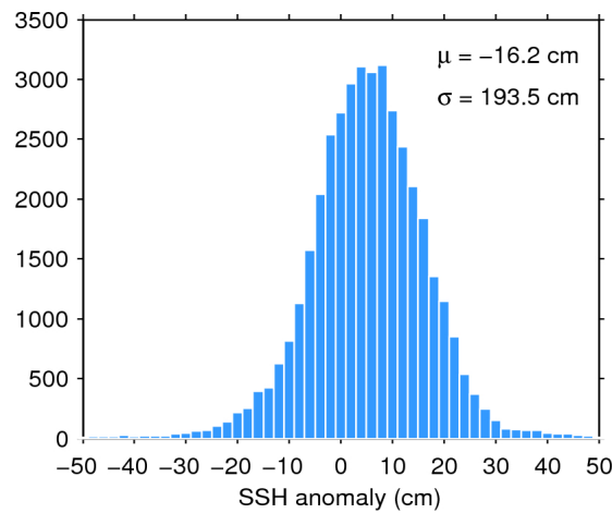
Figure 7. Histogram of flag-valid SSH anomaly over oceans and lakes for 22/09/2015. The mean ( \mu ) and standard deviation ( \sigma ) are also shown. Note that values outside [-50 50] cm are excluded from the histogram for the sake of readability but not from the computation of \mu and \sigma .
