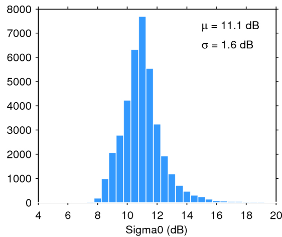
Figure 28. Histogram of science-valid sigma0 over oceans and lakes for 22/09/2015. The mean ( \mu ) and standard deviation ( \sigma ) are also shown. Note that values outside [4 20] dB are excluded from the histogram for the sake of readability but not from the computation of \mu and \sigma .
