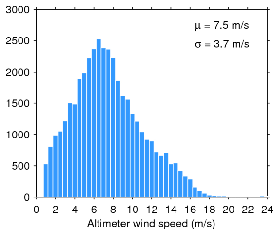
Figure 35. Histogram of science-valid wind over oceans and lakes for 22/09/2015. The mean ( \mu ) and standard deviation ( \sigma ) are also shown. Note that values larger than 24 m/s are excluded from the histogram for the sake of readability but not from the computation of \mu and \sigma .
