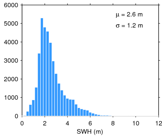
Figure 17. Histogram of flag-valid SWH over oceans and lakes for 22/09/2015. The mean ( \mu ) and standard deviation ( \sigma ) are also shown. Note that values larger than 12 m are excluded from the histogram for the sake of readability but not from the computation of \mu and \sigma .
