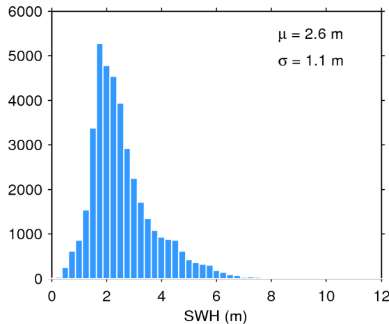
Figure 20. Histogram of science-valid SWH over oceans and lakes for 22/09/2015. The mean ( \mu ) and standard deviation ( \sigma ) are also shown. Note that values larger than 12 m are excluded from the histogram for the sake of readability but not from the computation of \mu and \sigma .
