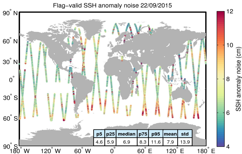
Figure 8. Geographical distribution of flag-valid 20-Hz SSH anomaly measurement noise over oceans and lakes for 22/09/2015. The statistical values shown in the table refer to the SSH anomaly noise and are calculated over all measurements shown in the figure.
