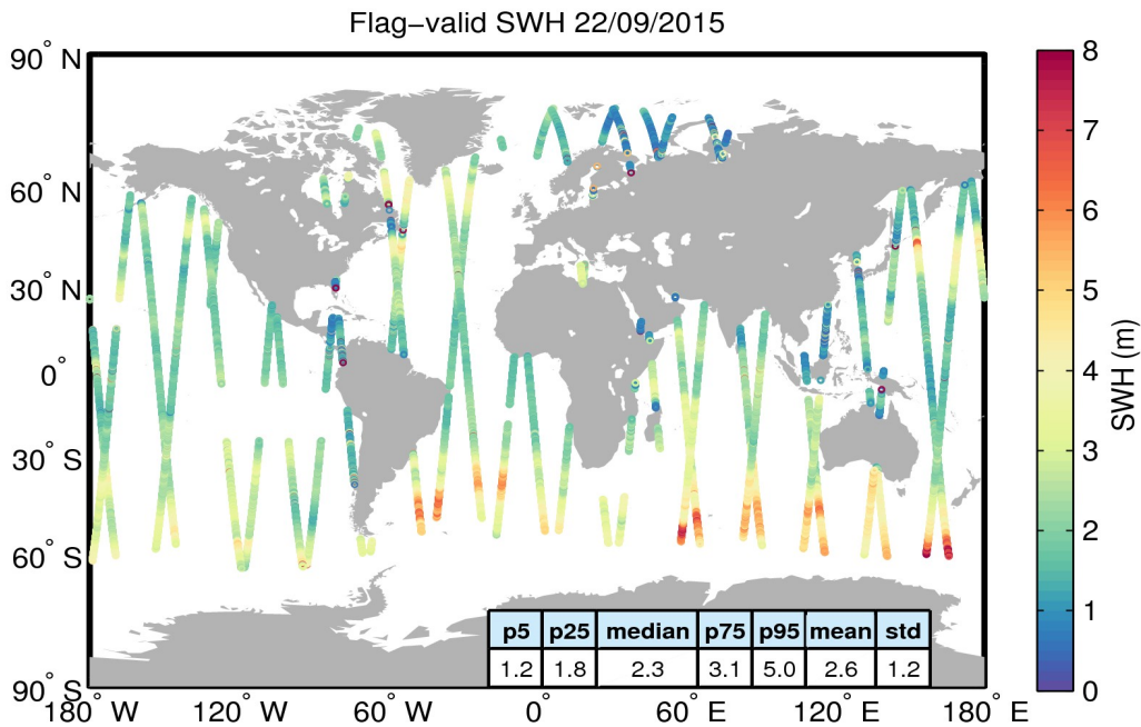
Figure 15. Geographical distribution of flag-valid SWH data over oceans and lakes for 22/09/2015. The statistical values shown in the table refer to the SWH in m and are calculated over all measurements shown in the figure.
