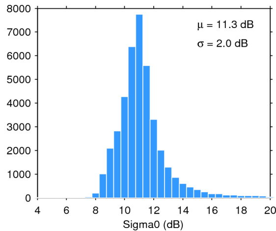
Figure 25. Histogram of flag-valid sigma0 over oceans and lakes for 22/09/2015. The mean ( \mu ) and standard deviation ( \sigma ) are also shown. Note that values outside [4 20] dB are excluded from the histogram for the sake of readability but not from the computation of \mu and \sigma .
