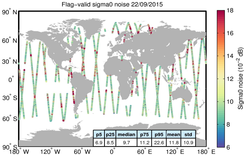
Figure 26. Geographical distribution of flag-valid 20-Hz sigma0 measurement noise over oceans and lakes for 22/09/2015. The statistical values shown in the table refer to the sigma0 noise and are calculated over all measurements shown in the figure.
