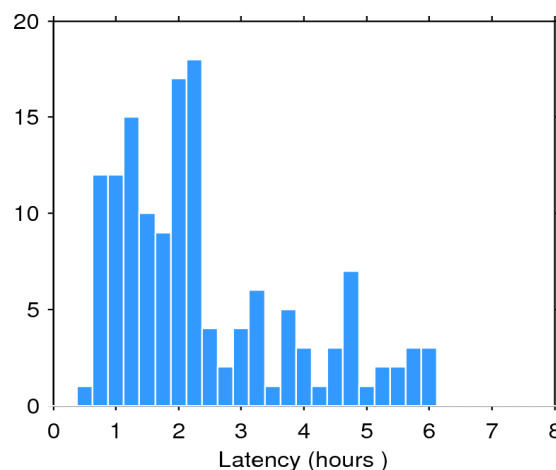
Figure 2. Histogram of the data latency for 22/09/2015. The y-axis denotes the number of files that are made available with a delay of x-hours with respect to the mean time of the records stored in the file.
