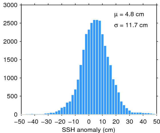
Figure 11. Histogram of science-valid SSH anomaly over oceans and lakes for 22/09/2015. The mean ( \mu ) and standard deviation ( \sigma ) are also shown. Note that values outside [-50 50] cm are excluded from the histogram for the sake of readability but not from the computation of \mu and \sigma .
