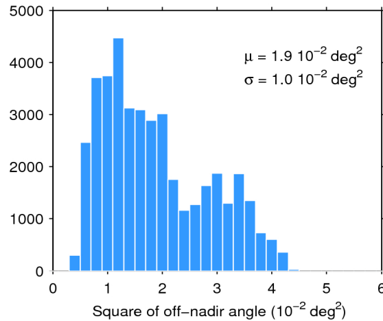
Figure 39. Histogram of flag-valid mispointing over oceans and lakes for 22/09/2015. The mean ( \mu ) and standard deviation ( \sigma ) are also shown. Note that values larger than 6 \cdot 10^{-2} \text{ deg}^2 are excluded from the histogram for the sake of readability but not from the computation of \mu and \sigma .
