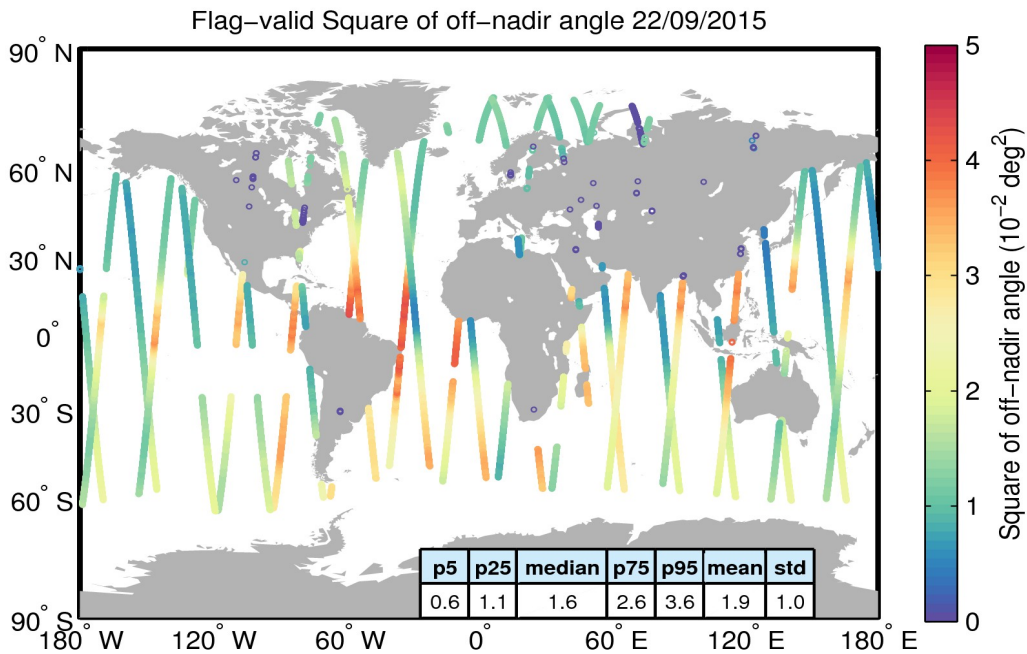
Figure 37. Geographical distribution of flag-valid mispointing data over oceans and lakes for 22/09/2015. The statistical values shown in the table refer to the mispointing in 10^{-2} deg 2 and are calculated over all measurements shown in the figure.
