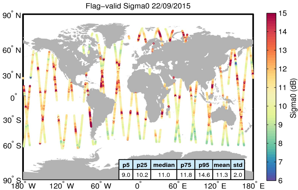
Figure 23. Geographical distribution of flag-valid sigma0 data over oceans and lakes for 22/09/2015. The statistical values shown in the table refer to the sigma0 in dB and are calculated over all measurements shown in the figure.
