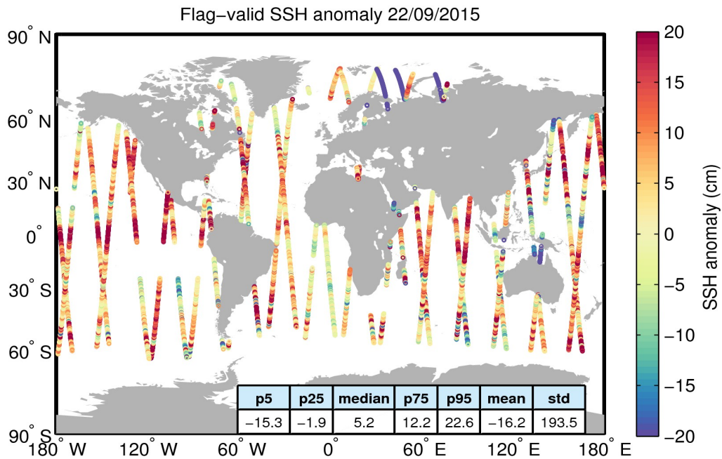
Figure 5. Geographical distribution of flag-valid 1-Hz SSH anomaly data over oceans and lakes for 22/09/2015. The statistical values shown in the table refer to the SSH anomaly in cm and are calculated over all measurements shown in the figure.
