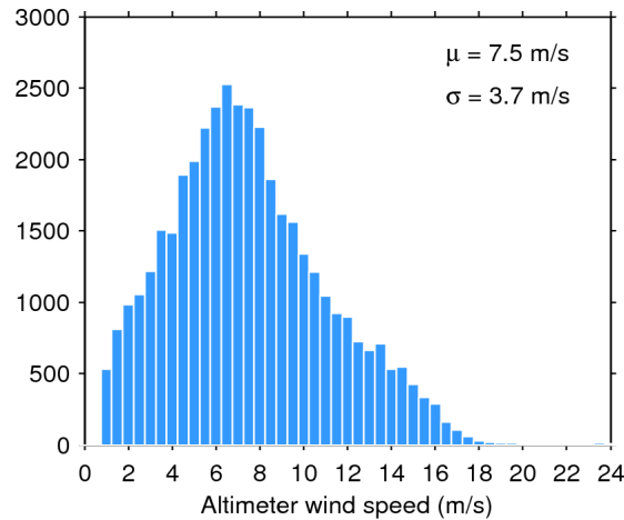
Figure 33. Histogram of flag-valid wind over oceans and lakes for 22/09/2015. The mean ( \mu ) and standard deviation ( \sigma ) are also shown. Note that values larger than 24 m/s are excluded from the histogram for the sake of readability but not from the computation of \mu and \sigma .
