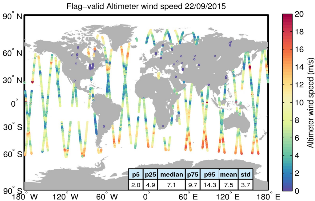
Figure 31. Geographical distribution of flag-valid wind data over oceans and lakes for 22/09/2015. The statistical values shown in the table refer to the wind in m/s and are calculated over all measurements shown in the figure.
