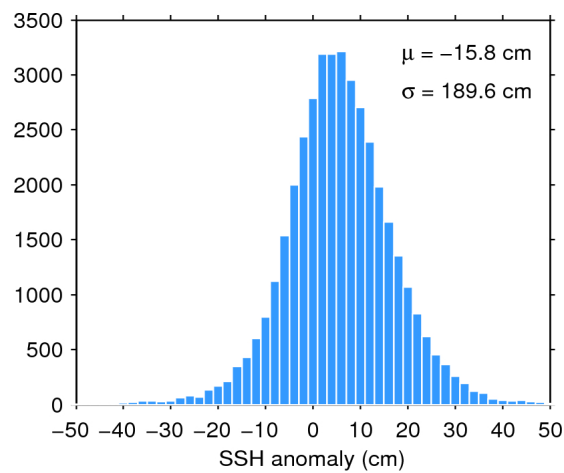
Figure 7. Histogram of flag-valid SSH anomaly over oceans and lakes for 20/09/2015. The mean ( \mu ) and standard deviation ( \sigma ) are also shown. Note that values outside [-50 50] cm are excluded from the histogram for the sake of readability but not from the computation of \mu and \sigma .
