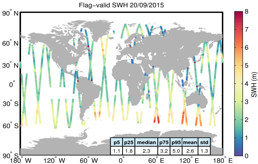
Figure 15. Geographical distribution of flag-valid SWH data over oceans and lakes for 20/09/2015. The statistical values shown in the table refer to the SWH in m and are calculated over all measurements shown in the figure.
