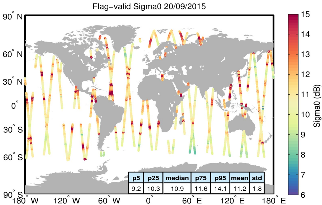
Figure 23. Geographical distribution of flag-valid sigma0 data over oceans and lakes for 20/09/2015. The statistical values shown in the table refer to the sigma0 in dB and are calculated over all measurements shown in the figure.
