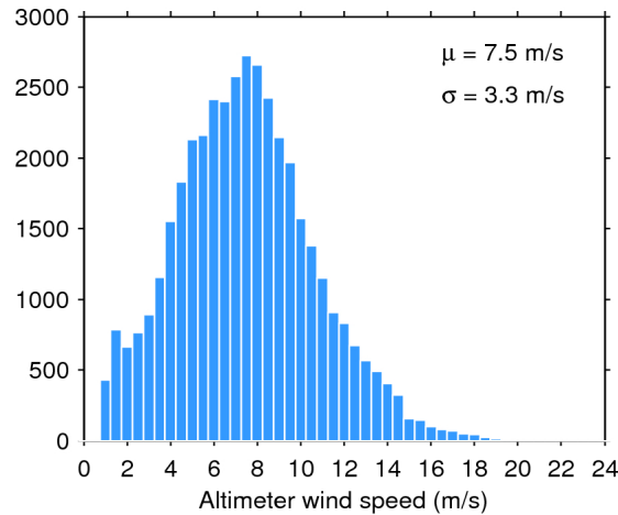
Figure 33. Histogram of flag-valid wind over oceans and lakes for 20/09/2015. The mean ( \mu ) and standard deviation ( \sigma ) are also shown. Note that values larger than 24 m/s are excluded from the histogram for the sake of readability but not from the computation of \mu and \sigma .
