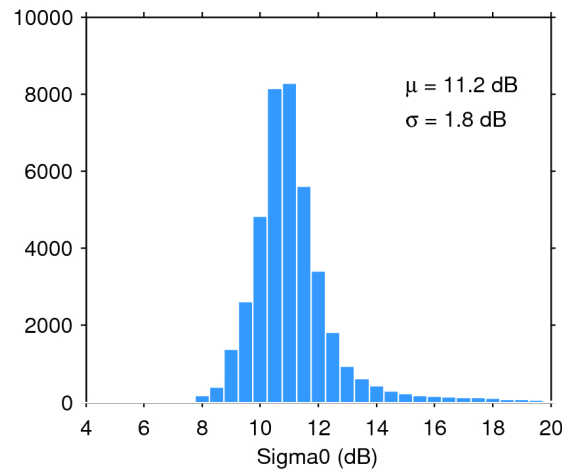
Figure 25. Histogram of flag-valid sigma0 over oceans and lakes for 20/09/2015. The mean ( \mu ) and standard deviation ( \sigma ) are also shown. Note that values outside [4 20] dB are excluded from the histogram for the sake of readability but not from the computation of \mu and \sigma .
