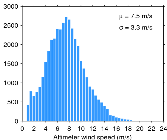
Figure 35. Histogram of science-valid wind over oceans and lakes for 20/09/2015. The mean ( \mu ) and standard deviation ( \sigma ) are also shown. Note that values larger than 24 m/s are excluded from the histogram for the sake of readability but not from the computation of \mu and \sigma .
