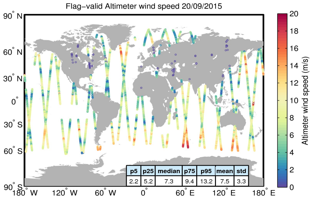
Figure 31. Geographical distribution of flag-valid wind data over oceans and lakes for 20/09/2015. The statistical values shown in the table refer to the wind in m/s and are calculated over all measurements shown in the figure.
