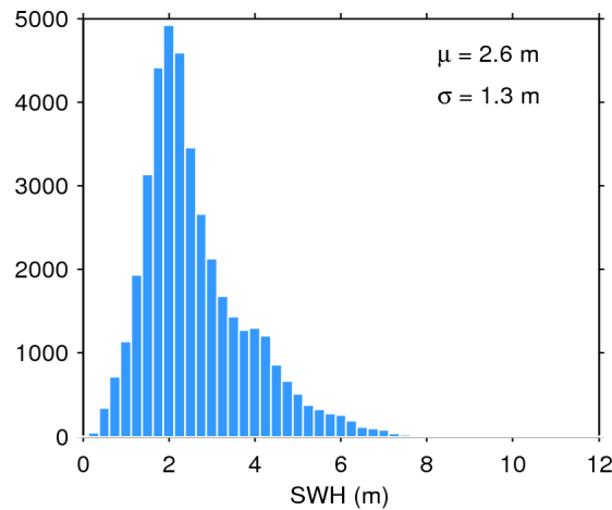
Figure 17. Histogram of flag-valid SWH over oceans and lakes for 20/09/2015. The mean ( \mu ) and standard deviation ( \sigma ) are also shown. Note that values larger than 12 m are excluded from the histogram for the sake of readability but not from the computation of \mu and \sigma .
