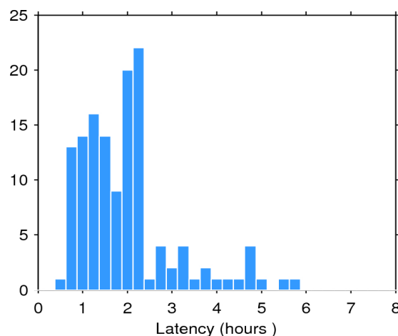
Figure 2. Histogram of the data latency for 20/09/2015. The y-axis denotes the number of files that are made available with a delay of x-hours with respect to the mean time of the records stored in the file.
