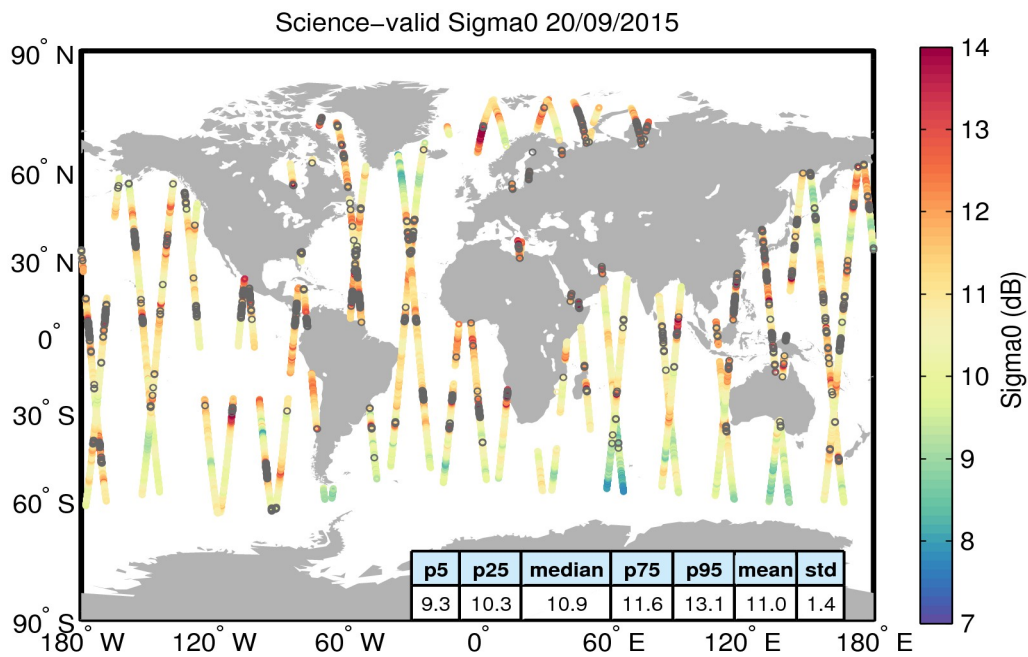
Figure 27. Geographical distribution of science-valid sigma0 data over oceans and lakes for 20/09/2015. The statistical values shown in the table refer to the sigma0 in dB and are calculated over all measurements shown in the figure. Gray circles denote records that have been rejected based on the editing criteria described in Table 4.
