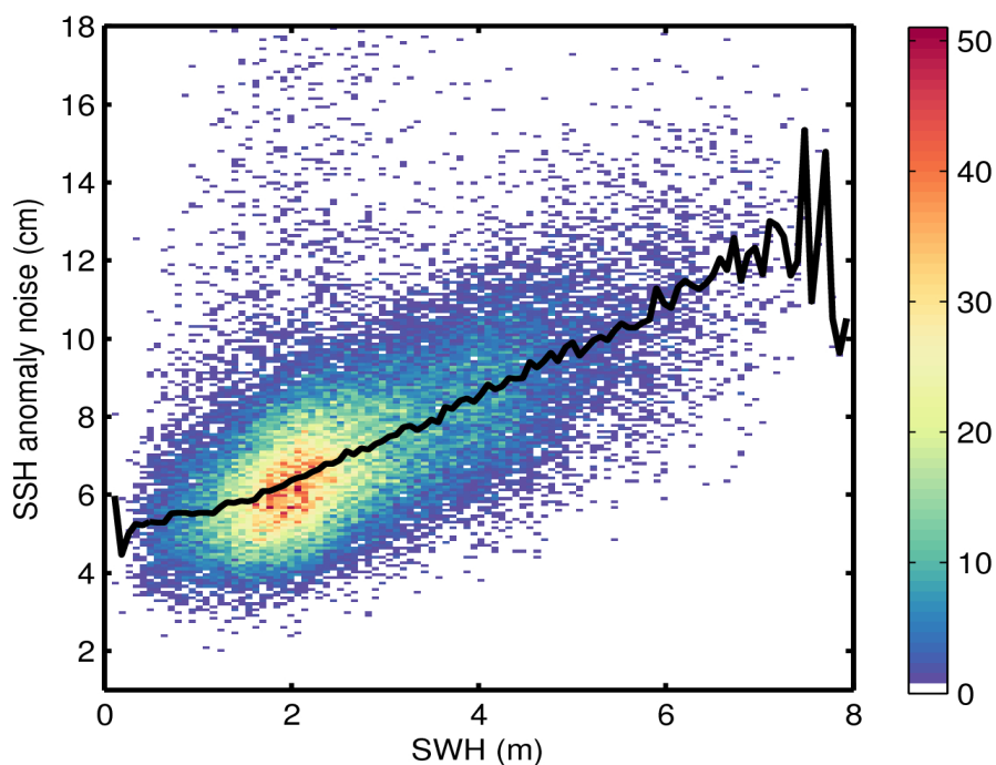
Figure 9. 2D histogram showing flag-valid SSH anomaly noise as a function of SWH for 20/09/2015. The black line denotes the median SSH anomaly noise as a function of SWH.
