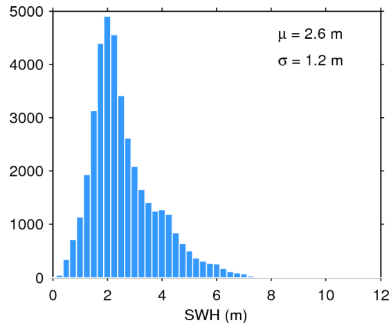
Figure 20. Histogram of science-valid SWH over oceans and lakes for 20/09/2015. The mean ( \mu ) and standard deviation ( \sigma ) are also shown. Note that values larger than 12 m are excluded from the histogram for the sake of readability but not from the computation of \mu and \sigma .
