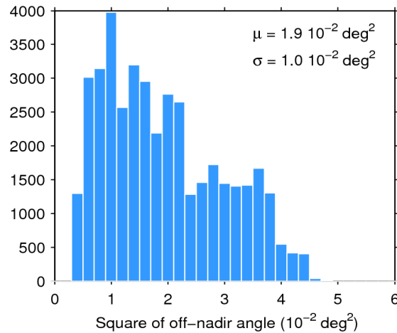
Figure 39. Histogram of flag-valid mispointing over oceans and lakes for 20/09/2015. The mean ( \mu ) and standard deviation ( \sigma ) are also shown. Note that values larger than 6 \cdot 10^{-2} \text{ deg}^2 are excluded from the histogram for the sake of readability but not from the computation of \mu and \sigma .
