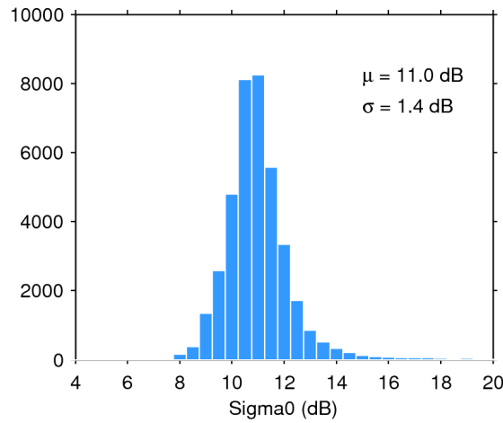
Figure 28. Histogram of science-valid sigma0 over oceans and lakes for 20/09/2015. The mean ( \mu ) and standard deviation ( \sigma ) are also shown. Note that values outside [4 20] dB are excluded from the histogram for the sake of readability but not from the computation of \mu and \sigma .
