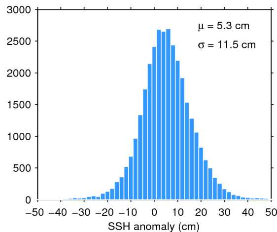
Figure 11. Histogram of science-valid SSH anomaly over oceans and lakes for 20/09/2015. The mean ( \mu ) and standard deviation ( \sigma ) are also shown. Note that values outside [-50 50] cm are excluded from the histogram for the sake of readability but not from the computation of \mu and \sigma .
