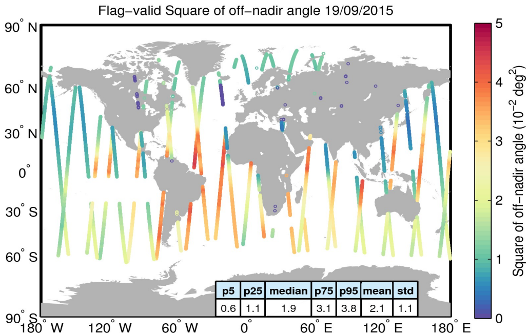
Figure 37. Geographical distribution of flag-valid mispointing data over oceans and lakes for 19/09/2015. The statistical values shown in the table refer to the mispointing in 10^{-2} deg 2 and are calculated over all measurements shown in the figure.
