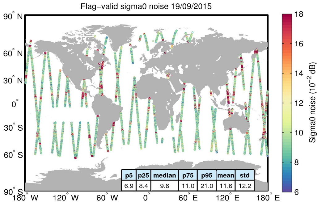
Figure 26. Geographical distribution of flag-valid 20-Hz sigma0 measurement noise over oceans and lakes for 19/09/2015. The statistical values shown in the table refer to the sigma0 noise and are calculated over all measurements shown in the figure.
