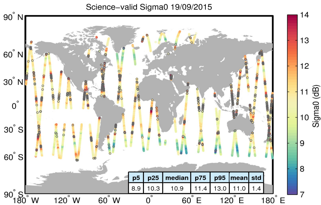
Figure 27. Geographical distribution of science-valid sigma0 data over oceans and lakes for 19/09/2015. The statistical values shown in the table refer to the sigma0 in dB and are calculated over all measurements shown in the figure. Gray circles denote records that have been rejected based on the editing criteria described in Table 4.
