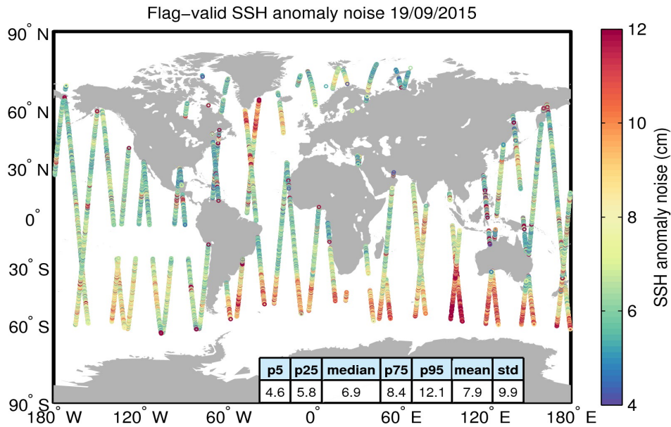
Figure 8. Geographical distribution of flag-valid 20-Hz SSH anomaly measurement noise over oceans and lakes for 19/09/2015. The statistical values shown in the table refer to the SSH anomaly noise and are calculated over all measurements shown in the figure.
