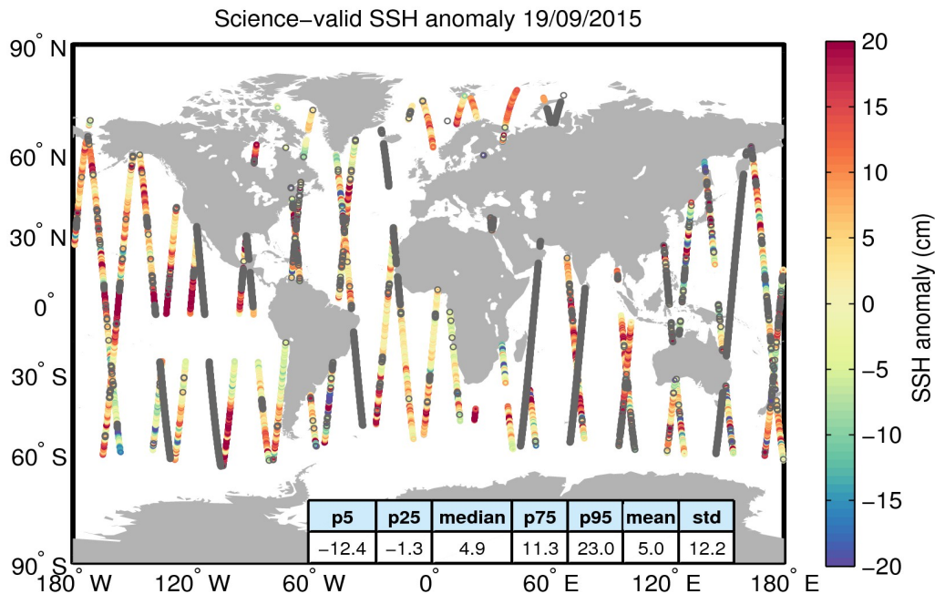
Figure 10. Geographical distribution of science-valid SSH anomaly data over oceans and lakes for 19/09/2015. The statistical values shown in the table refer to the SSH anomaly in cm and are calculated over all measurements shown in the figure. Gray circles denote records that have been rejected based on the editing criteria described in Table 2.
