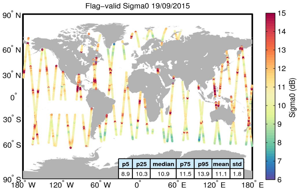
Figure 23. Geographical distribution of flag-valid sigma0 data over oceans and lakes for 19/09/2015. The statistical values shown in the table refer to the sigma0 in dB and are calculated over all measurements shown in the figure.
