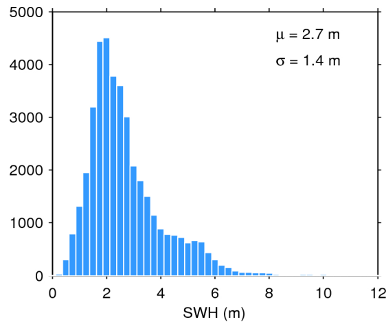
Figure 17. Histogram of flag-valid SWH over oceans and lakes for 19/09/2015. The mean ( \mu ) and standard deviation ( \sigma ) are also shown. Note that values larger than 12 m are excluded from the histogram for the sake of readability but not from the computation of \mu and \sigma .
