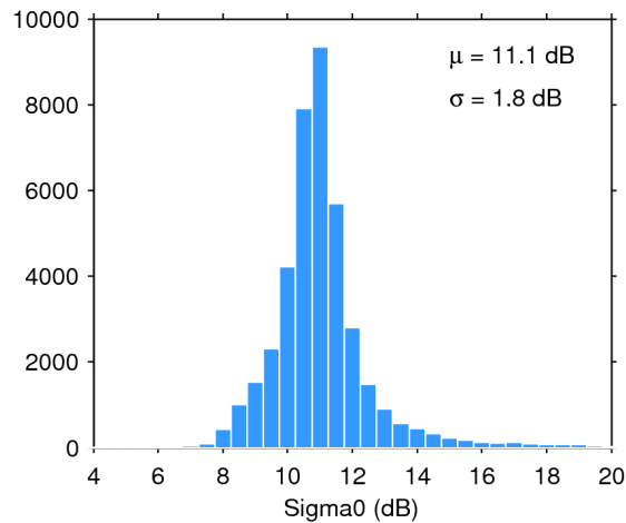
Figure 25. Histogram of flag-valid sigma0 over oceans and lakes for 19/09/2015. The mean ( \mu ) and standard deviation ( \sigma ) are also shown. Note that values outside [4 20] dB are excluded from the histogram for the sake of readability but not from the computation of \mu and \sigma .
