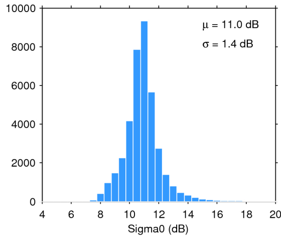
Figure 28. Histogram of science-valid sigma0 over oceans and lakes for 19/09/2015. The mean ( \mu ) and standard deviation ( \sigma ) are also shown. Note that values outside [4 20] dB are excluded from the histogram for the sake of readability but not from the computation of \mu and \sigma .
