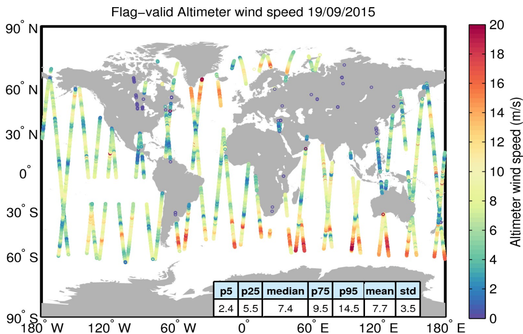
Figure 31. Geographical distribution of flag-valid wind data over oceans and lakes for 19/09/2015. The statistical values shown in the table refer to the wind in m/s and are calculated over all measurements shown in the figure.
