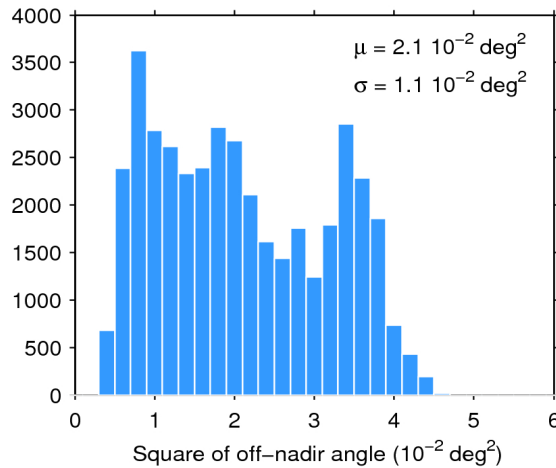
Figure 39. Histogram of flag-valid mispointing over oceans and lakes for 19/09/2015. The mean ( \mu ) and standard deviation ( \sigma ) are also shown. Note that values larger than 6 \cdot 10^{-2} \text{ deg}^2 are excluded from the histogram for the sake of readability but not from the computation of \mu and \sigma .
