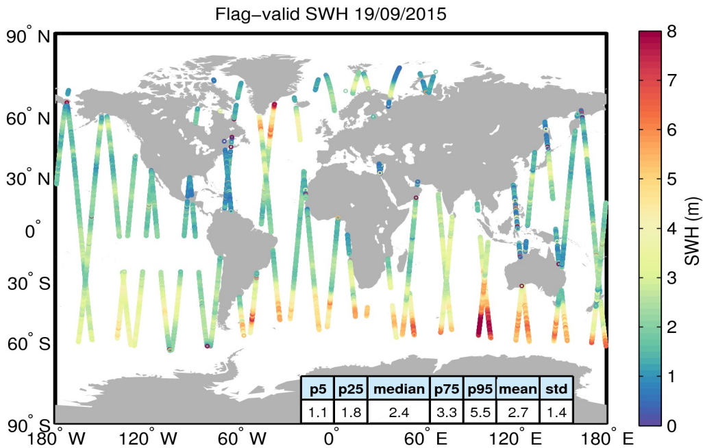
Figure 15. Geographical distribution of flag-valid SWH data over oceans and lakes for 19/09/2015. The statistical values shown in the table refer to the SWH in m and are calculated over all measurements shown in the figure.
