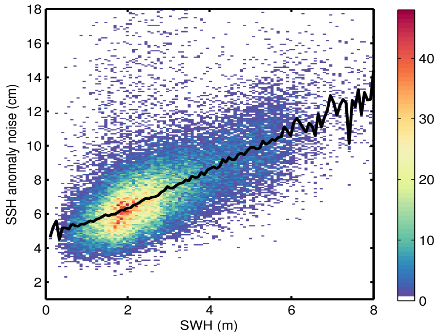
Figure 9. 2D histogram showing flag-valid SSH anomaly noise as a function of SWH for 19/09/2015. The black line denotes the median SSH anomaly noise as a function of SWH.
