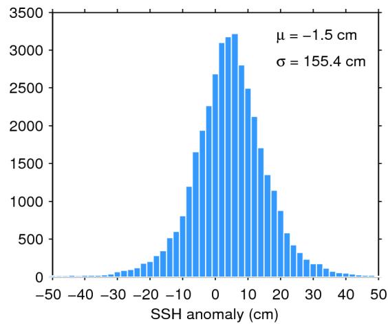
Figure 7. Histogram of flag-valid SSH anomaly over oceans and lakes for 19/09/2015. The mean ( \mu ) and standard deviation ( \sigma ) are also shown. Note that values outside [-50 50] cm are excluded from the histogram for the sake of readability but not from the computation of \mu and \sigma .
