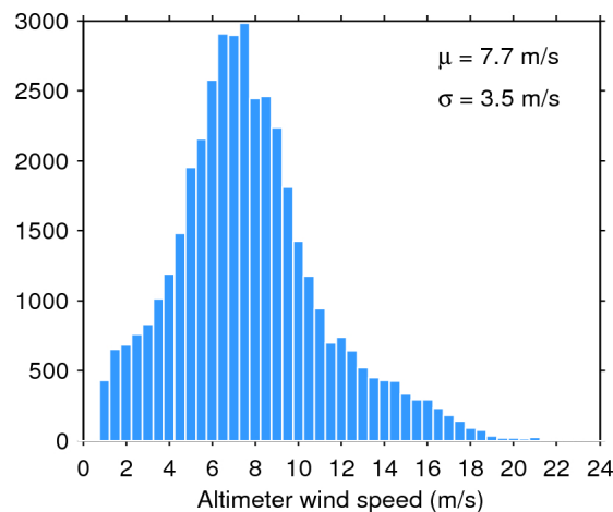
Figure 35. Histogram of science-valid wind over oceans and lakes for 19/09/2015. The mean ( \mu ) and standard deviation ( \sigma ) are also shown. Note that values larger than 24 m/s are excluded from the histogram for the sake of readability but not from the computation of \mu and \sigma .
