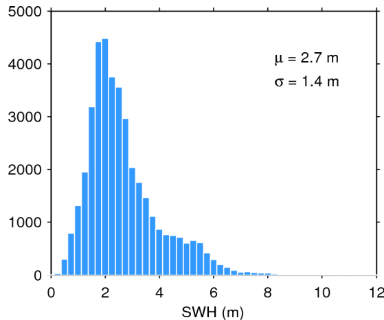
Figure 20. Histogram of science-valid SWH over oceans and lakes for 19/09/2015. The mean ( \mu ) and standard deviation ( \sigma ) are also shown. Note that values larger than 12 m are excluded from the histogram for the sake of readability but not from the computation of \mu and \sigma .
