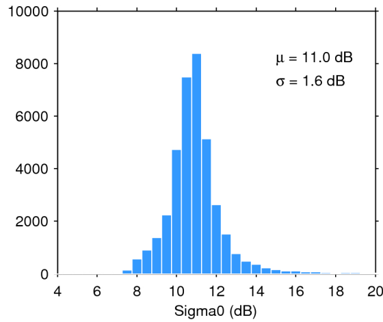
Figure 28. Histogram of science-valid sigma0 over oceans and lakes for 15/09/2015. The mean ( \mu ) and standard deviation ( \sigma ) are also shown. Note that values outside [4 20] dB are excluded from the histogram for the sake of readability but not from the computation of \mu and \sigma .
