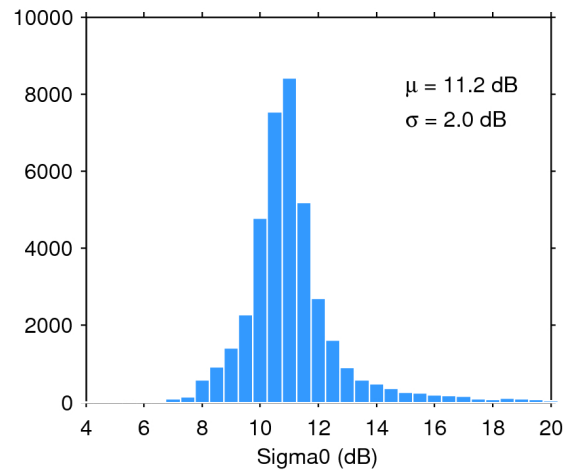
Figure 25. Histogram of flag-valid sigma0 over oceans and lakes for 15/09/2015. The mean ( \mu ) and standard deviation ( \sigma ) are also shown. Note that values outside [4 20] dB are excluded from the histogram for the sake of readability but not from the computation of \mu and \sigma .
