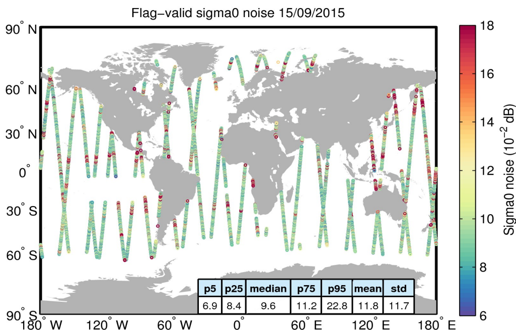
Figure 26. Geographical distribution of flag-valid 20-Hz sigma0 measurement noise over oceans and lakes for 15/09/2015. The statistical values shown in the table refer to the sigma0 noise and are calculated over all measurements shown in the figure.
