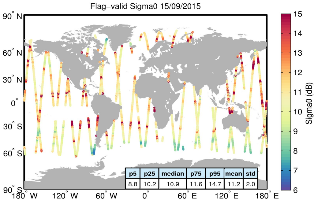
Figure 23. Geographical distribution of flag-valid sigma0 data over oceans and lakes for 15/09/2015. The statistical values shown in the table refer to the sigma0 in dB and are calculated over all measurements shown in the figure.
