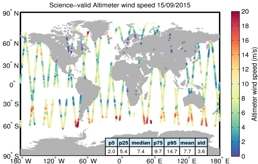
Figure 34. Geographical distribution of science-valid wind data over oceans and lakes for 15/09/2015. The statistical values shown in the table refer to the wind in m/s and are calculated over all measurements shown in the figure. Gray circles denote records that have been rejected based on the editing criteria described in Table 5.
