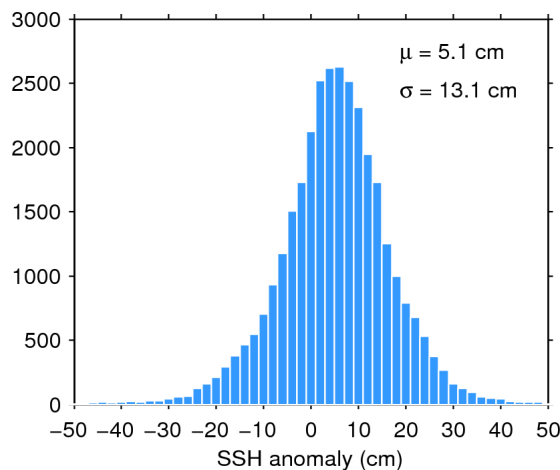
Figure 11. Histogram of science-valid SSH anomaly over oceans and lakes for 15/09/2015. The mean ( \mu ) and standard deviation ( \sigma ) are also shown. Note that values outside [-50 50] cm are excluded from the histogram for the sake of readability but not from the computation of \mu and \sigma .
