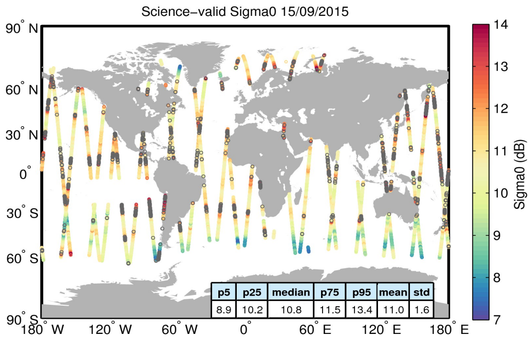
Figure 27. Geographical distribution of science-valid sigma0 data over oceans and lakes for 15/09/2015. The statistical values shown in the table refer to the sigma0 in dB and are calculated over all measurements shown in the figure. Gray circles denote records that have been rejected based on the editing criteria described in Table 4.
