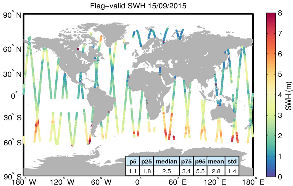
Figure 15. Geographical distribution of flag-valid SWH data over oceans and lakes for 15/09/2015. The statistical values shown in the table refer to the SWH in m and are calculated over all measurements shown in the figure.
