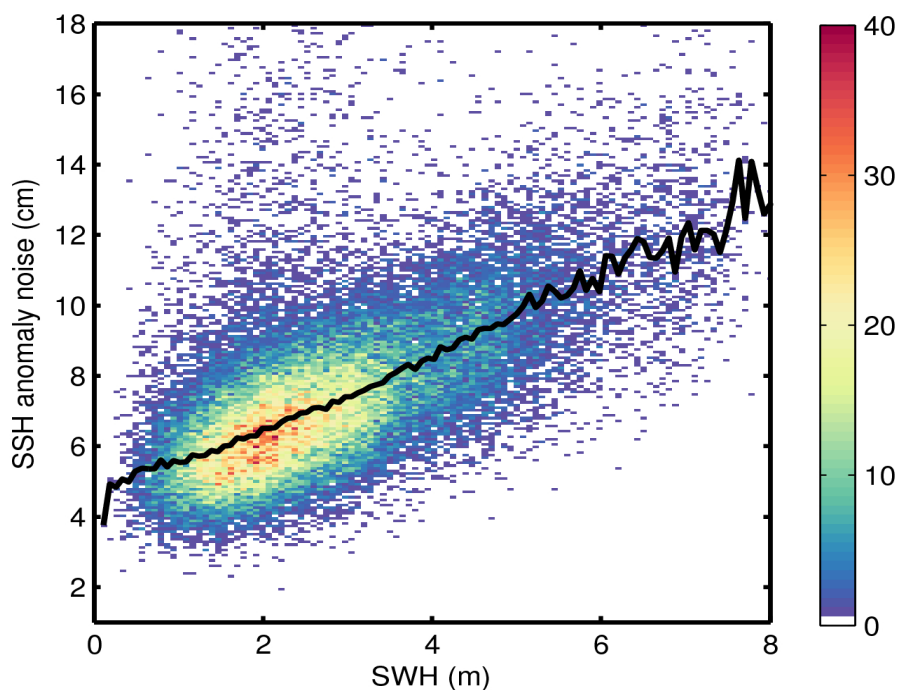
Figure 9. 2D histogram showing flag-valid SSH anomaly noise as a function of SWH for 15/09/2015. The black line denotes the median SSH anomaly noise as a function of SWH.
