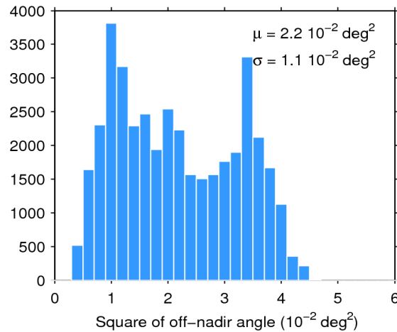
Figure 39. Histogram of flag-valid mispointing over oceans and lakes for 15/09/2015. The mean ( \mu ) and standard deviation ( \sigma ) are also shown. Note that values larger than 6 \cdot 10^{-2} \text{ deg}^2 are excluded from the histogram for the sake of readability but not from the computation of \mu and \sigma .
