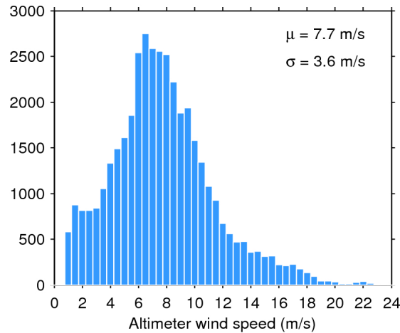
Figure 33. Histogram of flag-valid wind over oceans and lakes for 15/09/2015. The mean ( \mu ) and standard deviation ( \sigma ) are also shown. Note that values larger than 24 m/s are excluded from the histogram for the sake of readability but not from the computation of \mu and \sigma .
