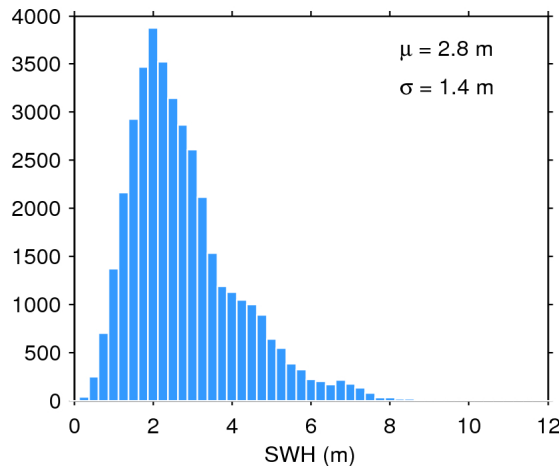
Figure 20. Histogram of science-valid SWH over oceans and lakes for 15/09/2015. The mean ( \mu ) and standard deviation ( \sigma ) are also shown. Note that values larger than 12 m are excluded from the histogram for the sake of readability but not from the computation of \mu and \sigma .
