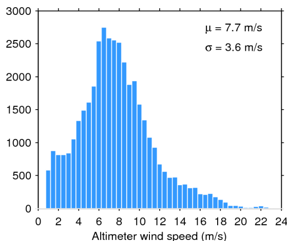
Figure 35. Histogram of science-valid wind over oceans and lakes for 15/09/2015. The mean ( \mu ) and standard deviation ( \sigma ) are also shown. Note that values larger than 24 m/s are excluded from the histogram for the sake of readability but not from the computation of \mu and \sigma .
