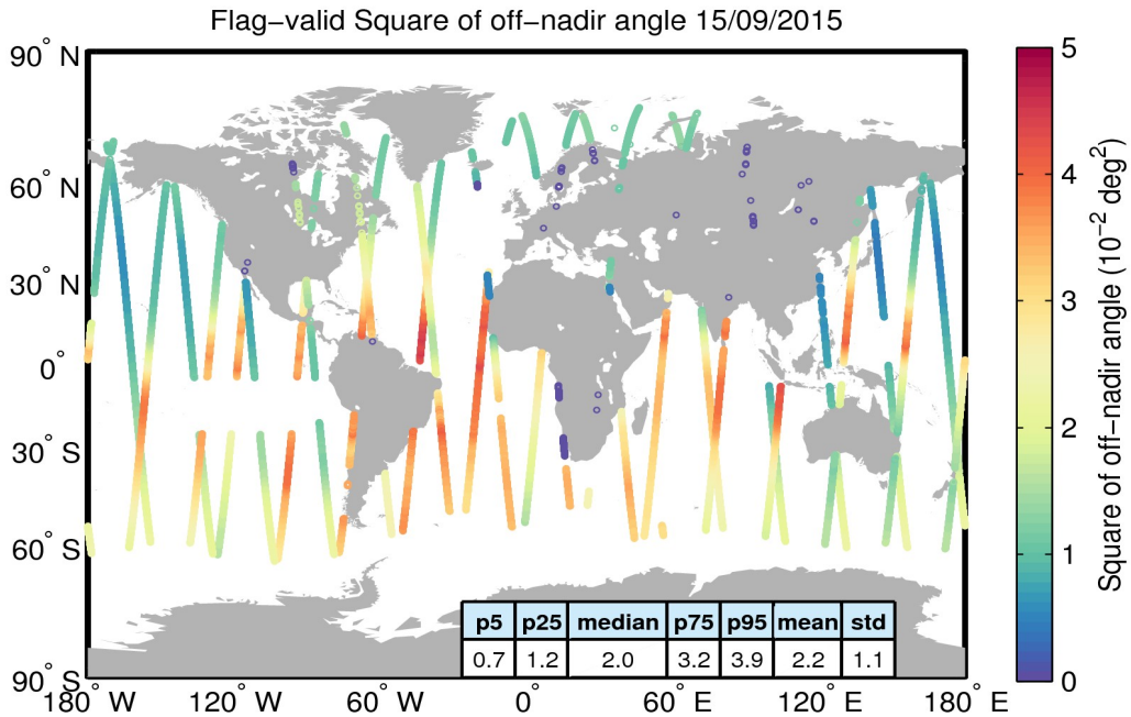
Figure 37. Geographical distribution of flag-valid mispointing data over oceans and lakes for 15/09/2015. The statistical values shown in the table refer to the mispointing in 10^{-2} deg 2 and are calculated over all measurements shown in the figure.
