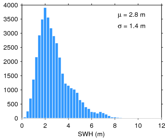
Figure 17. Histogram of flag-valid SWH over oceans and lakes for 15/09/2015. The mean ( \mu ) and standard deviation ( \sigma ) are also shown. Note that values larger than 12 m are excluded from the histogram for the sake of readability but not from the computation of \mu and \sigma .
