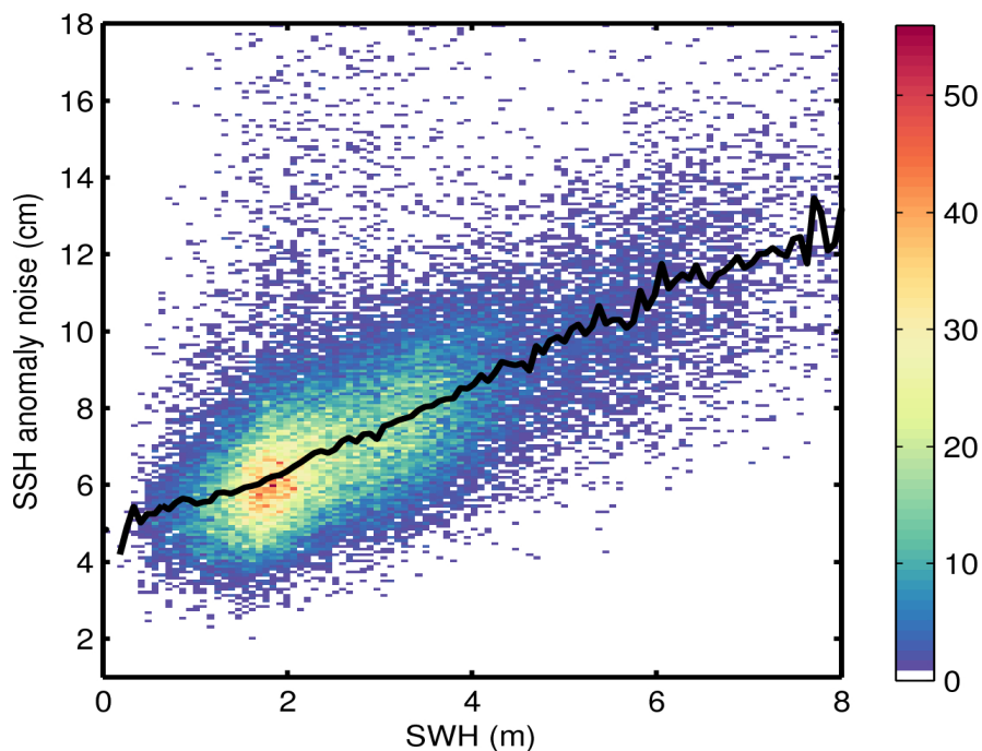
Figure 9. 2D histogram showing flag-valid SSH anomaly noise as a function of SWH for 14/09/2015. The black line denotes the median SSH anomaly noise as a function of SWH.
