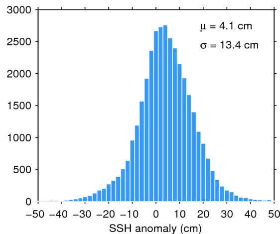
Figure 11. Histogram of science-valid SSH anomaly over oceans and lakes for 14/09/2015. The mean ( \mu ) and standard deviation ( \sigma ) are also shown. Note that values outside [-50 50] cm are excluded from the histogram for the sake of readability but not from the computation of \mu and \sigma .
