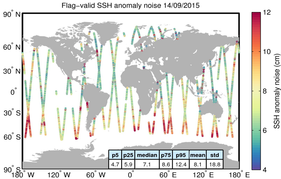
Figure 8. Geographical distribution of flag-valid 20-Hz SSH anomaly measurement noise over oceans and lakes for 14/09/2015. The statistical values shown in the table refer to the SSH anomaly noise and are calculated over all measurements shown in the figure.
