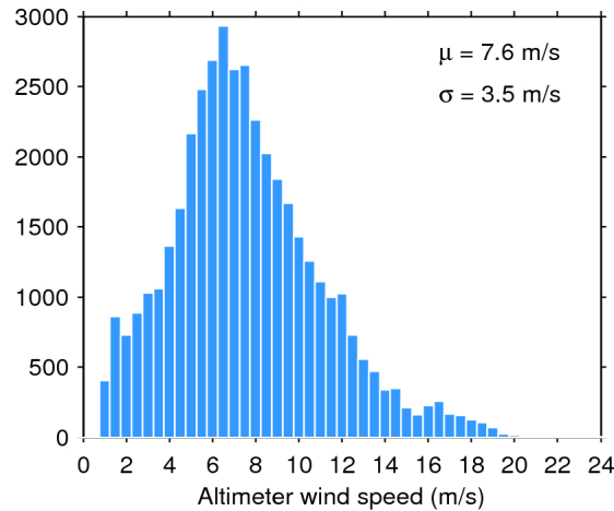
Figure 33. Histogram of flag-valid wind over oceans and lakes for 14/09/2015. The mean ( \mu ) and standard deviation ( \sigma ) are also shown. Note that values larger than 24 m/s are excluded from the histogram for the sake of readability but not from the computation of \mu and \sigma .
