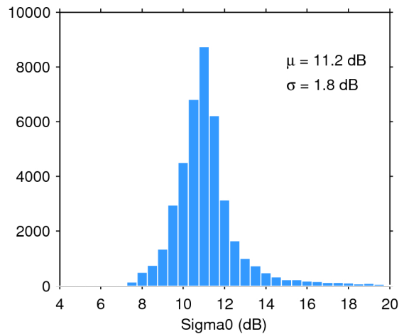
Figure 25. Histogram of flag-valid sigma0 over oceans and lakes for 14/09/2015. The mean ( \mu ) and standard deviation ( \sigma ) are also shown. Note that values outside [4 20] dB are excluded from the histogram for the sake of readability but not from the computation of \mu and \sigma .
