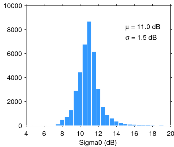
Figure 28. Histogram of science-valid sigma0 over oceans and lakes for 14/09/2015. The mean ( \mu ) and standard deviation ( \sigma ) are also shown. Note that values outside [4 20] dB are excluded from the histogram for the sake of readability but not from the computation of \mu and \sigma .
