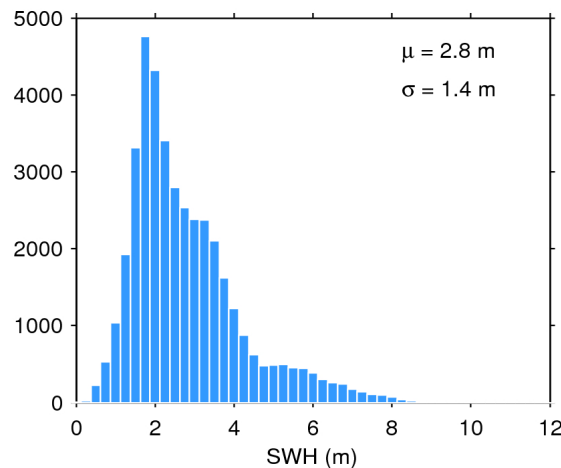
Figure 20. Histogram of science-valid SWH over oceans and lakes for 14/09/2015. The mean ( \mu ) and standard deviation ( \sigma ) are also shown. Note that values larger than 12 m are excluded from the histogram for the sake of readability but not from the computation of \mu and \sigma .
