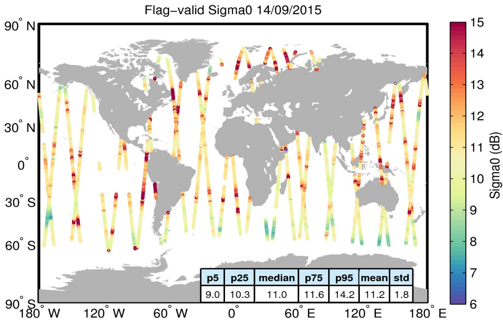
Figure 23. Geographical distribution of flag-valid sigma0 data over oceans and lakes for 14/09/2015. The statistical values shown in the table refer to the sigma0 in dB and are calculated over all measurements shown in the figure.
