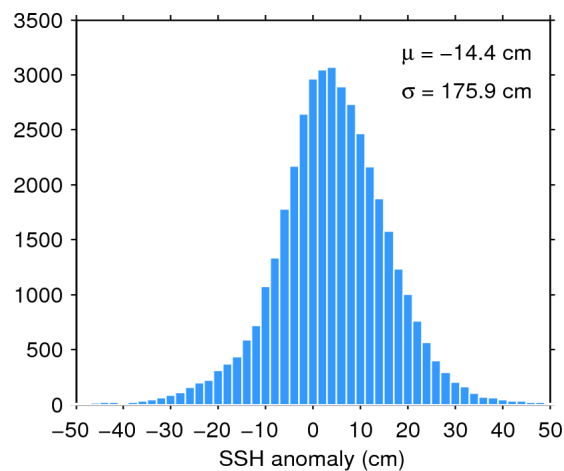
Figure 7. Histogram of flag-valid SSH anomaly over oceans and lakes for 14/09/2015. The mean ( \mu ) and standard deviation ( \sigma ) are also shown. Note that values outside [-50 50] cm are excluded from the histogram for the sake of readability but not from the computation of \mu and \sigma .
