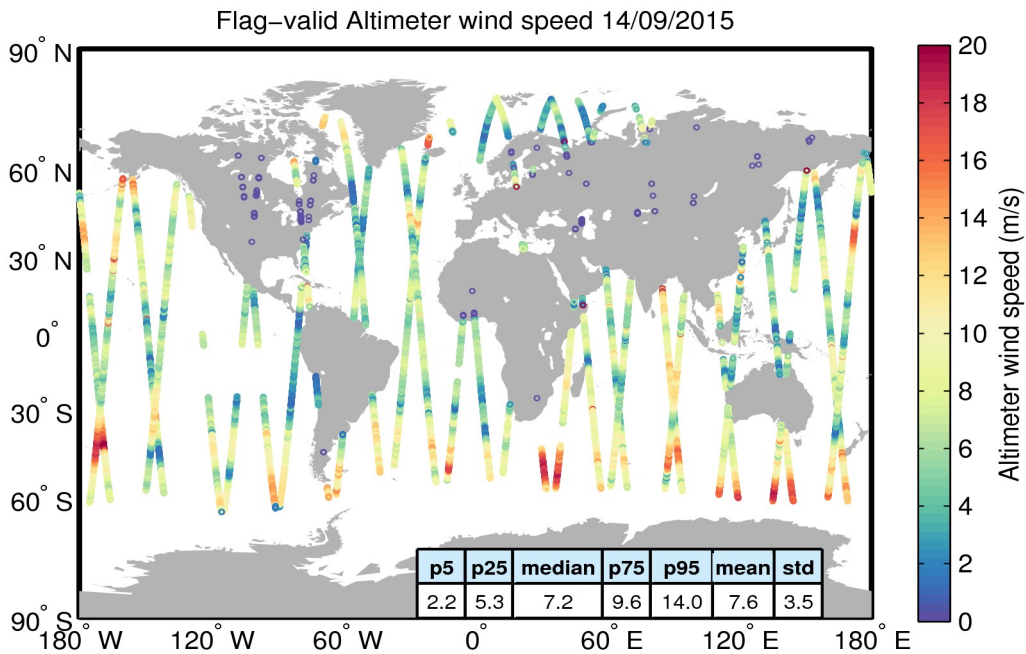
Figure 31. Geographical distribution of flag-valid wind data over oceans and lakes for 14/09/2015. The statistical values shown in the table refer to the wind in m/s and are calculated over all measurements shown in the figure.
