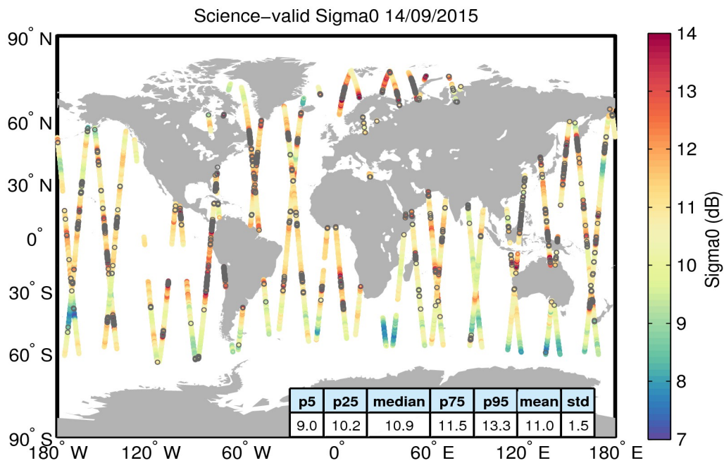
Figure 27. Geographical distribution of science-valid sigma0 data over oceans and lakes for 14/09/2015. The statistical values shown in the table refer to the sigma0 in dB and are calculated over all measurements shown in the figure. Gray circles denote records that have been rejected based on the editing criteria described in Table 4.
