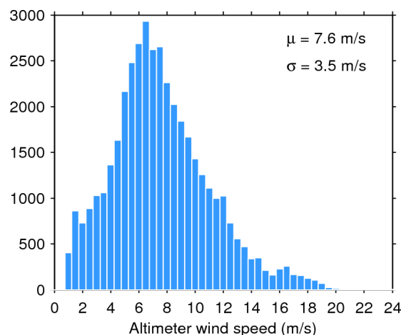
Figure 35. Histogram of science-valid wind over oceans and lakes for 14/09/2015. The mean ( \mu ) and standard deviation ( \sigma ) are also shown. Note that values larger than 24 m/s are excluded from the histogram for the sake of readability but not from the computation of \mu and \sigma .
