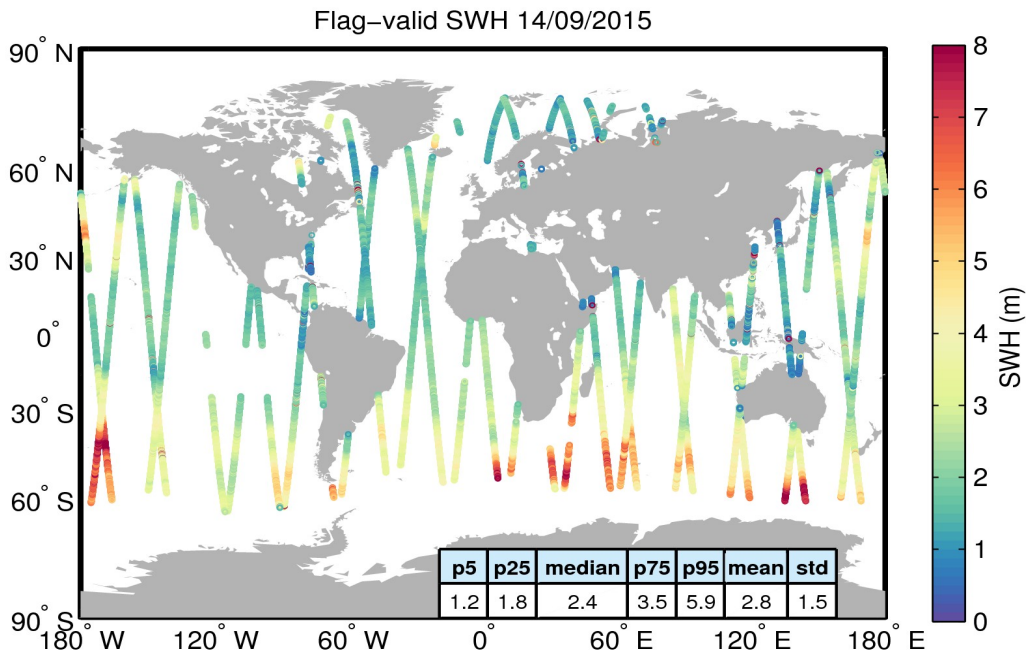
Figure 15. Geographical distribution of flag-valid SWH data over oceans and lakes for 14/09/2015. The statistical values shown in the table refer to the SWH in m and are calculated over all measurements shown in the figure.
