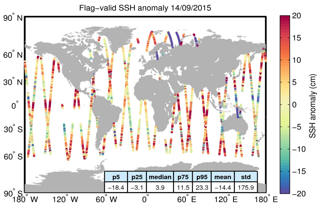
Figure 5. Geographical distribution of flag-valid 1-Hz SSH anomaly data over oceans and lakes for 14/09/2015. The statistical values shown in the table refer to the SSH anomaly in cm and are calculated over all measurements shown in the figure.
