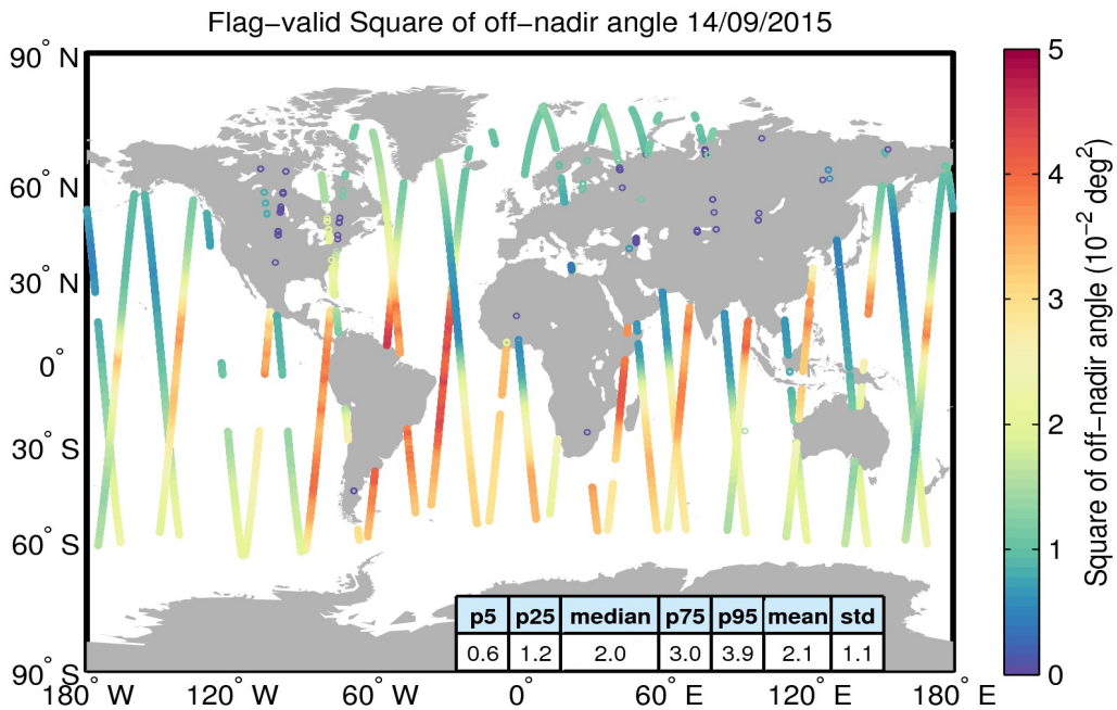
Figure 37. Geographical distribution of flag-valid mispointing data over oceans and lakes for 14/09/2015. The statistical values shown in the table refer to the mispointing in 10^{-2} deg 2 and are calculated over all measurements shown in the figure.
