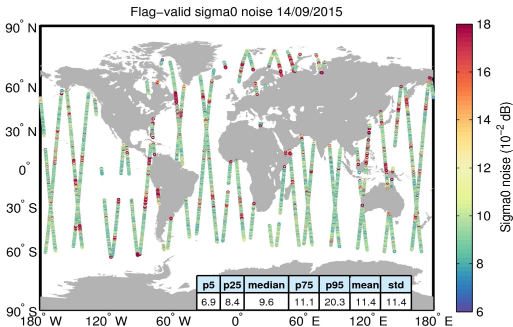
Figure 26. Geographical distribution of flag-valid 20-Hz sigma0 measurement noise over oceans and lakes for 14/09/2015. The statistical values shown in the table refer to the sigma0 noise and are calculated over all measurements shown in the figure.
