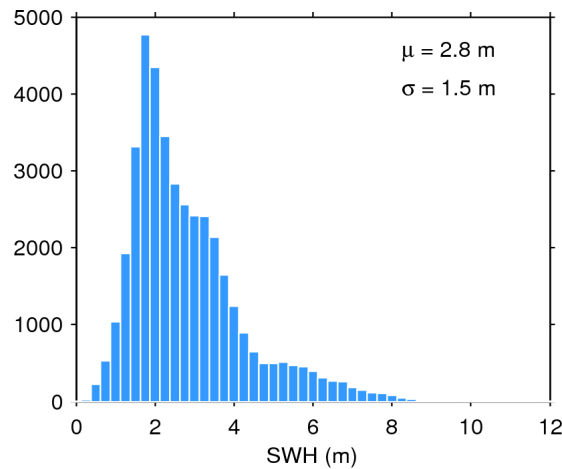
Figure 17. Histogram of flag-valid SWH over oceans and lakes for 14/09/2015. The mean ( \mu ) and standard deviation ( \sigma ) are also shown. Note that values larger than 12 m are excluded from the histogram for the sake of readability but not from the computation of \mu and \sigma .
