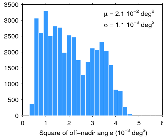
Figure 39. Histogram of flag-valid mispointing over oceans and lakes for 14/09/2015. The mean ( \mu ) and standard deviation ( \sigma ) are also shown. Note that values larger than 6 \cdot 10^{-2} \text{ deg}^2 are excluded from the histogram for the sake of readability but not from the computation of \mu and \sigma .
