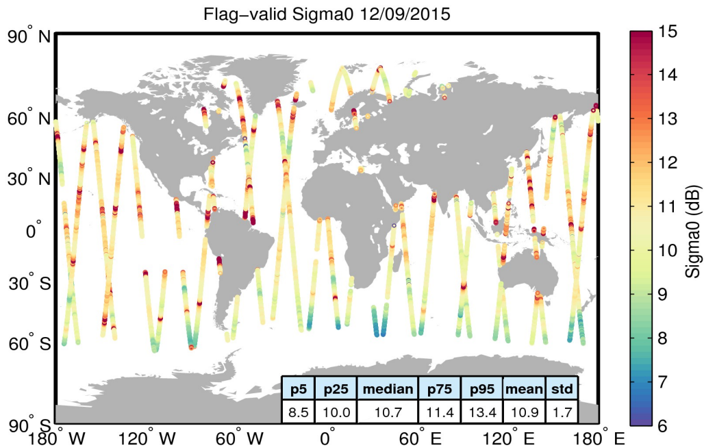
Figure 23. Geographical distribution of flag-valid sigma0 data over oceans and lakes for 12/09/2015. The statistical values shown in the table refer to the sigma0 in dB and are calculated over all measurements shown in the figure.
