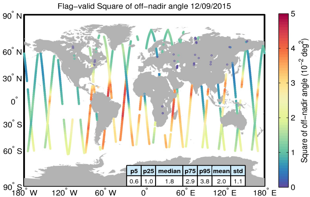
Figure 37. Geographical distribution of flag-valid mispointing data over oceans and lakes for 12/09/2015. The statistical values shown in the table refer to the mispointing in 10^{-2} \text{deg}^2 and are calculated over all measurements shown in the figure.
