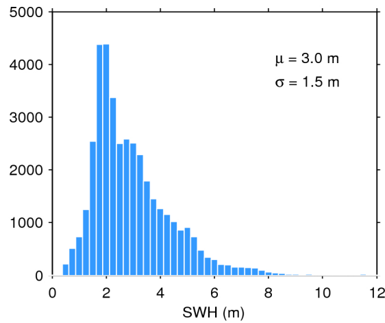
Figure 17. Histogram of flag-valid SWH over oceans and lakes for 12/09/2015. The mean ( \mu ) and standard deviation ( \sigma ) are also shown. Note that values larger than 12 m are excluded from the histogram for the sake of readability but not from the computation of \mu and \sigma .
