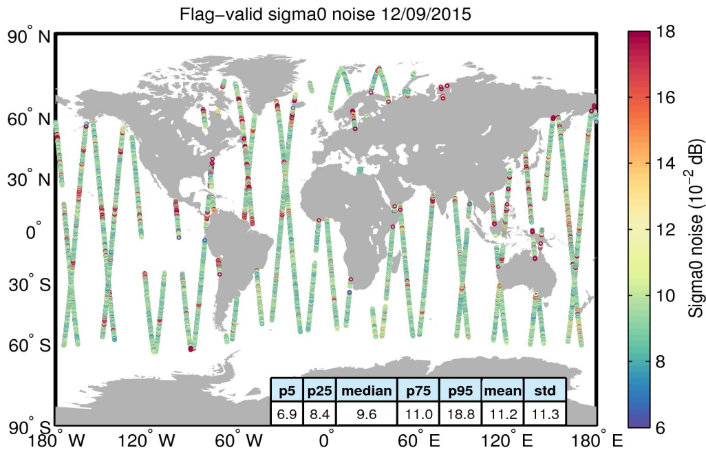
Figure 26. Geographical distribution of flag-valid 20-Hz sigma0 measurement noise over oceans and lakes for 12/09/2015. The statistical values shown in the table refer to the sigma0 noise and are calculated over all measurements shown in the figure.
