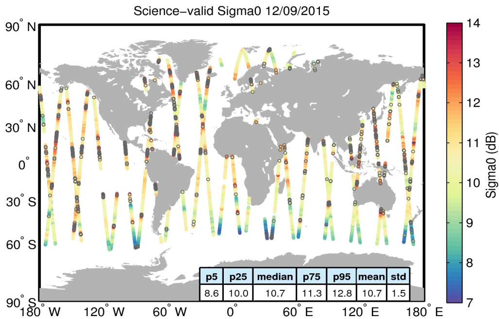
Figure 27. Geographical distribution of science-valid sigma0 data over oceans and lakes for 12/09/2015. The statistical values shown in the table refer to the sigma0 in dB and are calculated over all measurements shown in the figure. Gray circles denote records that have been rejected based on the editing criteria described in Table 4.
