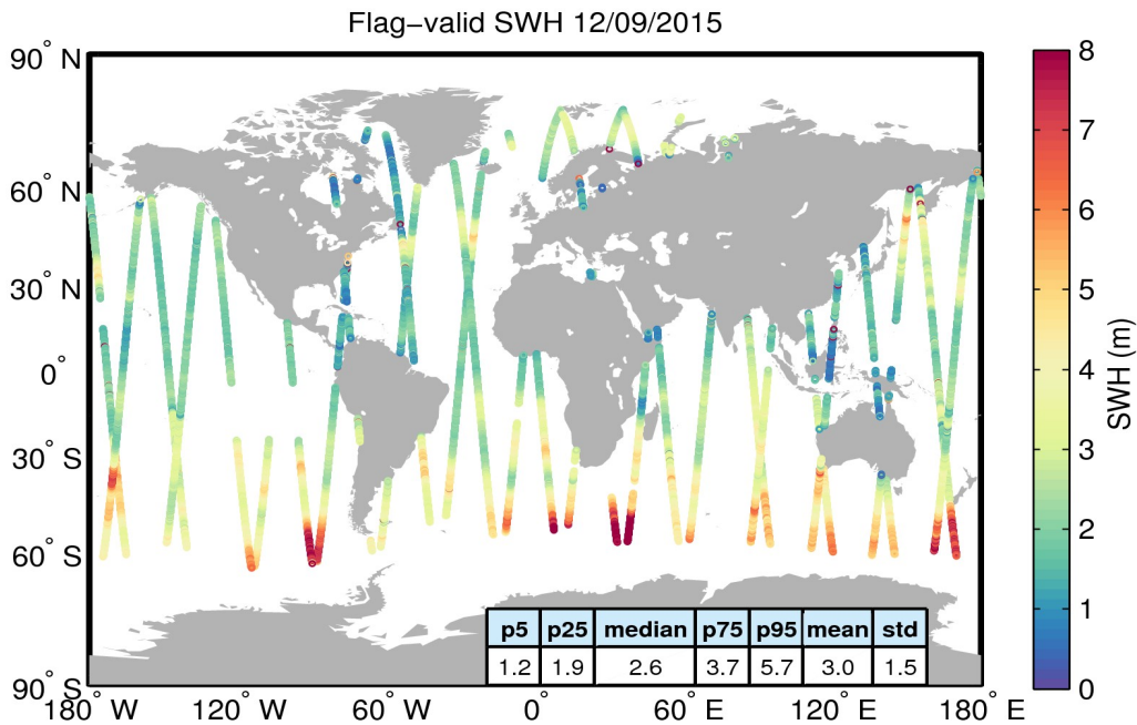
Figure 15. Geographical distribution of flag-valid SWH data over oceans and lakes for 12/09/2015. The statistical values shown in the table refer to the SWH in m and are calculated over all measurements shown in the figure.
