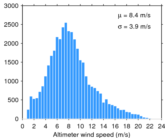
Figure 35. Histogram of science-valid wind over oceans and lakes for 12/09/2015. The mean ( \mu ) and standard deviation ( \sigma ) are also shown. Note that values larger than 24 m/s are excluded from the histogram for the sake of readability but not from the computation of \mu and \sigma .
