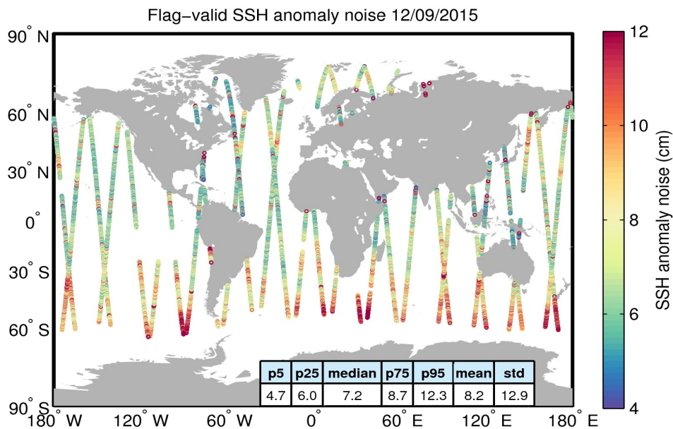
Figure 8. Geographical distribution of flag-valid 20-Hz SSH anomaly measurement noise over oceans and lakes for 12/09/2015. The statistical values shown in the table refer to the SSH anomaly noise and are calculated over all measurements shown in the figure.
