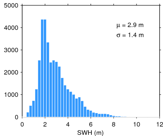
Figure 20. Histogram of science-valid SWH over oceans and lakes for 12/09/2015. The mean ( \mu ) and standard deviation ( \sigma ) are also shown. Note that values larger than 12 m are excluded from the histogram for the sake of readability but not from the computation of \mu and \sigma .
