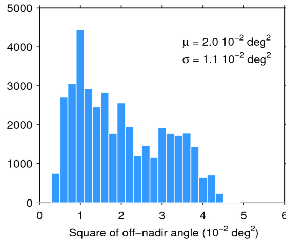
Figure 39. Histogram of flag-valid mispointing over oceans and lakes for 12/09/2015. The mean ( \mu ) and standard deviation ( \sigma ) are also shown. Note that values larger than 6 \cdot 10^{-2} \text{ deg}^2 are excluded from the histogram for the sake of readability but not from the computation of \mu and \sigma .
