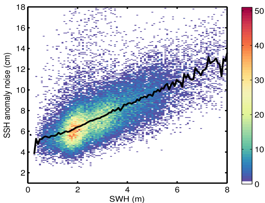
Figure 9. 2D histogram showing flag-valid SSH anomaly noise as a function of SWH for 12/09/2015. The black line denotes the median SSH anomaly noise as a function of SWH.
