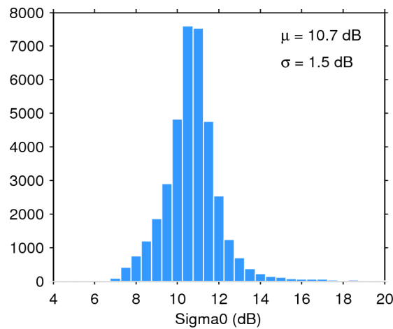
Figure 28. Histogram of science-valid sigma0 over oceans and lakes for 12/09/2015. The mean ( \mu ) and standard deviation ( \sigma ) are also shown. Note that values outside [4 20] dB are excluded from the histogram for the sake of readability but not from the computation of \mu and \sigma .
