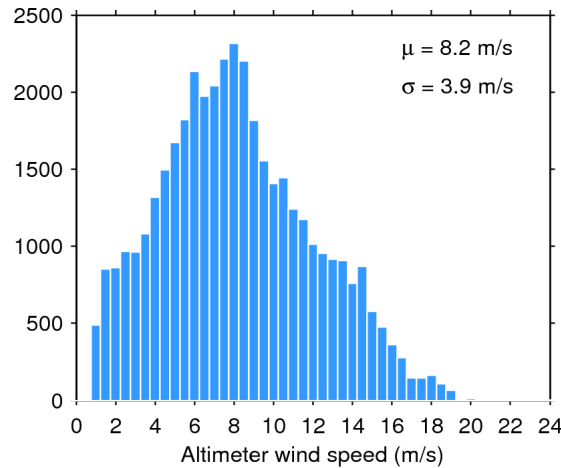
Figure 33. Histogram of flag-valid wind over oceans and lakes for 11/09/2015. The mean ( \mu ) and standard deviation ( \sigma ) are also shown. Note that values larger than 24 m/s are excluded from the histogram for the sake of readability but not from the computation of \mu and \sigma .
