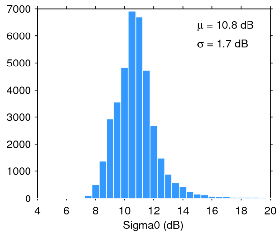
Figure 28. Histogram of science-valid sigma0 over oceans and lakes for 11/09/2015. The mean ( \mu ) and standard deviation ( \sigma ) are also shown. Note that values outside [4 20] dB are excluded from the histogram for the sake of readability but not from the computation of \mu and \sigma .
