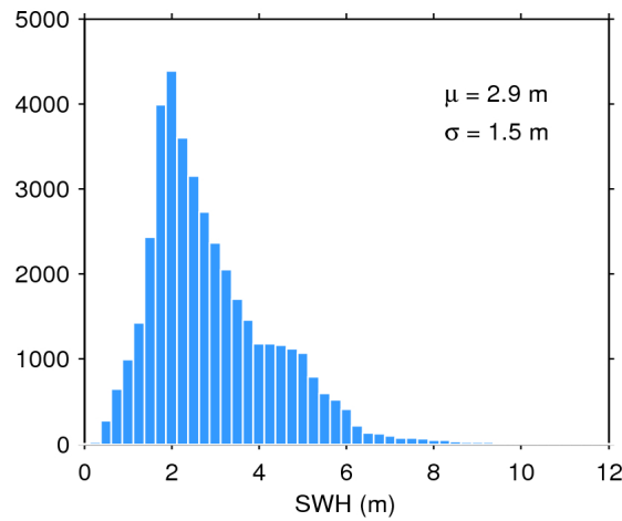
Figure 17. Histogram of flag-valid SWH over oceans and lakes for 11/09/2015. The mean ( \mu ) and standard deviation ( \sigma ) are also shown. Note that values larger than 12 m are excluded from the histogram for the sake of readability but not from the computation of \mu and \sigma .
