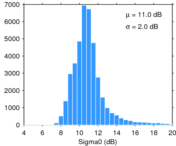
Figure 25. Histogram of flag-valid sigma0 over oceans and lakes for 11/09/2015. The mean ( \mu ) and standard deviation ( \sigma ) are also shown. Note that values outside [4 20] dB are excluded from the histogram for the sake of readability but not from the computation of \mu and \sigma .
