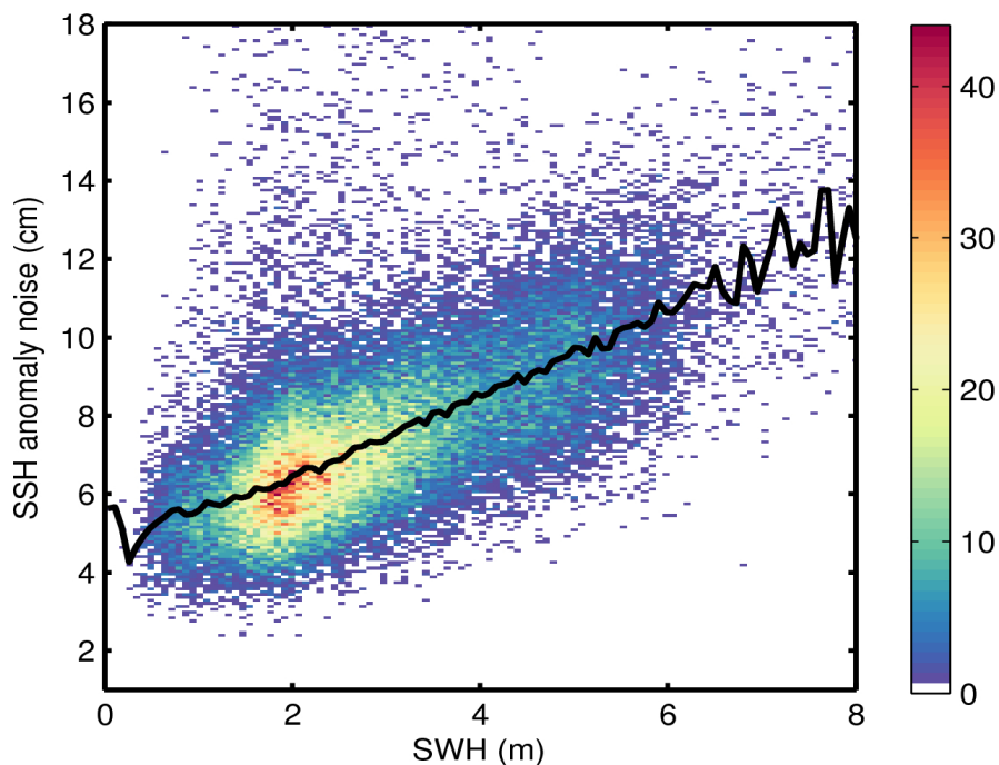
Figure 9. 2D histogram showing flag-valid SSH anomaly noise as a function of SWH for 11/09/2015. The black line denotes the median SSH anomaly noise as a function of SWH.
