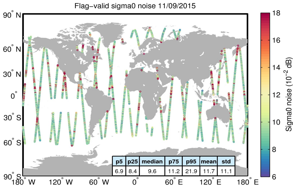
Figure 26. Geographical distribution of flag-valid 20-Hz sigma0 measurement noise over oceans and lakes for 11/09/2015. The statistical values shown in the table refer to the sigma0 noise and are calculated over all measurements shown in the figure.
