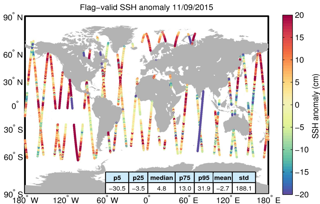
Figure 5. Geographical distribution of flag-valid 1-Hz SSH anomaly data over oceans and lakes for 11/09/2015. The statistical values shown in the table refer to the SSH anomaly in cm and are calculated over all measurements shown in the figure.
