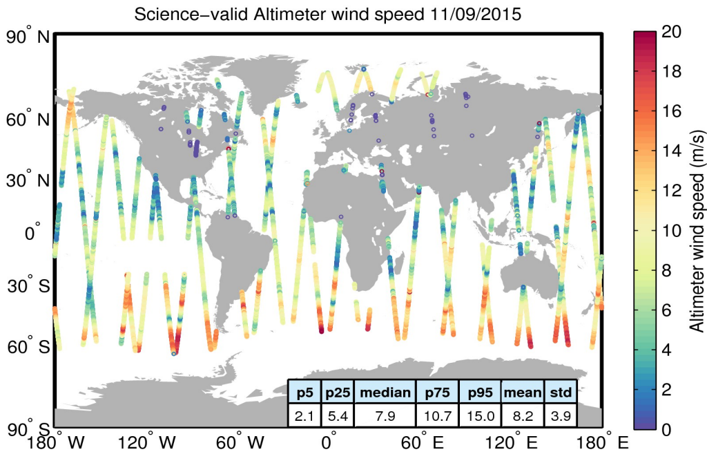
Figure 34. Geographical distribution of science-valid wind data over oceans and lakes for 11/09/2015. The statistical values shown in the table refer to the wind in m/s and are calculated over all measurements shown in the figure. Gray circles denote records that have been rejected based on the editing criteria described in Table 5.
