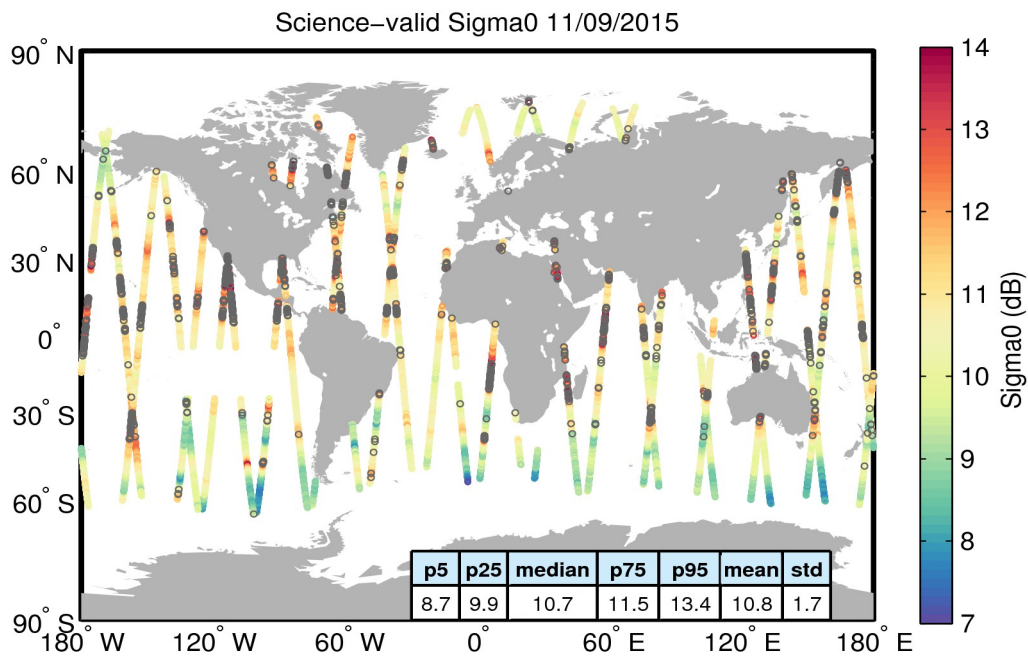
Figure 27. Geographical distribution of science-valid sigma0 data over oceans and lakes for 11/09/2015. The statistical values shown in the table refer to the sigma0 in dB and are calculated over all measurements shown in the figure. Gray circles denote records that have been rejected based on the editing criteria described in Table 4.
