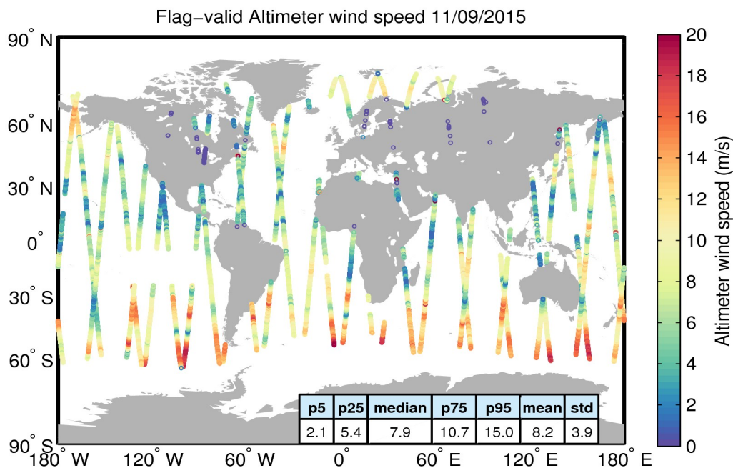
Figure 31. Geographical distribution of flag-valid wind data over oceans and lakes for 11/09/2015. The statistical values shown in the table refer to the wind in m/s and are calculated over all measurements shown in the figure.
