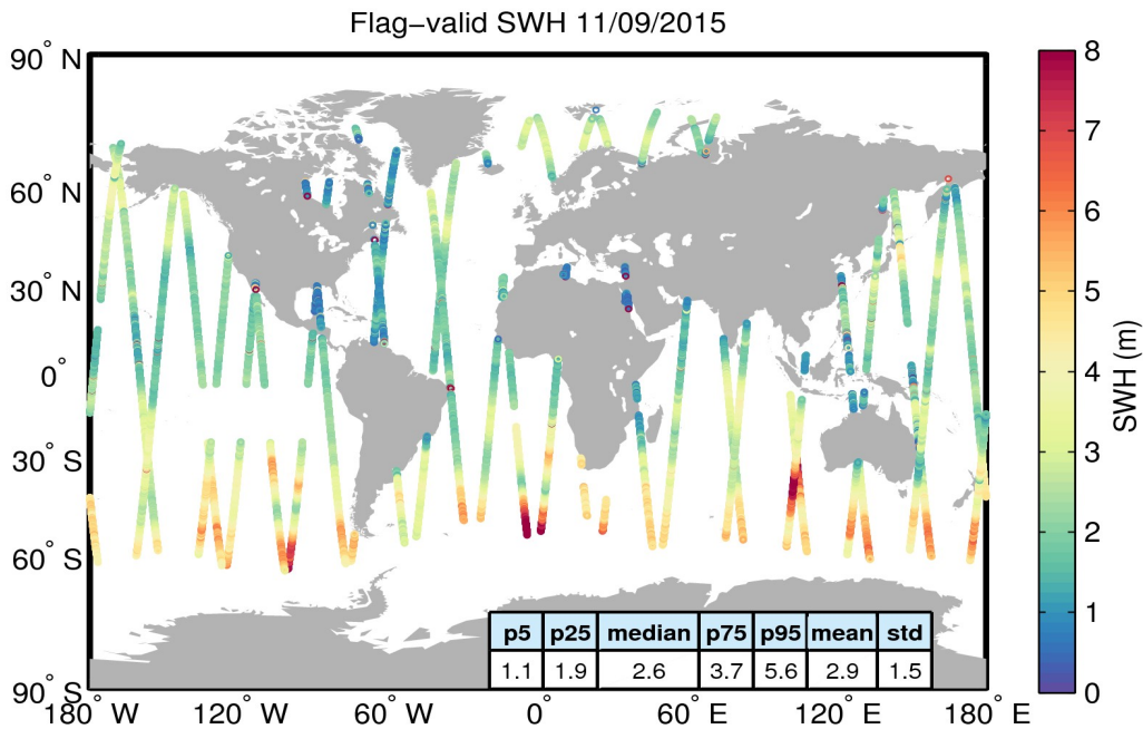
Figure 15. Geographical distribution of flag-valid SWH data over oceans and lakes for 11/09/2015. The statistical values shown in the table refer to the SWH in m and are calculated over all measurements shown in the figure.
