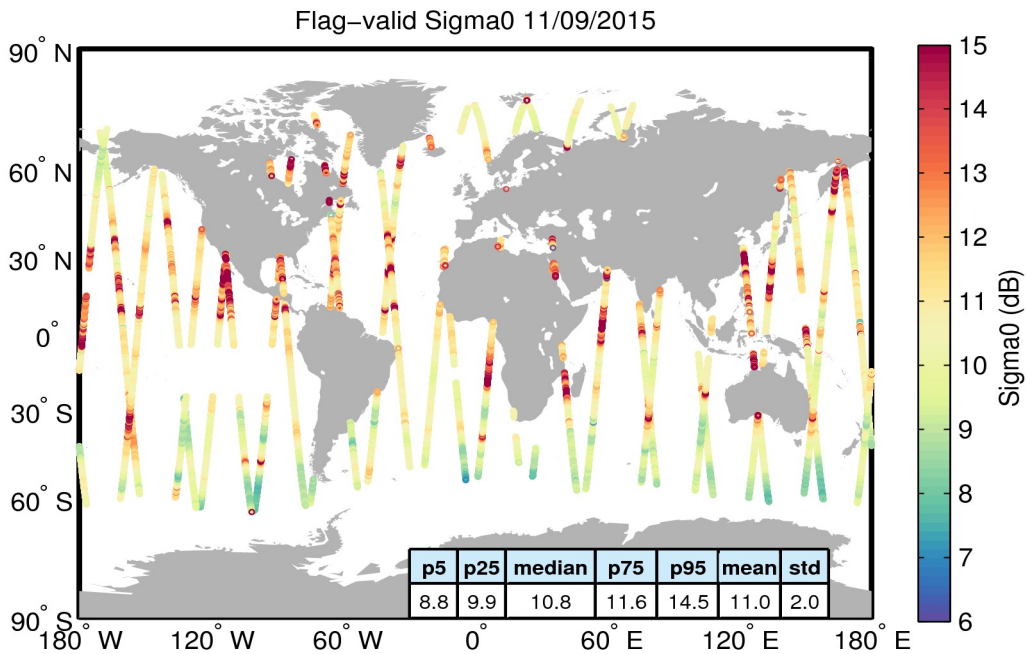
Figure 23. Geographical distribution of flag-valid sigma0 data over oceans and lakes for 11/09/2015. The statistical values shown in the table refer to the sigma0 in dB and are calculated over all measurements shown in the figure.
