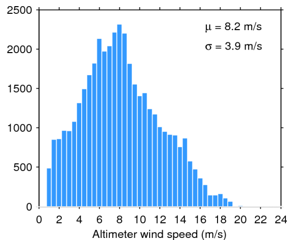
Figure 35. Histogram of science-valid wind over oceans and lakes for 11/09/2015. The mean ( \mu ) and standard deviation ( \sigma ) are also shown. Note that values larger than 24 m/s are excluded from the histogram for the sake of readability but not from the computation of \mu and \sigma .
