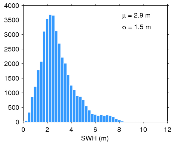
Figure 17. Histogram of flag-valid SWH over oceans and lakes for 07/09/2015. The mean ( \mu ) and standard deviation ( \sigma ) are also shown. Note that values larger than 12 m are excluded from the histogram for the sake of readability but not from the computation of \mu and \sigma .
