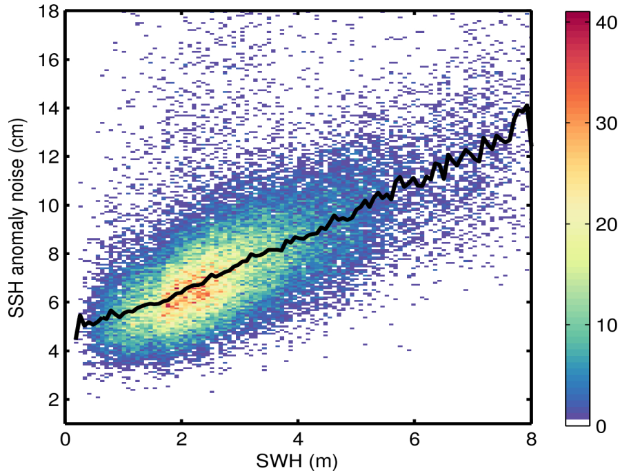
Figure 9. 2D histogram showing flag-valid SSH anomaly noise as a function of SWH for 07/09/2015. The black line denotes the median SSH anomaly as a function of SWH.
