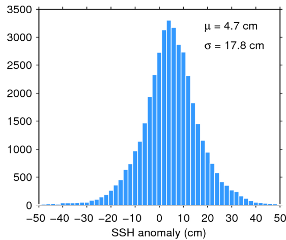
Figure 7. Histogram of flag-valid SSH anomaly over oceans and lakes for 07/09/2015. The mean ( \mu ) and standard deviation ( \sigma ) are also shown. Note that values outside [-50\ 50] cm are excluded from the histogram for the sake of readability but not from the computation of \mu and \sigma .
