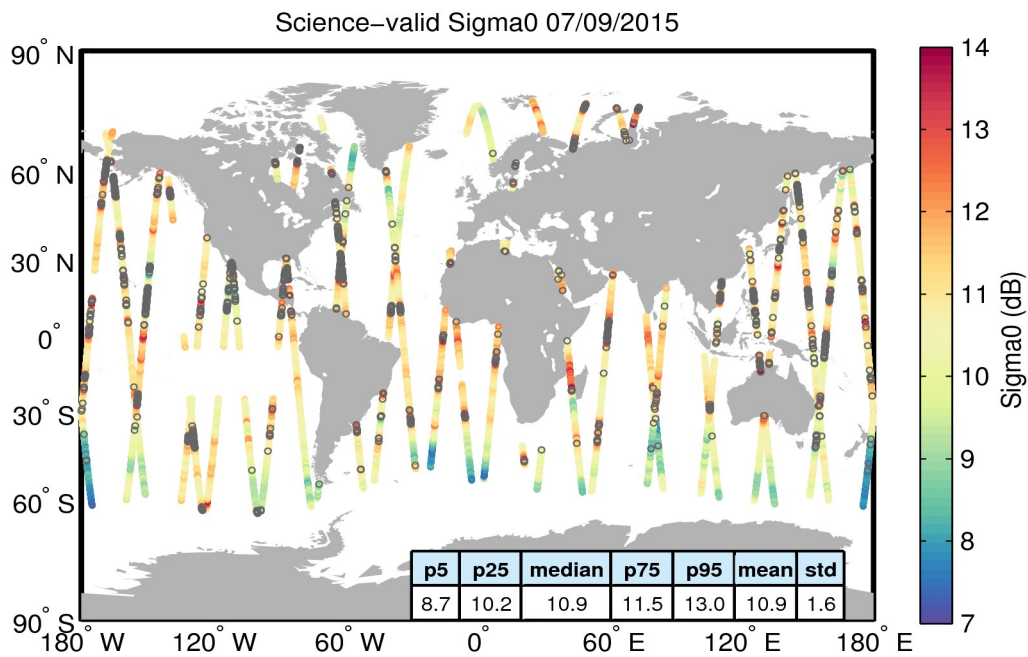
Figure 27. Geographical distribution of science-valid sigma0 data over oceans and lakes for 07/09/2015. The statistical values shown in the table refer to the sigma0 in dB and are calculated over all measurements shown in the figure. Gray circles denote records that have been rejected based on the editing criteria described in Table 4.
