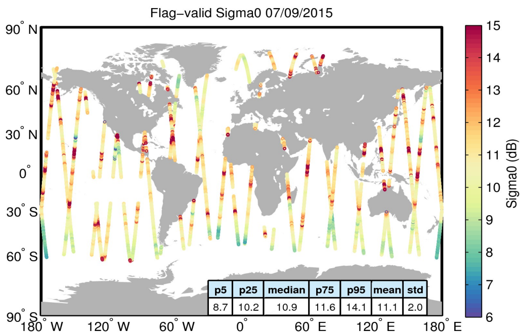
Figure 23. Geographical distribution of flag-valid sigma0 data over oceans and lakes for 07/09/2015. The statistical values shown in the table refer to the sigma0 in dB and are calculated over all measurements shown in the figure.
