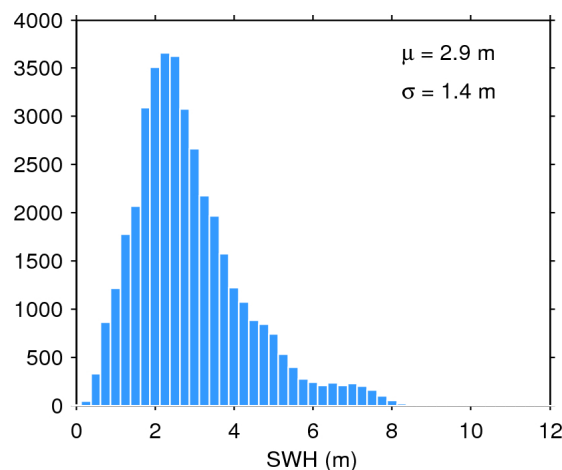
Figure 20. Histogram of science-valid SWH over oceans and lakes for 07/09/2015. The mean ( \mu ) and standard deviation ( \sigma ) are also shown. Note that values larger than 12 m are excluded from the histogram for the sake of readability but not from the computation of \mu and \sigma .
