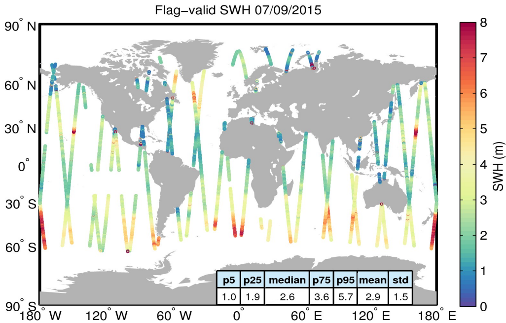
Figure 15. Geographical distribution of flag-valid SWH data over oceans and lakes for 07/09/2015. The statistical values shown in the table refer to the SWH in m and are calculated over all measurements shown in the figure.
