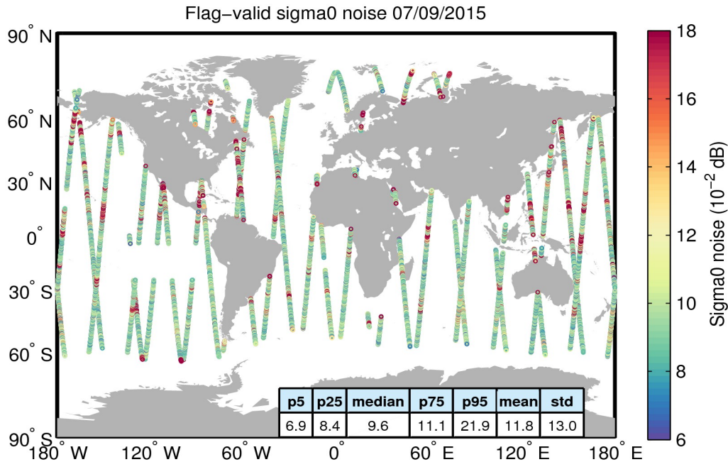
Figure 26. Geographical distribution of flag-valid 20-Hz sigma0 measurement noise over oceans and lakes for 07/09/2015. The statistical values shown in the table refer to the sigma0 noise and are calculated over all measurements shown in the figure.
