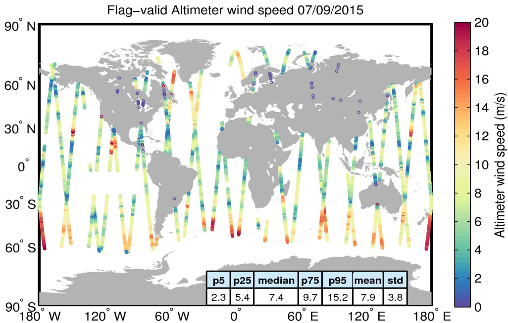
Figure 31. Geographical distribution of flag-valid wind data over oceans and lakes for 07/09/2015. The statistical values shown in the table refer to the wind in m/s and are calculated over all measurements shown in the figure.
