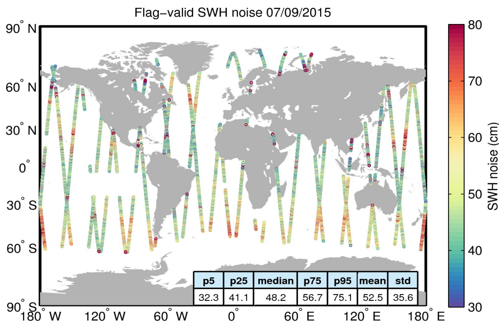
Figure 18. Geographical distribution of flag-valid 20-Hz SWH measurement noise over oceans and lakes for 07/09/2015. The statistical values shown in the table refer to the SWH noise and are calculated over all measurements shown in the figure.
