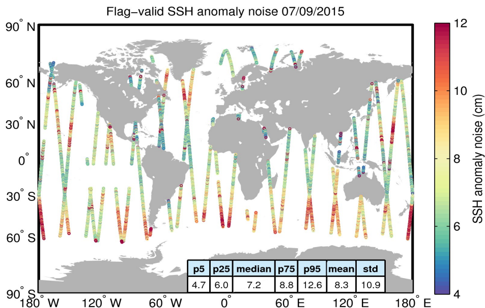
Figure 8. Geographical distribution of flag-valid 20-Hz SSH anomaly measurement noise over oceans and lakes for 07/09/2015. The statistical values shown in the table refer to the SSH anomaly noise and are calculated over all measurements shown in the figure.
