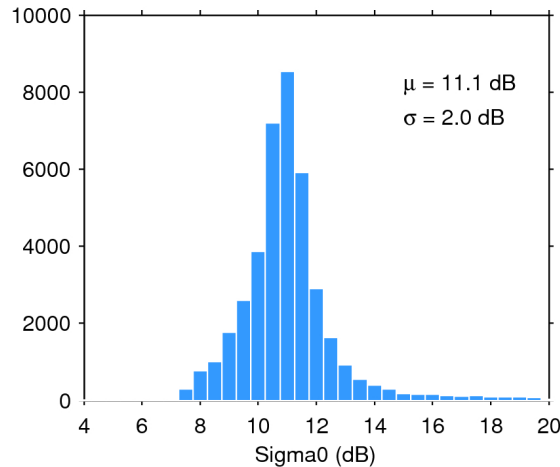
Figure 25. Histogram of flag-valid sigma0 over oceans and lakes for 07/09/2015. The mean ( \mu ) and standard deviation ( \sigma ) are also shown. Note that values outside [4 20] dB are excluded from the histogram for the sake of readability but not from the computation of \mu and \sigma .
