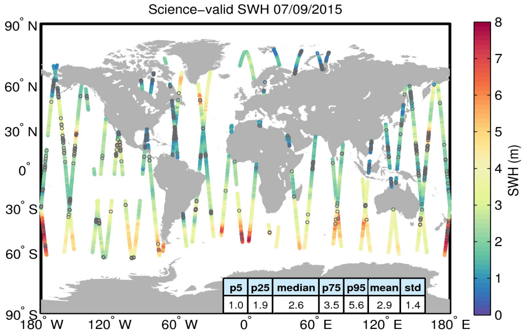
Figure 19. Geographical distribution of science-valid SWH data over oceans and lakes for 07/09/2015. The statistical values shown in the table refer to the SWH in m and are calculated over all measurements shown in the figure. Gray circles denote records that have been rejected based on the editing criteria described in Table 3.
