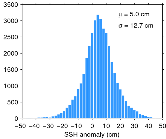
Figure 11. Histogram of science-valid SSH anomaly over oceans and lakes for 07/09/2015. The mean ( \mu ) and standard deviation ( \sigma ) are also shown. Note that values outside [-50 50] cm are excluded from the histogram for the sake of readability but not from the computation of \mu and \sigma .
