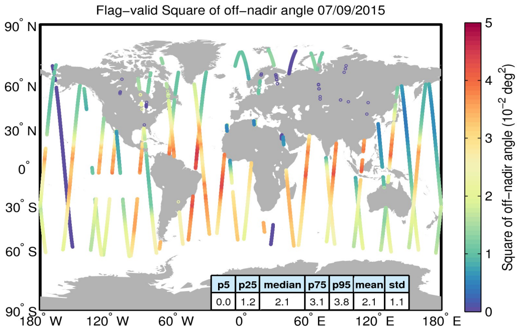
Figure 37. Geographical distribution of flag-valid mispointing data over oceans and lakes for 07/09/2015. The statistical values shown in the table refer to the mispointing in 10^{-2} \text{deg}^2 and are calculated over all measurements shown in the figure.
