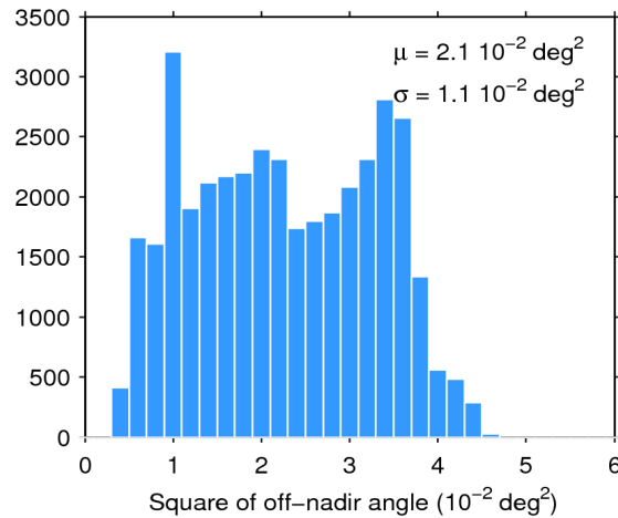
Figure 39. Histogram of flag-valid mispointing over oceans and lakes for 07/09/2015. The mean ( \mu ) and standard deviation ( \sigma ) are also shown. Note that values larger than 6 \cdot 10^{-2} \text{ deg}^2 are excluded from the histogram for the sake of readability but not from the computation of \mu and \sigma .
