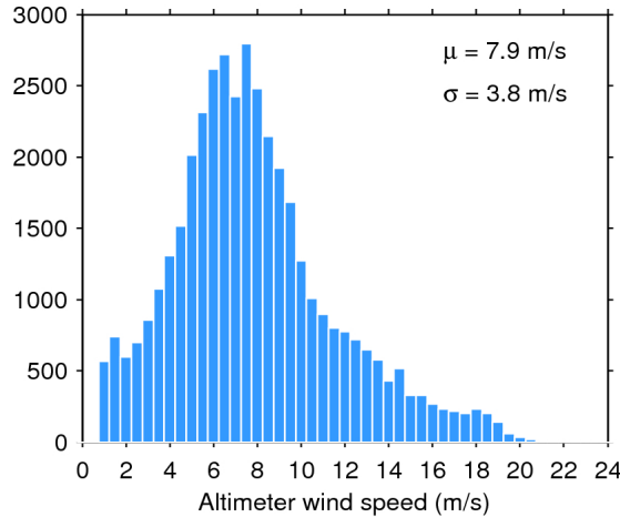
Figure 33. Histogram of flag-valid wind over oceans and lakes for 07/09/2015. The mean ( \mu ) and standard deviation ( \sigma ) are also shown. Note that values larger than 24 m/s are excluded from the histogram for the sake of readability but not from the computation of \mu and \sigma .
