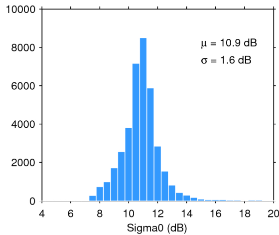
Figure 28. Histogram of science-valid sigma0 over oceans and lakes for 07/09/2015. The mean ( \mu ) and standard deviation ( \sigma ) are also shown. Note that values outside [4 20] dB are excluded from the histogram for the sake of readability but not from the computation of \mu and \sigma .
