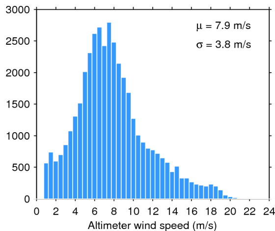
Figure 35. Histogram of science-valid wind over oceans and lakes for 07/09/2015. The mean ( \mu ) and standard deviation ( \sigma ) are also shown. Note that values larger than 24 m/s are excluded from the histogram for the sake of readability but not from the computation of \mu and \sigma .
