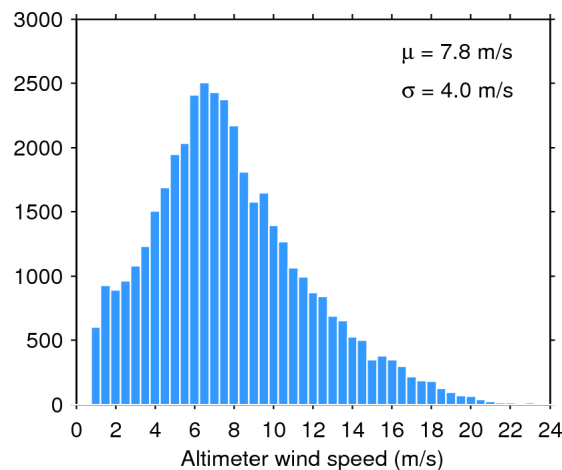
Figure 35. Histogram of science-valid wind over oceans and lakes for 03/09/2015. The mean ( \mu ) and standard deviation ( \sigma ) are also shown. Note that values larger than 24 m/s are excluded from the histogram for the sake of readability but not from the computation of \mu and \sigma .
