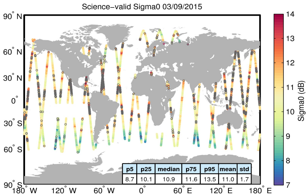
Figure 27. Geographical distribution of science-valid sigma0 data over oceans and lakes for 03/09/2015. The statistical values shown in the table refer to the sigma0 in dB and are calculated over all measurements shown in the figure. Gray circles denote records that have been rejected based on the editing criteria described in Table 4.
