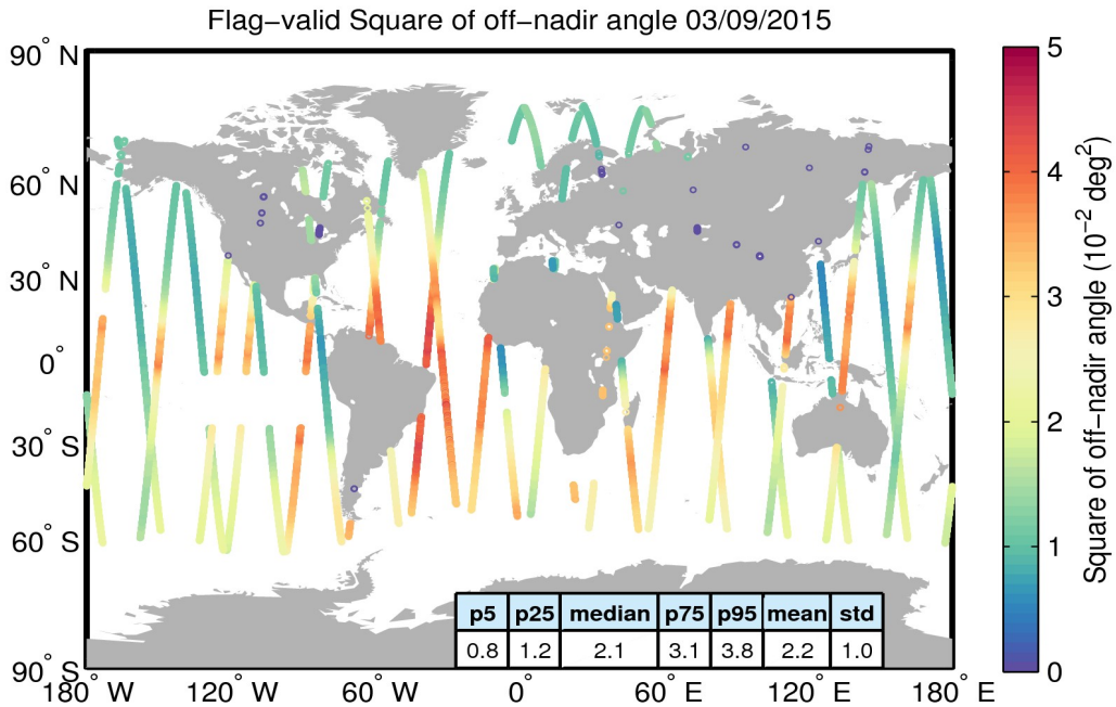
Figure 37. Geographical distribution of flag-valid mispointing data over oceans and lakes for 03/09/2015. The statistical values shown in the table refer to the mispointing in 10^{-2} \text{ deg}^2 and are calculated over all measurements shown in the figure.
