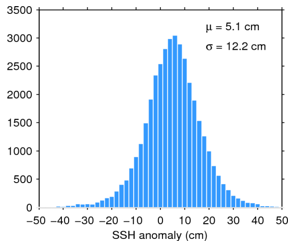
Figure 11. Histogram of science-valid SSH anomaly over oceans and lakes for 03/09/2015. The mean ( \mu ) and standard deviation ( \sigma ) are also shown. Note that values outside [-50 50] cm are excluded from the histogram for the sake of readability but not from the computation of \mu and \sigma .
