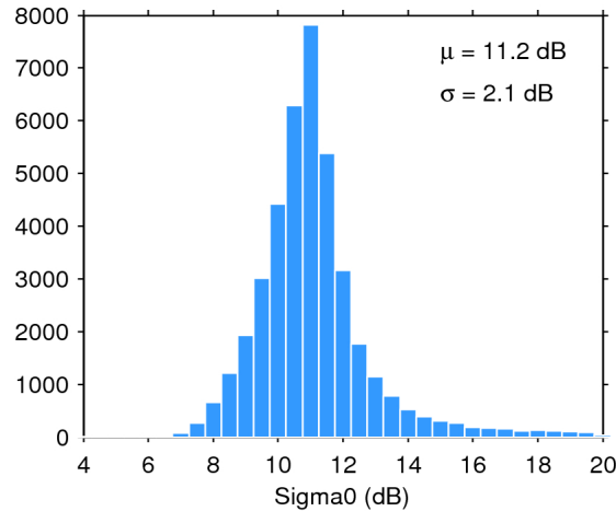
Figure 25. Histogram of flag-valid sigma0 over oceans and lakes for 03/09/2015. The mean ( \mu ) and standard deviation ( \sigma ) are also shown. Note that values outside [4 20] dB are excluded from the histogram for the sake of readability but not from the computation of \mu and \sigma .
