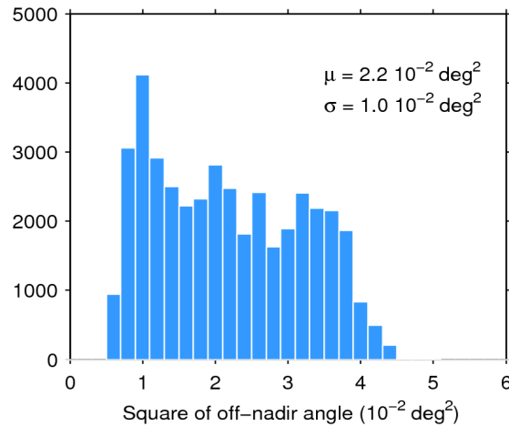
Figure 39. Histogram of flag-valid mispointing over oceans and lakes for 03/09/2015. The mean ( \mu ) and standard deviation ( \sigma ) are also shown. Note that values larger than 6 \cdot 10^{-2} \text{ deg}^2 are excluded from the histogram for the sake of readability but not from the computation of \mu and \sigma .
