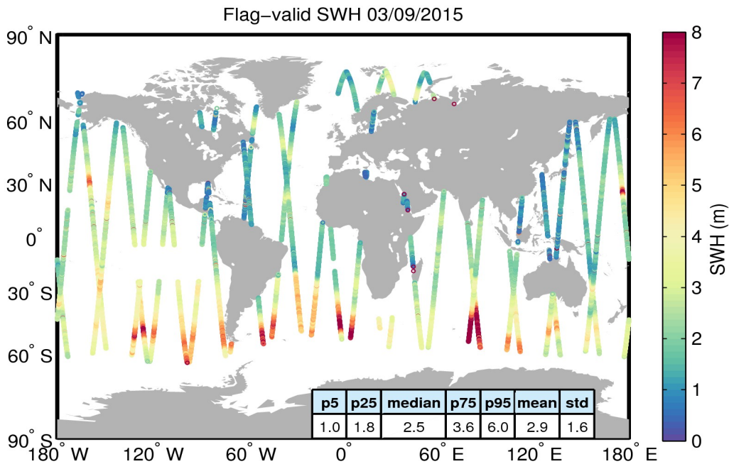
Figure 15. Geographical distribution of flag-valid SWH data over oceans and lakes for 03/09/2015. The statistical values shown in the table refer to the SWH in m and are calculated over all measurements shown in the figure.
