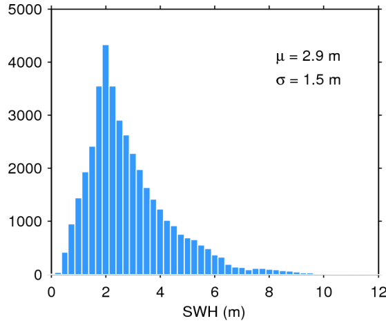
Figure 20. Histogram of science-valid SWH over oceans and lakes for 03/09/2015. The mean ( \mu ) and standard deviation ( \sigma ) are also shown. Note that values larger than 12 m are excluded from the histogram for the sake of readability but not from the computation of \mu and \sigma .
