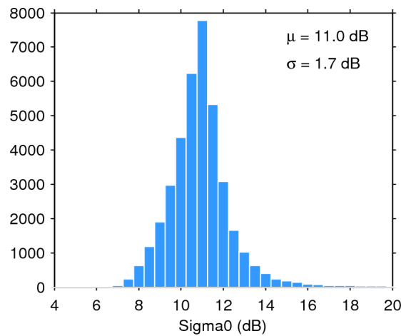
Figure 28. Histogram of science-valid sigma0 over oceans and lakes for 03/09/2015. The mean ( \mu ) and standard deviation ( \sigma ) are also shown. Note that values outside [4 20] dB are excluded from the histogram for the sake of readability but not from the computation of \mu and \sigma .
