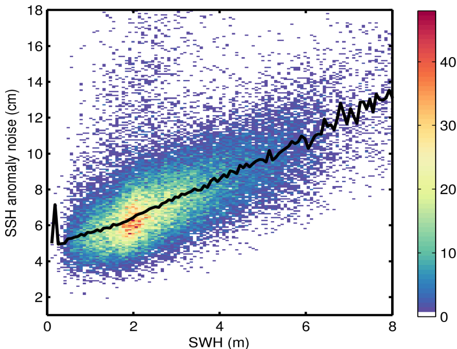
Figure 9. 2D histogram showing flag-valid SSH anomaly noise as a function of SWH for 03/09/2015. The black line denotes the median SSH anomaly as a function of SWH.
