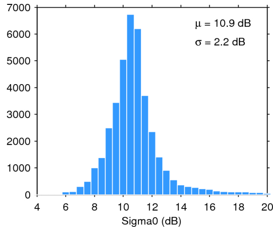
Figure 25. Histogram of flag-valid sigma0 over oceans and lakes for 02/09/2015. The mean ( \mu ) and standard deviation ( \sigma ) are also shown. Note that values outside [4 20] dB are excluded from the histogram for the sake of readability but not from the computation of \mu and \sigma .
