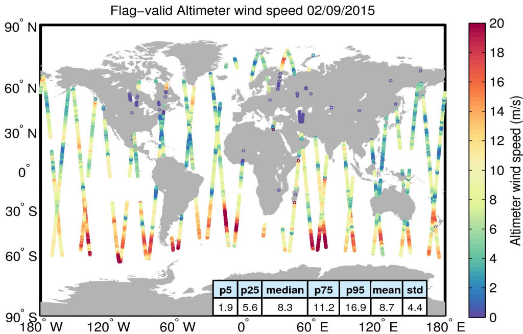
Figure 31. Geographical distribution of flag-valid wind data over oceans and lakes for 02/09/2015. The statistical values shown in the table refer to the wind in m/s and are calculated over all measurements shown in the figure.
