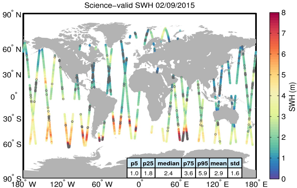
Figure 19. Geographical distribution of science-valid SWH data over oceans and lakes for 02/09/2015. The statistical values shown in the table refer to the SWH in m and are calculated over all measurements shown in the figure. Gray circles denote records that have been rejected based on the editing criteria described in Table 3.
