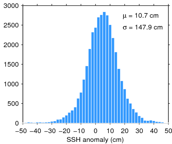
Figure 7. Histogram of flag-valid SSH anomaly over oceans and lakes for 02/09/2015. The mean ( \mu ) and standard deviation ( \sigma ) are also shown. Note that values outside [-50 50] cm are excluded from the histogram for the sake of readability but not from the computation of \mu and \sigma .
