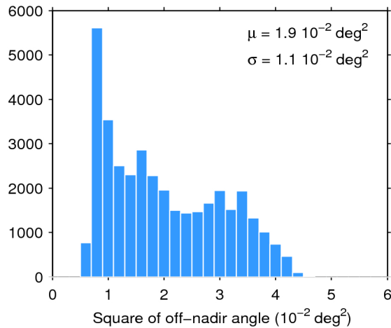
Figure 39. Histogram of flag-valid mispointing over oceans and lakes for 02/09/2015. The mean ( \mu ) and standard deviation ( \sigma ) are also shown. Note that values larger than 6 \cdot 10^{-2} \text{ deg}^2 are excluded from the histogram for the sake of readability but not from the computation of \mu and \sigma .
