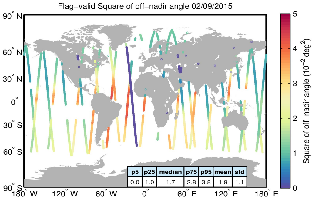
Figure 37. Geographical distribution of flag-valid mispointing data over oceans and lakes for 02/09/2015. The statistical values shown in the table refer to the mispointing in 10^{-2} deg 2 and are calculated over all measurements shown in the figure.
