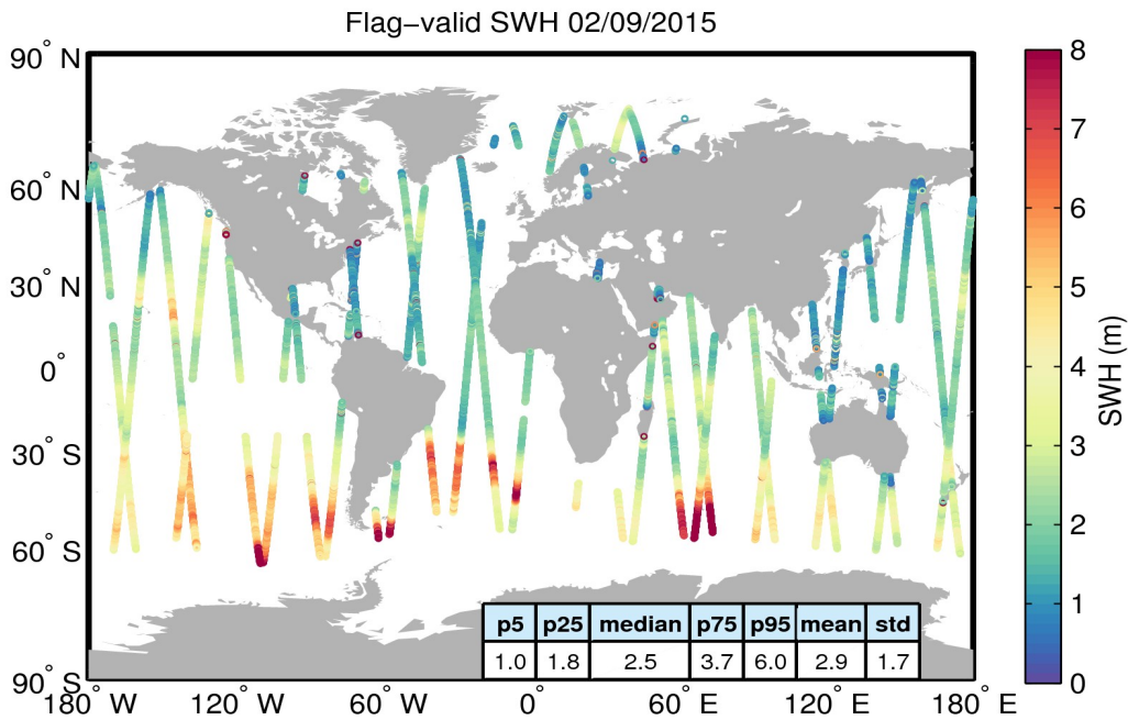
Figure 15. Geographical distribution of flag-valid SWH data over oceans and lakes for 02/09/2015. The statistical values shown in the table refer to the SWH in m and are calculated over all measurements shown in the figure.
