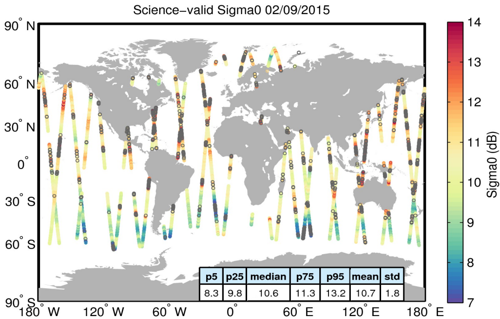
Figure 27. Geographical distribution of science-valid sigma0 data over oceans and lakes for 02/09/2015. The statistical values shown in the table refer to the sigma0 in dB and are calculated over all measurements shown in the figure. Gray circles denote records that have been rejected based on the editing criteria described in Table 4.
