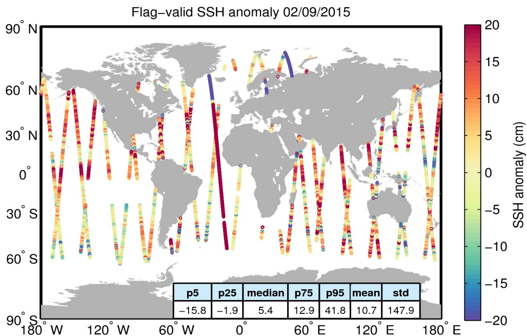
Figure 5. Geographical distribution of flag-valid 1-Hz SSH anomaly data over oceans and lakes for 02/09/2015. The statistical values shown in the table refer to the SSH anomaly in cm and are calculated over all measurements shown in the figure.
