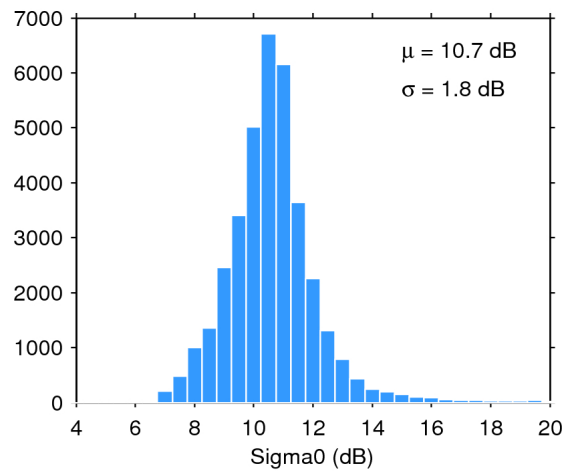
Figure 28. Histogram of science-valid sigma0 over oceans and lakes for 02/09/2015. The mean ( \mu ) and standard deviation ( \sigma ) are also shown. Note that values outside [4 20] dB are excluded from the histogram for the sake of readability but not from the computation of \mu and \sigma .
