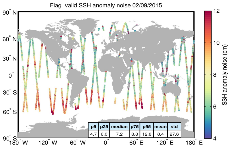
Figure 8. Geographical distribution of flag-valid 20-Hz SSH anomaly measurement noise over oceans and lakes for 02/09/2015. The statistical values shown in the table refer to the SSH anomaly noise and are calculated over all measurements shown in the figure.
