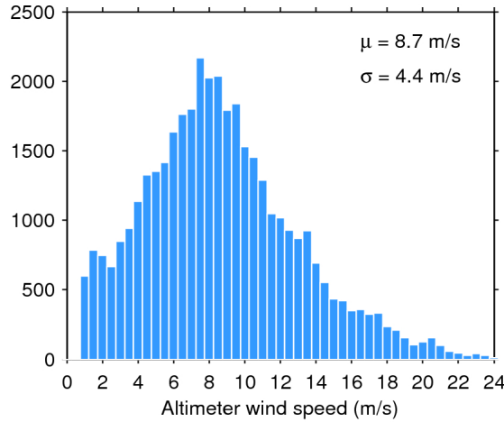
Figure 33. Histogram of flag-valid wind over oceans and lakes for 02/09/2015. The mean ( \mu ) and standard deviation ( \sigma ) are also shown. Note that values larger than 24 m/s are excluded from the histogram for the sake of readability but not from the computation of \mu and \sigma .
