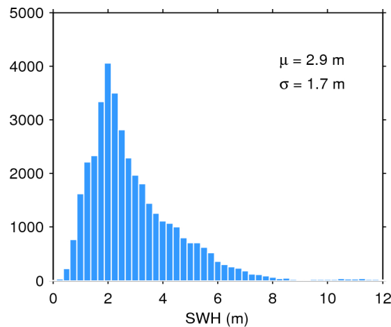
Figure 17. Histogram of flag-valid SWH over oceans and lakes for 02/09/2015. The mean ( \mu ) and standard deviation ( \sigma ) are also shown. Note that values larger than 12 m are excluded from the histogram for the sake of readability but not from the computation of \mu and \sigma .
