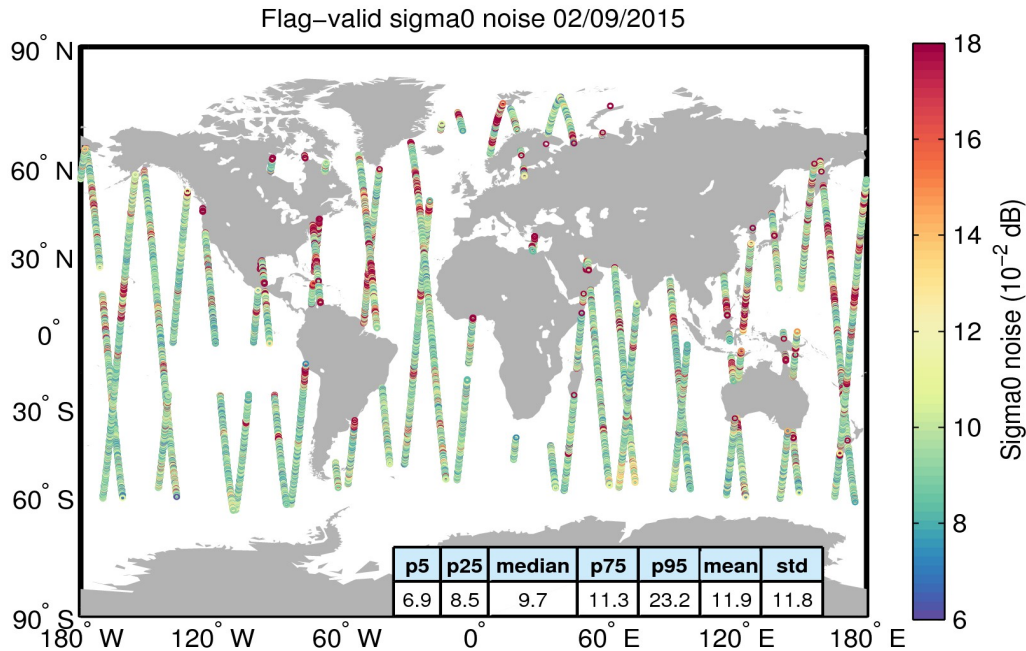
Figure 26. Geographical distribution of flag-valid 20-Hz sigma0 measurement noise over oceans and lakes for 02/09/2015. The statistical values shown in the table refer to the sigma0 noise and are calculated over all measurements shown in the figure.
