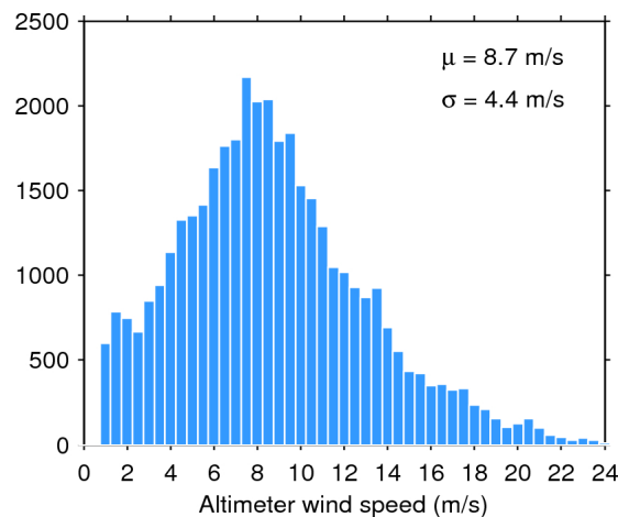
Figure 35. Histogram of science-valid wind over oceans and lakes for 02/09/2015. The mean ( \mu ) and standard deviation ( \sigma ) are also shown. Note that values larger than 24 m/s are excluded from the histogram for the sake of readability but not from the computation of \mu and \sigma .
