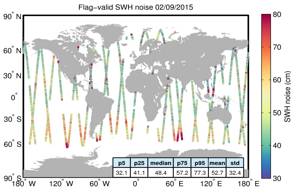
Figure 18. Geographical distribution of flag-valid 20-Hz SWH measurement noise over oceans and lakes for 02/09/2015. The statistical values shown in the table refer to the SWH noise and are calculated over all measurements shown in the figure.
