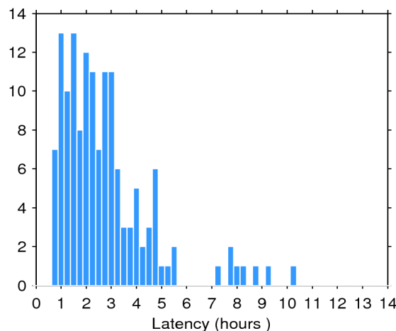
Figure 2. Histogram of the data latency for 02/09/2015. The y-axis denotes the number of files that are made available with a delay of x-hours with respect to the mean time of the records stored in the file.
