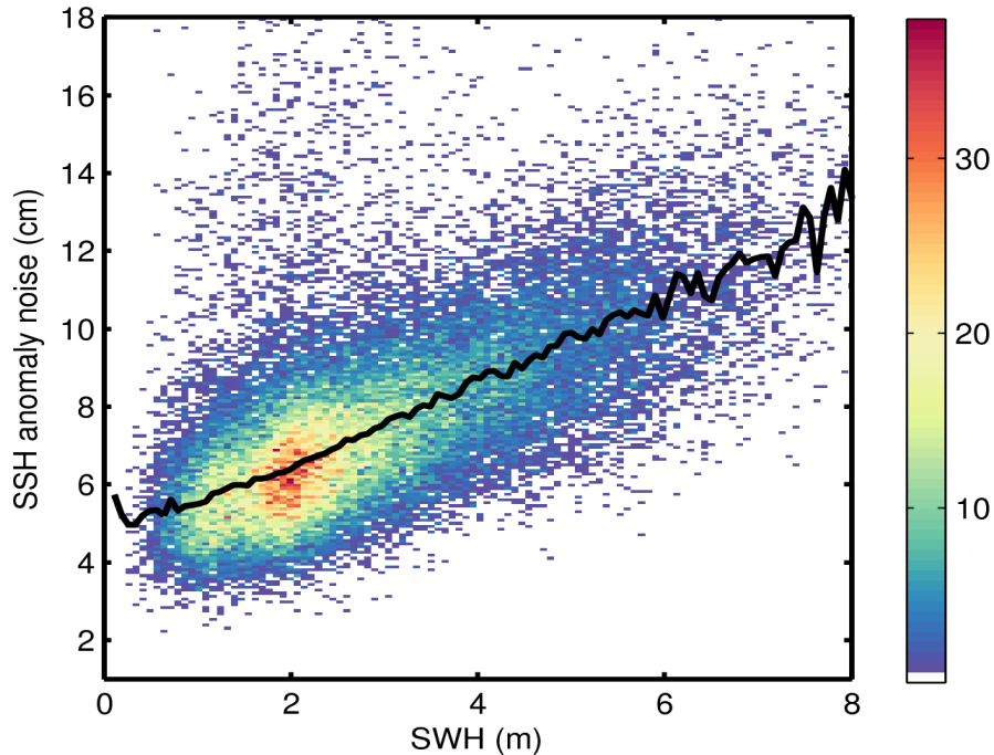
Figure 9. 2D histogram showing flag-valid SSH anomaly noise as a function of SWH for 02/09/2015. The black line denotes the median SSH anomaly as a function of SWH.
