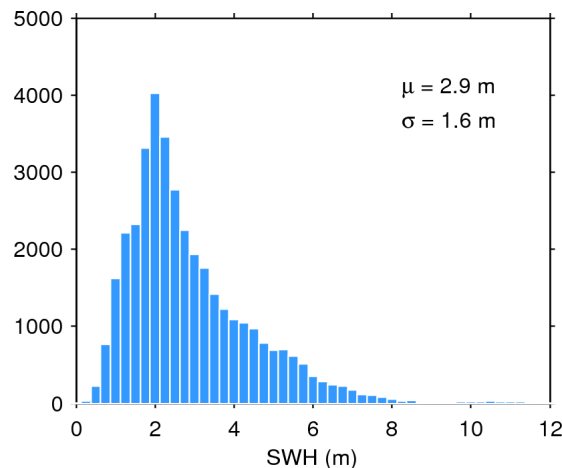
Figure 20. Histogram of science-valid SWH over oceans and lakes for 02/09/2015. The mean ( \mu ) and standard deviation ( \sigma ) are also shown. Note that values larger than 12 m are excluded from the histogram for the sake of readability but not from the computation of \mu and \sigma .
