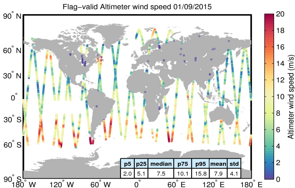
Figure 31. Geographical distribution of flag-valid wind data over oceans and lakes for 01/09/2015. The statistical values shown in the table refer to the wind in m/s and are calculated over all measurements shown in the figure.
