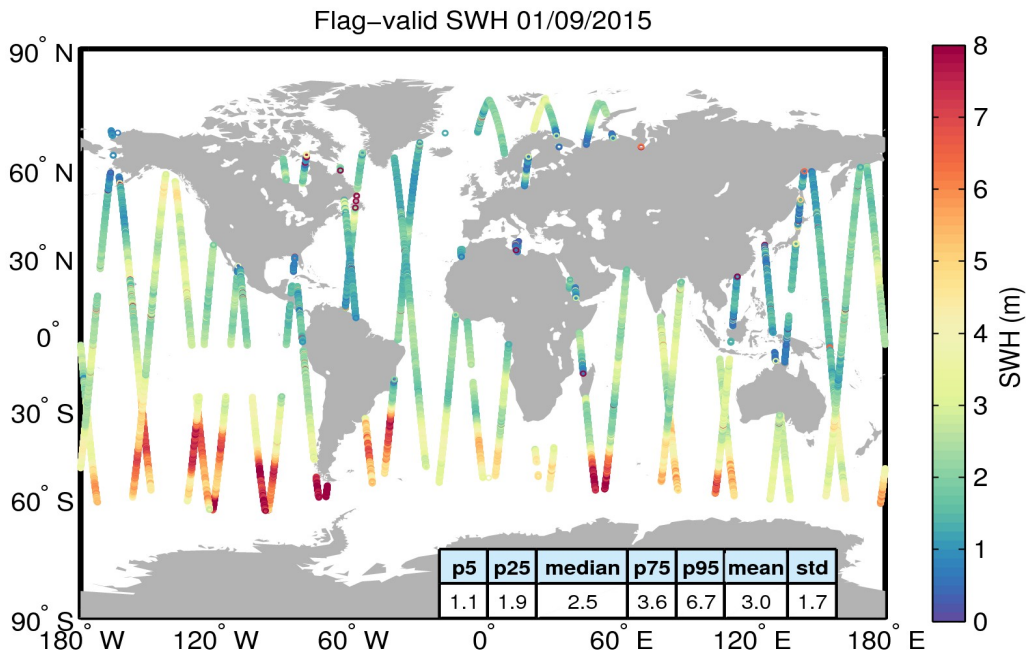
Figure 15. Geographical distribution of flag-valid SWH data over oceans and lakes for 01/09/2015. The statistical values shown in the table refer to the SWH in m and are calculated over all measurements shown in the figure.
