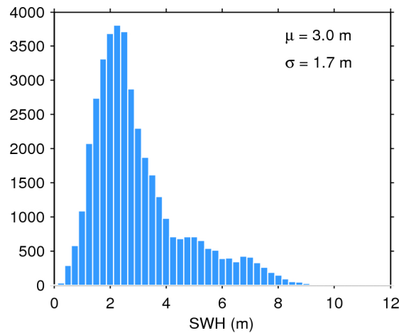
Figure 17. Histogram of flag-valid SWH over oceans and lakes for 01/09/2015. The mean ( \mu ) and standard deviation ( \sigma ) are also shown. Note that values larger than 12 m are excluded from the histogram for the sake of readability but not from the computation of \mu and \sigma .
