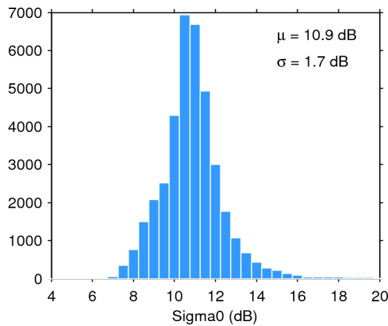
Figure 28. Histogram of science-valid sigma0 over oceans and lakes for 01/09/2015. The mean ( \mu ) and standard deviation ( \sigma ) are also shown. Note that values outside [4 20] dB are excluded from the histogram for the sake of readability but not from the computation of \mu and \sigma .
