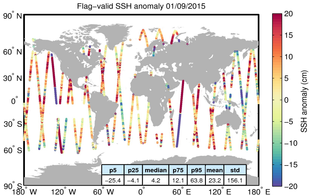
Figure 5. Geographical distribution of flag-valid 1-Hz SSH anomaly data over oceans and lakes for 01/09/2015. The statistical values shown in the table refer to the SSH anomaly in cm and are calculated over all measurements shown in the figure.
