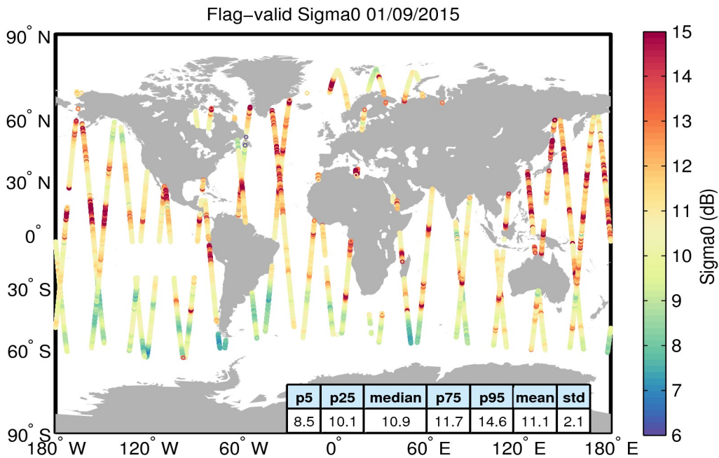
Figure 23. Geographical distribution of flag-valid sigma0 data over oceans and lakes for 01/09/2015. The statistical values shown in the table refer to the sigma0 in dB and are calculated over all measurements shown in the figure.
