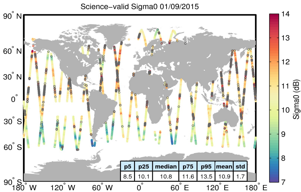
Figure 27. Geographical distribution of science-valid sigma0 data over oceans and lakes for 01/09/2015. The statistical values shown in the table refer to the sigma0 in dB and are calculated over all measurements shown in the figure. Gray circles denote records that have been rejected based on the editing criteria described in Table 4.
