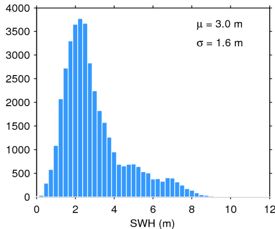
Figure 20. Histogram of science-valid SWH over oceans and lakes for 01/09/2015. The mean ( \mu ) and standard deviation ( \sigma ) are also shown. Note that values larger than 12 m are excluded from the histogram for the sake of readability but not from the computation of \mu and \sigma .
