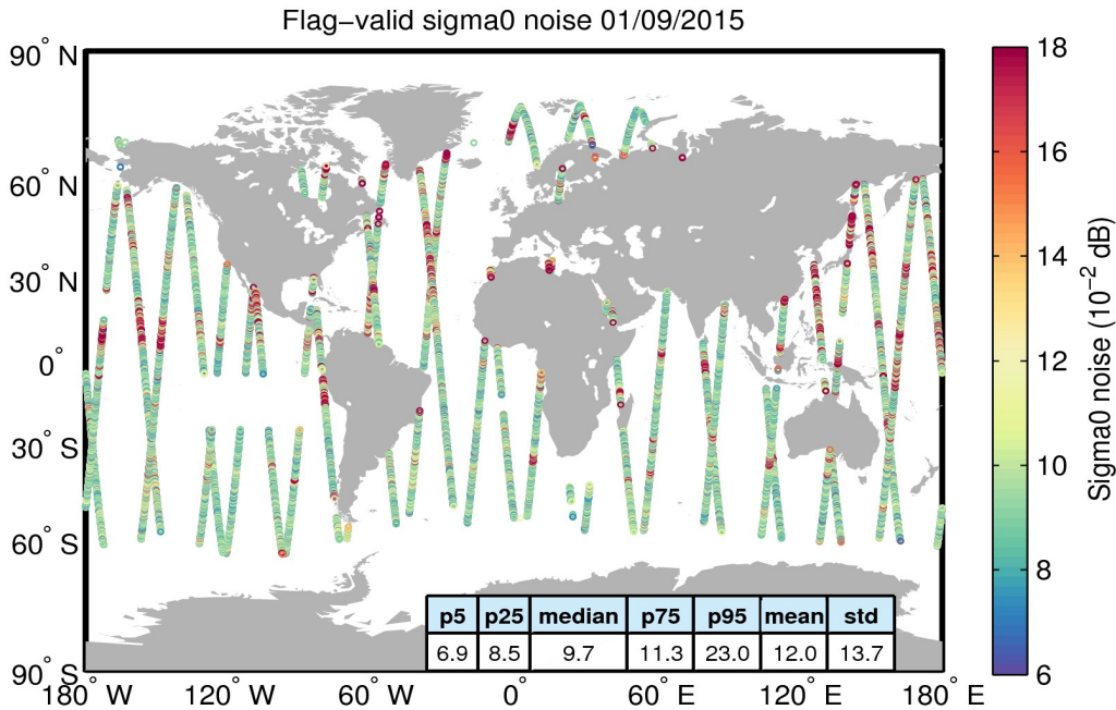
Figure 26. Geographical distribution of flag-valid 20-Hz sigma0 measurement noise over oceans and lakes for 01/09/2015. The statistical values shown in the table refer to the sigma0 noise and are calculated over all measurements shown in the figure.
