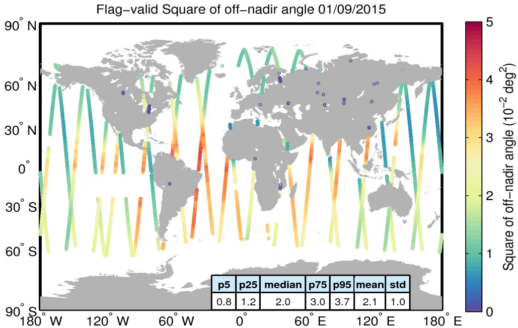
Figure 37. Geographical distribution of flag-valid mispointing data over oceans and lakes for 01/09/2015. The statistical values shown in the table refer to the mispointing in 10^{-2} \text{deg}^2 and are calculated over all measurements shown in the figure.
