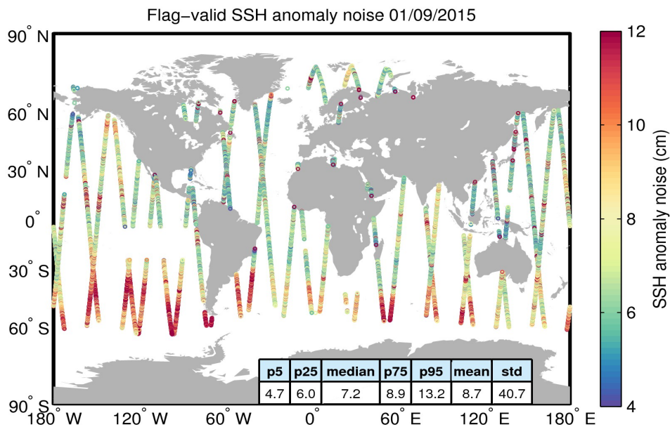
Figure 8. Geographical distribution of flag-valid 20-Hz SSH anomaly measurement noise over oceans and lakes for 01/09/2015. The statistical values shown in the table refer to the SSH anomaly noise and are calculated over all measurements shown in the figure.
