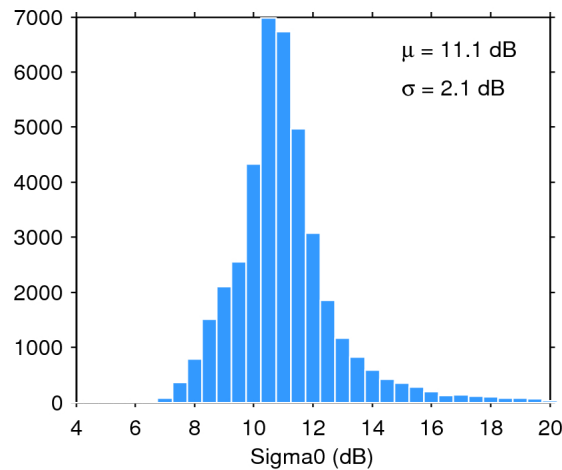
Figure 25. Histogram of flag-valid sigma0 over oceans and lakes for 01/09/2015. The mean ( \mu ) and standard deviation ( \sigma ) are also shown. Note that values outside [4 20] dB are excluded from the histogram for the sake of readability but not from the computation of \mu and \sigma .
