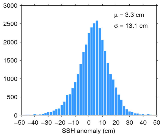
Figure 11. Histogram of science-valid SSH anomaly over oceans and lakes for 01/09/2015. The mean ( \mu ) and standard deviation ( \sigma ) are also shown. Note that values outside [-50 50] cm are excluded from the histogram for the sake of readability but not from the computation of \mu and \sigma .
