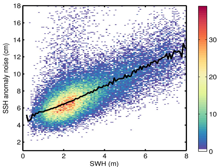
Figure 9. 2D histogram showing flag-valid SSH anomaly noise as a function of SWH for 01/09/2015. The black line denotes the median SSH anomaly as a function of SWH.
