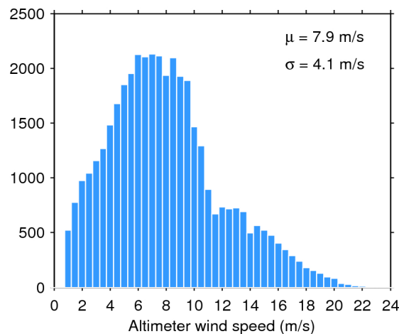
Figure 35. Histogram of science-valid wind over oceans and lakes for 01/09/2015. The mean ( \mu ) and standard deviation ( \sigma ) are also shown. Note that values larger than 24 m/s are excluded from the histogram for the sake of readability but not from the computation of \mu and \sigma .
