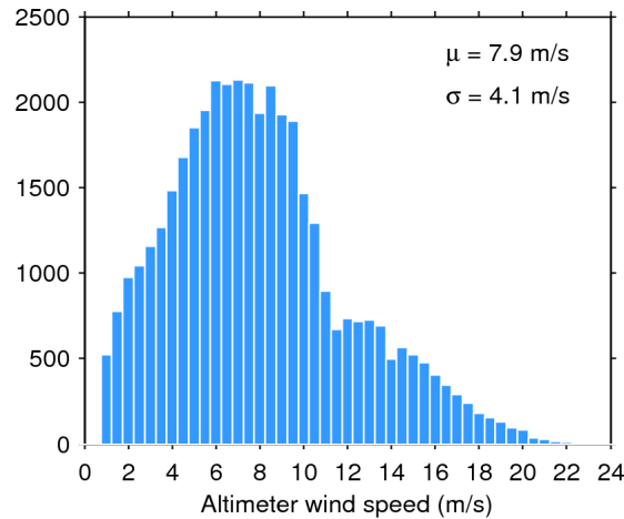
Figure 33. Histogram of flag-valid wind over oceans and lakes for 01/09/2015. The mean ( \mu ) and standard deviation ( \sigma ) are also shown. Note that values larger than 24 m/s are excluded from the histogram for the sake of readability but not from the computation of \mu and \sigma .
