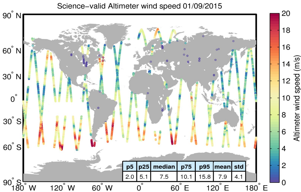
Figure 34. Geographical distribution of science-valid wind data over oceans and lakes for 01/09/2015. The statistical values shown in the table refer to the wind in m/s and are calculated over all measurements shown in the figure. Gray circles denote records that have been rejected based on the editing criteria described in Table 5.
