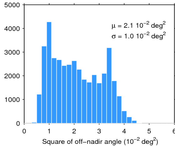
Figure 39. Histogram of flag-valid mispointing over oceans and lakes for 01/09/2015. The mean ( \mu ) and standard deviation ( \sigma ) are also shown. Note that values larger than 6 \cdot 10^{-2} \text{ deg}^2 are excluded from the histogram for the sake of readability but not from the computation of \mu and \sigma .
