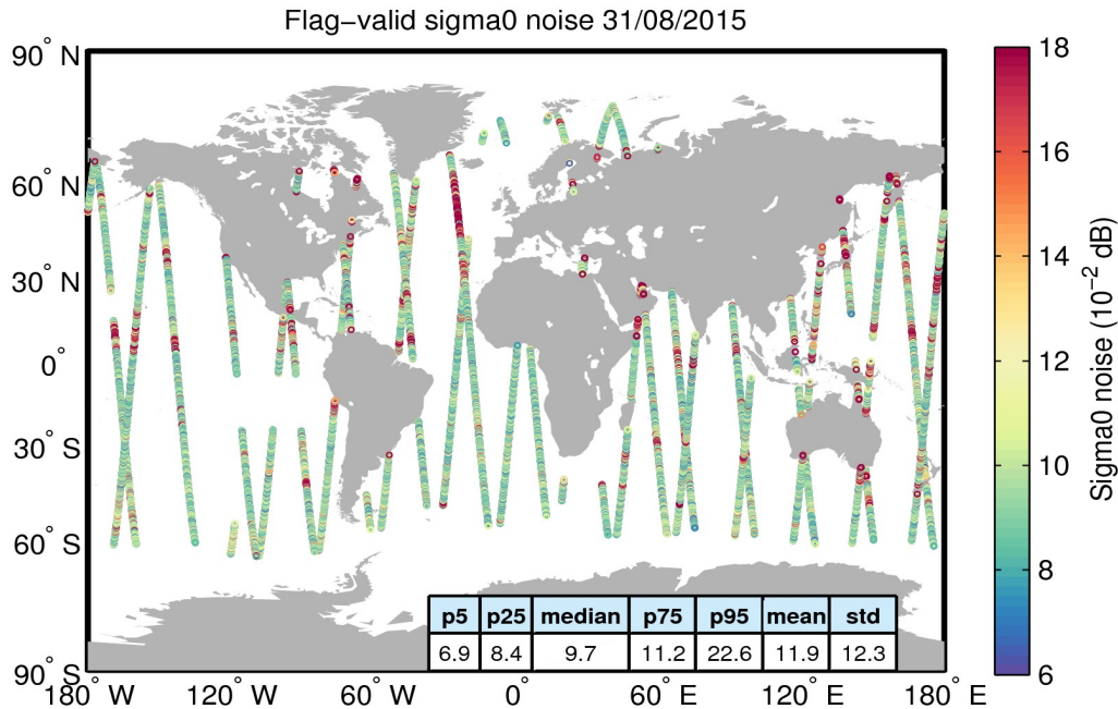
Figure 26. Geographical distribution of flag-valid 20-Hz sigma0 measurement noise over oceans and lakes for 31/08/2015. The statistical values shown in the table refer to the sigma0 noise and are calculated over all measurements shown in the figure.
