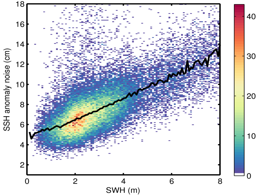
Figure 9. 2D histogram showing flag-valid SSH anomaly noise as a function of SWH for 31/08/2015. The black line denotes the median SSH anomaly as a function of SWH.
