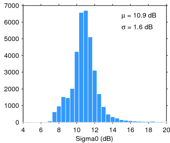
Figure 28. Histogram of science-valid sigma0 over oceans and lakes for 31/08/2015. The mean ( \mu ) and standard deviation ( \sigma ) are also shown. Note that values outside [4 20] dB are excluded from the histogram for the sake of readability but not from the computation of \mu and \sigma .
