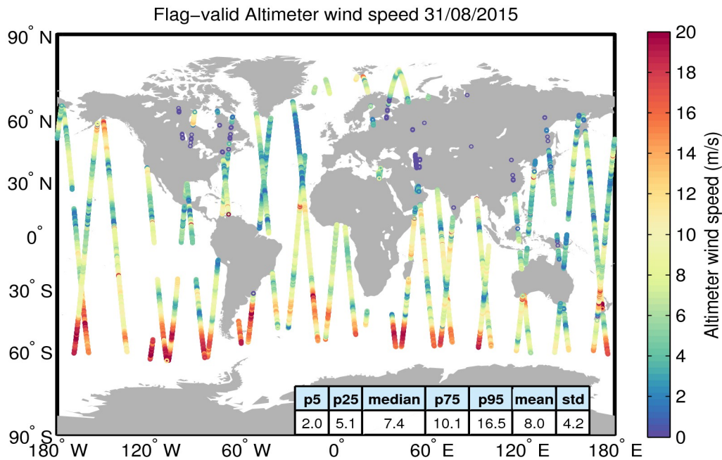
Figure 31. Geographical distribution of flag-valid wind data over oceans and lakes for 31/08/2015. The statistical values shown in the table refer to the wind in m/s and are calculated over all measurements shown in the figure.
