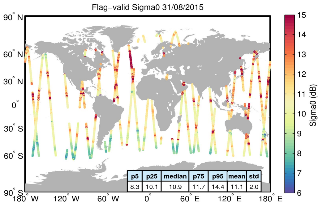
Figure 23. Geographical distribution of flag-valid sigma0 data over oceans and lakes for 31/08/2015. The statistical values shown in the table refer to the sigma0 in dB and are calculated over all measurements shown in the figure.
