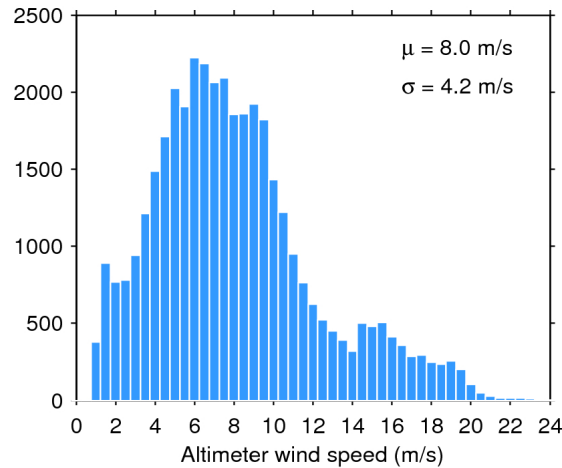
Figure 33. Histogram of flag-valid wind over oceans and lakes for 31/08/2015. The mean ( \mu ) and standard deviation ( \sigma ) are also shown. Note that values larger than 24 m/s are excluded from the histogram for the sake of readability but not from the computation of \mu and \sigma .
