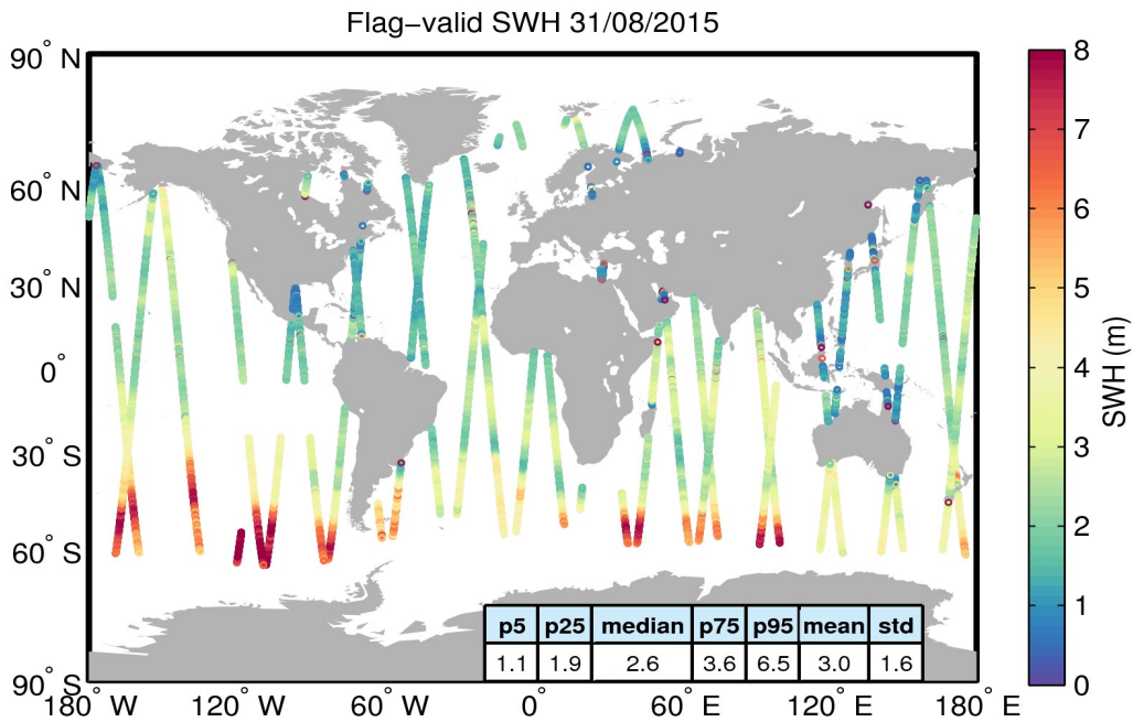
Figure 15. Geographical distribution of flag-valid SWH data over oceans and lakes for 31/08/2015. The statistical values shown in the table refer to the SWH in m and are calculated over all measurements shown in the figure.
