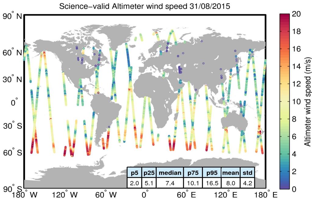
Figure 34. Geographical distribution of science-valid wind data over oceans and lakes for 31/08/2015. The statistical values shown in the table refer to the wind in m/s and are calculated over all measurements shown in the figure. Gray circles denote records that have been rejected based on the editing criteria described in Table 5.
