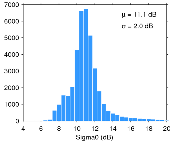
Figure 25. Histogram of flag-valid sigma0 over oceans and lakes for 31/08/2015. The mean ( \mu ) and standard deviation ( \sigma ) are also shown. Note that values outside [4 20] dB are excluded from the histogram for the sake of readability but not from the computation of \mu and \sigma .
