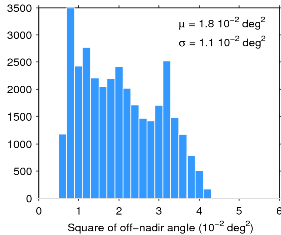
Figure 39. Histogram of flag-valid mispointing over oceans and lakes for 31/08/2015. The mean ( \mu ) and standard deviation ( \sigma ) are also shown. Note that values larger than 6 \cdot 10^{-2} \text{ deg}^2 are excluded from the histogram for the sake of readability but not from the computation of \mu and \sigma .
