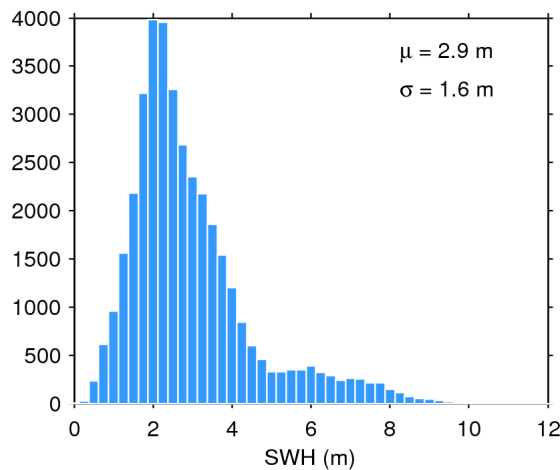
Figure 20. Histogram of science-valid SWH over oceans and lakes for 31/08/2015. The mean ( \mu ) and standard deviation ( \sigma ) are also shown. Note that values larger than 12 m are excluded from the histogram for the sake of readability but not from the computation of \mu and \sigma .
