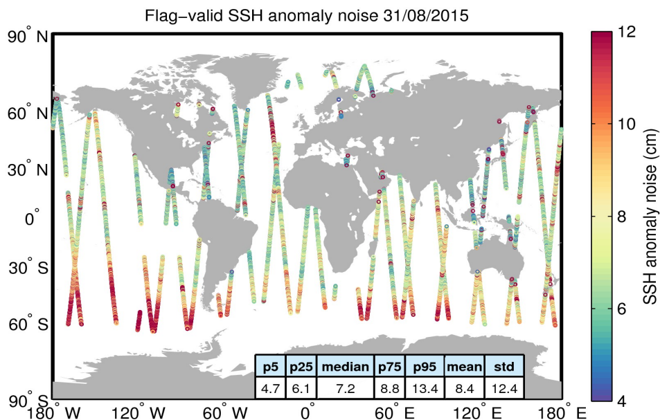
Figure 8. Geographical distribution of flag-valid 20-Hz SSH anomaly measurement noise over oceans and lakes for 31/08/2015. The statistical values shown in the table refer to the SSH anomaly noise and are calculated over all measurements shown in the figure.
