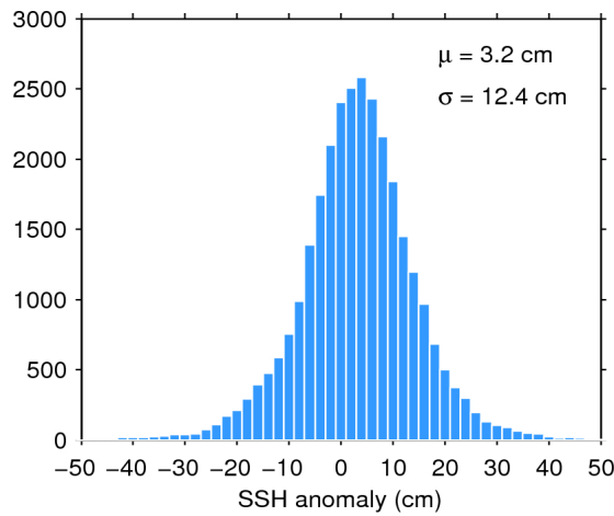
Figure 11. Histogram of science-valid SSH anomaly over oceans and lakes for 31/08/2015. The mean ( \mu ) and standard deviation ( \sigma ) are also shown. Note that values outside [-50 50] cm are excluded from the histogram for the sake of readability but not from the computation of \mu and \sigma .
