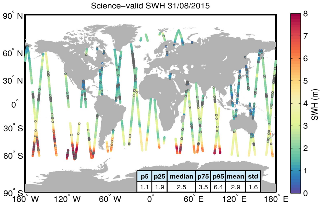
Figure 19. Geographical distribution of science-valid SWH data over oceans and lakes for 31/08/2015. The statistical values shown in the table refer to the SWH in m and are calculated over all measurements shown in the figure. Gray circles denote records that have been rejected based on the editing criteria described in Table 3.
