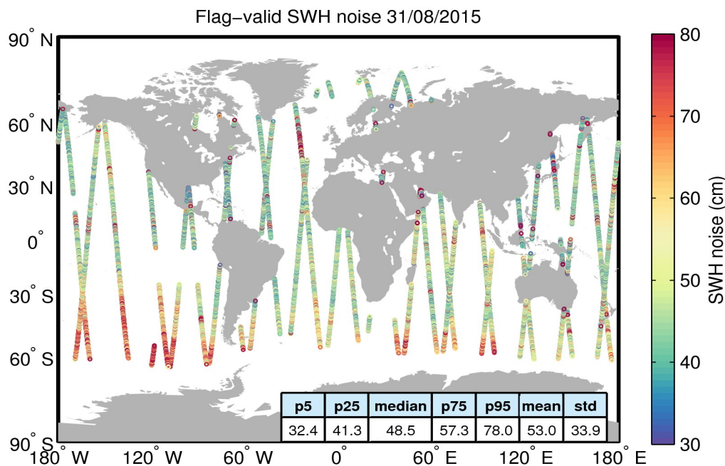
Figure 18. Geographical distribution of flag-valid 20-Hz SWH measurement noise over oceans and lakes for 31/08/2015. The statistical values shown in the table refer to the SWH noise and are calculated over all measurements shown in the figure.
