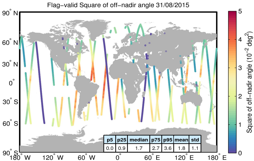
Figure 37. Geographical distribution of flag-valid mispointing data over oceans and lakes for 31/08/2015. The statistical values shown in the table refer to the mispointing in 10^{-2} \text{deg}^2 and are calculated over all measurements shown in the figure.
