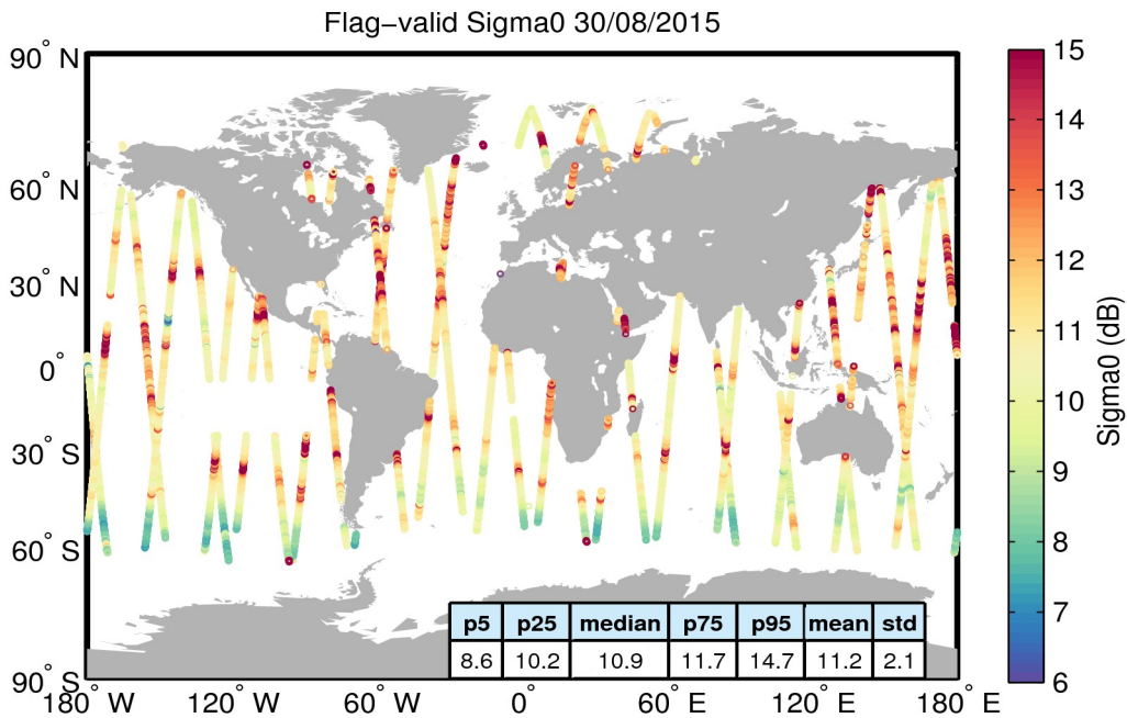
Figure 23. Geographical distribution of flag-valid sigma0 data over oceans and lakes for 30/08/2015. The statistical values shown in the table refer to the sigma0 in dB and are calculated over all measurements shown in the figure.
