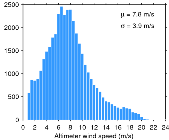
Figure 33. Histogram of flag-valid wind over oceans and lakes for 30/08/2015. The mean ( \mu ) and standard deviation ( \sigma ) are also shown. Note that values larger than 24 m/s are excluded from the histogram for the sake of readability but not from the computation of \mu and \sigma .
