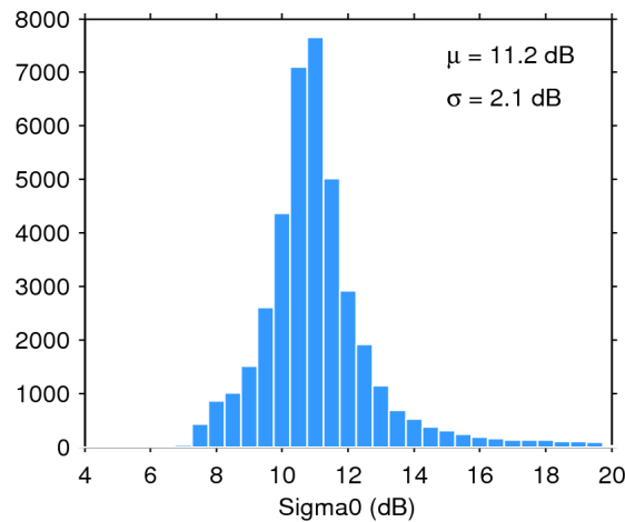
Figure 25. Histogram of flag-valid sigma0 over oceans and lakes for 30/08/2015. The mean ( \mu ) and standard deviation ( \sigma ) are also shown. Note that values outside [4 20] dB are excluded from the histogram for the sake of readability but not from the computation of \mu and \sigma .
