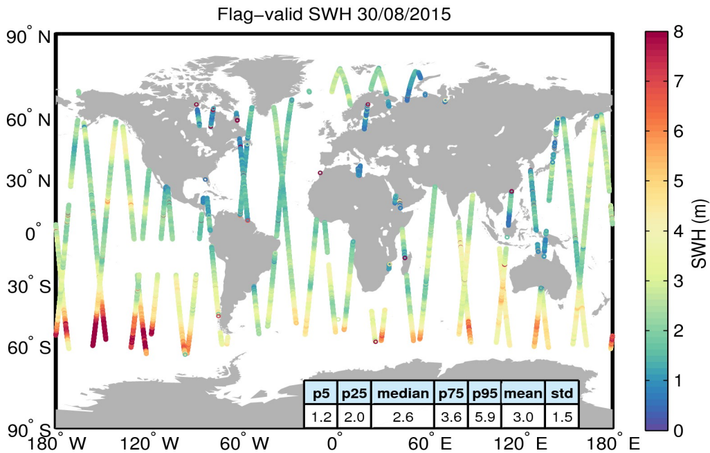
Figure 15. Geographical distribution of flag-valid SWH data over oceans and lakes for 30/08/2015. The statistical values shown in the table refer to the SWH in m and are calculated over all measurements shown in the figure.
