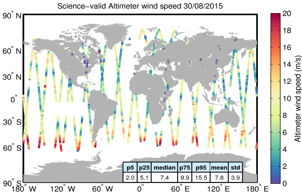
Figure 34. Geographical distribution of science-valid wind data over oceans and lakes for 30/08/2015. The statistical values shown in the table refer to the wind in m/s and are calculated over all measurements shown in the figure. Gray circles denote records that have been rejected based on the editing criteria described in Table 5.
