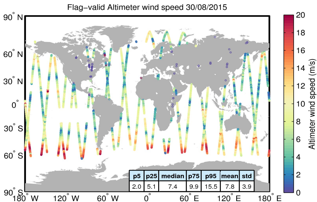
Figure 31. Geographical distribution of flag-valid wind data over oceans and lakes for 30/08/2015. The statistical values shown in the table refer to the wind in m/s and are calculated over all measurements shown in the figure.
