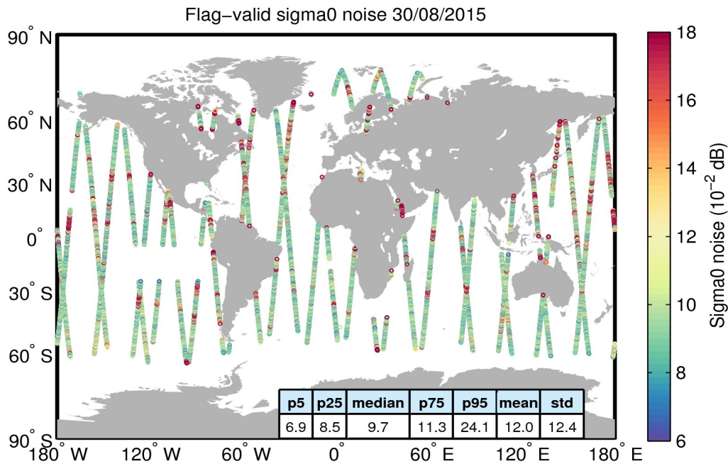
Figure 26. Geographical distribution of flag-valid 20-Hz sigma0 measurement noise over oceans and lakes for 30/08/2015. The statistical values shown in the table refer to the sigma0 noise and are calculated over all measurements shown in the figure.
