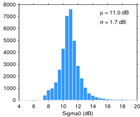
Figure 28. Histogram of science-valid sigma0 over oceans and lakes for 30/08/2015. The mean ( \mu ) and standard deviation ( \sigma ) are also shown. Note that values outside [4 20] dB are excluded from the histogram for the sake of readability but not from the computation of \mu and \sigma .
