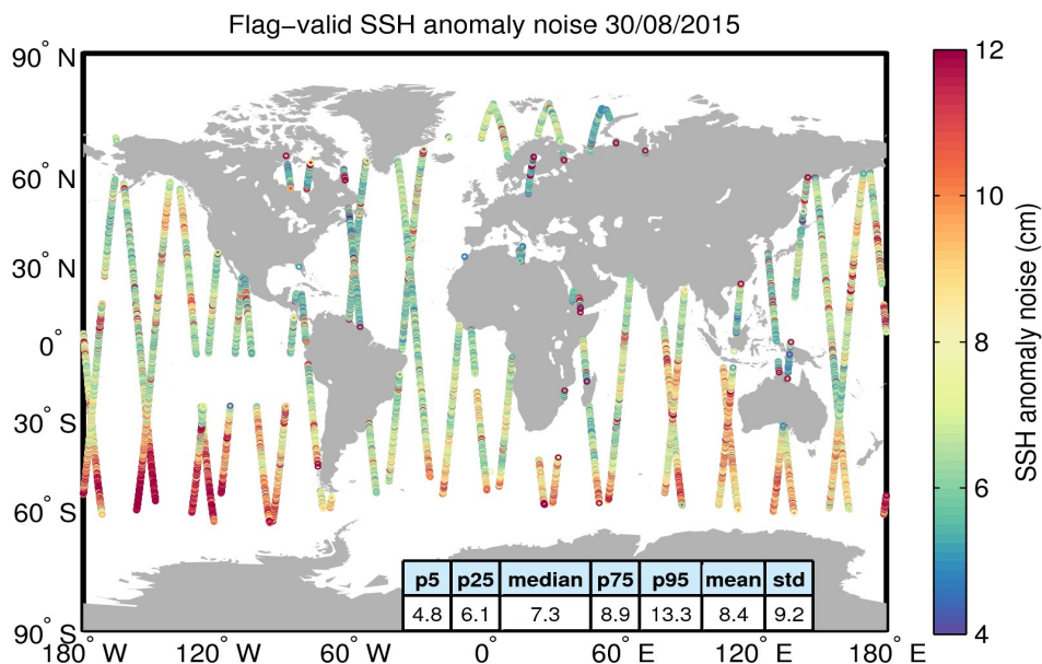
Figure 8. Geographical distribution of flag-valid 20-Hz SSH anomaly measurement noise over oceans and lakes for 30/08/2015. The statistical values shown in the table refer to the SSH anomaly noise and are calculated over all measurements shown in the figure.
