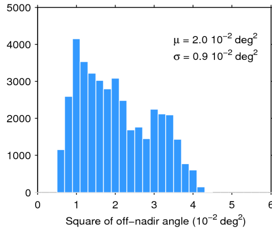
Figure 39. Histogram of flag-valid mispointing over oceans and lakes for 30/08/2015. The mean ( \mu ) and standard deviation ( \sigma ) are also shown. Note that values larger than 6 \cdot 10^{-2} \text{ deg}^2 are excluded from the histogram for the sake of readability but not from the computation of \mu and \sigma .
