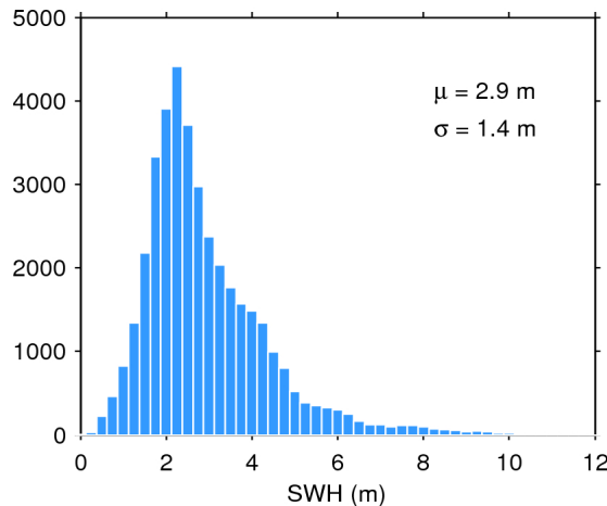
Figure 20. Histogram of science-valid SWH over oceans and lakes for 30/08/2015. The mean ( \mu ) and standard deviation ( \sigma ) are also shown. Note that values larger than 12 m are excluded from the histogram for the sake of readability but not from the computation of \mu and \sigma .
