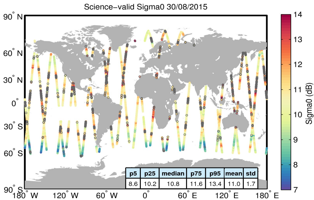
Figure 27. Geographical distribution of science-valid sigma0 data over oceans and lakes for 30/08/2015. The statistical values shown in the table refer to the sigma0 in dB and are calculated over all measurements shown in the figure. Gray circles denote records that have been rejected based on the editing criteria described in Table 4.
