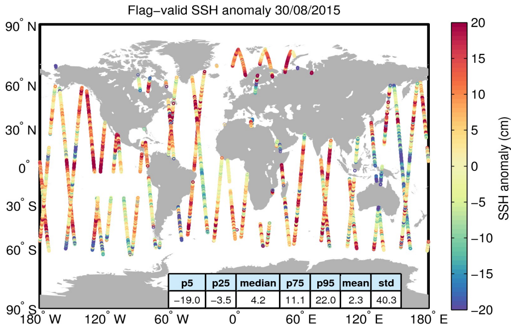
Figure 5. Geographical distribution of flag-valid 1-Hz SSH anomaly data over oceans and lakes for 30/08/2015. The statistical values shown in the table refer to the SSH anomaly in cm and are calculated over all measurements shown in the figure.
