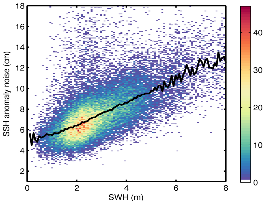
Figure 9. 2D histogram showing flag-valid SSH anomaly noise as a function of SWH for 30/08/2015. The black line denotes the median SSH anomaly as a function of SWH.
