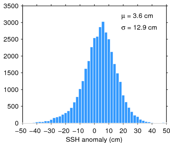
Figure 11. Histogram of science-valid SSH anomaly over oceans and lakes for 30/08/2015. The mean ( \mu ) and standard deviation ( \sigma ) are also shown. Note that values outside [-50 50] cm are excluded from the histogram for the sake of readability but not from the computation of \mu and \sigma .
