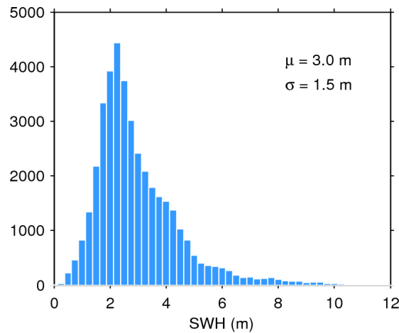
Figure 17. Histogram of flag-valid SWH over oceans and lakes for 30/08/2015. The mean ( \mu ) and standard deviation ( \sigma ) are also shown. Note that values larger than 12 m are excluded from the histogram for the sake of readability but not from the computation of \mu and \sigma .
