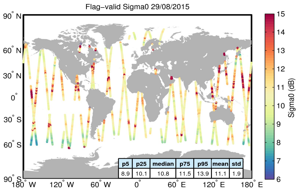
Figure 23. Geographical distribution of flag-valid sigma0 data over oceans and lakes for 29/08/2015. The statistical values shown in the table refer to the sigma0 in dB and are calculated over all measurements shown in the figure.
