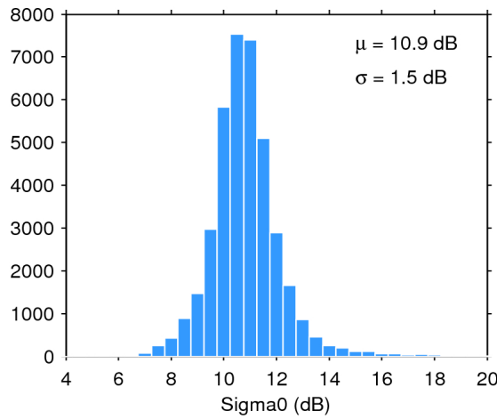
Figure 28. Histogram of science-valid sigma0 over oceans and lakes for 29/08/2015. The mean ( \mu ) and standard deviation ( \sigma ) are also shown. Note that values outside [4 20] dB are excluded from the histogram for the sake of readability but not from the computation of \mu and \sigma .
