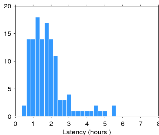
Figure 2. Histogram of the data latency for 29/08/2015. The y-axis denotes the number of files that are made available with a delay of x-hours with respect to the mean time of the records stored in the file.
