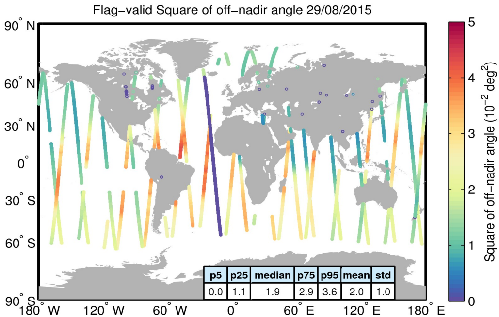
Figure 37. Geographical distribution of flag-valid mispointing data over oceans and lakes for 29/08/2015. The statistical values shown in the table refer to the mispointing in 10^{-2} \text{deg}^2 and are calculated over all measurements shown in the figure.
