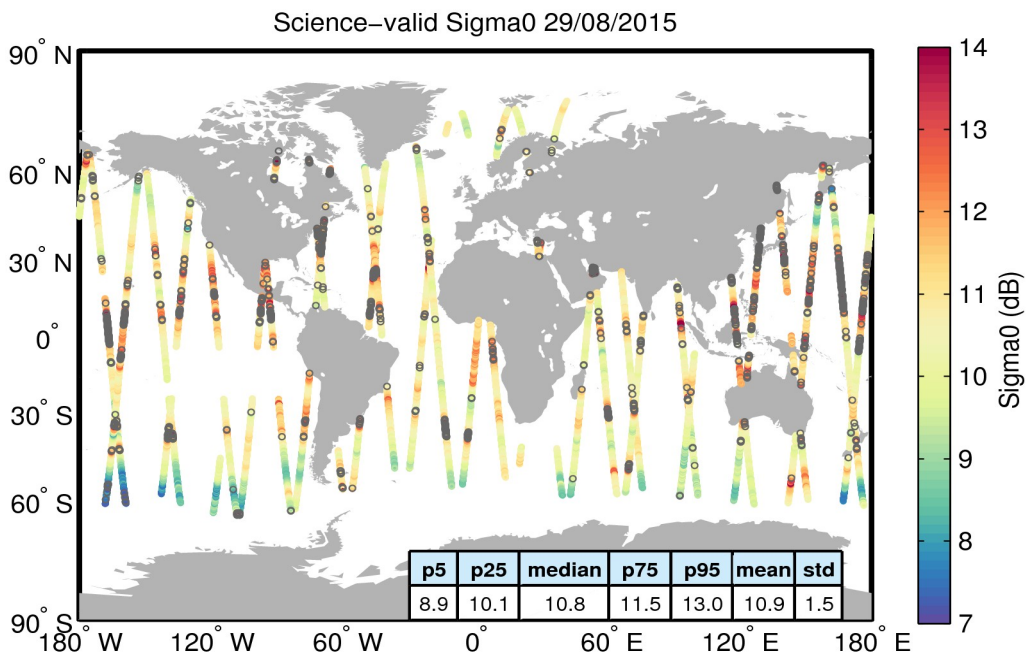
Figure 27. Geographical distribution of science-valid sigma0 data over oceans and lakes for 29/08/2015. The statistical values shown in the table refer to the sigma0 in dB and are calculated over all measurements shown in the figure. Gray circles denote records that have been rejected based on the editing criteria described in Table 4.
