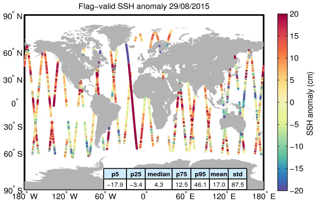
Figure 5. Geographical distribution of flag-valid 1-Hz SSH anomaly data over oceans and lakes for 29/08/2015. The statistical values shown in the table refer to the SSH anomaly in cm and are calculated over all measurements shown in the figure.
