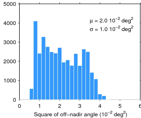
Figure 39. Histogram of flag-valid mispointing over oceans and lakes for 29/08/2015. The mean ( \mu ) and standard deviation ( \sigma ) are also shown. Note that values larger than 6 \cdot 10^{-2} \text{ deg}^2 are excluded from the histogram for the sake of readability but not from the computation of \mu and \sigma .
