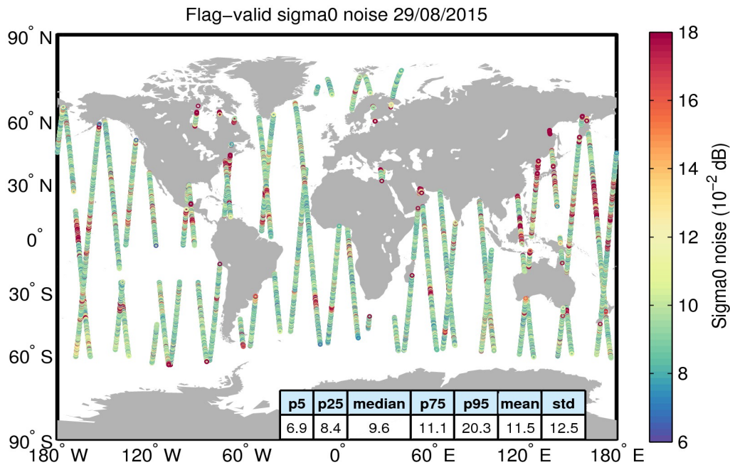
Figure 26. Geographical distribution of flag-valid 20-Hz sigma0 measurement noise over oceans and lakes for 29/08/2015. The statistical values shown in the table refer to the sigma0 noise and are calculated over all measurements shown in the figure.
