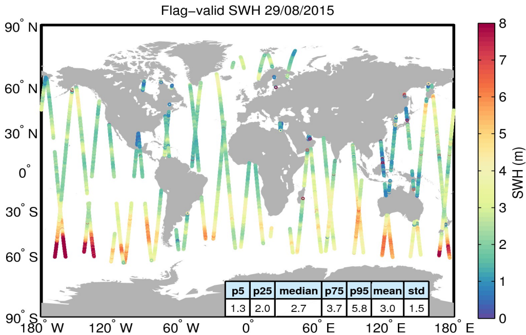
Figure 15. Geographical distribution of flag-valid SWH data over oceans and lakes for 29/08/2015. The statistical values shown in the table refer to the SWH in m and are calculated over all measurements shown in the figure.
