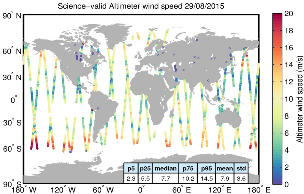
Figure 34. Geographical distribution of science-valid wind data over oceans and lakes for 29/08/2015. The statistical values shown in the table refer to the wind in m/s and are calculated over all measurements shown in the figure. Gray circles denote records that have been rejected based on the editing criteria described in Table 5.
