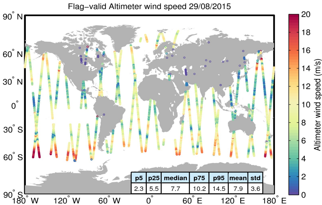
Figure 31. Geographical distribution of flag-valid wind data over oceans and lakes for 29/08/2015. The statistical values shown in the table refer to the wind in m/s and are calculated over all measurements shown in the figure.
