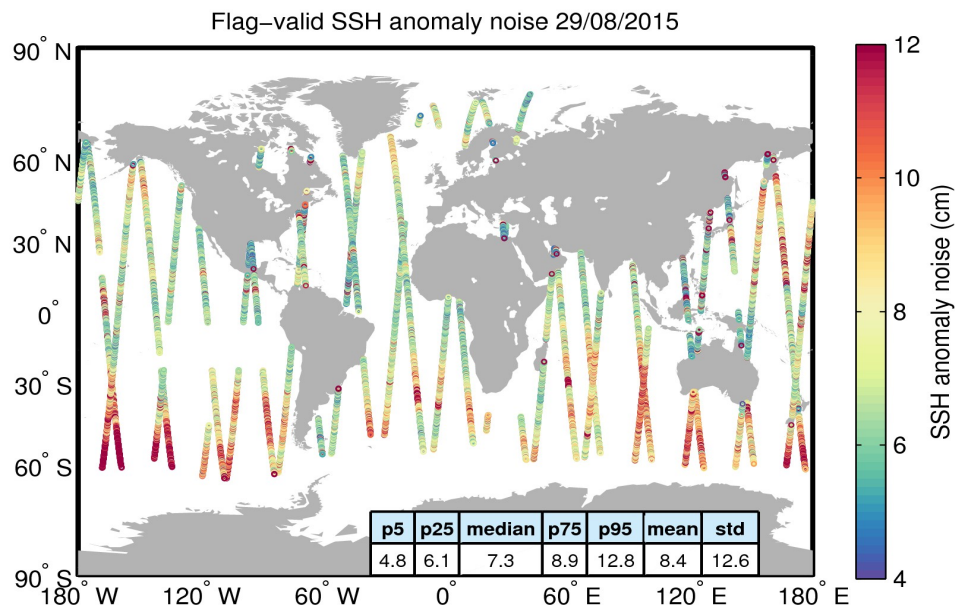
Figure 8. Geographical distribution of flag-valid 20-Hz SSH anomaly measurement noise over oceans and lakes for 29/08/2015. The statistical values shown in the table refer to the SSH anomaly noise and are calculated over all measurements shown in the figure.
