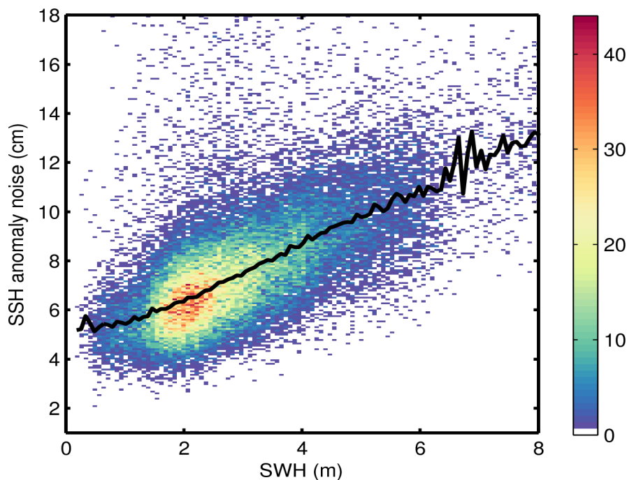
Figure 9. 2D histogram showing flag-valid SSH anomaly noise as a function of SWH for 29/08/2015. The black line denotes the median SSH anomaly as a function of SWH.
