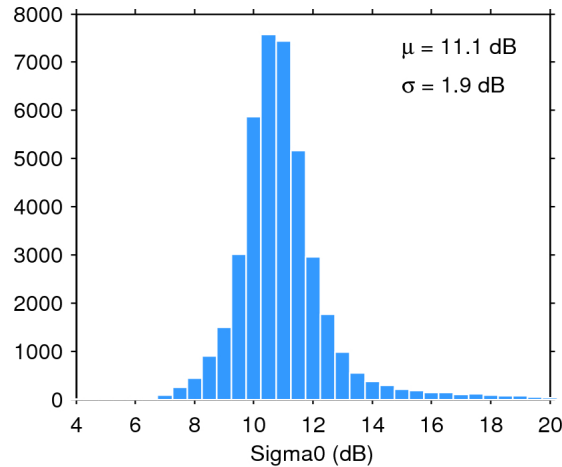
Figure 25. Histogram of flag-valid sigma0 over oceans and lakes for 29/08/2015. The mean ( \mu ) and standard deviation ( \sigma ) are also shown. Note that values outside [4 20] dB are excluded from the histogram for the sake of readability but not from the computation of \mu and \sigma .
