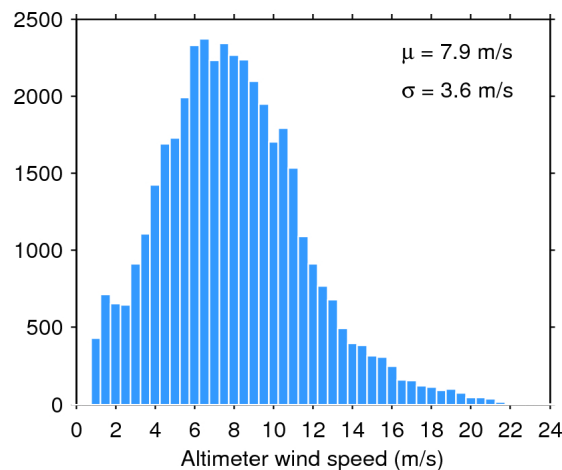
Figure 35. Histogram of science-valid wind over oceans and lakes for 29/08/2015. The mean ( \mu ) and standard deviation ( \sigma ) are also shown. Note that values larger than 24 m/s are excluded from the histogram for the sake of readability but not from the computation of \mu and \sigma .
