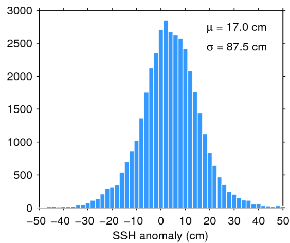
Figure 7. Histogram of flag-valid SSH anomaly over oceans and lakes for 29/08/2015. The mean ( \mu ) and standard deviation ( \sigma ) are also shown. Note that values outside [-50 50] cm are excluded from the histogram for the sake of readability but not from the computation of \mu and \sigma .
