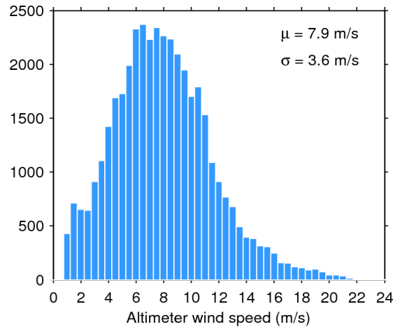
Figure 33. Histogram of flag-valid wind over oceans and lakes for 29/08/2015. The mean ( \mu ) and standard deviation ( \sigma ) are also shown. Note that values larger than 24 m/s are excluded from the histogram for the sake of readability but not from the computation of \mu and \sigma .
