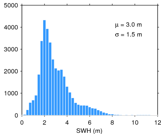
Figure 20. Histogram of science-valid SWH over oceans and lakes for 28/08/2015. The mean ( \mu ) and standard deviation ( \sigma ) are also shown. Note that values larger than 12 m are excluded from the histogram for the sake of readability but not from the computation of \mu and \sigma .
