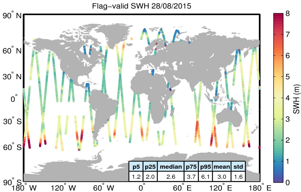
Figure 15. Geographical distribution of flag-valid SWH data over oceans and lakes for 28/08/2015. The statistical values shown in the table refer to the SWH in m and are calculated over all measurements shown in the figure.
