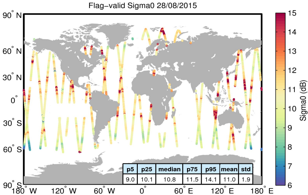
Figure 23. Geographical distribution of flag-valid sigma0 data over oceans and lakes for 28/08/2015. The statistical values shown in the table refer to the sigma0 in dB and are calculated over all measurements shown in the figure.
