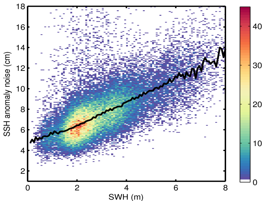
Figure 9. 2D histogram showing flag-valid SSH anomaly noise as a function of SWH for 28/08/2015. The black line denotes the median SSH anomaly as a function of SWH.
