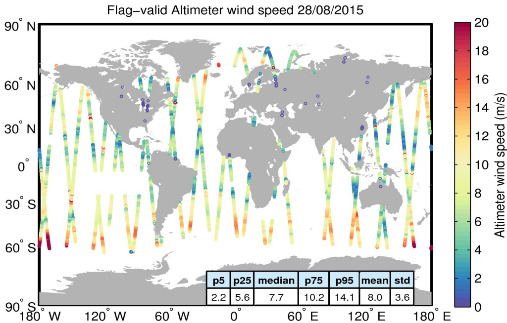
Figure 31. Geographical distribution of flag-valid wind data over oceans and lakes for 28/08/2015. The statistical values shown in the table refer to the wind in m/s and are calculated over all measurements shown in the figure.
