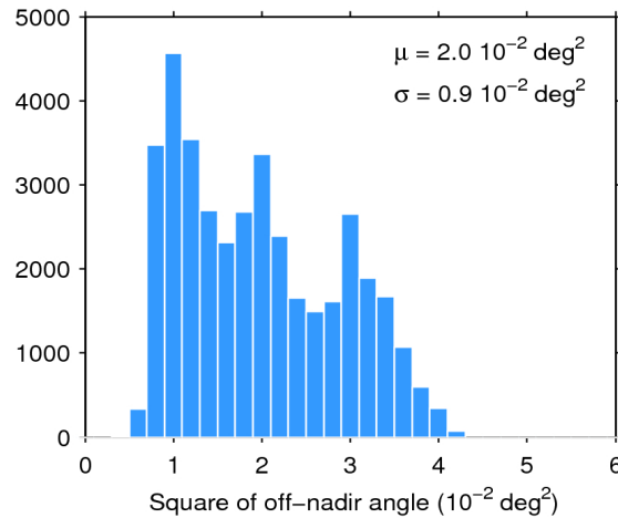
Figure 39. Histogram of flag-valid mispointing over oceans and lakes for 28/08/2015. The mean ( \mu ) and standard deviation ( \sigma ) are also shown. Note that values larger than 6 \cdot 10^{-2} \text{ deg}^2 are excluded from the histogram for the sake of readability but not from the computation of \mu and \sigma .
