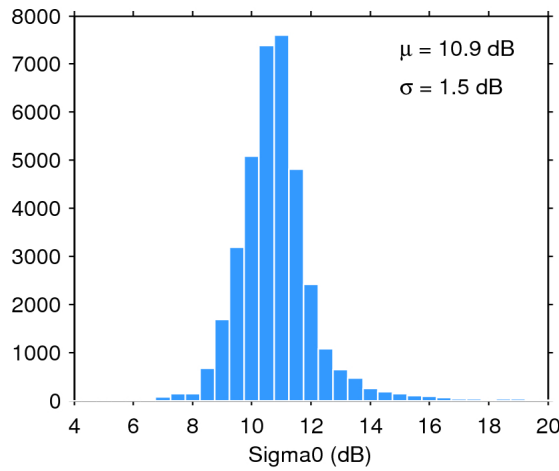
Figure 28. Histogram of science-valid sigma0 over oceans and lakes for 28/08/2015. The mean ( \mu ) and standard deviation ( \sigma ) are also shown. Note that values outside [4 20] dB are excluded from the histogram for the sake of readability but not from the computation of \mu and \sigma .
