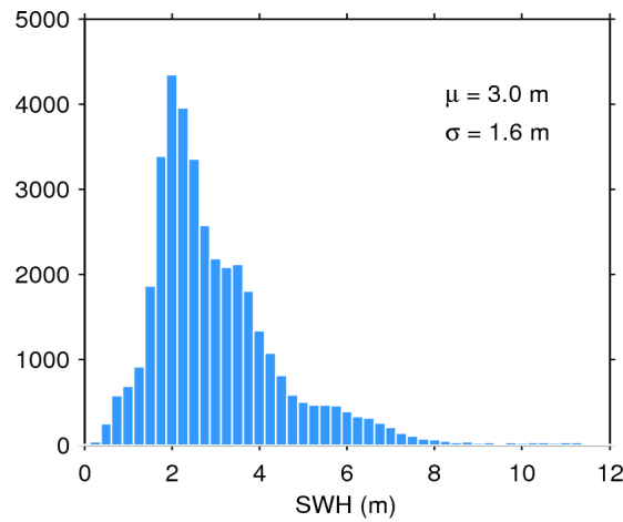
Figure 17. Histogram of flag-valid SWH over oceans and lakes for 28/08/2015. The mean ( \mu ) and standard deviation ( \sigma ) are also shown. Note that values larger than 12 m are excluded from the histogram for the sake of readability but not from the computation of \mu and \sigma .
