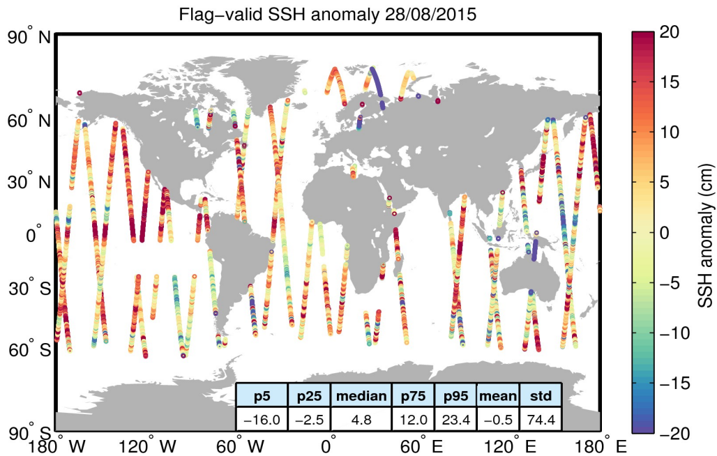
Figure 5. Geographical distribution of flag-valid 1-Hz SSH anomaly data over oceans and lakes for 28/08/2015. The statistical values shown in the table refer to the SSH anomaly in cm and are calculated over all measurements shown in the figure.
