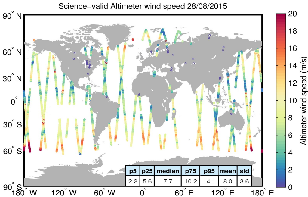
Figure 34. Geographical distribution of science-valid wind data over oceans and lakes for 28/08/2015. The statistical values shown in the table refer to the wind in m/s and are calculated over all measurements shown in the figure. Gray circles denote records that have been rejected based on the editing criteria described in Table 5.
