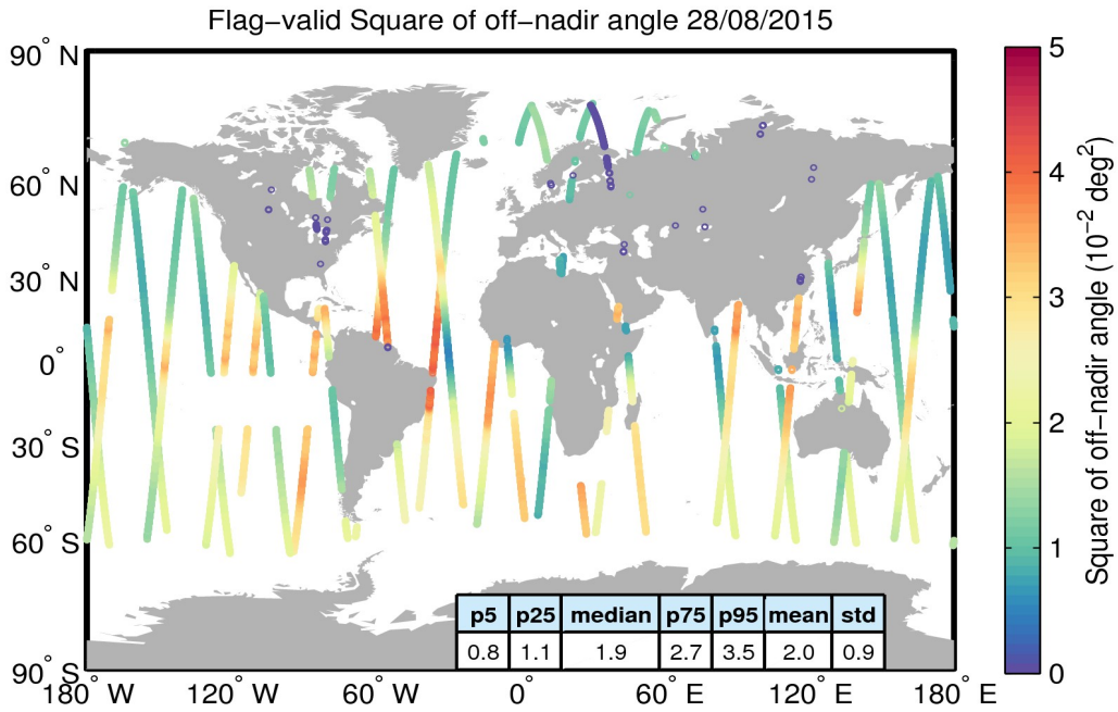
Figure 37. Geographical distribution of flag-valid mispointing data over oceans and lakes for 28/08/2015. The statistical values shown in the table refer to the mispointing in 10^{-2} \text{ deg}^2 and are calculated over all measurements shown in the figure.
