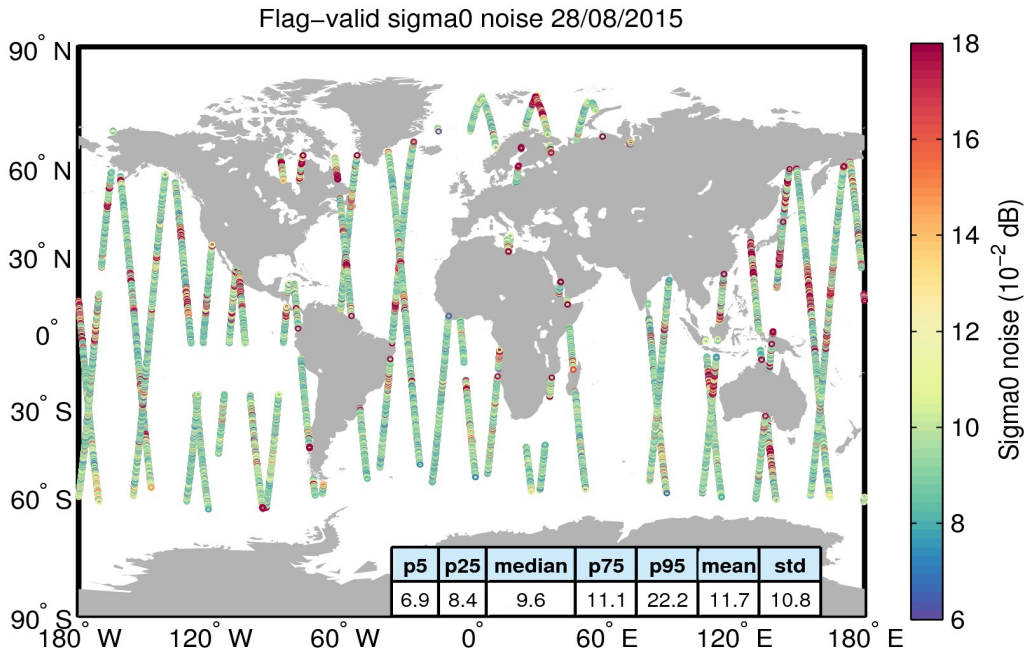
Figure 26. Geographical distribution of flag-valid 20-Hz sigma0 measurement noise over oceans and lakes for 28/08/2015. The statistical values shown in the table refer to the sigma0 noise and are calculated over all measurements shown in the figure.
