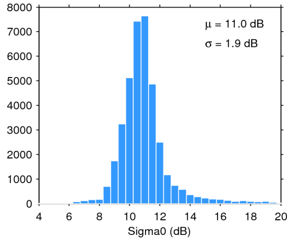
Figure 25. Histogram of flag-valid sigma0 over oceans and lakes for 28/08/2015. The mean ( \mu ) and standard deviation ( \sigma ) are also shown. Note that values outside [4 20] dB are excluded from the histogram for the sake of readability but not from the computation of \mu and \sigma .
