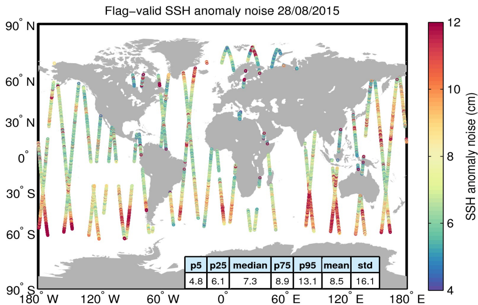
Figure 8. Geographical distribution of flag-valid 20-Hz SSH anomaly measurement noise over oceans and lakes for 28/08/2015. The statistical values shown in the table refer to the SSH anomaly noise and are calculated over all measurements shown in the figure.
