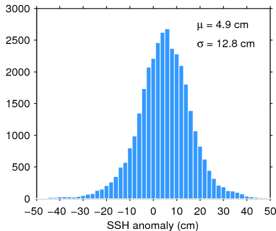
Figure 11. Histogram of science-valid SSH anomaly over oceans and lakes for 28/08/2015. The mean ( \mu ) and standard deviation ( \sigma ) are also shown. Note that values outside [-50 50] cm are excluded from the histogram for the sake of readability but not from the computation of \mu and \sigma .
