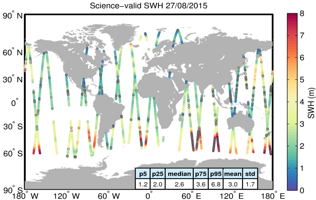
Figure 19. Geographical distribution of science-valid SWH data over oceans and lakes for 27/08/2015. The statistical values shown in the table refer to the SWH in m and are calculated over all measurements shown in the figure. Gray circles denote records that have been rejected based on the editing criteria described in Table 3.
