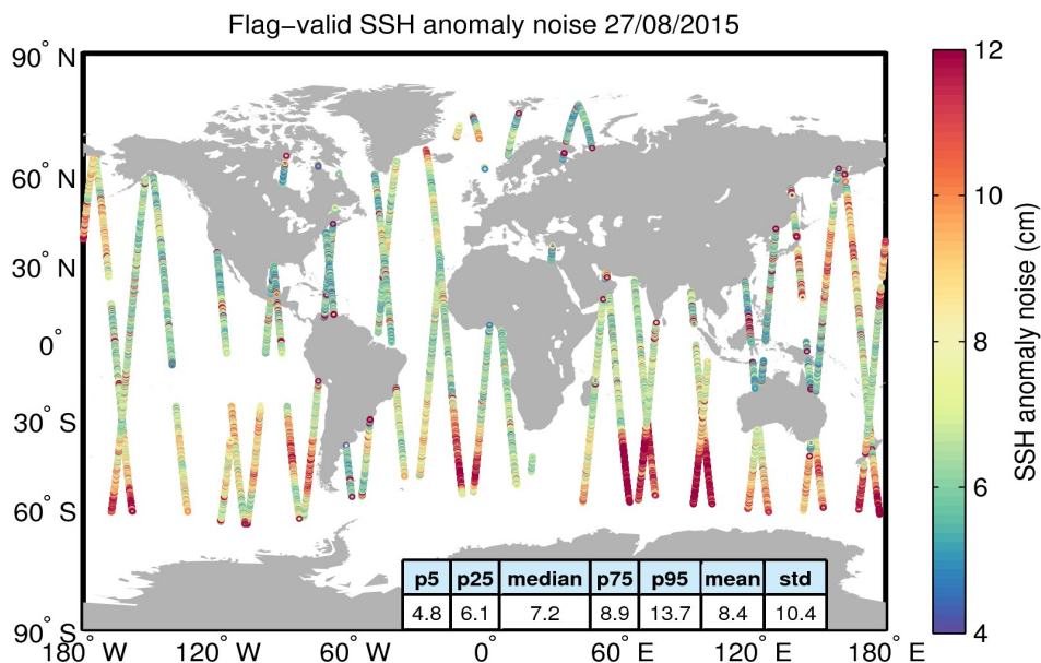
Figure 8. Geographical distribution of flag-valid 20-Hz SSH anomaly measurement noise over oceans and lakes for 27/08/2015. The statistical values shown in the table refer to the SSH anomaly noise and are calculated over all measurements shown in the figure.
