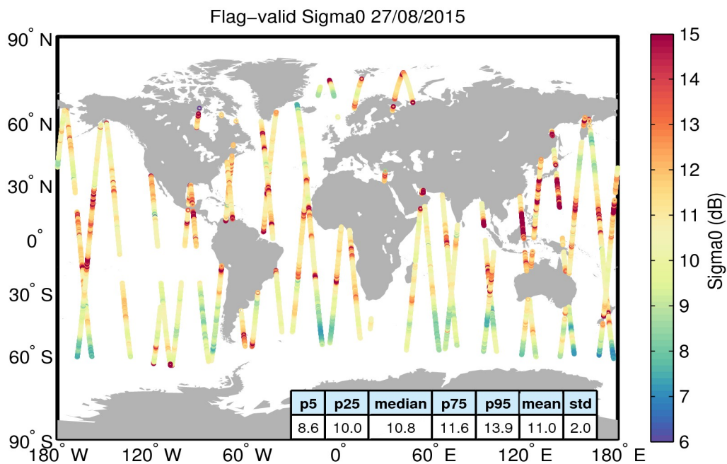
Figure 23. Geographical distribution of flag-valid sigma0 data over oceans and lakes for 27/08/2015. The statistical values shown in the table refer to the sigma0 in dB and are calculated over all measurements shown in the figure.
