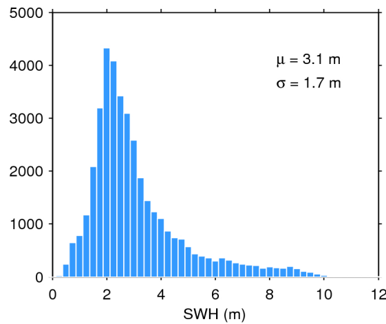
Figure 17. Histogram of flag-valid SWH over oceans and lakes for 27/08/2015. The mean ( \mu ) and standard deviation ( \sigma ) are also shown. Note that values larger than 12 m are excluded from the histogram for the sake of readability but not from the computation of \mu and \sigma .
