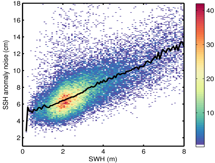
Figure 9. 2D histogram showing flag-valid SSH anomaly noise as a function of SWH for 27/08/2015. The black line denotes the median SSH anomaly as a function of SWH.
