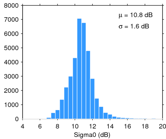
Figure 28. Histogram of science-valid sigma0 over oceans and lakes for 27/08/2015. The mean ( \mu ) and standard deviation ( \sigma ) are also shown. Note that values outside [4 20] dB are excluded from the histogram for the sake of readability but not from the computation of \mu and \sigma .
