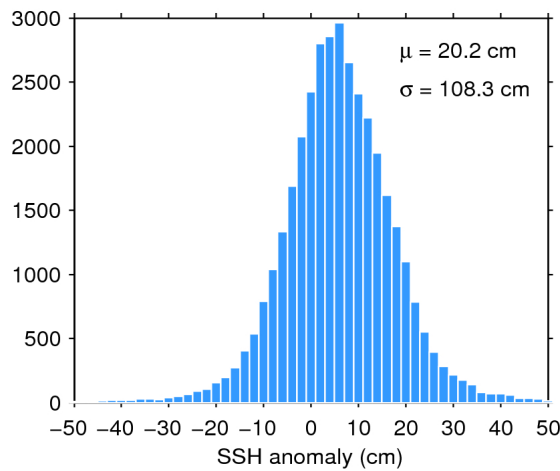
Figure 7. Histogram of flag-valid SSH anomaly over oceans and lakes for 27/08/2015. The mean ( \mu ) and standard deviation ( \sigma ) are also shown. Note that values outside [-50 50] cm are excluded from the histogram for the sake of readability but not from the computation of \mu and \sigma .
