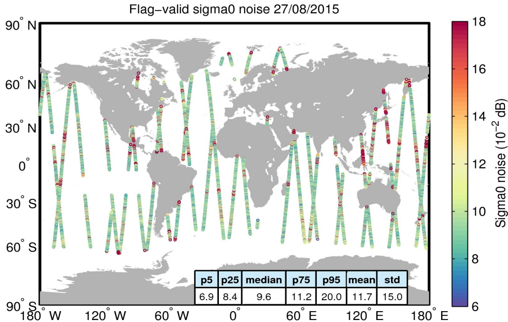
Figure 26. Geographical distribution of flag-valid 20-Hz sigma0 measurement noise over oceans and lakes for 27/08/2015. The statistical values shown in the table refer to the sigma0 noise and are calculated over all measurements shown in the figure.
