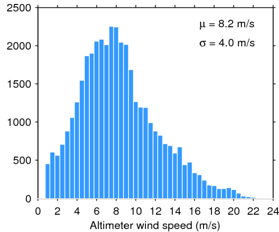
Figure 33. Histogram of flag-valid wind over oceans and lakes for 27/08/2015. The mean ( \mu ) and standard deviation ( \sigma ) are also shown. Note that values larger than 24 m/s are excluded from the histogram for the sake of readability but not from the computation of \mu and \sigma .
