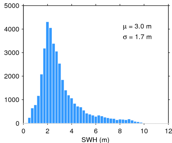
Figure 20. Histogram of science-valid SWH over oceans and lakes for 27/08/2015. The mean ( \mu ) and standard deviation ( \sigma ) are also shown. Note that values larger than 12 m are excluded from the histogram for the sake of readability but not from the computation of \mu and \sigma .
