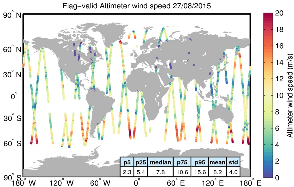
Figure 31. Geographical distribution of flag-valid wind data over oceans and lakes for 27/08/2015. The statistical values shown in the table refer to the wind in m/s and are calculated over all measurements shown in the figure.
