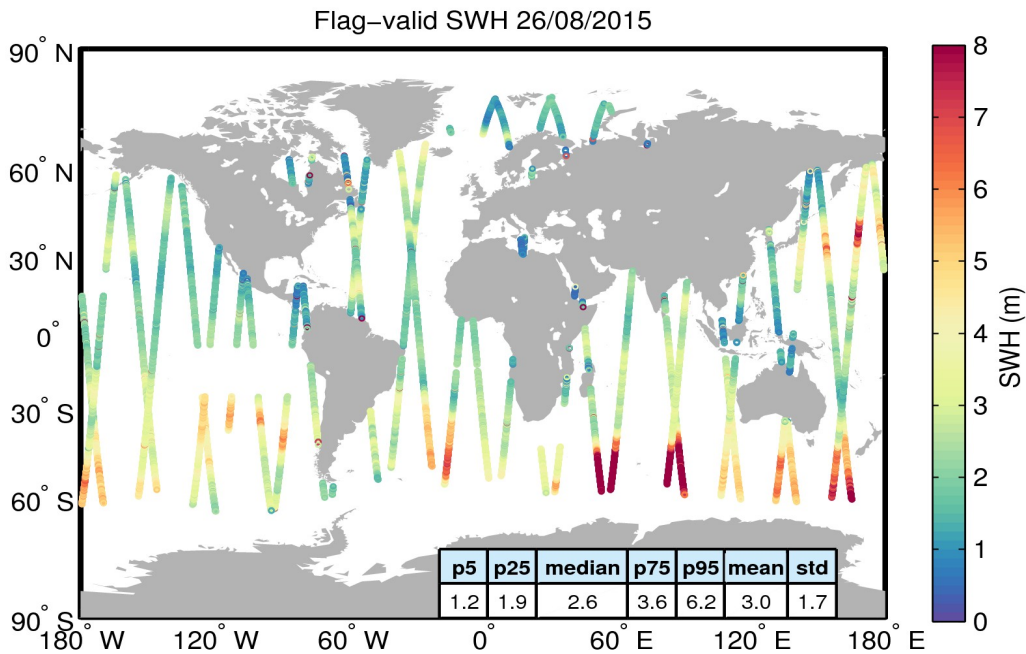
Figure 15. Geographical distribution of flag-valid SWH data over oceans and lakes for 26/08/2015. The statistical values shown in the table refer to the SWH in m and are calculated over all measurements shown in the figure.
