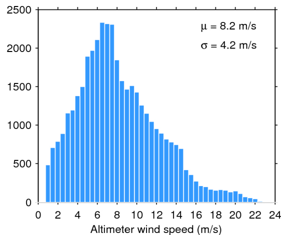
Figure 35. Histogram of science-valid wind over oceans and lakes for 26/08/2015. The mean ( \mu ) and standard deviation ( \sigma ) are also shown. Note that values larger than 24 m/s are excluded from the histogram for the sake of readability but not from the computation of \mu and \sigma .
