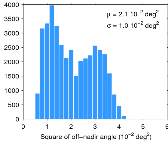
Figure 39. Histogram of flag-valid mispointing over oceans and lakes for 26/08/2015. The mean ( \mu ) and standard deviation ( \sigma ) are also shown. Note that values larger than 6 \cdot 10^{-2} \text{ deg}^2 are excluded from the histogram for the sake of readability but not from the computation of \mu and \sigma .
