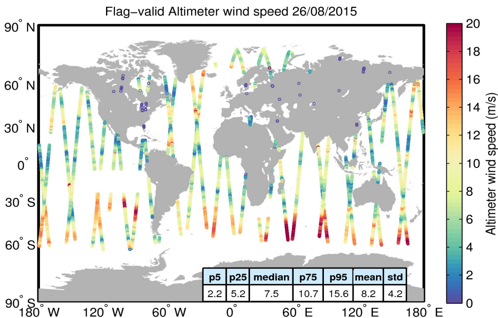
Figure 31. Geographical distribution of flag-valid wind data over oceans and lakes for 26/08/2015. The statistical values shown in the table refer to the wind in m/s and are calculated over all measurements shown in the figure.
