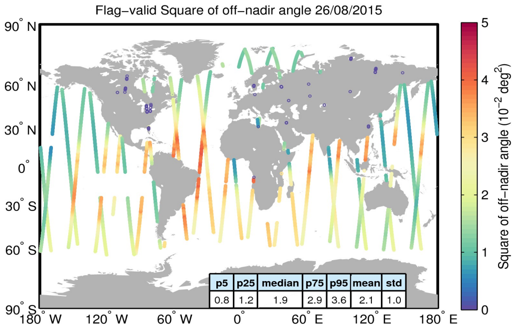
Figure 37. Geographical distribution of flag-valid mispointing data over oceans and lakes for 26/08/2015. The statistical values shown in the table refer to the mispointing in 10^{-2} deg 2 and are calculated over all measurements shown in the figure.
