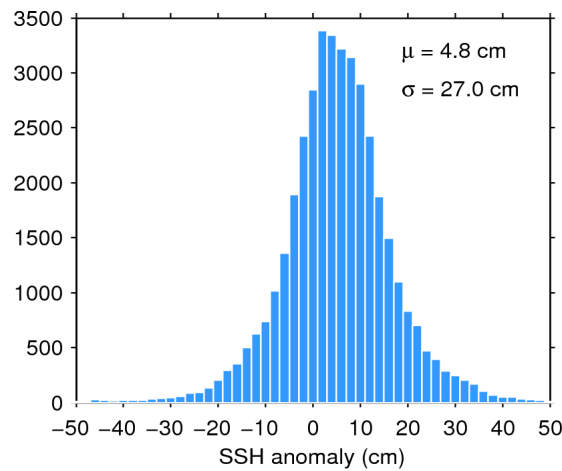
Figure 7. Histogram of flag-valid SSH anomaly over oceans and lakes for 26/08/2015. The mean ( \mu ) and standard deviation ( \sigma ) are also shown. Note that values outside [-50\ 50] cm are excluded from the histogram for the sake of readability but not from the computation of \mu and \sigma .
