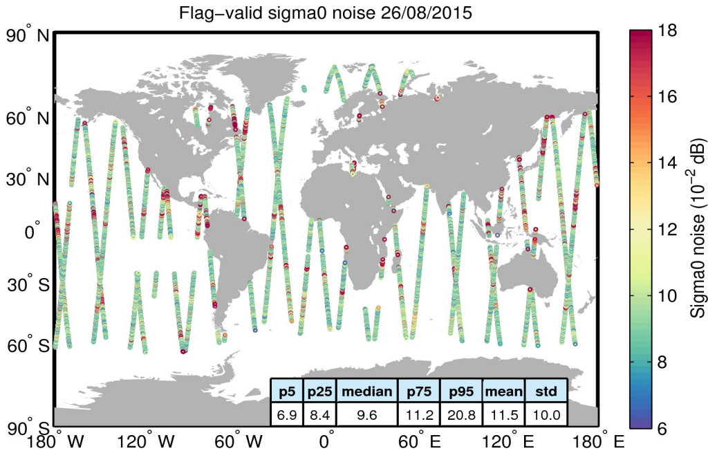
Figure 26. Geographical distribution of flag-valid 20-Hz sigma0 measurement noise over oceans and lakes for 26/08/2015. The statistical values shown in the table refer to the sigma0 noise and are calculated over all measurements shown in the figure.
