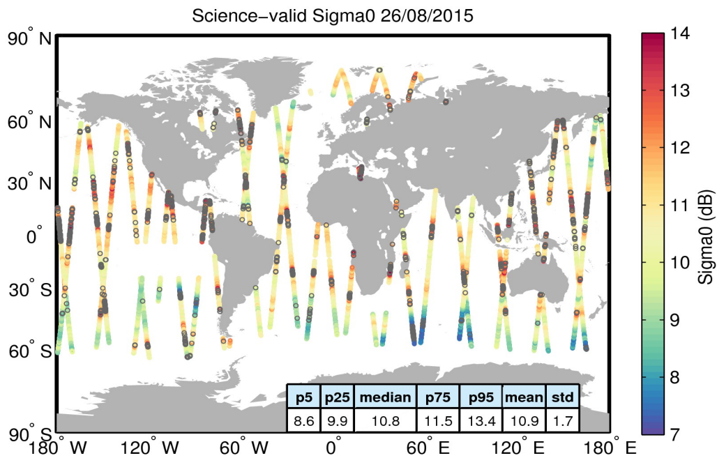
Figure 27. Geographical distribution of science-valid sigma0 data over oceans and lakes for 26/08/2015. The statistical values shown in the table refer to the sigma0 in dB and are calculated over all measurements shown in the figure. Gray circles denote records that have been rejected based on the editing criteria described in Table 4.
