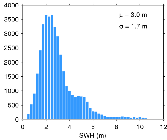
Figure 17. Histogram of flag-valid SWH over oceans and lakes for 26/08/2015. The mean ( \mu ) and standard deviation ( \sigma ) are also shown. Note that values larger than 12 m are excluded from the histogram for the sake of readability but not from the computation of \mu and \sigma .
