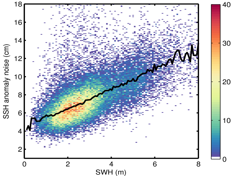
Figure 9. 2D histogram showing flag-valid SSH anomaly noise as a function of SWH for 26/08/2015. The black line denotes the median SSH anomaly as a function of SWH.
