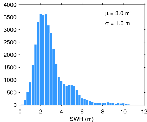
Figure 20. Histogram of science-valid SWH over oceans and lakes for 26/08/2015. The mean ( \mu ) and standard deviation ( \sigma ) are also shown. Note that values larger than 12 m are excluded from the histogram for the sake of readability but not from the computation of \mu and \sigma .
