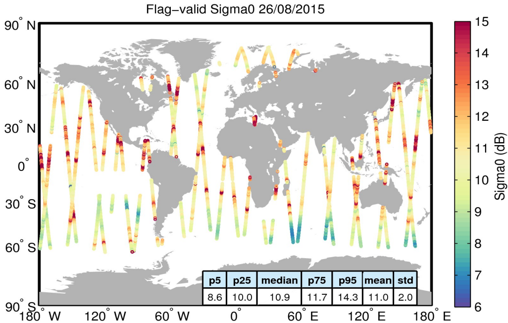
Figure 23. Geographical distribution of flag-valid sigma0 data over oceans and lakes for 26/08/2015. The statistical values shown in the table refer to the sigma0 in dB and are calculated over all measurements shown in the figure.
