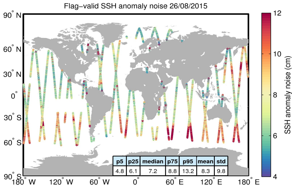
Figure 8. Geographical distribution of flag-valid 20-Hz SSH anomaly measurement noise over oceans and lakes for 26/08/2015. The statistical values shown in the table refer to the SSH anomaly noise and are calculated over all measurements shown in the figure.
