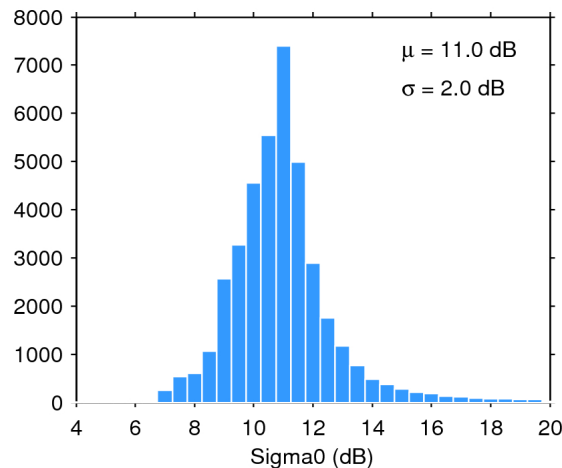
Figure 25. Histogram of flag-valid sigma0 over oceans and lakes for 26/08/2015. The mean ( \mu ) and standard deviation ( \sigma ) are also shown. Note that values outside [4 20] dB are excluded from the histogram for the sake of readability but not from the computation of \mu and \sigma .
