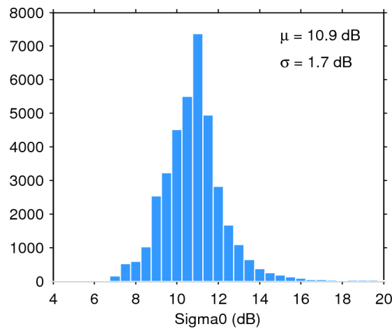
Figure 28. Histogram of science-valid sigma0 over oceans and lakes for 26/08/2015. The mean ( \mu ) and standard deviation ( \sigma ) are also shown. Note that values outside [4 20] dB are excluded from the histogram for the sake of readability but not from the computation of \mu and \sigma .
