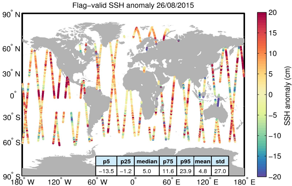
Figure 5. Geographical distribution of flag-valid 1-Hz SSH anomaly data over oceans and lakes for 26/08/2015. The statistical values shown in the table refer to the SSH anomaly in cm and are calculated over all measurements shown in the figure.
