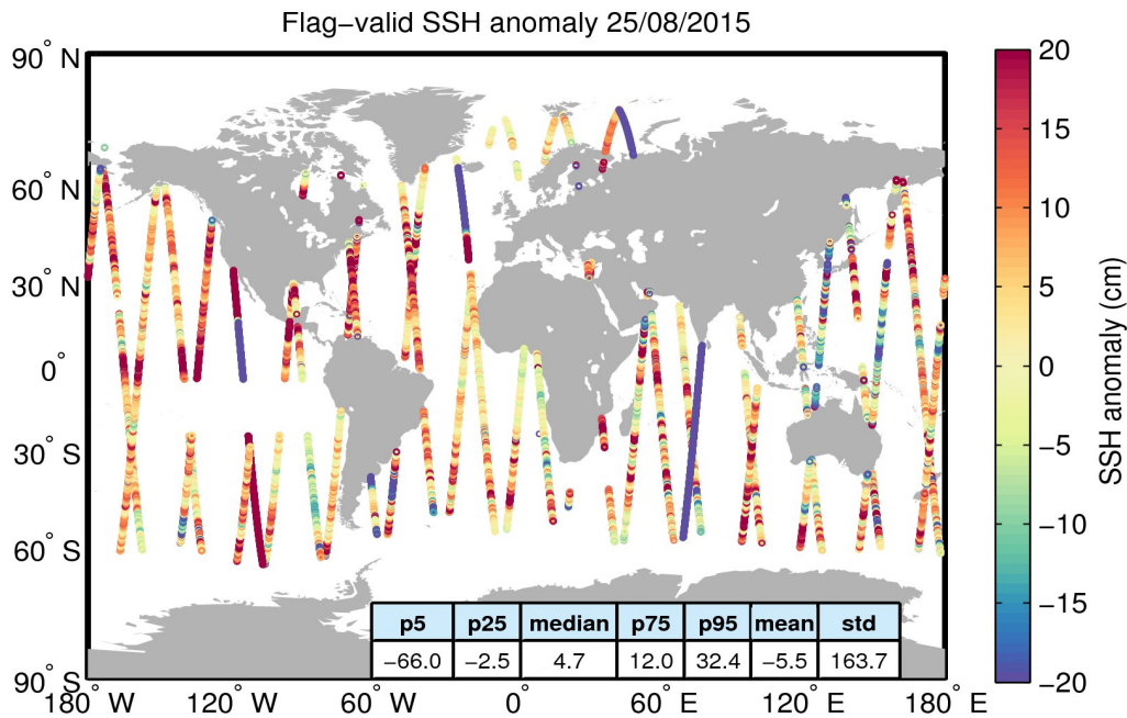
Figure 5. Geographical distribution of flag-valid 1-Hz SSH anomaly data over oceans and lakes for 25/08/2015. The statistical values shown in the table refer to the SSH anomaly in cm and are calculated over all measurements shown in the figure.
