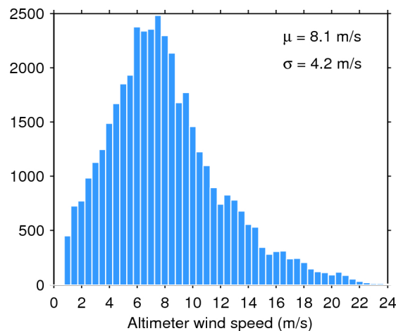
Figure 35. Histogram of science-valid wind over oceans and lakes for 25/08/2015. The mean ( \mu ) and standard deviation ( \sigma ) are also shown. Note that values larger than 24 m/s are excluded from the histogram for the sake of readability but not from the computation of \mu and \sigma .
