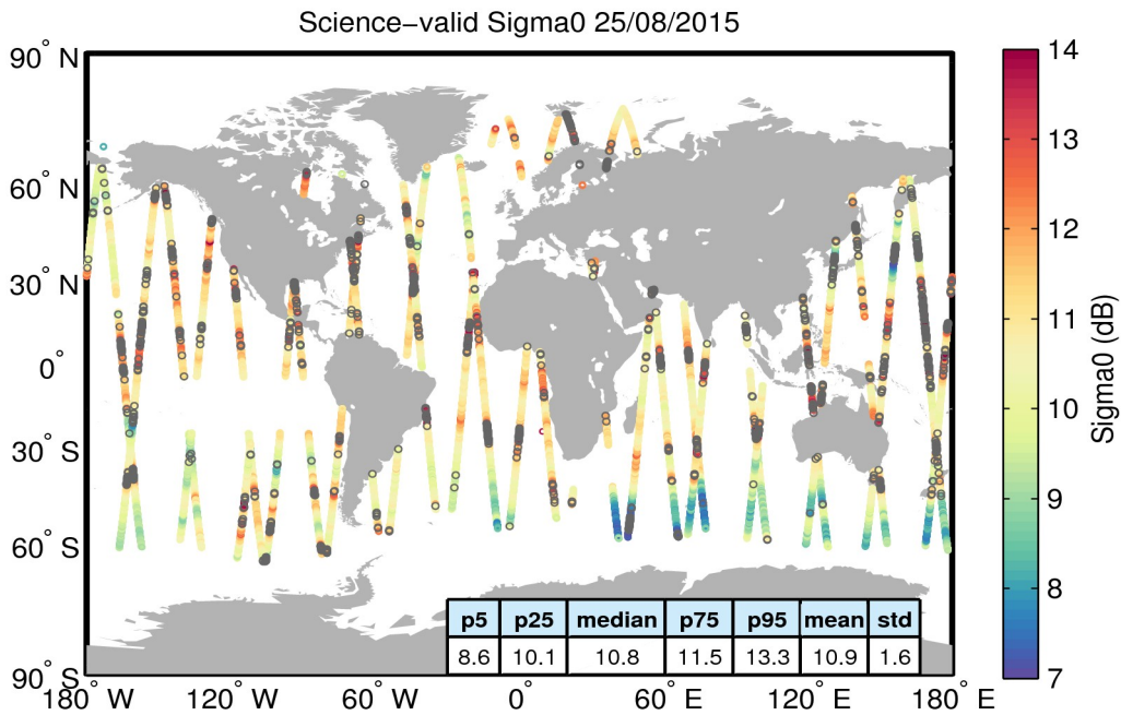
Figure 27. Geographical distribution of science-valid sigma0 data over oceans and lakes for 25/08/2015. The statistical values shown in the table refer to the sigma0 in dB and are calculated over all measurements shown in the figure. Gray circles denote records that have been rejected based on the editing criteria described in Table 4.
