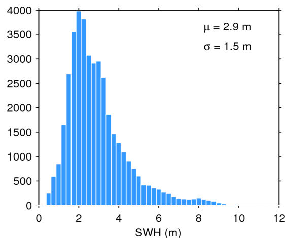
Figure 20. Histogram of science-valid SWH over oceans and lakes for 25/08/2015. The mean ( \mu ) and standard deviation ( \sigma ) are also shown. Note that values larger than 12 m are excluded from the histogram for the sake of readability but not from the computation of \mu and \sigma .
