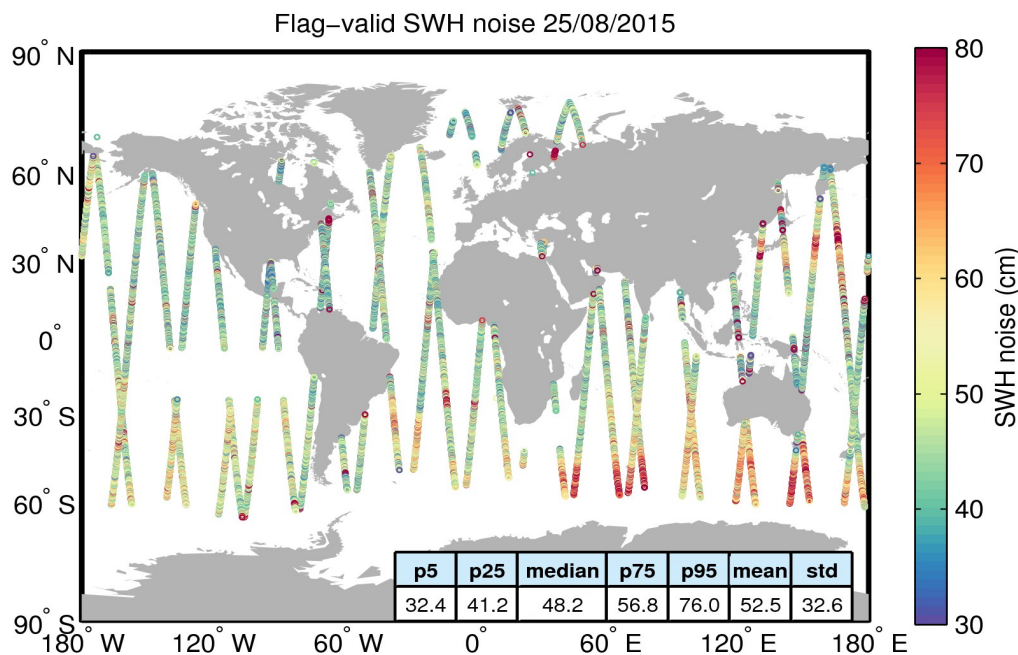
Figure 18. Geographical distribution of flag-valid 20-Hz SWH measurement noise over oceans and lakes for 25/08/2015. The statistical values shown in the figure refer to the SWH noise and are calculated over all measurements shown in the figure.
