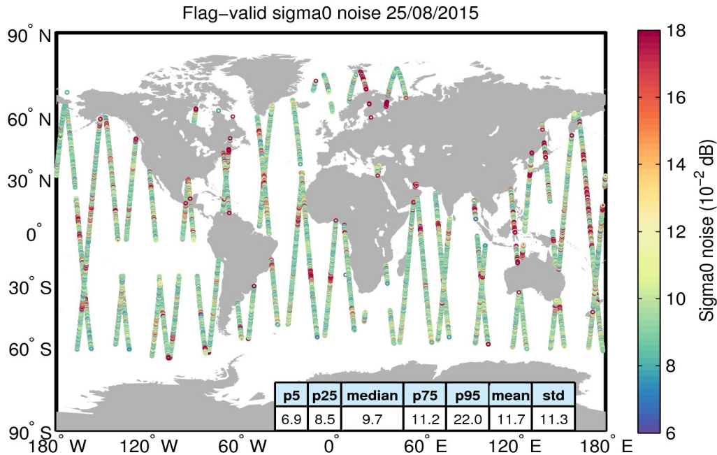
Figure 26. Geographical distribution of flag-valid 20-Hz sigma0 measurement noise over oceans and lakes for 25/08/2015. The statistical values shown in the table refer to the sigma0 noise and are calculated over all measurements shown in the figure.
