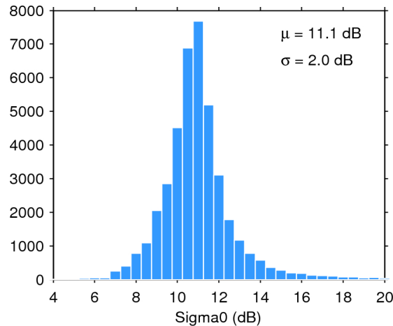
Figure 25. Histogram of flag-valid sigma0 over oceans and lakes for 25/08/2015. The mean ( \mu ) and standard deviation ( \sigma ) are also shown. Note that values outside [4 20] dB are excluded from the histogram for the sake of readability but not from the computation of \mu and \sigma .
