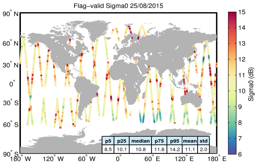
Figure 23. Geographical distribution of flag-valid sigma0 data over oceans and lakes for 25/08/2015. The statistical values shown in the table refer to the sigma0 in dB and are calculated over all measurements shown in the figure.
