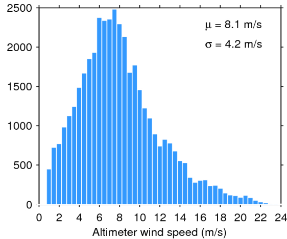
Figure 33. Histogram of flag-valid wind over oceans and lakes for 25/08/2015. The mean ( \mu ) and standard deviation ( \sigma ) are also shown. Note that values larger than 24 m/s are excluded from the histogram for the sake of readability but not from the computation of \mu and \sigma .
