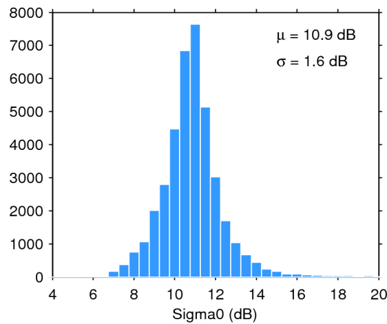
Figure 28. Histogram of science-valid sigma0 over oceans and lakes for 25/08/2015. The mean ( \mu ) and standard deviation ( \sigma ) are also shown. Note that values outside [4 20] dB are excluded from the histogram for the sake of readability but not from the computation of \mu and \sigma .
