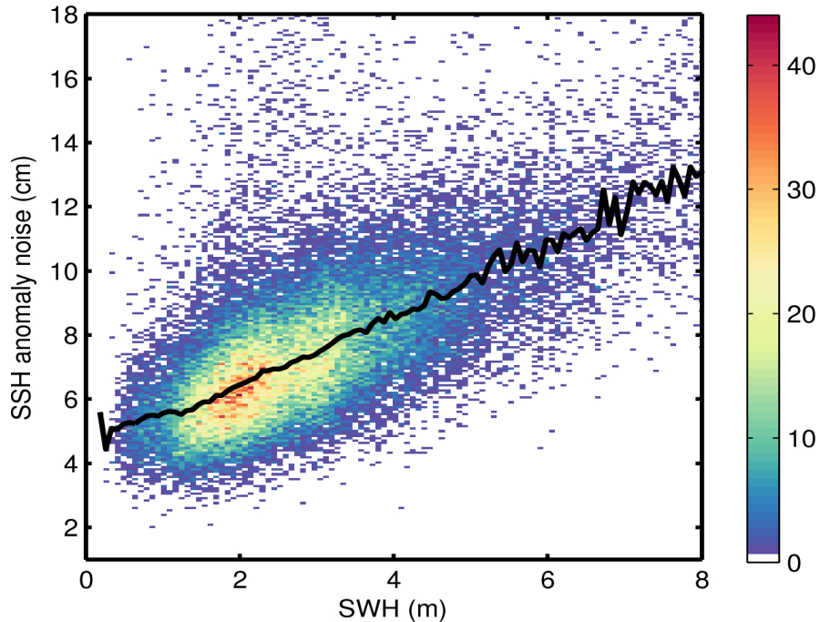
Figure 9. 2D histogram showing flag-valid SSH anomaly noise as a function of SWH for 25/08/2015. The black line denotes the median SSH anomaly as a function of SWH.
