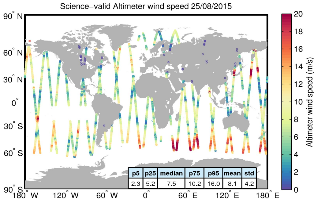
Figure 34. Geographical distribution of science-valid wind data over oceans and lakes for 25/08/2015. The statistical values shown in the table refer to the wind in m/s and are calculated over all measurements shown in the figure. Gray circles denote records that have been rejected based on the editing criteria described in Table 5.
