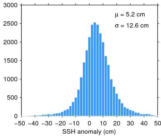
Figure 11. Histogram of science-valid SSH anomaly over oceans and lakes for 25/08/2015. The mean ( \mu ) and standard deviation ( \sigma ) are also shown. Note that values outside [-50 50] cm are excluded from the histogram for the sake of readability but not from the computation of \mu and \sigma .
