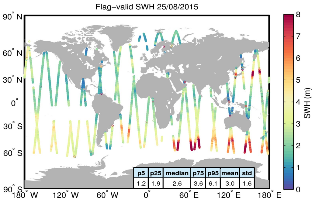
Figure 15. Geographical distribution of flag-valid SWH data over oceans and lakes for 25/08/2015. The statistical values shown in the table refer to the SWH in m and are calculated over all measurements shown in the figure.
