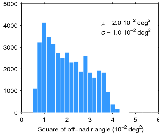
Figure 39. Histogram of flag-valid mispointing over oceans and lakes for 25/08/2015. The mean ( \mu ) and standard deviation ( \sigma ) are also shown. Note that values larger than 6 \cdot 10^{-2} \text{ deg}^2 are excluded from the histogram for the sake of readability but not from the computation of \mu and \sigma .
