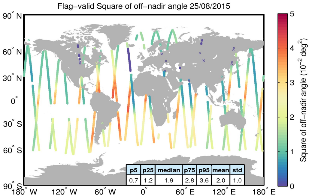
Figure 37. Geographical distribution of flag-valid mispointing data over oceans and lakes for 25/08/2015. The statistical values shown in the table refer to the mispointing in 10^{-2} \text{ deg}^2 and are calculated over all measurements shown in the figure.
