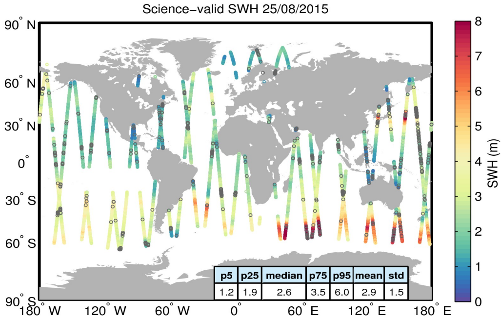
Figure 19. Geographical distribution of science-valid SWH data over oceans and lakes for 25/08/2015. The statistical values shown in the table refer to the SWH in m and are calculated over all measurements shown in the figure. Gray circles denote records that have been rejected based on the editing criteria described in Table 3.
