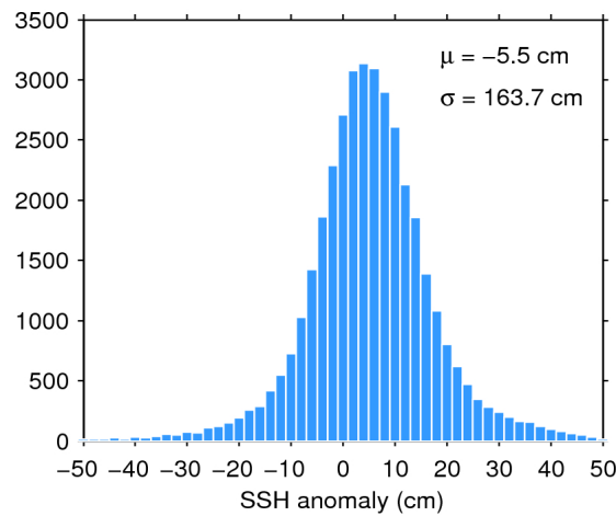
Figure 7. Histogram of flag-valid SSH anomaly over oceans and lakes for 25/08/2015. The mean ( \mu ) and standard deviation ( \sigma ) are also shown. Note that values outside [-50\ 50] cm are excluded from the histogram for the sake of readability but not from the computation of \mu and \sigma .
