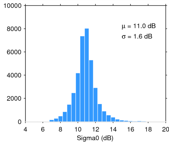
Figure 28. Histogram of science-valid sigma0 over oceans and lakes for 24/08/2015. The mean ( \mu ) and standard deviation ( \sigma ) are also shown. Note that values outside [4 20] dB are excluded from the histogram for the sake of readability but not from the computation of \mu and \sigma .
