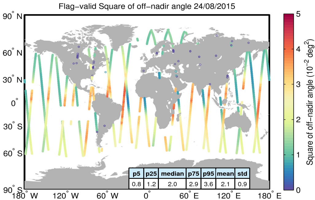
Figure 37. Geographical distribution of flag-valid mispointing data over oceans and lakes for 24/08/2015. The statistical values shown in the table refer to the mispointing in 10^{-2} \text{deg}^2 and are calculated over all measurements shown in the figure.
