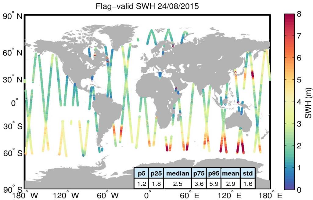
Figure 15. Geographical distribution of flag-valid SWH data over oceans and lakes for 24/08/2015. The statistical values shown in the table refer to the SWH in m and are calculated over all measurements shown in the figure.
