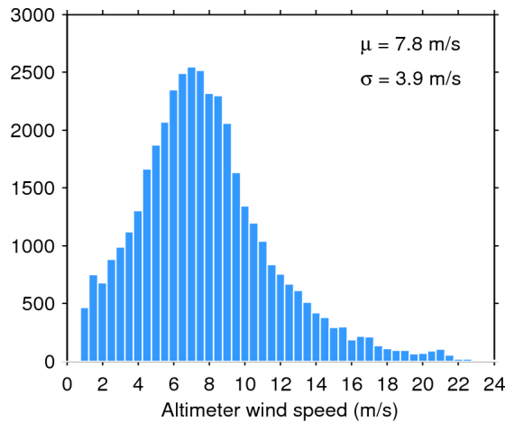
Figure 33. Histogram of flag-valid wind over oceans and lakes for 24/08/2015. The mean ( \mu ) and standard deviation ( \sigma ) are also shown. Note that values larger than 24 m/s are excluded from the histogram for the sake of readability but not from the computation of \mu and \sigma .
