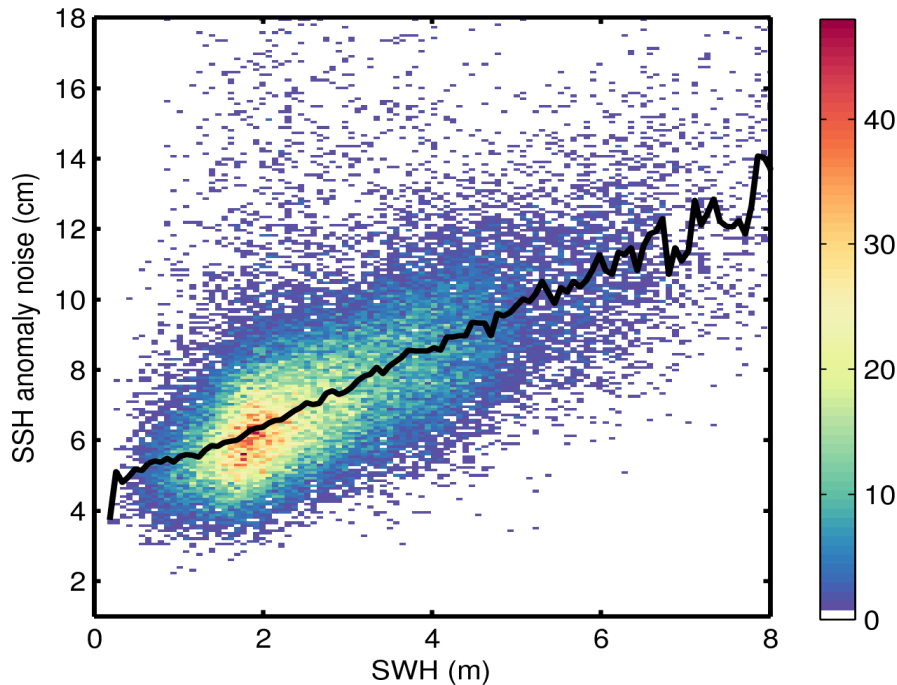
Figure 9. 2D histogram showing flag-valid SSH anomaly noise as a function of SWH for 24/08/2015. The black line denotes the median SSH anomaly as a function of SWH.
