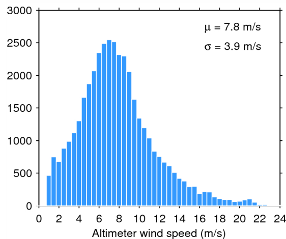
Figure 35. Histogram of science-valid wind over oceans and lakes for 24/08/2015. The mean ( \mu ) and standard deviation ( \sigma ) are also shown. Note that values larger than 24 m/s are excluded from the histogram for the sake of readability but not from the computation of \mu and \sigma .
