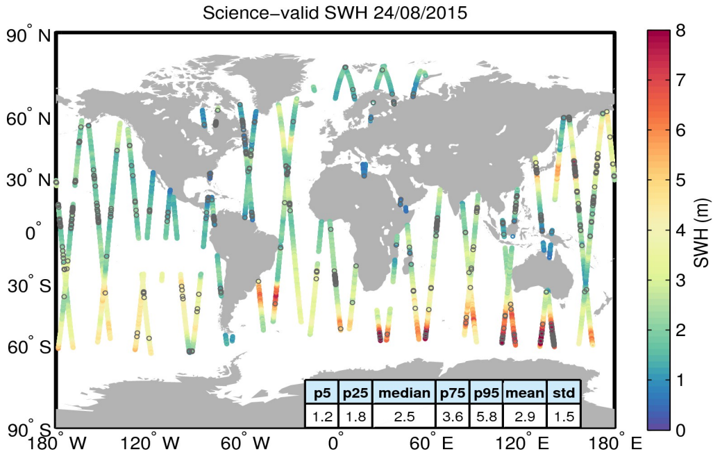
Figure 19. Geographical distribution of science-valid SWH data over oceans and lakes for 24/08/2015. The statistical values shown in the table refer to the SWH in m and are calculated over all measurements shown in the figure. Gray circles denote records that have been rejected based on the editing criteria described in Table 3.
