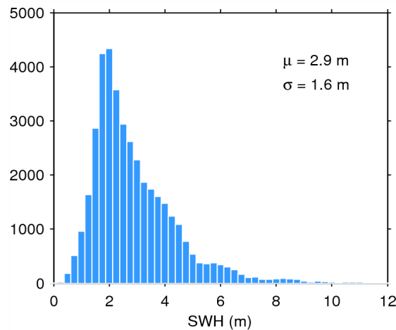
Figure 17. Histogram of flag-valid SWH over oceans and lakes for 24/08/2015. The mean ( \mu ) and standard deviation ( \sigma ) are also shown. Note that values larger than 12 m are excluded from the histogram for the sake of readability but not from the computation of \mu and \sigma .
