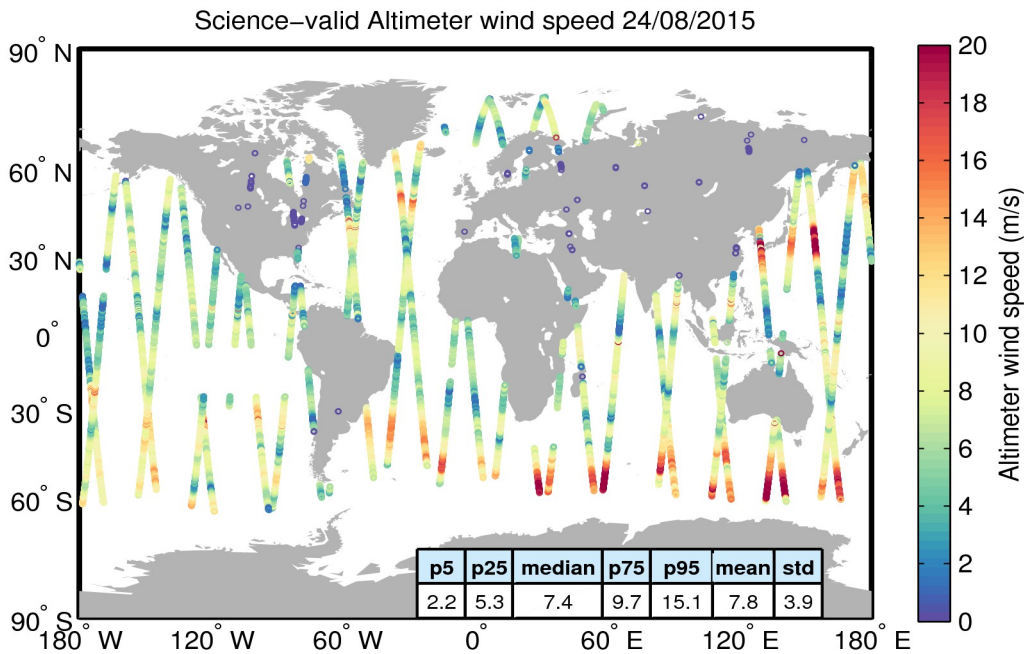
Figure 34. Geographical distribution of science-valid wind data over oceans and lakes for 24/08/2015. The statistical values shown in the table refer to the wind in m/s and are calculated over all measurements shown in the figure. Gray circles denote records that have been rejected based on the editing criteria described in Table 5.
