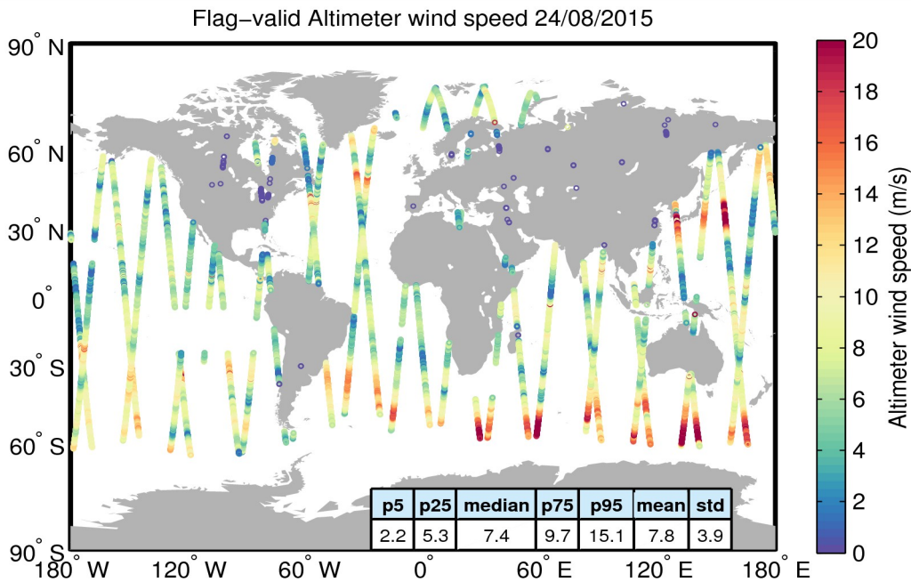
Figure 31. Geographical distribution of flag-valid wind data over oceans and lakes for 24/08/2015. The statistical values shown in the table refer to the wind in m/s and are calculated over all measurements shown in the figure.
