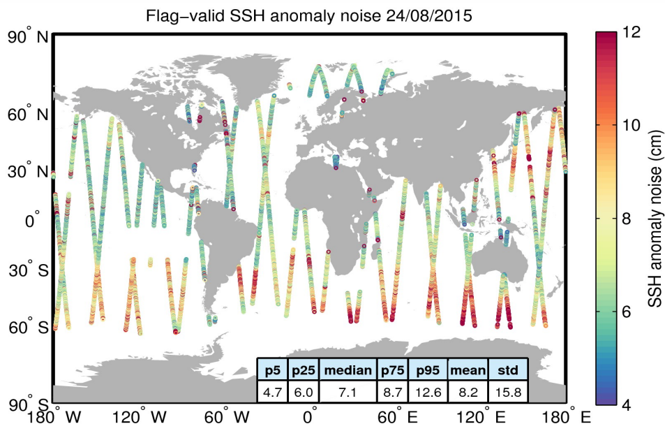
Figure 8. Geographical distribution of flag-valid 20-Hz SSH anomaly measurement noise over oceans and lakes for 24/08/2015. The statistical values shown in the table refer to the SSH anomaly noise and are calculated over all measurements shown in the figure.
