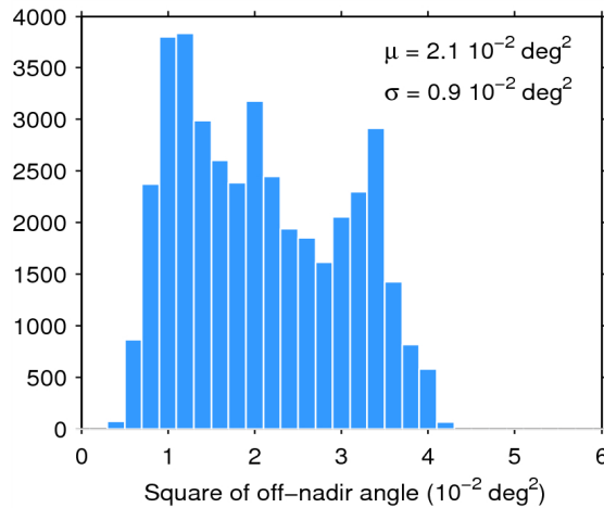
Figure 39. Histogram of flag-valid mispointing over oceans and lakes for 24/08/2015. The mean ( \mu ) and standard deviation ( \sigma ) are also shown. Note that values larger than 6 \cdot 10^{-2} \text{ deg}^2 are excluded from the histogram for the sake of readability but not from the computation of \mu and \sigma .
