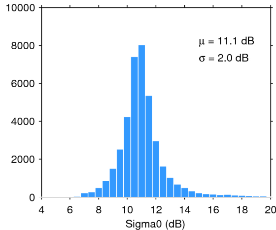
Figure 25. Histogram of flag-valid sigma0 over oceans and lakes for 24/08/2015. The mean ( \mu ) and standard deviation ( \sigma ) are also shown. Note that values outside [4 20] dB are excluded from the histogram for the sake of readability but not from the computation of \mu and \sigma .
