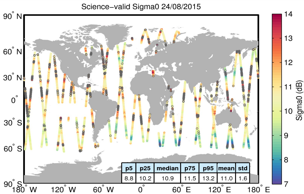
Figure 27. Geographical distribution of science-valid sigma0 data over oceans and lakes for 24/08/2015. The statistical values shown in the table refer to the sigma0 in dB and are calculated over all measurements shown in the figure. Gray circles denote records that have been rejected based on the editing criteria described in Table 4.
