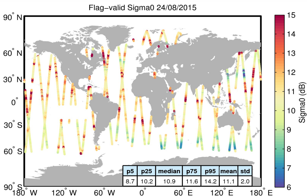
Figure 23. Geographical distribution of flag-valid sigma0 data over oceans and lakes for 24/08/2015. The statistical values shown in the table refer to the sigma0 in dB and are calculated over all measurements shown in the figure.
