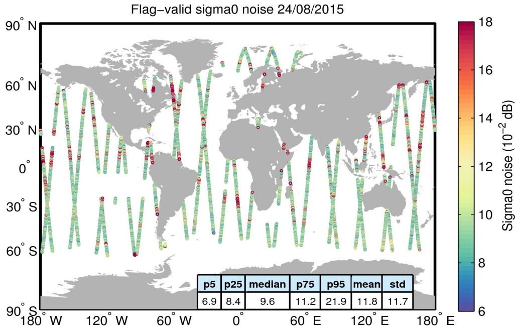
Figure 26. Geographical distribution of flag-valid 20-Hz sigma0 measurement noise over oceans and lakes for 24/08/2015. The statistical values shown in the table refer to the sigma0 noise and are calculated over all measurements shown in the figure.
