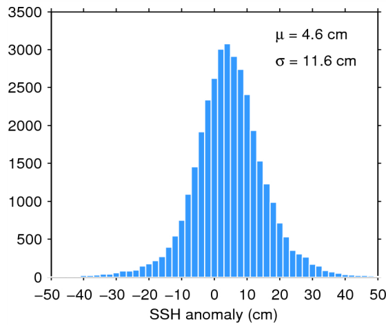
Figure 11. Histogram of science-valid SSH anomaly over oceans and lakes for 24/08/2015. The mean ( \mu ) and standard deviation ( \sigma ) are also shown. Note that values outside [-50 50] cm are excluded from the histogram for the sake of readability but not from the computation of \mu and \sigma .
