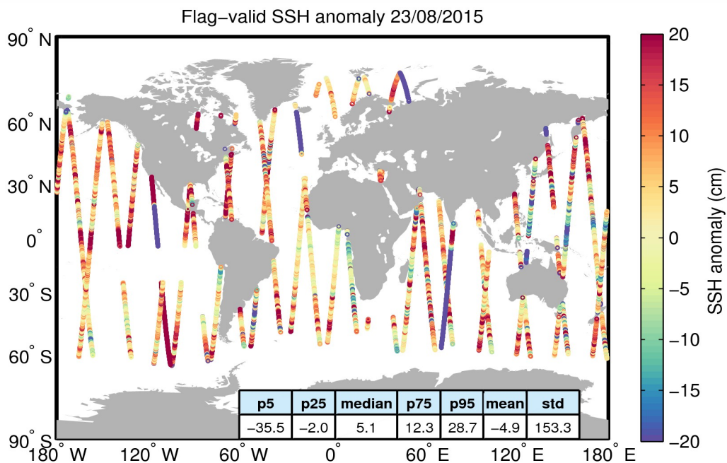
Figure 5. Geographical distribution of flag-valid 1-Hz SSH anomaly data over oceans and lakes for 23/08/2015. The statistical values shown in the table refer to the SSH anomaly in cm and are calculated over all measurements shown in the figure.
