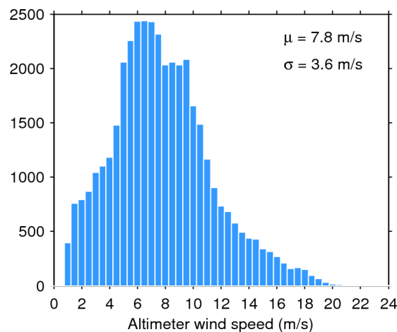
Figure 35. Histogram of science-valid wind over oceans and lakes for 23/08/2015. The mean ( \mu ) and standard deviation ( \sigma ) are also shown. Note that values larger than 24 m/s are excluded from the histogram for the sake of readability but not from the computation of \mu and \sigma .
