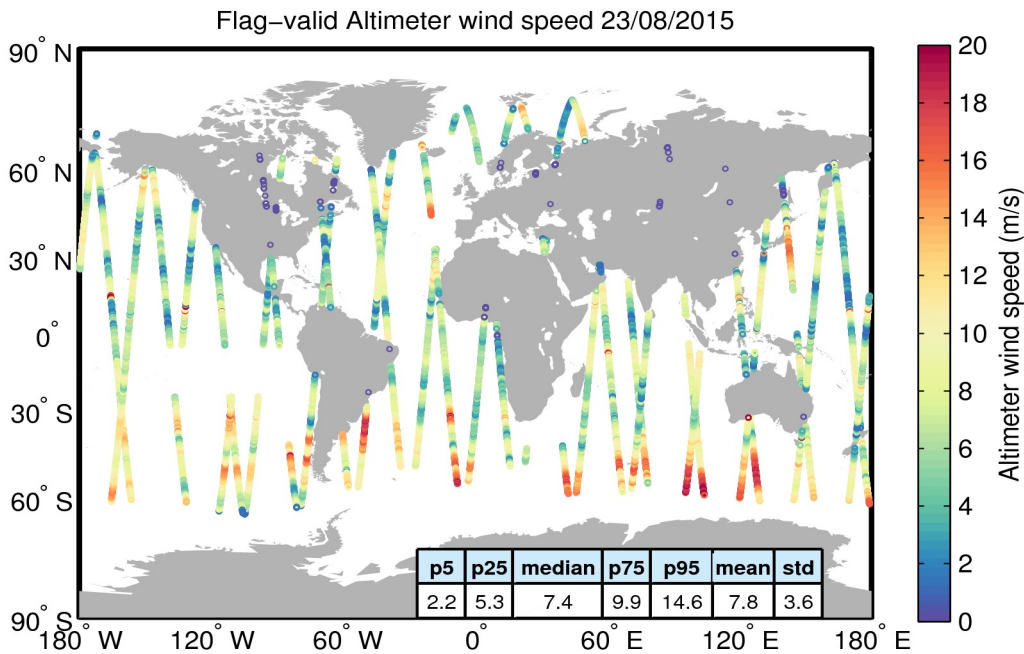
Figure 31. Geographical distribution of flag-valid wind data over oceans and lakes for 23/08/2015. The statistical values shown in the table refer to the wind in m/s and are calculated over all measurements shown in the figure.
