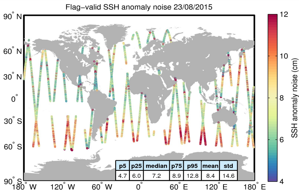
Figure 8. Geographical distribution of flag-valid 20-Hz SSH anomaly measurement noise over oceans and lakes for 23/08/2015. The statistical values shown in the table refer to the SSH anomaly noise and are calculated over all measurements shown in the figure.
