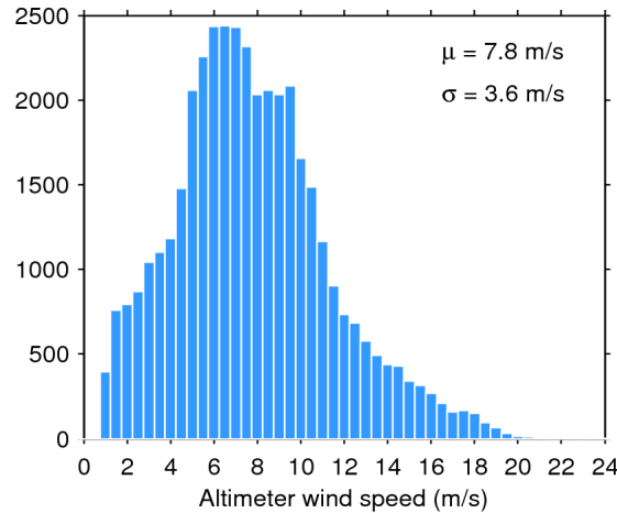
Figure 33. Histogram of flag-valid wind over oceans and lakes for 23/08/2015. The mean ( \mu ) and standard deviation ( \sigma ) are also shown. Note that values larger than 24 m/s are excluded from the histogram for the sake of readability but not from the computation of \mu and \sigma .
