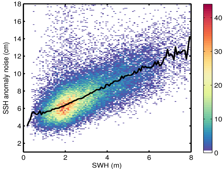
Figure 9. 2D histogram showing flag-valid SSH anomaly noise as a function of SWH for 23/08/2015. The black line denotes the median SSH anomaly as a function of SWH.
