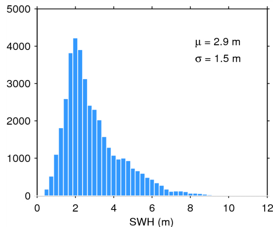
Figure 20. Histogram of science-valid SWH over oceans and lakes for 23/08/2015. The mean ( \mu ) and standard deviation ( \sigma ) are also shown. Note that values larger than 12 m are excluded from the histogram for the sake of readability but not from the computation of \mu and \sigma .
