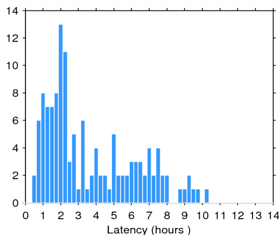
Figure 2. Histogram of the data latency for 23/08/2015. The y-axis denotes the number of files that are made available with a delay of x-hours with respect to the mean time of the records stored in the file.
