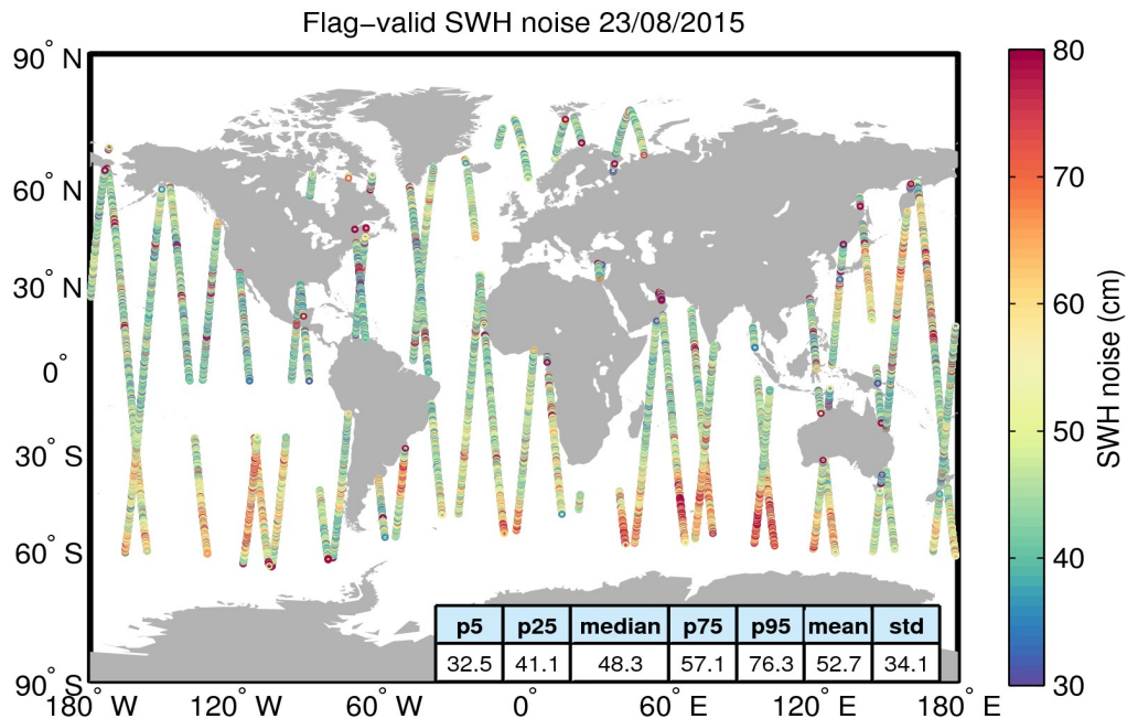
Figure 18. Geographical distribution of flag-valid 20-Hz SWH measurement noise over oceans and lakes for 23/08/2015. The statistical values shown in the figure refer to the SWH noise and are calculated over all measurements shown in the figure.
