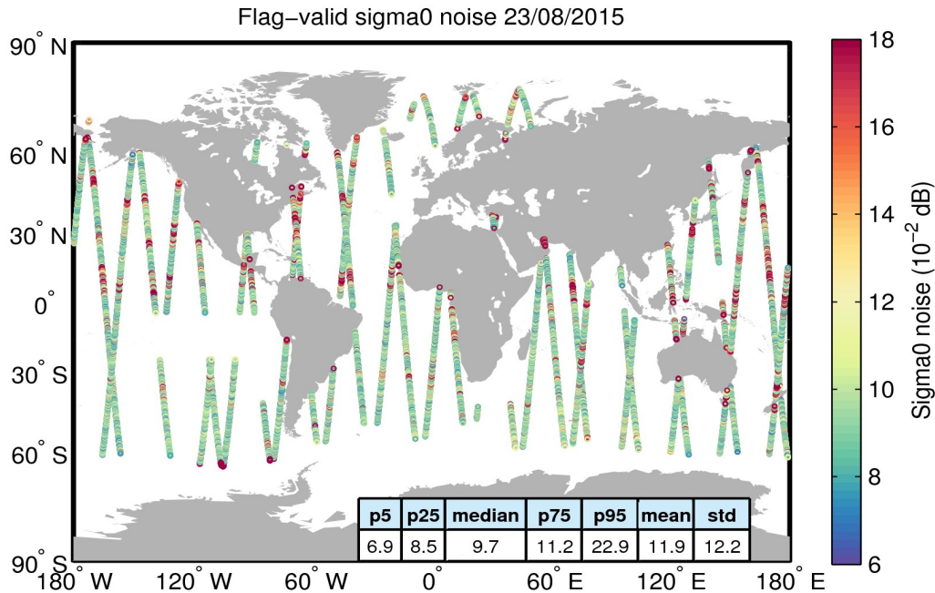
Figure 26. Geographical distribution of flag-valid 20-Hz sigma0 measurement noise over oceans and lakes for 23/08/2015. The statistical values shown in the table refer to the sigma0 noise and are calculated over all measurements shown in the figure.
