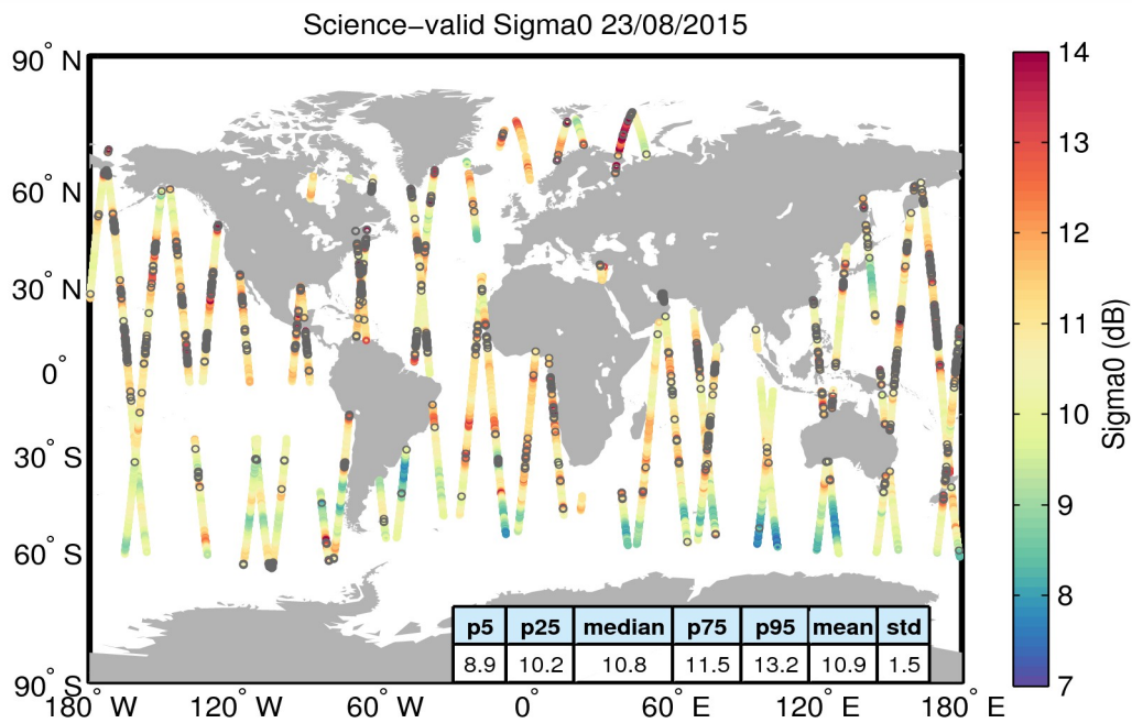
Figure 27. Geographical distribution of science-valid sigma0 data over oceans and lakes for 23/08/2015. The statistical values shown in the table refer to the sigma0 in dB and are calculated over all measurements shown in the figure. Gray circles denote records that have been rejected based on the editing criteria described in Table 4.
