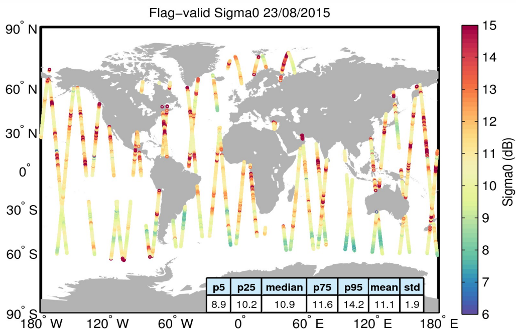
Figure 23. Geographical distribution of flag-valid sigma0 data over oceans and lakes for 23/08/2015. The statistical values shown in the table refer to the sigma0 in dB and are calculated over all measurements shown in the figure.
