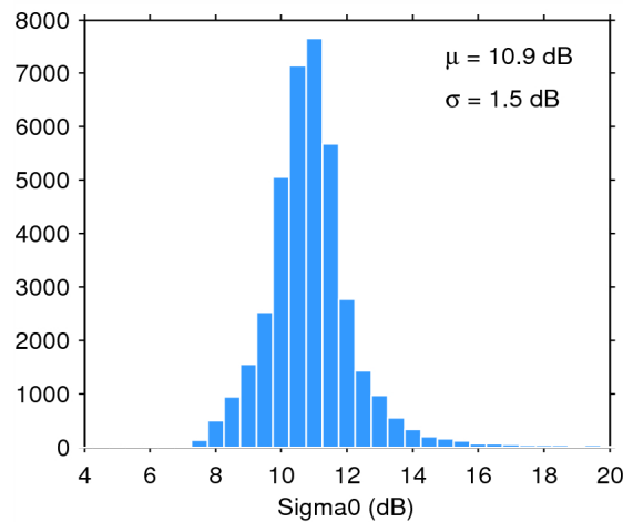
Figure 28. Histogram of science-valid sigma0 over oceans and lakes for 23/08/2015. The mean ( \mu ) and standard deviation ( \sigma ) are also shown. Note that values outside [4 20] dB are excluded from the histogram for the sake of readability but not from the computation of \mu and \sigma .
