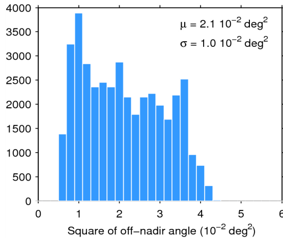
Figure 39. Histogram of flag-valid mispointing over oceans and lakes for 23/08/2015. The mean ( \mu ) and standard deviation ( \sigma ) are also shown. Note that values larger than 6 \cdot 10^{-2} \text{ deg}^2 are excluded from the histogram for the sake of readability but not from the computation of \mu and \sigma .
