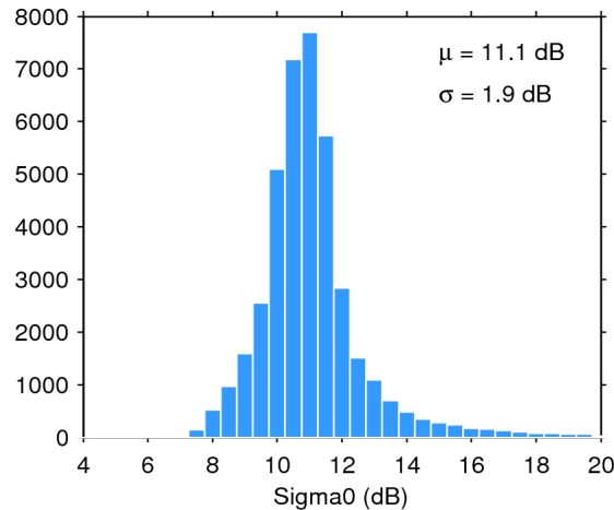
Figure 25. Histogram of flag-valid sigma0 over oceans and lakes for 23/08/2015. The mean ( \mu ) and standard deviation ( \sigma ) are also shown. Note that values outside [4 20] dB are excluded from the histogram for the sake of readability but not from the computation of \mu and \sigma .
