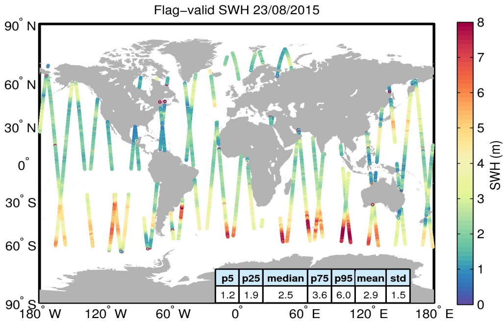
Figure 15. Geographical distribution of flag-valid SWH data over oceans and lakes for 23/08/2015. The statistical values shown in the table refer to the SWH in m and are calculated over all measurements shown in the figure.
