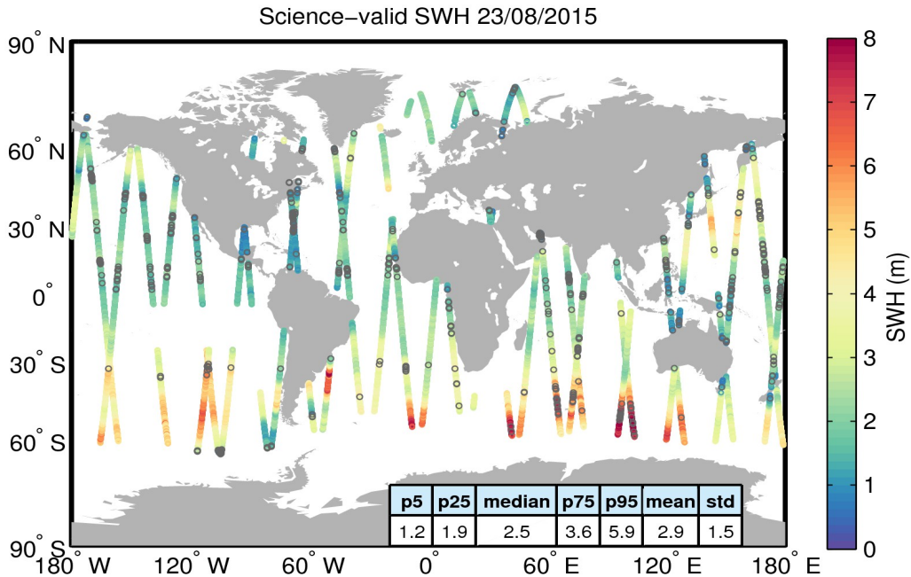
Figure 19. Geographical distribution of science-valid SWH data over oceans and lakes for 23/08/2015. The statistical values shown in the table refer to the SWH in m and are calculated over all measurements shown in the figure. Gray circles denote records that have been rejected based on the editing criteria described in Table 3.
