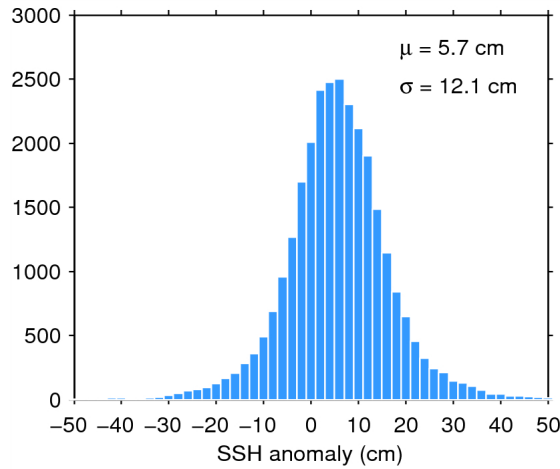
Figure 11. Histogram of science-valid SSH anomaly over oceans and lakes for 23/08/2015. The mean ( \mu ) and standard deviation ( \sigma ) are also shown. Note that values outside [-50 50] cm are excluded from the histogram for the sake of readability but not from the computation of \mu and \sigma .
