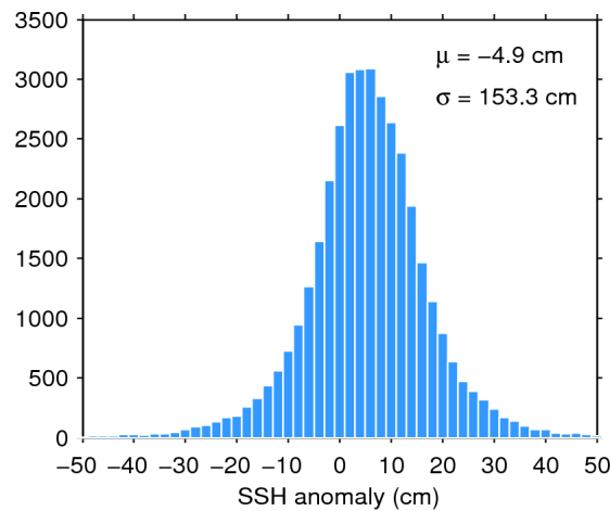
Figure 7. Histogram of flag-valid SSH anomaly over oceans and lakes for 23/08/2015. The mean ( \mu ) and standard deviation ( \sigma ) are also shown. Note that values outside [-50\ 50] cm are excluded from the histogram for the sake of readability but not from the computation of \mu and \sigma .
