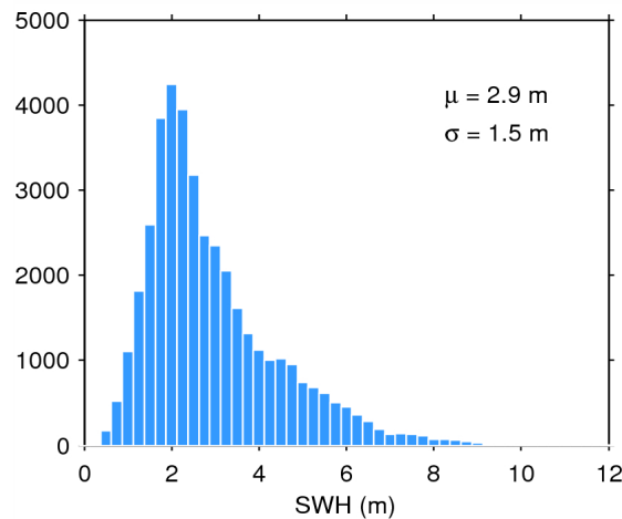
Figure 17. Histogram of flag-valid SWH over oceans and lakes for 23/08/2015. The mean ( \mu ) and standard deviation ( \sigma ) are also shown. Note that values larger than 12 m are excluded from the histogram for the sake of readability but not from the computation of \mu and \sigma .
