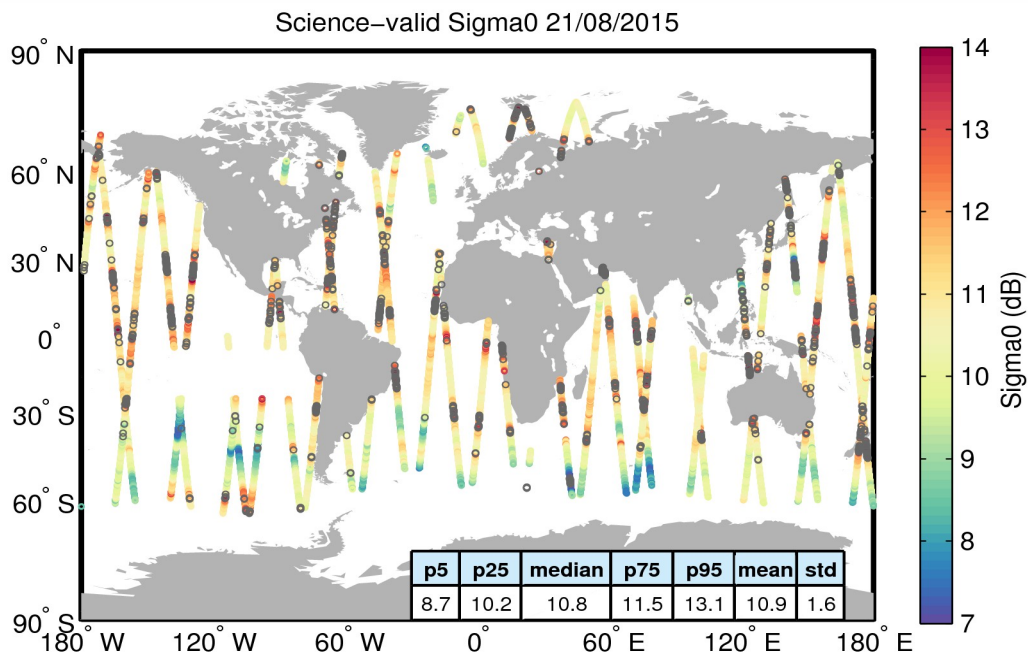
Figure 27. Geographical distribution of science-valid sigma0 data over oceans and lakes for 21/08/2015. The statistical values shown in the table refer to the sigma0 in dB and are calculated over all measurements shown in the figure. Gray circles denote records that have been rejected based on the editing criteria described in Table 4.
