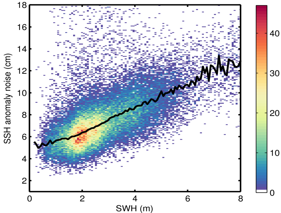
Figure 9. 2D histogram showing flag-valid SSH anomaly noise as a function of SWH for 21/08/2015. The black line denotes the median SSH anomaly as a function of SWH.
