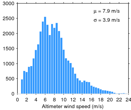
Figure 33. Histogram of flag-valid wind over oceans and lakes for 21/08/2015. The mean ( \mu ) and standard deviation ( \sigma ) are also shown. Note that values larger than 24 m/s are excluded from the histogram for the sake of readability but not from the computation of \mu and \sigma .
