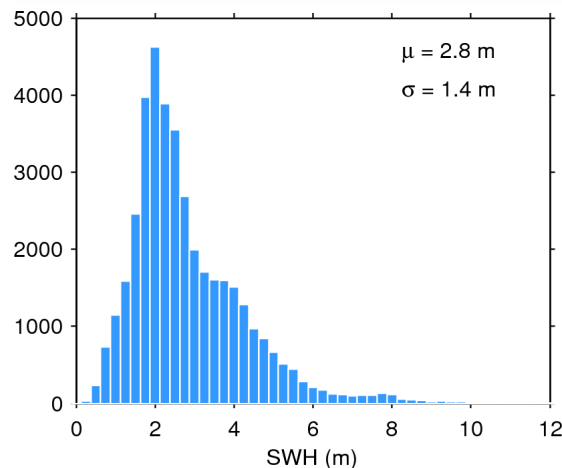
Figure 20. Histogram of science-valid SWH over oceans and lakes for 21/08/2015. The mean ( \mu ) and standard deviation ( \sigma ) are also shown. Note that values larger than 12 m are excluded from the histogram for the sake of readability but not from the computation of \mu and \sigma .
