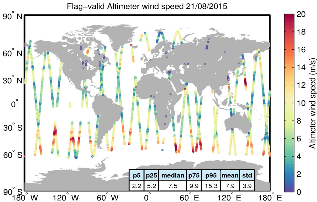
Figure 31. Geographical distribution of flag-valid wind data over oceans and lakes for 21/08/2015. The statistical values shown in the table refer to the wind in m/s and are calculated over all measurements shown in the figure.
