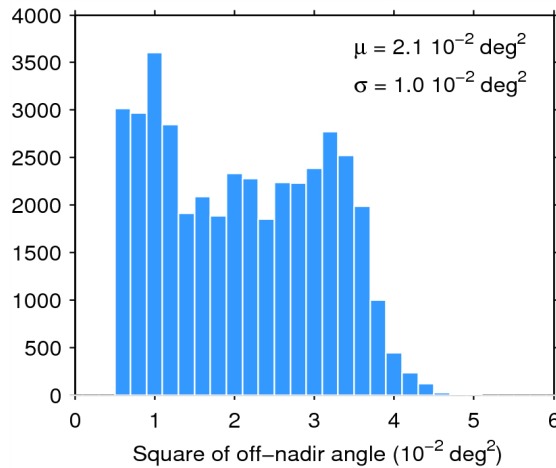
Figure 39. Histogram of flag-valid mispointing over oceans and lakes for 21/08/2015. The mean ( \mu ) and standard deviation ( \sigma ) are also shown. Note that values larger than 6 \cdot 10^{-2} \text{ deg}^2 are excluded from the histogram for the sake of readability but not from the computation of \mu and \sigma .
