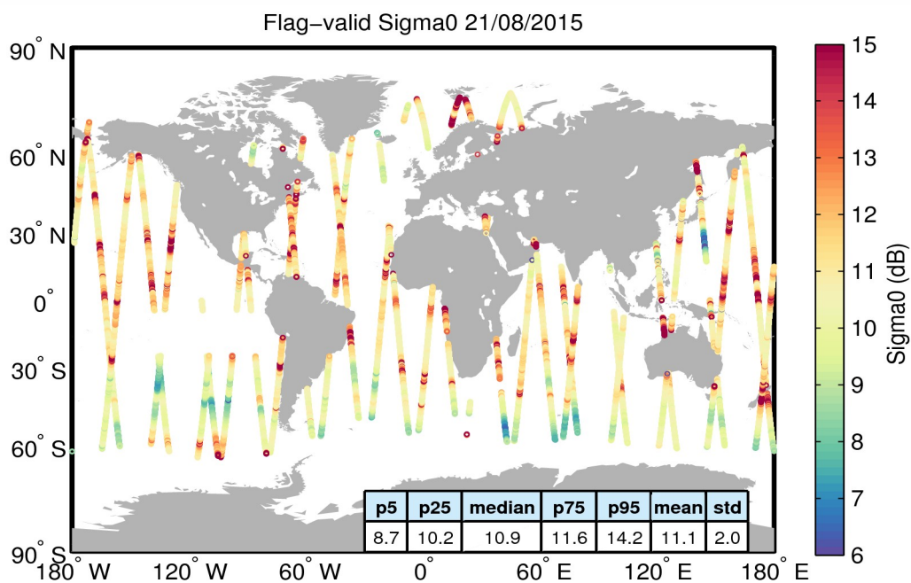
Figure 23. Geographical distribution of flag-valid sigma0 data over oceans and lakes for 21/08/2015. The statistical values shown in the table refer to the sigma0 in dB and are calculated over all measurements shown in the figure.
