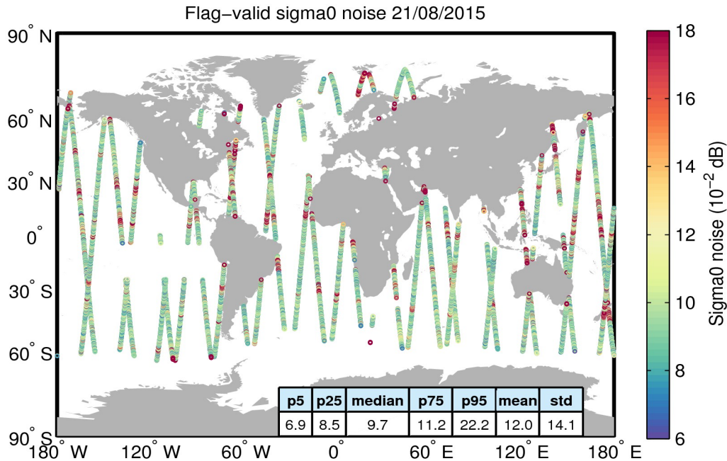
Figure 26. Geographical distribution of flag-valid 20-Hz sigma0 measurement noise over oceans and lakes for 21/08/2015. The statistical values shown in the table refer to the sigma0 noise and are calculated over all measurements shown in the figure.
