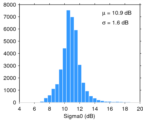
Figure 28. Histogram of science-valid sigma0 over oceans and lakes for 21/08/2015. The mean ( \mu ) and standard deviation ( \sigma ) are also shown. Note that values outside [4 20] dB are excluded from the histogram for the sake of readability but not from the computation of \mu and \sigma .
