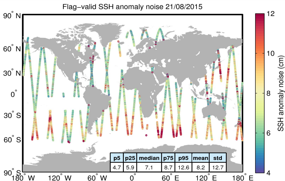
Figure 8. Geographical distribution of flag-valid 20-Hz SSH anomaly measurement noise over oceans and lakes for 21/08/2015. The statistical values shown in the table refer to the SSH anomaly noise and are calculated over all measurements shown in the figure.
