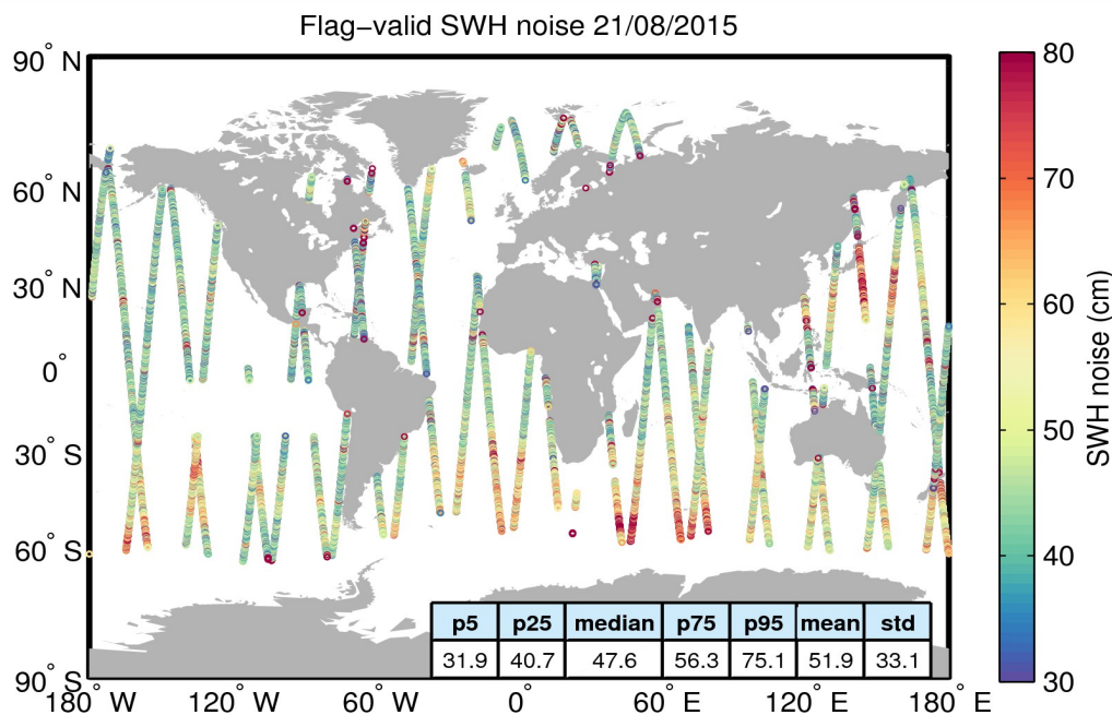
Figure 18. Geographical distribution of flag-valid 20-Hz SWH measurement noise over oceans and lakes for 21/08/2015. The statistical values shown in the figure refer to the SWH noise and are calculated over all measurements shown in the figure.
