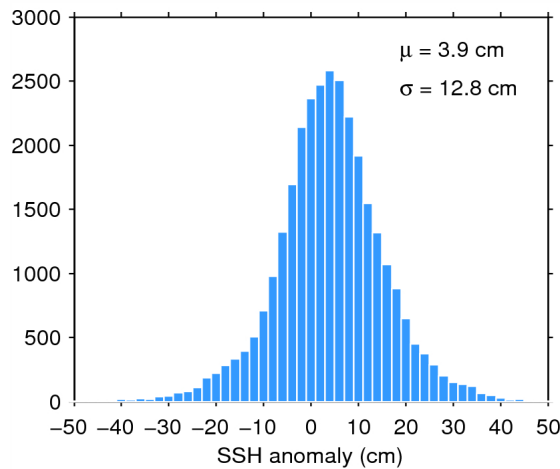
Figure 11. Histogram of science-valid SSH anomaly over oceans and lakes for 21/08/2015. The mean ( \mu ) and standard deviation ( \sigma ) are also shown. Note that values outside [-50 50] cm are excluded from the histogram for the sake of readability but not from the computation of \mu and \sigma .
