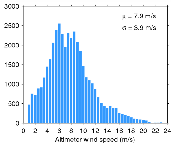
Figure 35. Histogram of science-valid wind over oceans and lakes for 21/08/2015. The mean ( \mu ) and standard deviation ( \sigma ) are also shown. Note that values larger than 24 m/s are excluded from the histogram for the sake of readability but not from the computation of \mu and \sigma .
