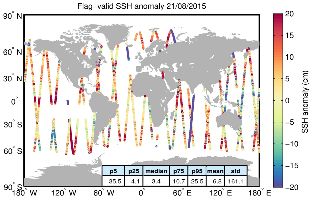
Figure 5. Geographical distribution of flag-valid 1-Hz SSH anomaly data over oceans and lakes for 21/08/2015. The statistical values shown in the table refer to the SSH anomaly in cm and are calculated over all measurements shown in the figure.
