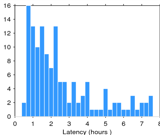
Figure 2. Histogram of the data latency for 21/08/2015. The y-axis denotes the number of files that are made available with a delay of x-hours with respect to the mean time of the records stored in the file.
