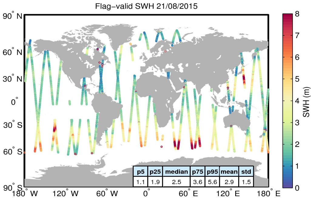
Figure 15. Geographical distribution of flag-valid SWH data over oceans and lakes for 21/08/2015. The statistical values shown in the table refer to the SWH in m and are calculated over all measurements shown in the figure.
