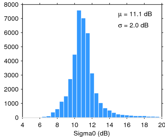
Figure 25. Histogram of flag-valid sigma0 over oceans and lakes for 21/08/2015. The mean ( \mu ) and standard deviation ( \sigma ) are also shown. Note that values outside [4 20] dB are excluded from the histogram for the sake of readability but not from the computation of \mu and \sigma .
