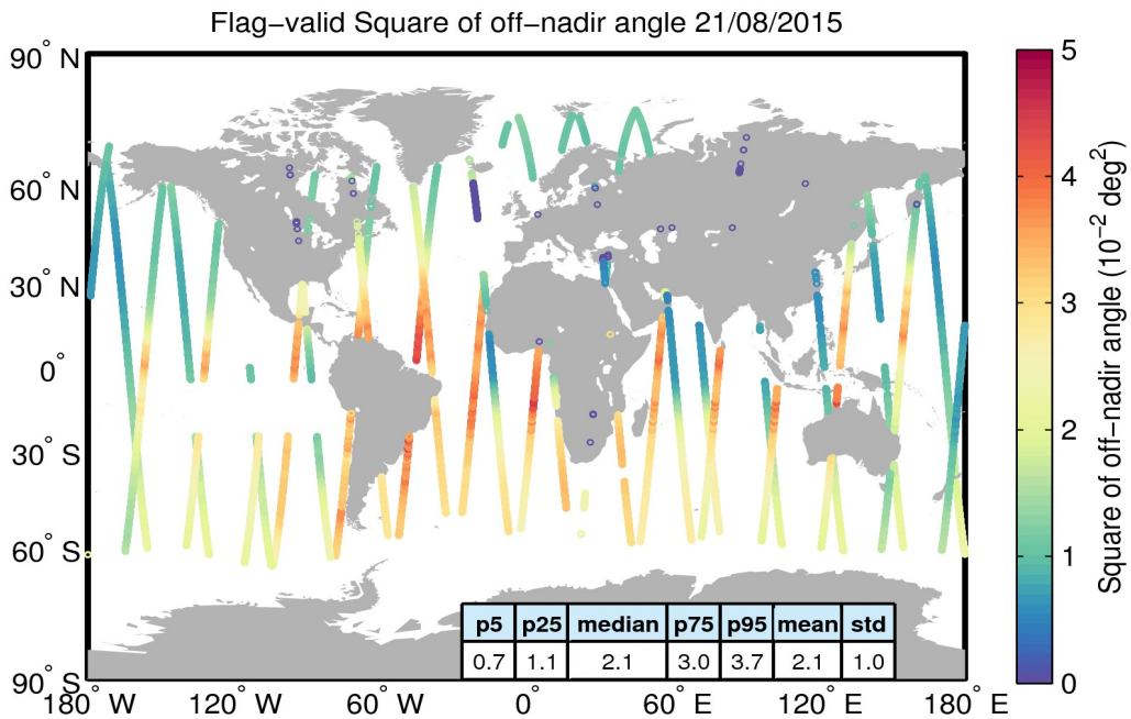
Figure 37. Geographical distribution of flag-valid mispointing data over oceans and lakes for 21/08/2015. The statistical values shown in the table refer to the mispointing in 10^{-2} \text{deg}^2 and are calculated over all measurements shown in the figure.
