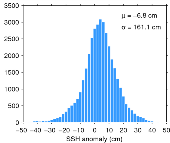
Figure 7. Histogram of flag-valid SSH anomaly over oceans and lakes for 21/08/2015. The mean ( \mu ) and standard deviation ( \sigma ) are also shown. Note that values outside [-50\ 50] cm are excluded from the histogram for the sake of readability but not from the computation of \mu and \sigma .
