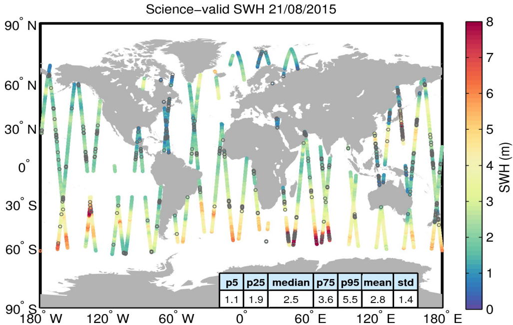
Figure 19. Geographical distribution of science-valid SWH data over oceans and lakes for 21/08/2015. The statistical values shown in the table refer to the SWH in m and are calculated over all measurements shown in the figure. Gray circles denote records that have been rejected based on the editing criteria described in Table 3.
