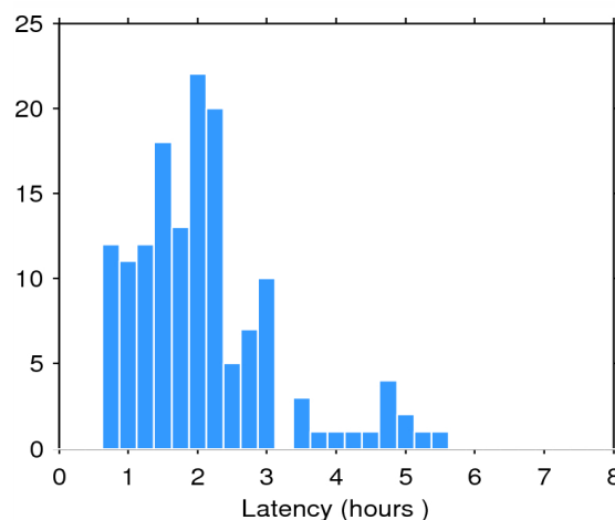
Figure 2. Histogram of the data latency for 20/08/2015. The y-axis denotes the number of files that are made available with a delay of x-hours with respect to the mean time of the records stored in the file.
