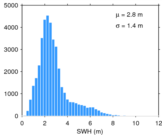
Figure 17. Histogram of flag-valid SWH over oceans and lakes for 19/08/2015. The mean ( \mu ) and standard deviation ( \sigma ) are also shown. Note that values larger than 12 m are excluded from the histogram for the sake of readability but not from the computation of \mu and \sigma .
