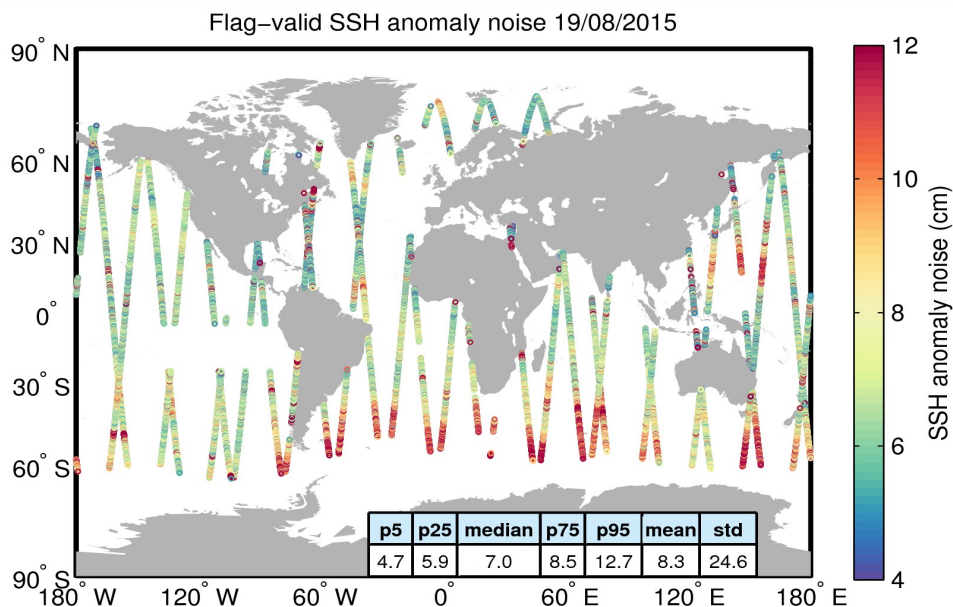
Figure 8. Geographical distribution of flag-valid 20-Hz SSH anomaly measurement noise over oceans and lakes for 19/08/2015. The statistical values shown in the table refer to the SSH anomaly noise and are calculated over all measurements shown in the figure.
