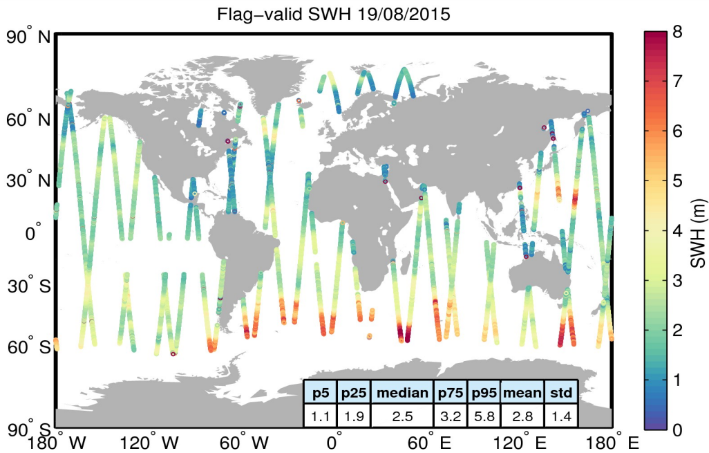
Figure 15. Geographical distribution of flag-valid SWH data over oceans and lakes for 19/08/2015. The statistical values shown in the table refer to the SWH in m and are calculated over all measurements shown in the figure.
