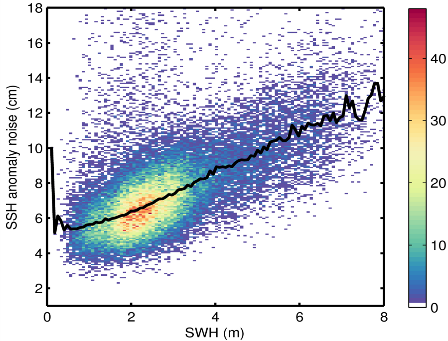
Figure 9. 2D histogram showing flag-valid SSH anomaly noise as a function of SWH for 19/08/2015. The black line denotes the median SSH anomaly as a function of SWH.
