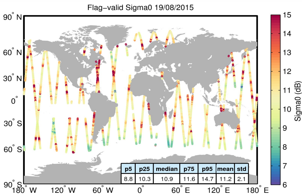
Figure 23. Geographical distribution of flag-valid sigma0 data over oceans and lakes for 19/08/2015. The statistical values shown in the table refer to the sigma0 in dB and are calculated over all measurements shown in the figure.
