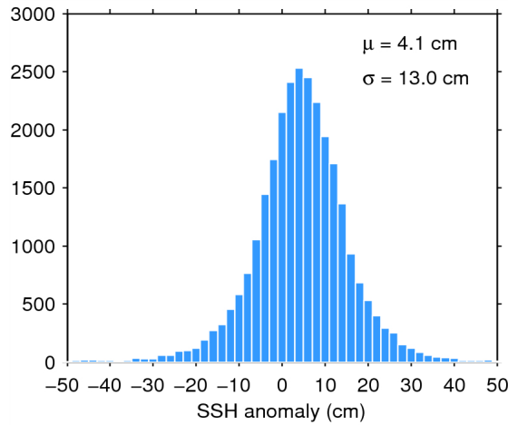
Figure 11. Histogram of science-valid SSH anomaly over oceans and lakes for 19/08/2015. The mean ( \mu ) and standard deviation ( \sigma ) are also shown. Note that values outside [-50 50] cm are excluded from the histogram for the sake of readability but not from the computation of \mu and \sigma .
