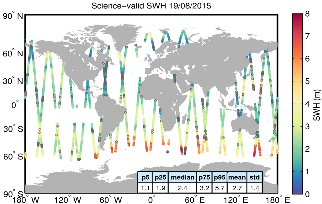
Figure 19. Geographical distribution of science-valid SWH data over oceans and lakes for 19/08/2015. The statistical values shown in the table refer to the SWH in m and are calculated over all measurements shown in the figure. Gray circles denote records that have been rejected based on the editing criteria described in Table 3.
