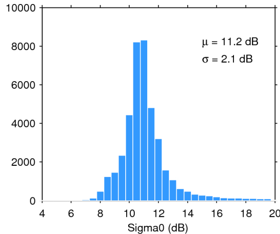
Figure 25. Histogram of flag-valid sigma0 over oceans and lakes for 19/08/2015. The mean ( \mu ) and standard deviation ( \sigma ) are also shown. Note that values outside [4 20] dB are excluded from the histogram for the sake of readability but not from the computation of \mu and \sigma .
