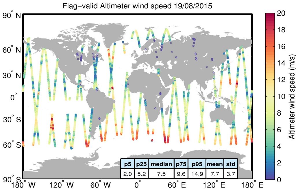
Figure 31. Geographical distribution of flag-valid wind data over oceans and lakes for 19/08/2015. The statistical values shown in the table refer to the wind in m/s and are calculated over all measurements shown in the figure.
