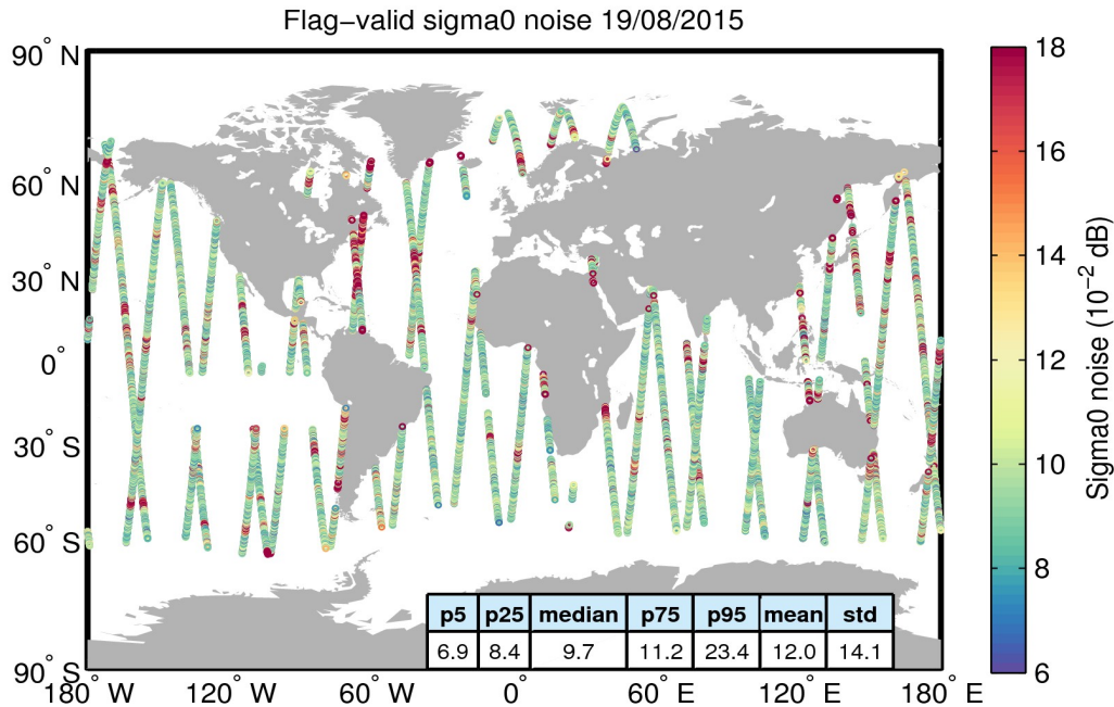
Figure 26. Geographical distribution of flag-valid 20-Hz sigma0 measurement noise over oceans and lakes for 19/08/2015. The statistical values shown in the table refer to the sigma0 noise and are calculated over all measurements shown in the figure.
