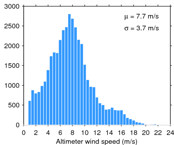
Figure 35. Histogram of science-valid wind over oceans and lakes for 19/08/2015. The mean ( \mu ) and standard deviation ( \sigma ) are also shown. Note that values larger than 24 m/s are excluded from the histogram for the sake of readability but not from the computation of \mu and \sigma .
