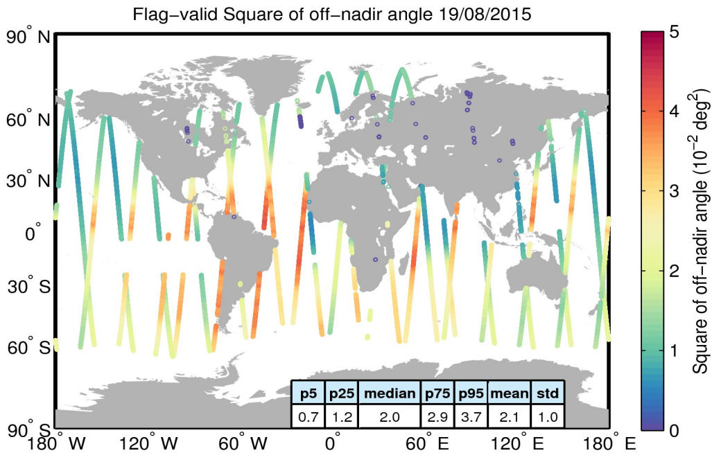
Figure 37. Geographical distribution of flag-valid mispointing data over oceans and lakes for 19/08/2015. The statistical values shown in the table refer to the mispointing in 10^{-2} deg 2 and are calculated over all measurements shown in the figure.
