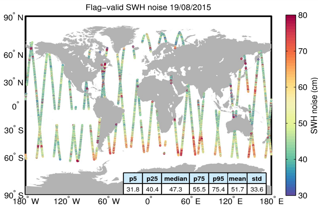
Figure 18. Geographical distribution of flag-valid 20-Hz SWH measurement noise over oceans and lakes for 19/08/2015. The statistical values shown in the figure refer to the SWH noise and are calculated over all measurements shown in the figure.
