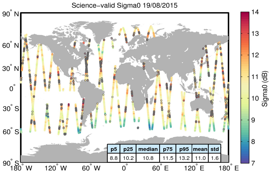
Figure 27. Geographical distribution of science-valid sigma0 data over oceans and lakes for 19/08/2015. The statistical values shown in the table refer to the sigma0 in dB and are calculated over all measurements shown in the figure. Gray circles denote records that have been rejected based on the editing criteria described in Table 4.
