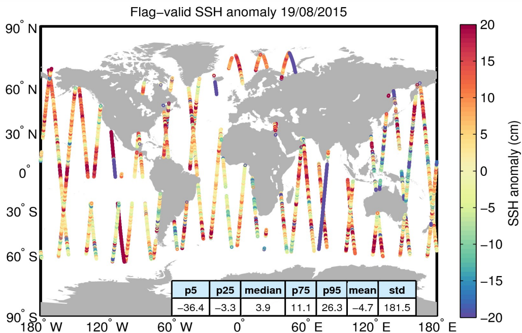
Figure 5. Geographical distribution of flag-valid 1-Hz SSH anomaly data over oceans and lakes for 19/08/2015. The statistical values shown in the table refer to the SSH anomaly in cm and are calculated over all measurements shown in the figure.
