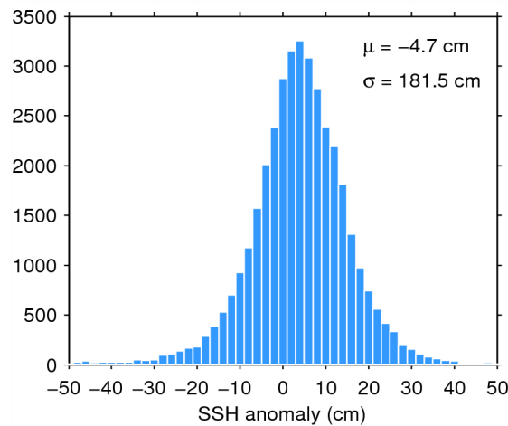
Figure 7. Histogram of flag-valid SSH anomaly over oceans and lakes for 19/08/2015. The mean ( \mu ) and standard deviation ( \sigma ) are also shown. Note that values outside [-50\ 50] cm are excluded from the histogram for the sake of readability but not from the computation of \mu and \sigma .
