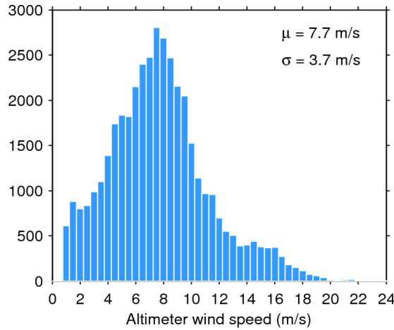
Figure 33. Histogram of flag-valid wind over oceans and lakes for 19/08/2015. The mean ( \mu ) and standard deviation ( \sigma ) are also shown. Note that values larger than 24 m/s are excluded from the histogram for the sake of readability but not from the computation of \mu and \sigma .
