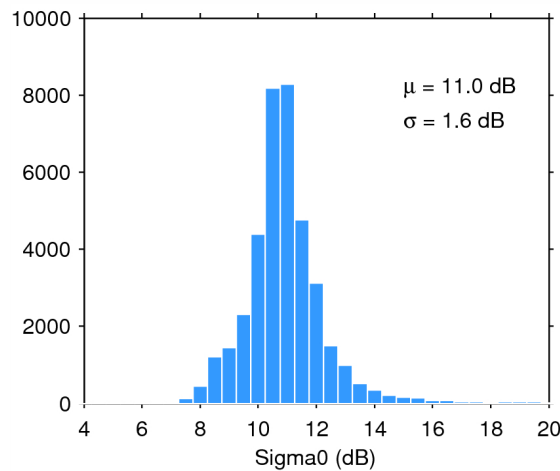
Figure 28. Histogram of science-valid sigma0 over oceans and lakes for 19/08/2015. The mean ( \mu ) and standard deviation ( \sigma ) are also shown. Note that values outside [4 20] dB are excluded from the histogram for the sake of readability but not from the computation of \mu and \sigma .
