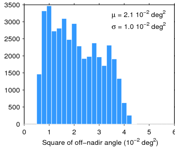
Figure 39. Histogram of flag-valid mispointing over oceans and lakes for 19/08/2015. The mean ( \mu ) and standard deviation ( \sigma ) are also shown. Note that values larger than 6 \cdot 10^{-2} \text{ deg}^2 are excluded from the histogram for the sake of readability but not from the computation of \mu and \sigma .
