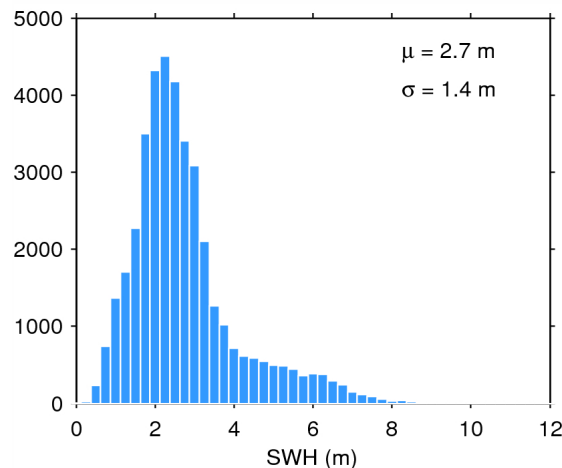
Figure 20. Histogram of science-valid SWH over oceans and lakes for 19/08/2015. The mean ( \mu ) and standard deviation ( \sigma ) are also shown. Note that values larger than 12 m are excluded from the histogram for the sake of readability but not from the computation of \mu and \sigma .
