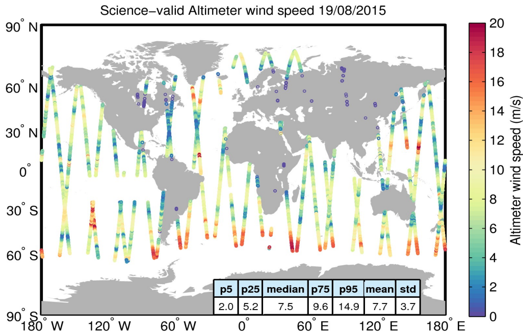
Figure 34. Geographical distribution of science-valid wind data over oceans and lakes for 19/08/2015. The statistical values shown in the table refer to the wind in m/s and are calculated over all measurements shown in the figure. Gray circles denote records that have been rejected based on the editing criteria described in Table 5.
