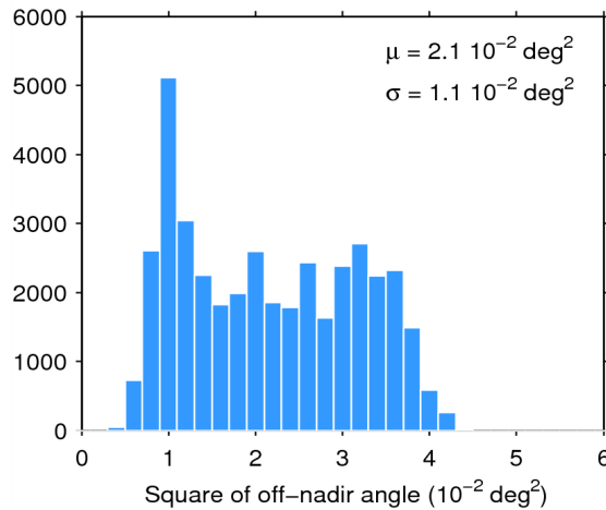
Figure 39. Histogram of flag-valid mispointing over oceans and lakes for 17/08/2015. The mean ( \mu ) and standard deviation ( \sigma ) are also shown. Note that values larger than 6 \cdot 10^{-2} \text{ deg}^2 are excluded from the histogram for the sake of readability but not from the computation of \mu and \sigma .
