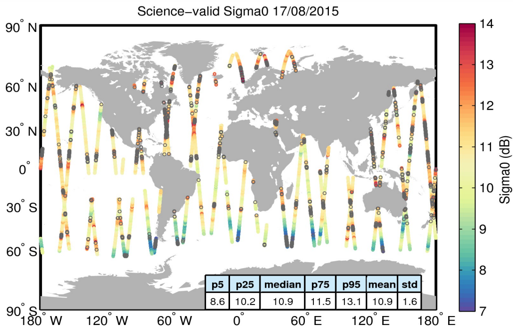
Figure 27. Geographical distribution of science-valid sigma0 data over oceans and lakes for 17/08/2015. The statistical values shown in the table refer to the sigma0 in dB and are calculated over all measurements shown in the figure. Gray circles denote records that have been rejected based on the editing criteria described in Table 4.
