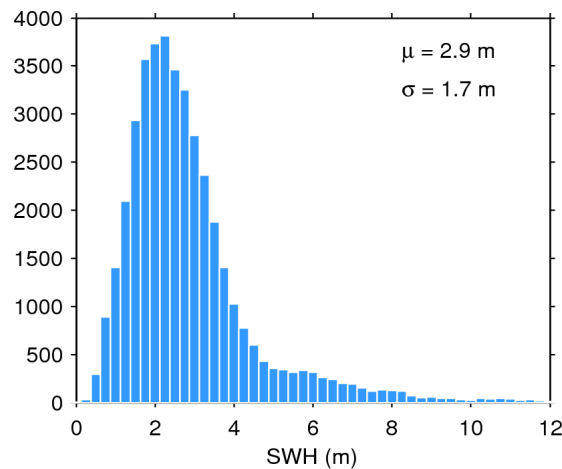
Figure 17. Histogram of flag-valid SWH over oceans and lakes for 17/08/2015. The mean ( \mu ) and standard deviation ( \sigma ) are also shown. Note that values larger than 12 m are excluded from the histogram for the sake of readability but not from the computation of \mu and \sigma .
