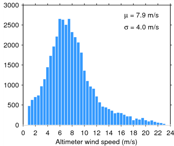
Figure 33. Histogram of flag-valid wind over oceans and lakes for 17/08/2015. The mean ( \mu ) and standard deviation ( \sigma ) are also shown. Note that values larger than 24 m/s are excluded from the histogram for the sake of readability but not from the computation of \mu and \sigma .
