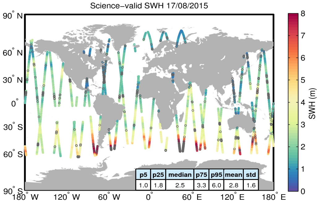
Figure 19. Geographical distribution of science-valid SWH data over oceans and lakes for 17/08/2015. The statistical values shown in the table refer to the SWH in m and are calculated over all measurements shown in the figure. Gray circles denote records that have been rejected based on the editing criteria described in Table 3.
