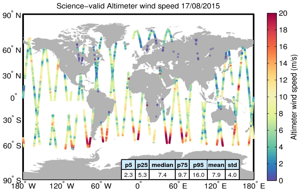
Figure 34. Geographical distribution of science-valid wind data over oceans and lakes for 17/08/2015. The statistical values shown in the table refer to the wind in m/s and are calculated over all measurements shown in the figure. Gray circles denote records that have been rejected based on the editing criteria described in Table 5.
