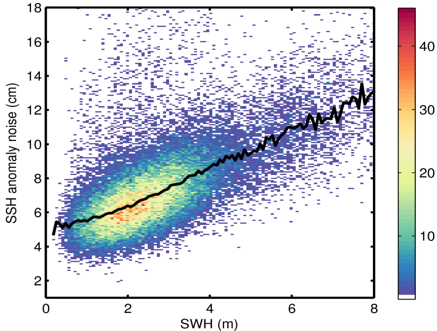
Figure 9. 2D histogram showing flag-valid SSH anomaly noise as a function of SWH for 17/08/2015. The black line denotes the median SSH anomaly as a function of SWH.
