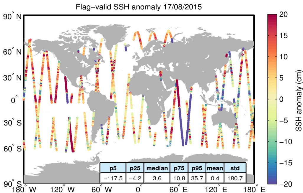
Figure 5. Geographical distribution of flag-valid 1-Hz SSH anomaly data over oceans and lakes for 17/08/2015. The statistical values shown in the table refer to the SSH anomaly in cm and are calculated over all measurements shown in the figure.
