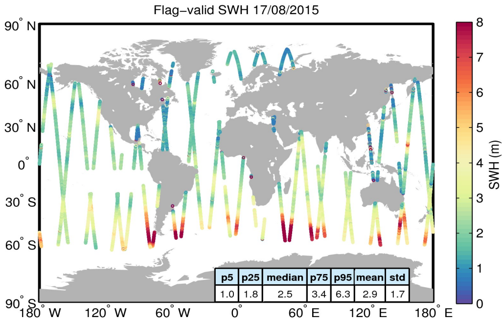
Figure 15. Geographical distribution of flag-valid SWH data over oceans and lakes for 17/08/2015. The statistical values shown in the table refer to the SWH in m and are calculated over all measurements shown in the figure.
