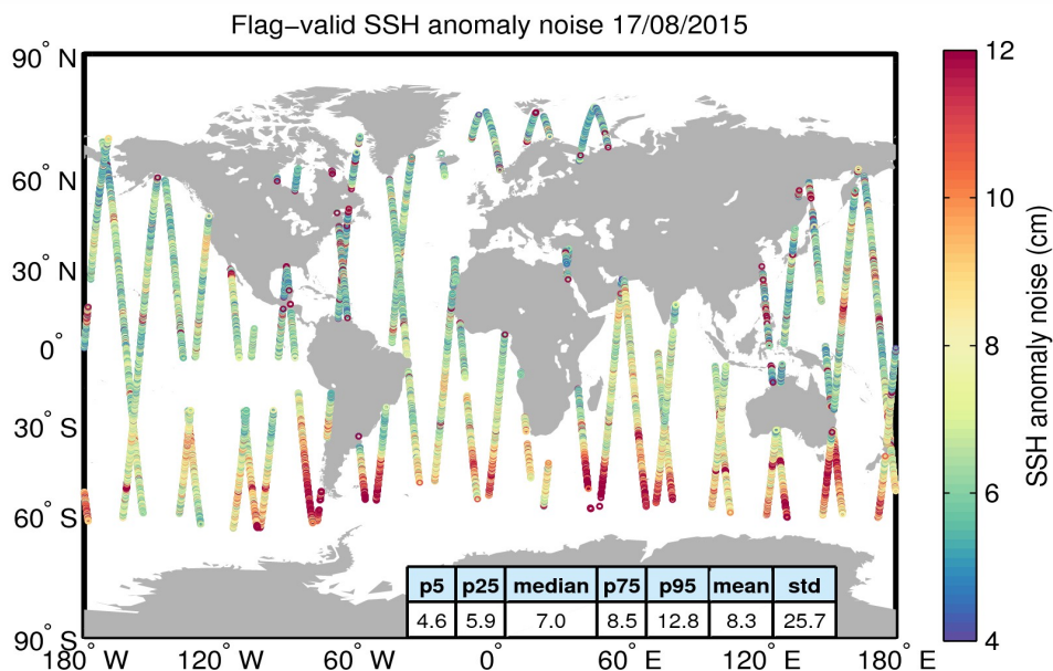
Figure 8. Geographical distribution of flag-valid 20-Hz SSH anomaly measurement noise over oceans and lakes for 17/08/2015. The statistical values shown in the table refer to the SSH anomaly noise and are calculated over all measurements shown in the figure.
