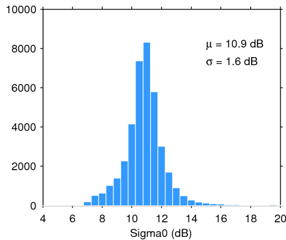
Figure 28. Histogram of science-valid sigma0 over oceans and lakes for 17/08/2015. The mean ( \mu ) and standard deviation ( \sigma ) are also shown. Note that values outside [4 20] dB are excluded from the histogram for the sake of readability but not from the computation of \mu and \sigma .
