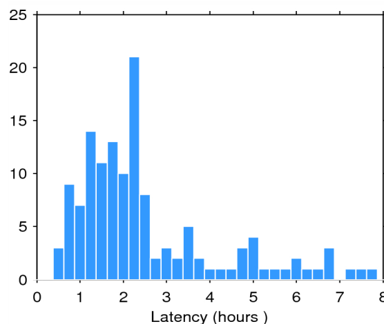
Figure 2. Histogram of the data latency for 17/08/2015. The y-axis denotes the number of files that are made available with a delay of x-hours with respect to the mean time of the records stored in the file.
