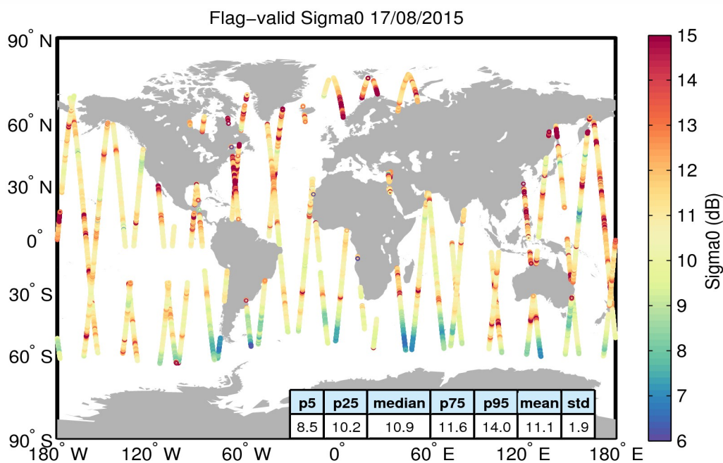
Figure 23. Geographical distribution of flag-valid sigma0 data over oceans and lakes for 17/08/2015. The statistical values shown in the table refer to the sigma0 in dB and are calculated over all measurements shown in the figure.
