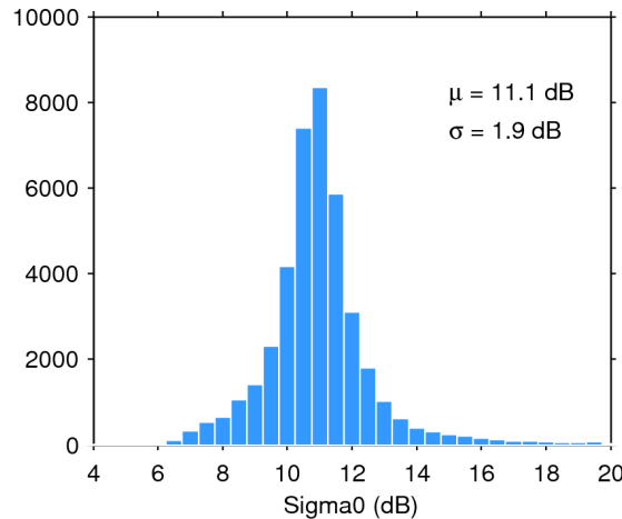
Figure 25. Histogram of flag-valid sigma0 over oceans and lakes for 17/08/2015. The mean ( \mu ) and standard deviation ( \sigma ) are also shown. Note that values outside [4 20] dB are excluded from the histogram for the sake of readability but not from the computation of \mu and \sigma .
