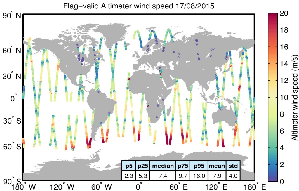
Figure 31. Geographical distribution of flag-valid wind data over oceans and lakes for 17/08/2015. The statistical values shown in the table refer to the wind in m/s and are calculated over all measurements shown in the figure.
