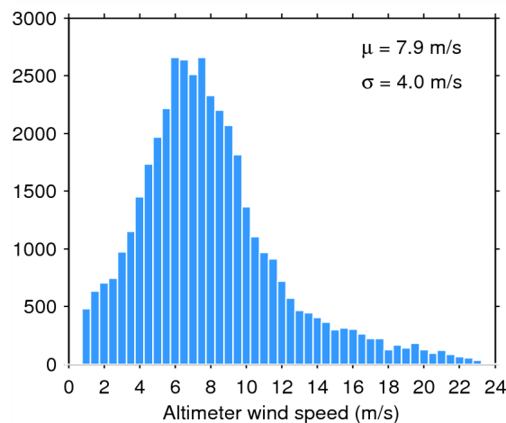
Figure 35. Histogram of science-valid wind over oceans and lakes for 17/08/2015. The mean ( \mu ) and standard deviation ( \sigma ) are also shown. Note that values larger than 24 m/s are excluded from the histogram for the sake of readability but not from the computation of \mu and \sigma .
