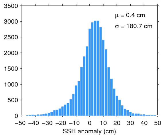
Figure 7. Histogram of flag-valid SSH anomaly over oceans and lakes for 17/08/2015. The mean ( \mu ) and standard deviation ( \sigma ) are also shown. Note that values outside [-50\ 50] cm are excluded from the histogram for the sake of readability but not from the computation of \mu and \sigma .
