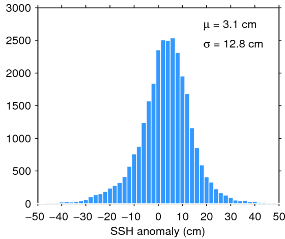
Figure 11. Histogram of science-valid SSH anomaly over oceans and lakes for 17/08/2015. The mean ( \mu ) and standard deviation ( \sigma ) are also shown. Note that values outside [-50 50] cm are excluded from the histogram for the sake of readability but not from the computation of \mu and \sigma .
