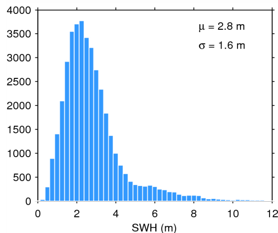
Figure 20. Histogram of science-valid SWH over oceans and lakes for 17/08/2015. The mean ( \mu ) and standard deviation ( \sigma ) are also shown. Note that values larger than 12 m are excluded from the histogram for the sake of readability but not from the computation of \mu and \sigma .
