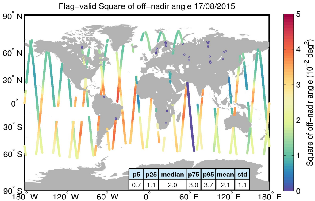
Figure 37. Geographical distribution of flag-valid mispointing data over oceans and lakes for 17/08/2015. The statistical values shown in the table refer to the mispointing in 10^{-2} \text{deg}^2 and are calculated over all measurements shown in the figure.
