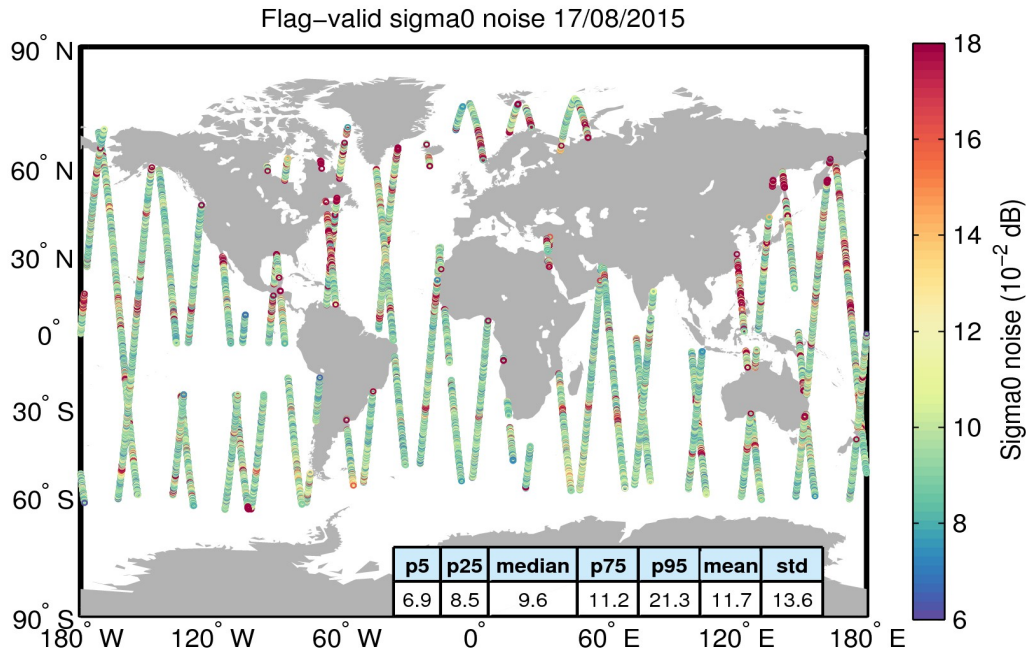
Figure 26. Geographical distribution of flag-valid 20-Hz sigma0 measurement noise over oceans and lakes for 17/08/2015. The statistical values shown in the table refer to the sigma0 noise and are calculated over all measurements shown in the figure.
