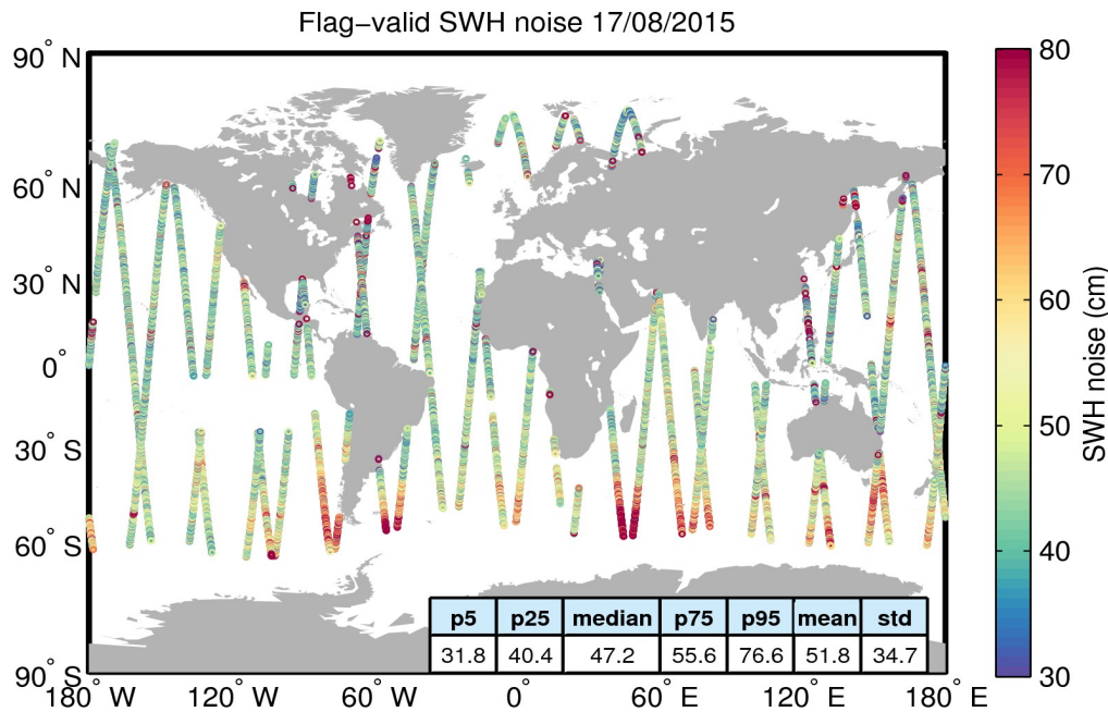
Figure 18. Geographical distribution of flag-valid 20-Hz SWH measurement noise over oceans and lakes for 17/08/2015. The statistical values shown in the figure refer to the SWH noise and are calculated over all measurements shown in the figure.
