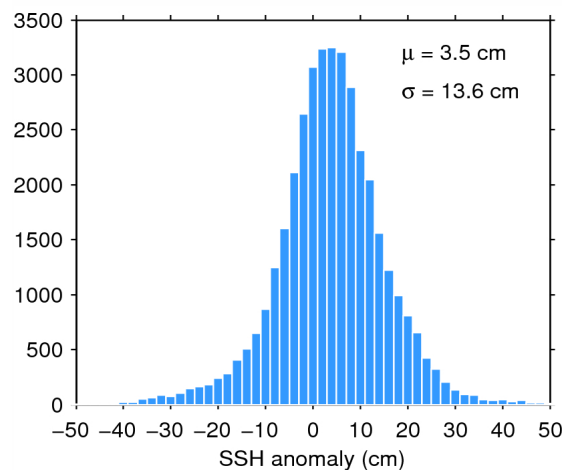
Figure 11. Histogram of science-valid SSH anomaly over oceans and lakes for 16/08/2015. The mean ( \mu ) and standard deviation ( \sigma ) are also shown. Note that values outside [-50 50] cm are excluded from the histogram for the sake of readability but not from the computation of \mu and \sigma .
