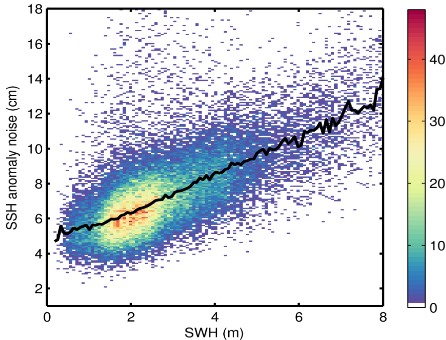
Figure 9. 2D histogram showing flag-valid SSH anomaly noise as a function of SWH for 16/08/2015. The black line denotes the median SSH anomaly as a function of SWH.
