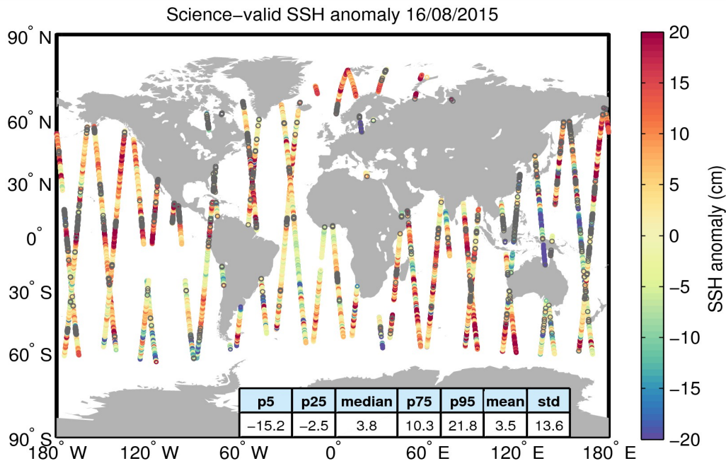
Figure 10. Geographical distribution of science-valid SSH anomaly data over oceans and lakes for 16/08/2015. The statistical values shown in the table refer to the SSH anomaly in cm and are calculated over all measurements shown in the figure. Gray circles denote records that have been rejected based on the editing criteria described in Table 2.
