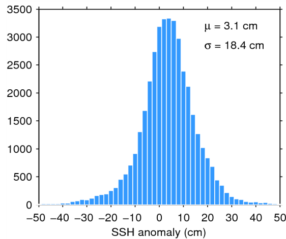
Figure 7. Histogram of flag-valid SSH anomaly over oceans and lakes for 16/08/2015. The mean ( \mu ) and standard deviation ( \sigma ) are also shown. Note that values outside [-50 50] cm are excluded from the histogram for the sake of readability but not from the computation of \mu and \sigma .
