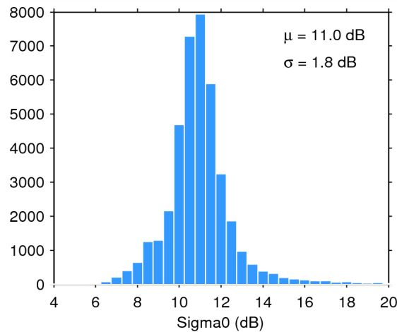
Figure 25. Histogram of flag-valid sigma0 over oceans and lakes for 16/08/2015. The mean ( \mu ) and standard deviation ( \sigma ) are also shown. Note that values outside [4 20] dB are excluded from the histogram for the sake of readability but not from the computation of \mu and \sigma .
