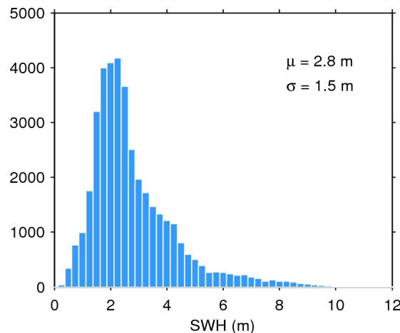
Figure 20. Histogram of science-valid SWH over oceans and lakes for 16/08/2015. The mean ( \mu ) and standard deviation ( \sigma ) are also shown. Note that values larger than 12 m are excluded from the histogram for the sake of readability but not from the computation of \mu and \sigma .
