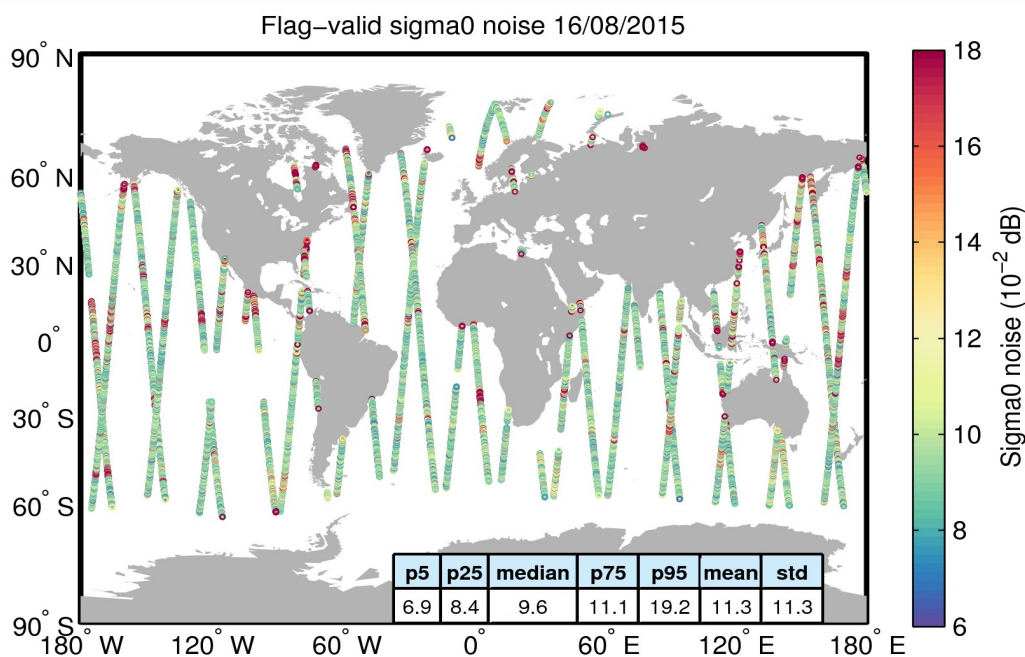
Figure 26. Geographical distribution of flag-valid 20-Hz sigma0 measurement noise over oceans and lakes for 16/08/2015. The statistical values shown in the table refer to the sigma0 noise and are calculated over all measurements shown in the figure.
