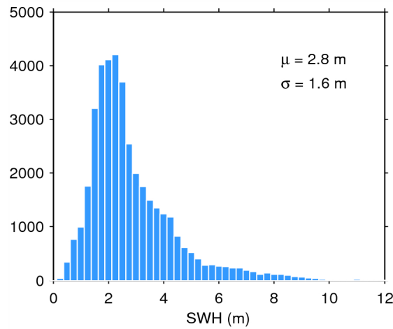
Figure 17. Histogram of flag-valid SWH over oceans and lakes for 16/08/2015. The mean ( \mu ) and standard deviation ( \sigma ) are also shown. Note that values larger than 12 m are excluded from the histogram for the sake of readability but not from the computation of \mu and \sigma .
