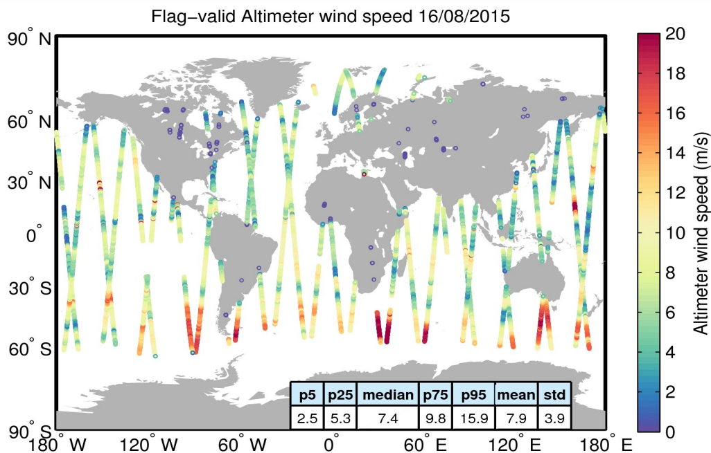
Figure 31. Geographical distribution of flag-valid wind data over oceans and lakes for 16/08/2015. The statistical values shown in the table refer to the wind in m/s and are calculated over all measurements shown in the figure.
