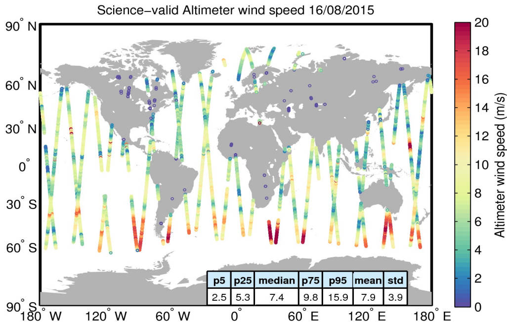
Figure 34. Geographical distribution of science-valid wind data over oceans and lakes for 16/08/2015. The statistical values shown in the table refer to the wind in m/s and are calculated over all measurements shown in the figure. Gray circles denote records that have been rejected based on the editing criteria described in Table 5.
