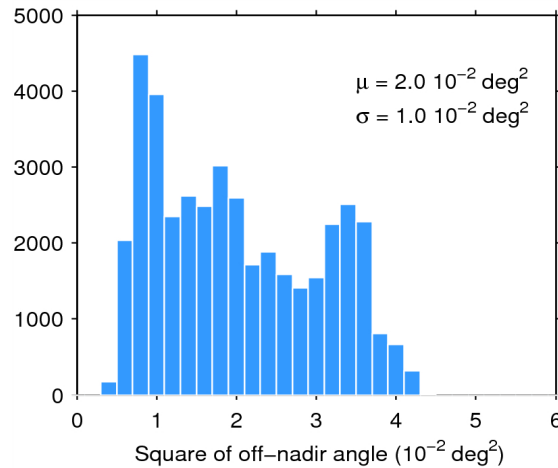
Figure 39. Histogram of flag-valid mispointing over oceans and lakes for 16/08/2015. The mean ( \mu ) and standard deviation ( \sigma ) are also shown. Note that values larger than 6 \cdot 10^{-2} \text{ deg}^2 are excluded from the histogram for the sake of readability but not from the computation of \mu and \sigma .
