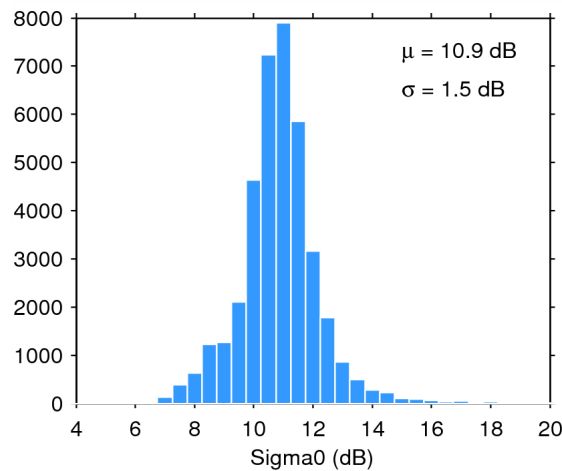
Figure 28. Histogram of science-valid sigma0 over oceans and lakes for 16/08/2015. The mean ( \mu ) and standard deviation ( \sigma ) are also shown. Note that values outside [4 20] dB are excluded from the histogram for the sake of readability but not from the computation of \mu and \sigma .
