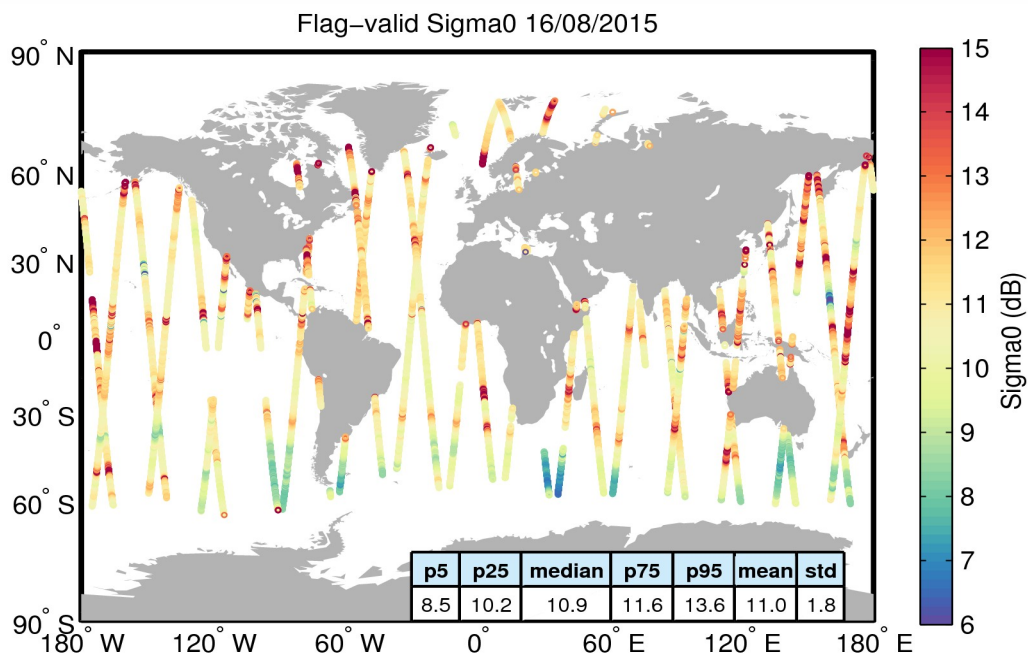
Figure 23. Geographical distribution of flag-valid sigma0 data over oceans and lakes for 16/08/2015. The statistical values shown in the table refer to the sigma0 in dB and are calculated over all measurements shown in the figure.
