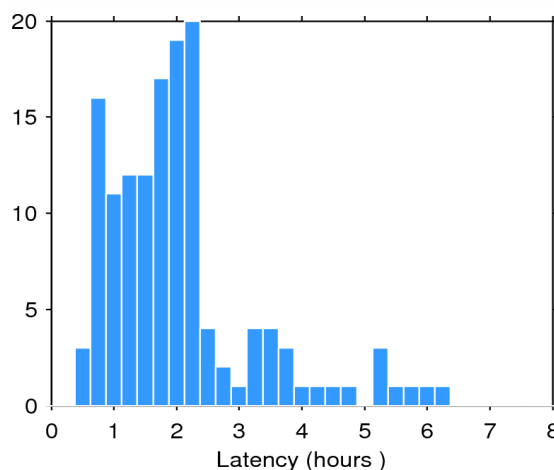
Figure 2. Histogram of the data latency for 16/08/2015. The y-axis denotes the number of files that are made available with a delay of x-hours with respect to the mean time of the records stored in the file.
