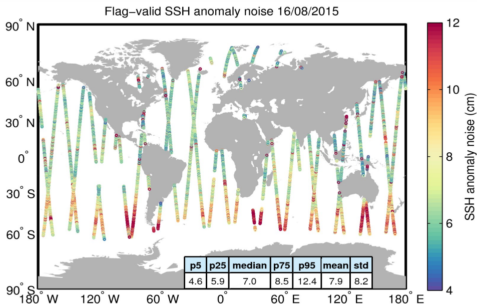
Figure 8. Geographical distribution of flag-valid 20-Hz SSH anomaly measurement noise over oceans and lakes for 16/08/2015. The statistical values shown in the table refer to the SSH anomaly noise and are calculated over all measurements shown in the figure.
