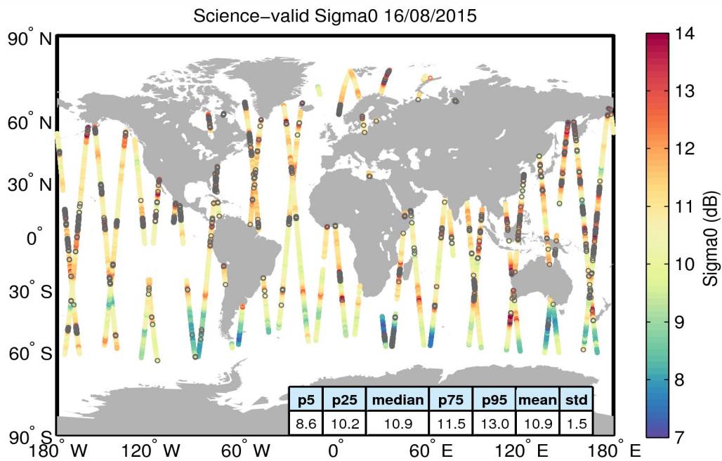
Figure 27. Geographical distribution of science-valid sigma0 data over oceans and lakes for 16/08/2015. The statistical values shown in the table refer to the sigma0 in dB and are calculated over all measurements shown in the figure. Gray circles denote records that have been rejected based on the editing criteria described in Table 4.
