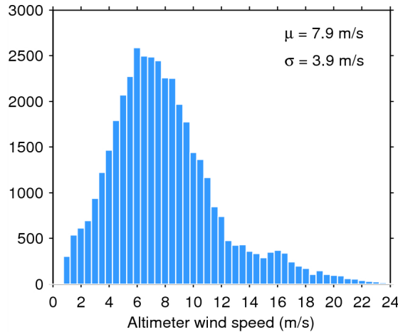
Figure 33. Histogram of flag-valid wind over oceans and lakes for 16/08/2015. The mean ( \mu ) and standard deviation ( \sigma ) are also shown. Note that values larger than 24 m/s are excluded from the histogram for the sake of readability but not from the computation of \mu and \sigma .
