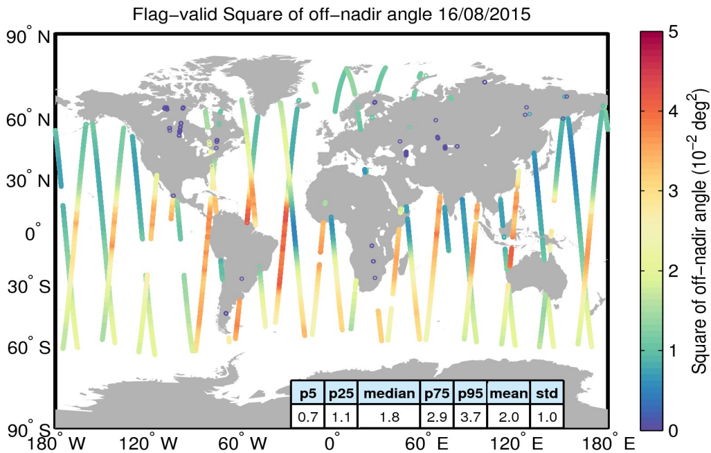
Figure 37. Geographical distribution of flag-valid mispointing data over oceans and lakes for 16/08/2015. The statistical values shown in the table refer to the mispointing in 10^{-2} \text{deg}^2 and are calculated over all measurements shown in the figure.
