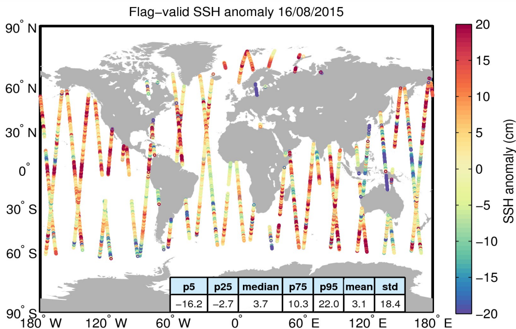
Figure 5. Geographical distribution of flag-valid 1-Hz SSH anomaly data over oceans and lakes for 16/08/2015. The statistical values shown in the table refer to the SSH anomaly in cm and are calculated over all measurements shown in the figure.
