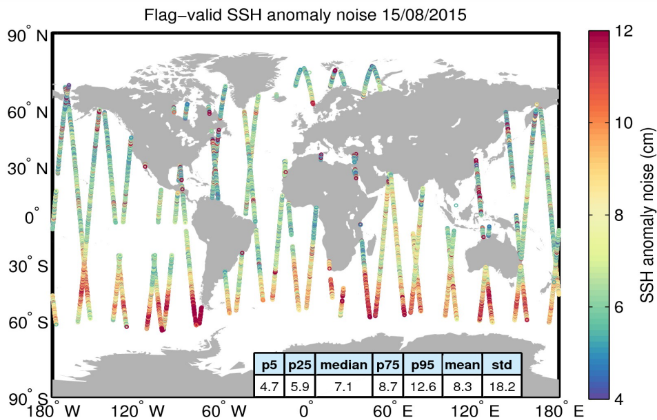
Figure 8. Geographical distribution of flag-valid 20-Hz SSH anomaly measurement noise over oceans and lakes for 15/08/2015. The statistical values shown in the table refer to the SSH anomaly noise and are calculated over all measurements shown in the figure.
