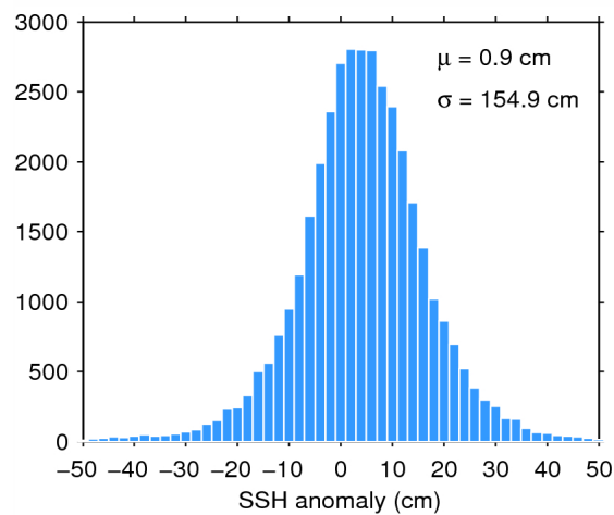
Figure 7. Histogram of flag-valid SSH anomaly over oceans and lakes for 15/08/2015. The mean ( \mu ) and standard deviation ( \sigma ) are also shown. Note that values outside [-50 50] cm are excluded from the histogram for the sake of readability but not from the computation of \mu and \sigma .
