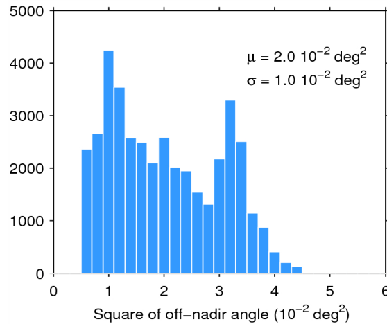
Figure 39. Histogram of flag-valid mispointing over oceans and lakes for 15/08/2015. The mean ( \mu ) and standard deviation ( \sigma ) are also shown. Note that values larger than 6 \cdot 10^{-2} \text{ deg}^2 are excluded from the histogram for the sake of readability but not from the computation of \mu and \sigma .
