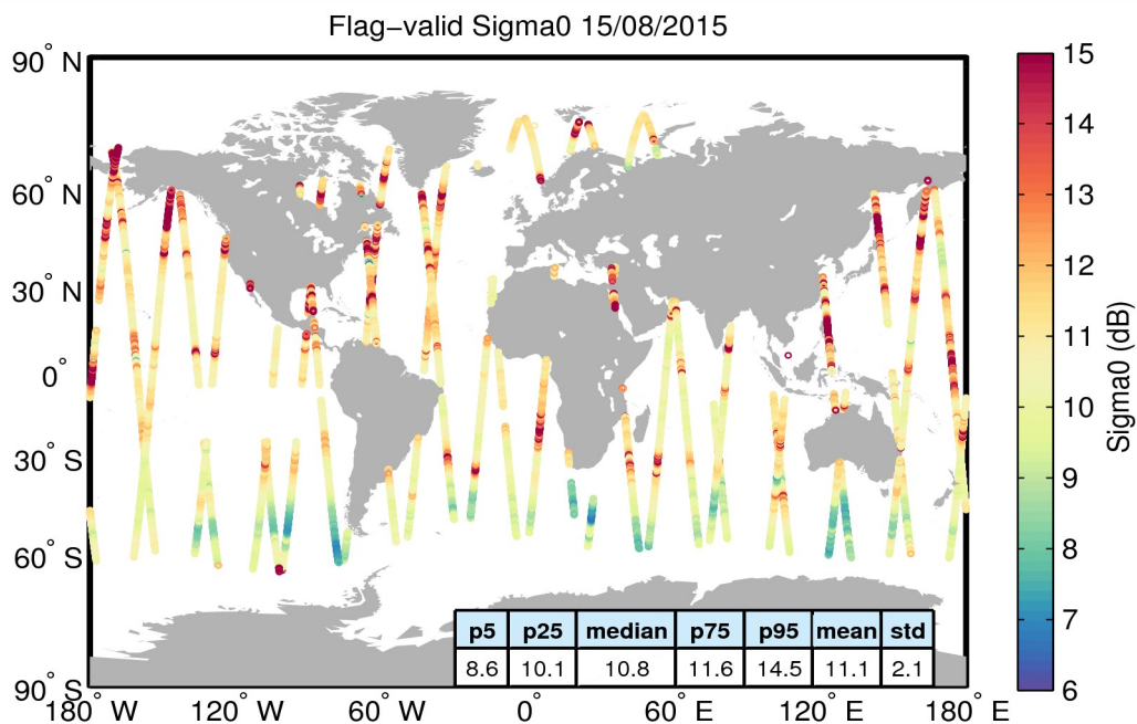
Figure 23. Geographical distribution of flag-valid sigma0 data over oceans and lakes for 15/08/2015. The statistical values shown in the table refer to the sigma0 in dB and are calculated over all measurements shown in the figure.
