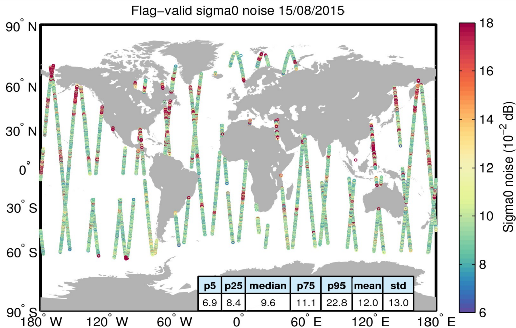
Figure 26. Geographical distribution of flag-valid 20-Hz sigma0 measurement noise over oceans and lakes for 15/08/2015. The statistical values shown in the table refer to the sigma0 noise and are calculated over all measurements shown in the figure.
