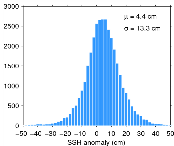
Figure 11. Histogram of science-valid SSH anomaly over oceans and lakes for 15/08/2015. The mean ( \mu ) and standard deviation ( \sigma ) are also shown. Note that values outside [-50 50] cm are excluded from the histogram for the sake of readability but not from the computation of \mu and \sigma .
