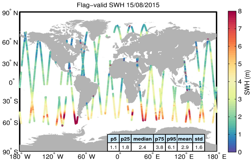
Figure 15. Geographical distribution of flag-valid SWH data over oceans and lakes for 15/08/2015. The statistical values shown in the table refer to the SWH in m and are calculated over all measurements shown in the figure.
