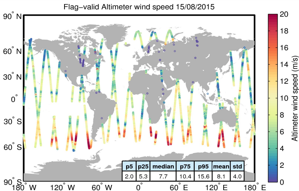
Figure 31. Geographical distribution of flag-valid wind data over oceans and lakes for 15/08/2015. The statistical values shown in the table refer to the wind in m/s and are calculated over all measurements shown in the figure.
