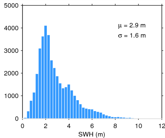
Figure 20. Histogram of science-valid SWH over oceans and lakes for 15/08/2015. The mean ( \mu ) and standard deviation ( \sigma ) are also shown. Note that values larger than 12 m are excluded from the histogram for the sake of readability but not from the computation of \mu and \sigma .
