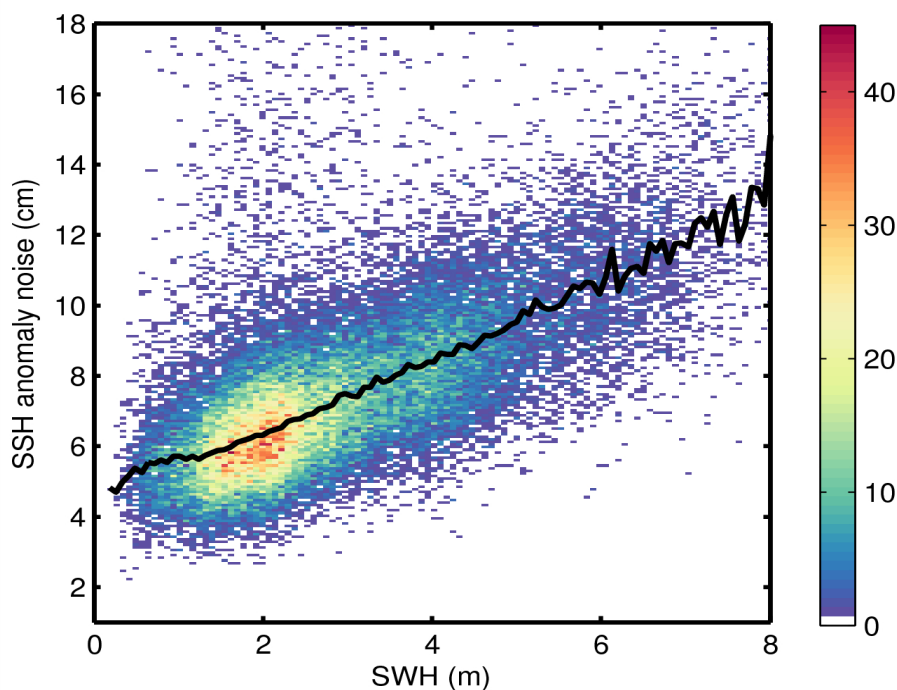
Figure 9. 2D histogram showing flag-valid SSH anomaly noise as a function of SWH for 15/08/2015. The black line denotes the median SSH anomaly as a function of SWH.
