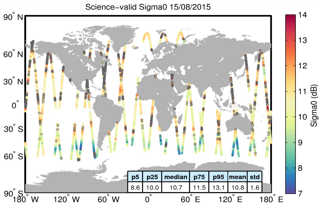
Figure 27. Geographical distribution of science-valid sigma0 data over oceans and lakes for 15/08/2015. The statistical values shown in the table refer to the sigma0 in dB and are calculated over all measurements shown in the figure. Gray circles denote records that have been rejected based on the editing criteria described in Table 4.
