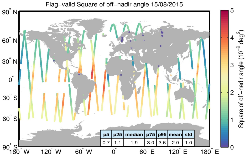
Figure 37. Geographical distribution of flag-valid mispointing data over oceans and lakes for 15/08/2015. The statistical values shown in the table refer to the mispointing in 10^{-2} deg 2 and are calculated over all measurements shown in the figure.
