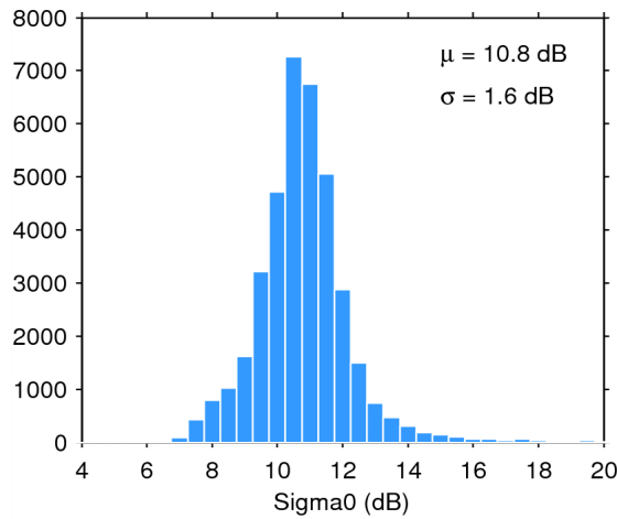
Figure 28. Histogram of science-valid sigma0 over oceans and lakes for 15/08/2015. The mean ( \mu ) and standard deviation ( \sigma ) are also shown. Note that values outside [4 20] dB are excluded from the histogram for the sake of readability but not from the computation of \mu and \sigma .
