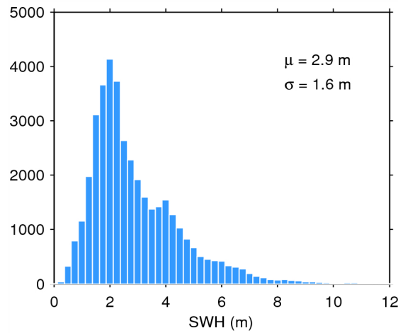
Figure 17. Histogram of flag-valid SWH over oceans and lakes for 15/08/2015. The mean ( \mu ) and standard deviation ( \sigma ) are also shown. Note that values larger than 12 m are excluded from the histogram for the sake of readability but not from the computation of \mu and \sigma .
