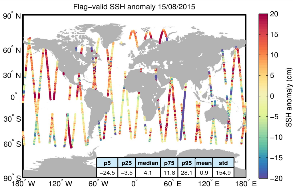
Figure 5. Geographical distribution of flag-valid 1-Hz SSH anomaly data over oceans and lakes for 15/08/2015. The statistical values shown in the table refer to the SSH anomaly in cm and are calculated over all measurements shown in the figure.
