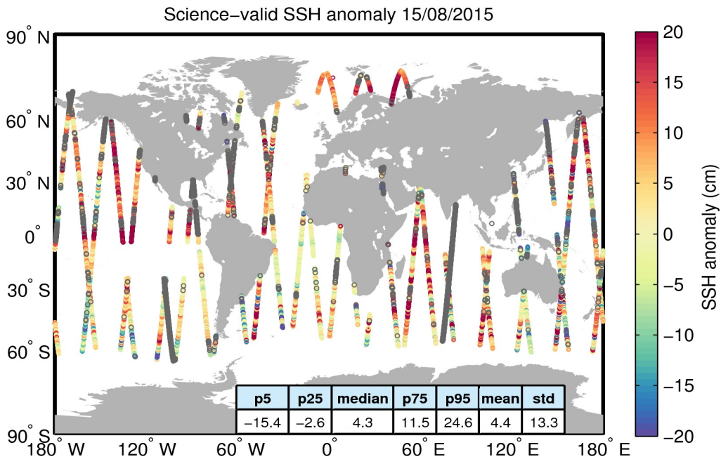
Figure 10. Geographical distribution of science-valid SSH anomaly data over oceans and lakes for 15/08/2015. The statistical values shown in the table refer to the SSH anomaly in cm and are calculated over all measurements shown in the figure. Gray circles denote records that have been rejected based on the editing criteria described in Table 2.
