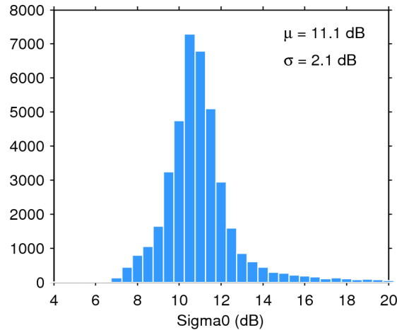
Figure 25. Histogram of flag-valid sigma0 over oceans and lakes for 15/08/2015. The mean ( \mu ) and standard deviation ( \sigma ) are also shown. Note that values outside [4 20] dB are excluded from the histogram for the sake of readability but not from the computation of \mu and \sigma .
