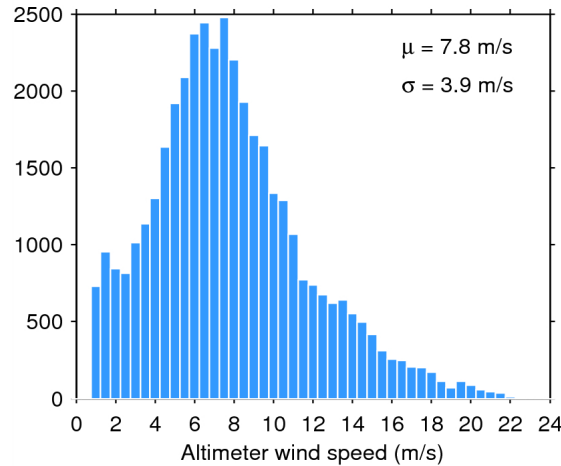
Figure 33. Histogram of flag-valid wind over oceans and lakes for 14/08/2015. The mean ( \mu ) and standard deviation ( \sigma ) are also shown. Note that values larger than 24 m/s are excluded from the histogram for the sake of readability but not from the computation of \mu and \sigma .
