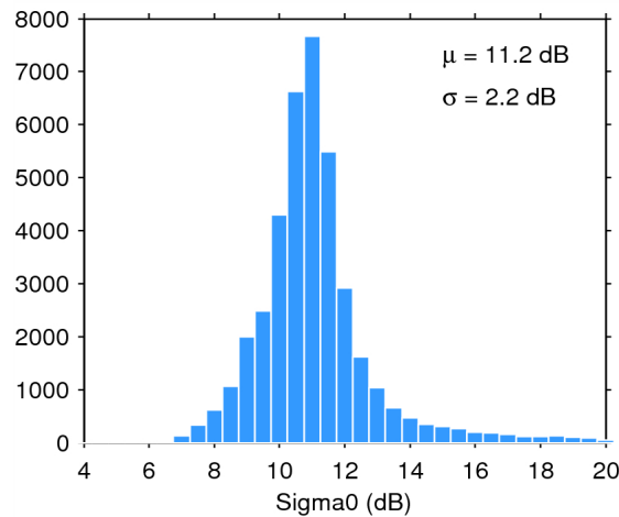
Figure 25. Histogram of flag-valid sigma0 over oceans and lakes for 14/08/2015. The mean ( \mu ) and standard deviation ( \sigma ) are also shown. Note that values outside [4 20] dB are excluded from the histogram for the sake of readability but not from the computation of \mu and \sigma .
