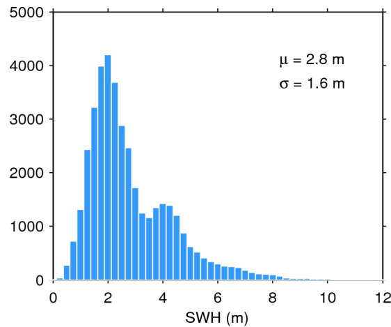
Figure 17. Histogram of flag-valid SWH over oceans and lakes for 14/08/2015. The mean ( \mu ) and standard deviation ( \sigma ) are also shown. Note that values larger than 12 m are excluded from the histogram for the sake of readability but not from the computation of \mu and \sigma .
