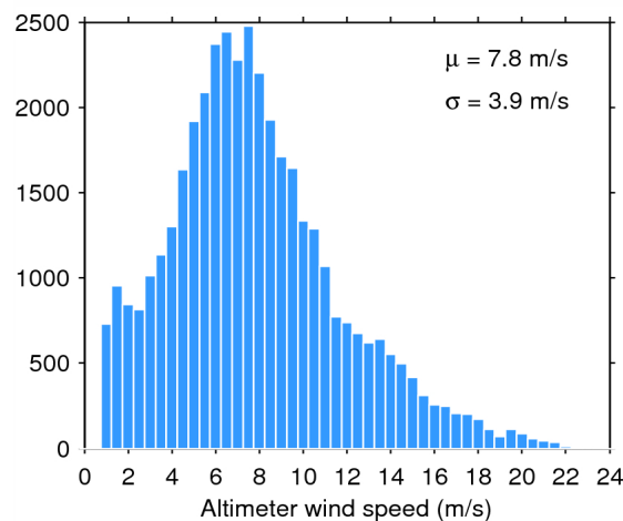
Figure 35. Histogram of science-valid wind over oceans and lakes for 14/08/2015. The mean ( \mu ) and standard deviation ( \sigma ) are also shown. Note that values larger than 24 m/s are excluded from the histogram for the sake of readability but not from the computation of \mu and \sigma .
