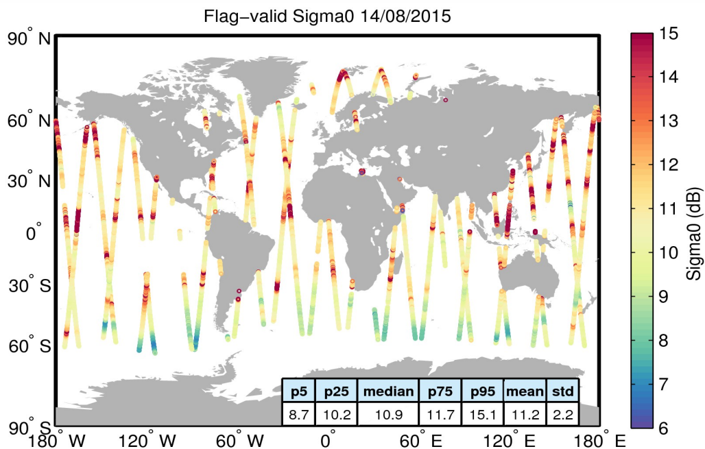
Figure 23. Geographical distribution of flag-valid sigma0 data over oceans and lakes for 14/08/2015. The statistical values shown in the table refer to the sigma0 in dB and are calculated over all measurements shown in the figure.
