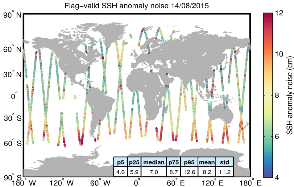
Figure 8. Geographical distribution of flag-valid 20-Hz SSH anomaly measurement noise over oceans and lakes for 14/08/2015. The statistical values shown in the table refer to the SSH anomaly noise and are calculated over all measurements shown in the figure.
