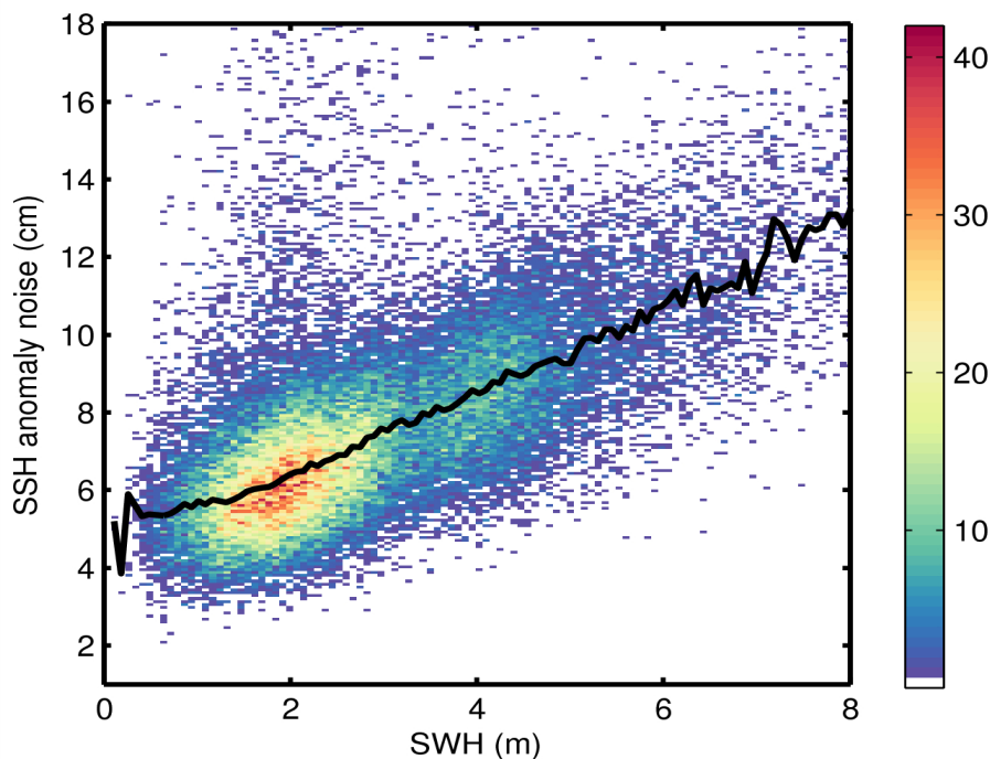
Figure 9. 2D histogram showing flag-valid SSH anomaly noise as a function of SWH for 14/08/2015. The black line denotes the median SSH anomaly as a function of SWH.
