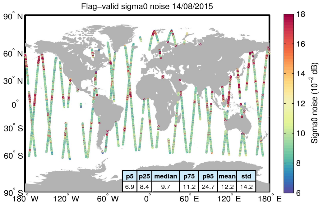
Figure 26. Geographical distribution of flag-valid 20-Hz sigma0 measurement noise over oceans and lakes for 14/08/2015. The statistical values shown in the table refer to the sigma0 noise and are calculated over all measurements shown in the figure.
