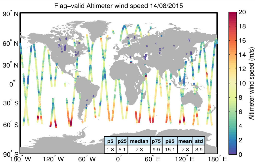
Figure 31. Geographical distribution of flag-valid wind data over oceans and lakes for 14/08/2015. The statistical values shown in the table refer to the wind in m/s and are calculated over all measurements shown in the figure.
