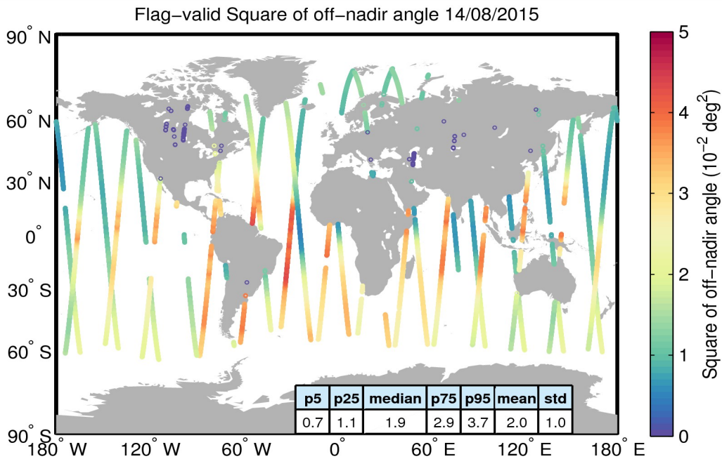
Figure 37. Geographical distribution of flag-valid mispointing data over oceans and lakes for 14/08/2015. The statistical values shown in the table refer to the mispointing in 10^{-2} \text{ deg}^2 and are calculated over all measurements shown in the figure.
