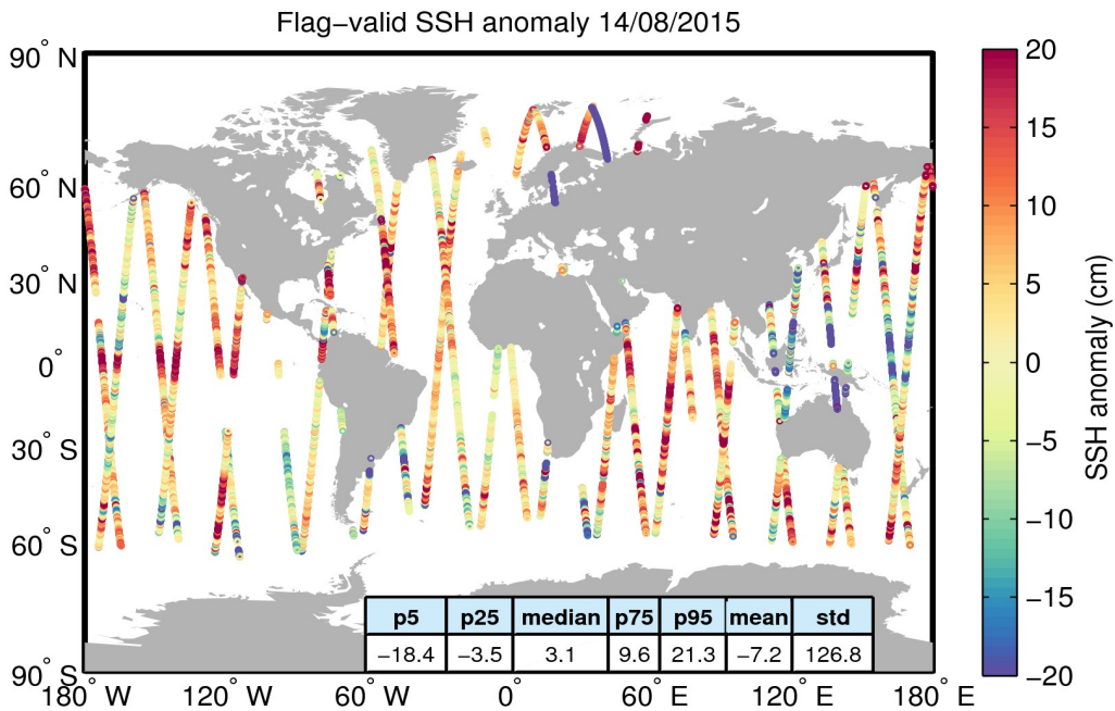
Figure 5. Geographical distribution of flag-valid 1-Hz SSH anomaly data over oceans and lakes for 14/08/2015. The statistical values shown in the table refer to the SSH anomaly in cm and are calculated over all measurements shown in the figure.
