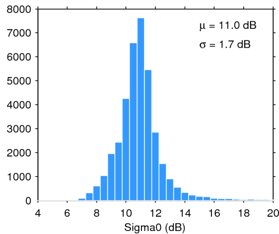
Figure 28. Histogram of science-valid sigma0 over oceans and lakes for 14/08/2015. The mean ( \mu ) and standard deviation ( \sigma ) are also shown. Note that values outside [4 20] dB are excluded from the histogram for the sake of readability but not from the computation of \mu and \sigma .
