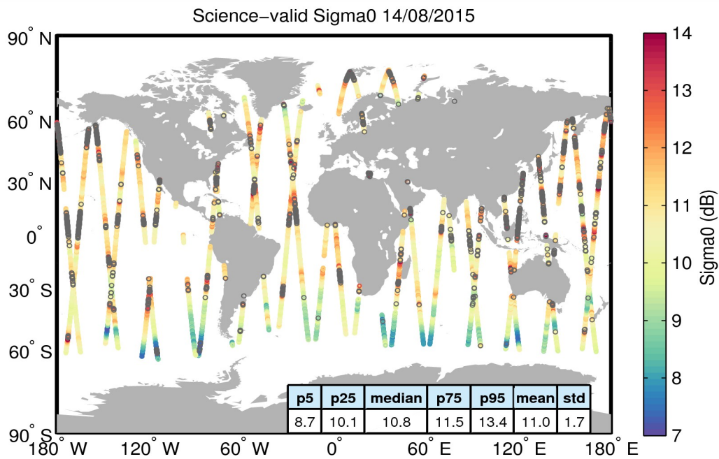
Figure 27. Geographical distribution of science-valid sigma0 data over oceans and lakes for 14/08/2015. The statistical values shown in the table refer to the sigma0 in dB and are calculated over all measurements shown in the figure. Gray circles denote records that have been rejected based on the editing criteria described in Table 4.
