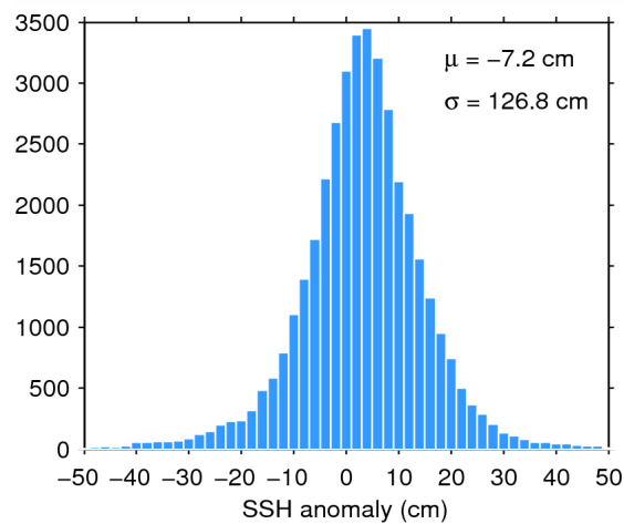
Figure 7. Histogram of flag-valid SSH anomaly over oceans and lakes for 14/08/2015. The mean ( \mu ) and standard deviation ( \sigma ) are also shown. Note that values outside [-50 50] cm are excluded from the histogram for the sake of readability but not from the computation of \mu and \sigma .
