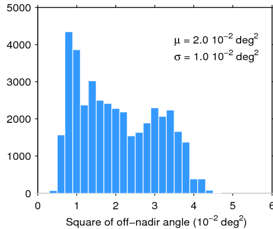
Figure 39. Histogram of flag-valid mispointing over oceans and lakes for 14/08/2015. The mean ( \mu ) and standard deviation ( \sigma ) are also shown. Note that values larger than 6 \cdot 10^{-2} \text{ deg}^2 are excluded from the histogram for the sake of readability but not from the computation of \mu and \sigma .
