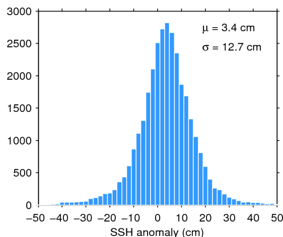
Figure 11. Histogram of science-valid SSH anomaly over oceans and lakes for 14/08/2015. The mean ( \mu ) and standard deviation ( \sigma ) are also shown. Note that values outside [-50 50] cm are excluded from the histogram for the sake of readability but not from the computation of \mu and \sigma .
