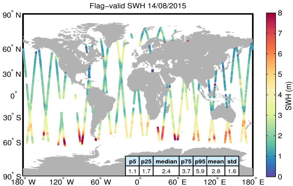
Figure 15. Geographical distribution of flag-valid SWH data over oceans and lakes for 14/08/2015. The statistical values shown in the table refer to the SWH in m and are calculated over all measurements shown in the figure.
