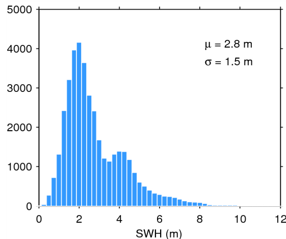
Figure 20. Histogram of science-valid SWH over oceans and lakes for 14/08/2015. The mean ( \mu ) and standard deviation ( \sigma ) are also shown. Note that values larger than 12 m are excluded from the histogram for the sake of readability but not from the computation of \mu and \sigma .
