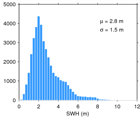
Figure 17. Histogram of flag-valid SWH over oceans and lakes for 13/08/2015. The mean ( \mu ) and standard deviation ( \sigma ) are also shown. Note that values larger than 12 m are excluded from the histogram for the sake of readability but not from the computation of \mu and \sigma .
