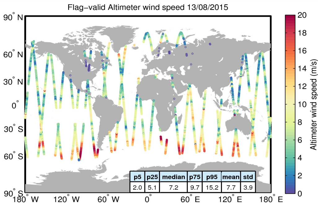
Figure 31. Geographical distribution of flag-valid wind data over oceans and lakes for 13/08/2015. The statistical values shown in the table refer to the wind in m/s and are calculated over all measurements shown in the figure.
