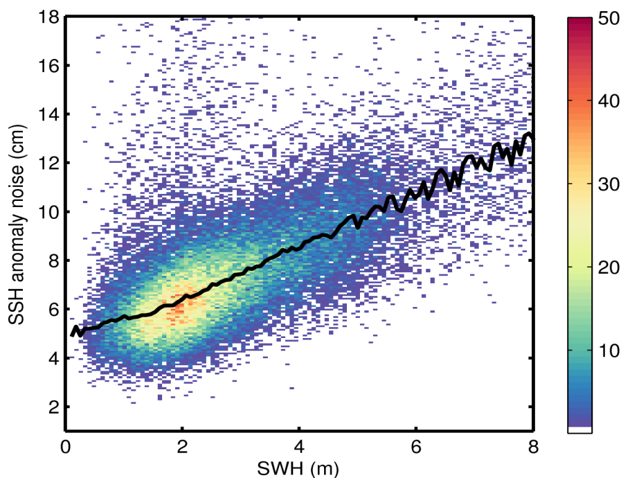
Figure 9. 2D histogram showing flag-valid SSH anomaly noise as a function of SWH for 13/08/2015. The black line denotes the median SSH anomaly as a function of SWH.
