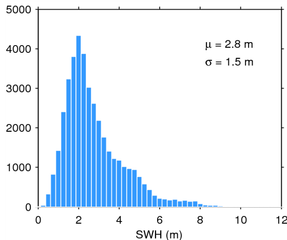
Figure 20. Histogram of science-valid SWH over oceans and lakes for 13/08/2015. The mean ( \mu ) and standard deviation ( \sigma ) are also shown. Note that values larger than 12 m are excluded from the histogram for the sake of readability but not from the computation of \mu and \sigma .
