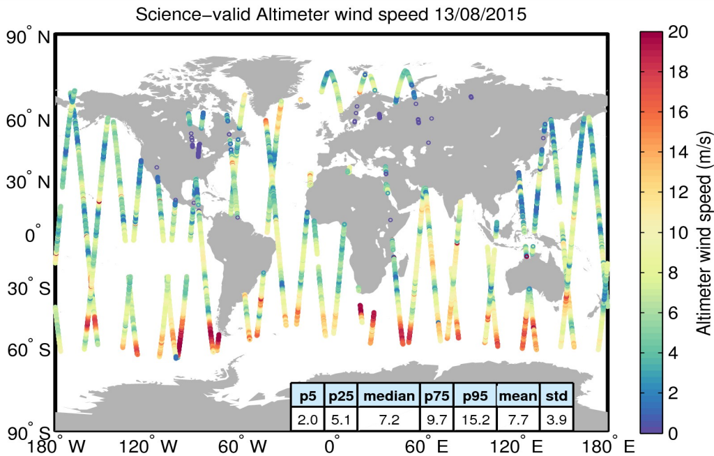
Figure 34. Geographical distribution of science-valid wind data over oceans and lakes for 13/08/2015. The statistical values shown in the table refer to the wind in m/s and are calculated over all measurements shown in the figure. Gray circles denote records that have been rejected based on the editing criteria described in Table 5.
