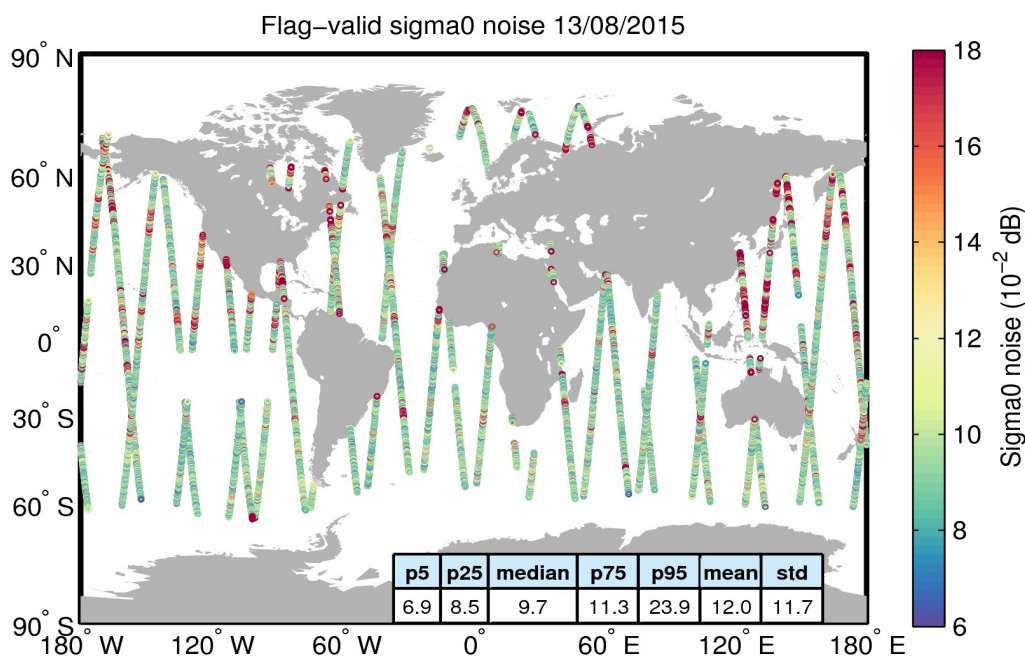
Figure 26. Geographical distribution of flag-valid 20-Hz sigma0 measurement noise over oceans and lakes for 13/08/2015. The statistical values shown in the table refer to the sigma0 noise and are calculated over all measurements shown in the figure.
