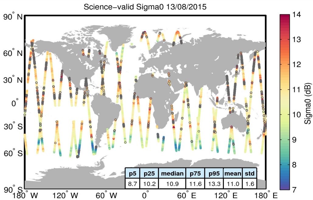
Figure 27. Geographical distribution of science-valid sigma0 data over oceans and lakes for 13/08/2015. The statistical values shown in the table refer to the sigma0 in dB and are calculated over all measurements shown in the figure. Gray circles denote records that have been rejected based on the editing criteria described in Table 4.
