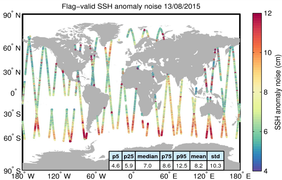
Figure 8. Geographical distribution of flag-valid 20-Hz SSH anomaly measurement noise over oceans and lakes for 13/08/2015. The statistical values shown in the table refer to the SSH anomaly noise and are calculated over all measurements shown in the figure.
