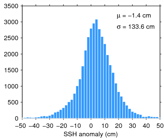
Figure 7. Histogram of flag-valid SSH anomaly over oceans and lakes for 13/08/2015. The mean ( \mu ) and standard deviation ( \sigma ) are also shown. Note that values outside [-50 50] cm are excluded from the histogram for the sake of readability but not from the computation of \mu and \sigma .
