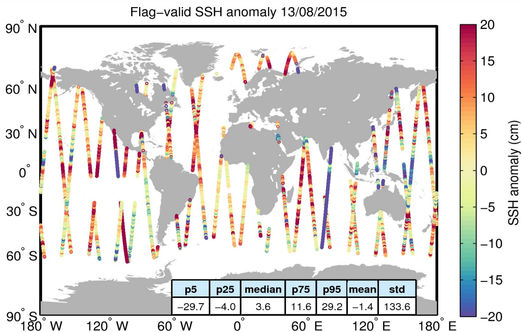
Figure 5. Geographical distribution of flag-valid 1-Hz SSH anomaly data over oceans and lakes for 13/08/2015. The statistical values shown in the table refer to the SSH anomaly in cm and are calculated over all measurements shown in the figure.
