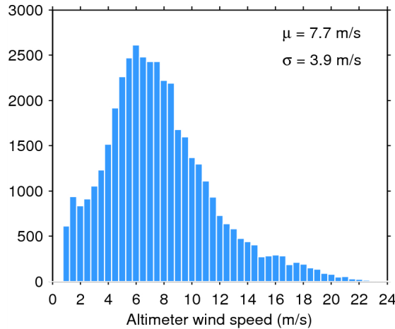
Figure 33. Histogram of flag-valid wind over oceans and lakes for 13/08/2015. The mean ( \mu ) and standard deviation ( \sigma ) are also shown. Note that values larger than 24 m/s are excluded from the histogram for the sake of readability but not from the computation of \mu and \sigma .
