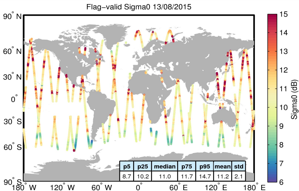
Figure 23. Geographical distribution of flag-valid sigma0 data over oceans and lakes for 13/08/2015. The statistical values shown in the table refer to the sigma0 in dB and are calculated over all measurements shown in the figure.
