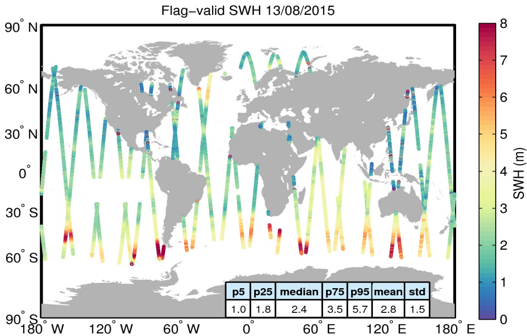
Figure 15. Geographical distribution of flag-valid SWH data over oceans and lakes for 13/08/2015. The statistical values shown in the table refer to the SWH in m and are calculated over all measurements shown in the figure.
