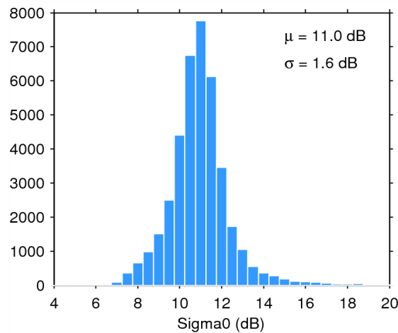
Figure 28. Histogram of science-valid sigma0 over oceans and lakes for 13/08/2015. The mean ( \mu ) and standard deviation ( \sigma ) are also shown. Note that values outside [4 20] dB are excluded from the histogram for the sake of readability but not from the computation of \mu and \sigma .
