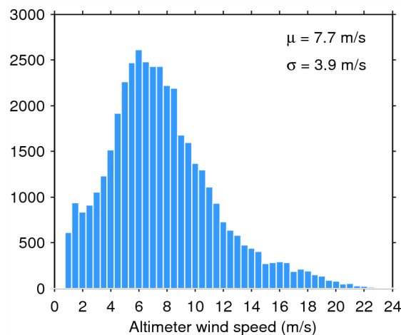
Figure 35. Histogram of science-valid wind over oceans and lakes for 13/08/2015. The mean ( \mu ) and standard deviation ( \sigma ) are also shown. Note that values larger than 24 m/s are excluded from the histogram for the sake of readability but not from the computation of \mu and \sigma .
