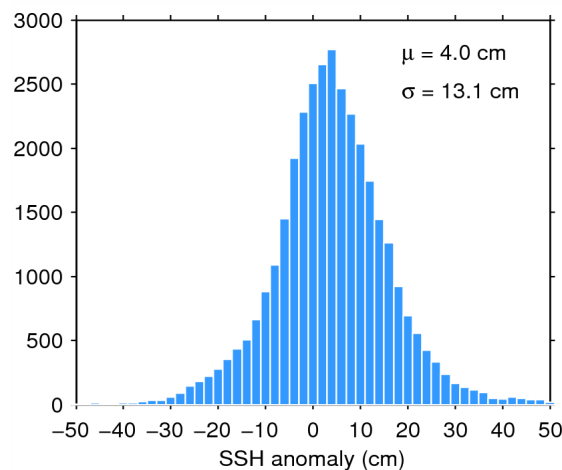
Figure 11. Histogram of science-valid SSH anomaly over oceans and lakes for 13/08/2015. The mean ( \mu ) and standard deviation ( \sigma ) are also shown. Note that values outside [-50 50] cm are excluded from the histogram for the sake of readability but not from the computation of \mu and \sigma .
