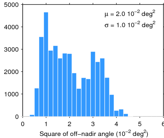
Figure 39. Histogram of flag-valid mispointing over oceans and lakes for 13/08/2015. The mean ( \mu ) and standard deviation ( \sigma ) are also shown. Note that values larger than 6 \cdot 10^{-2} \text{ deg}^2 are excluded from the histogram for the sake of readability but not from the computation of \mu and \sigma .
