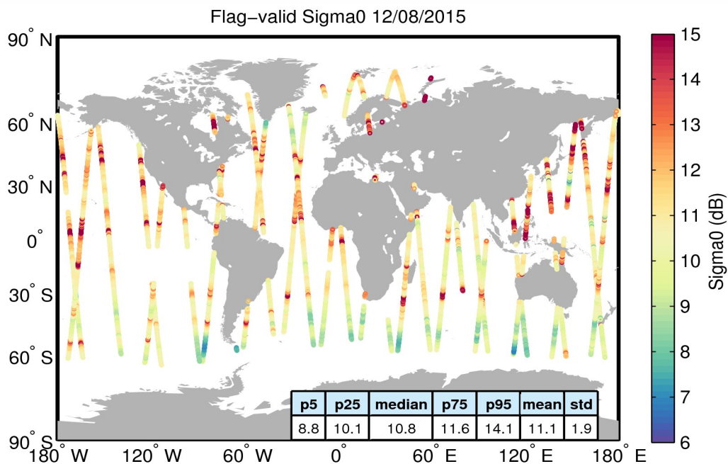
Figure 23. Geographical distribution of flag-valid sigma0 data over oceans and lakes for 12/08/2015. The statistical values shown in the table refer to the sigma0 in dB and are calculated over all measurements shown in the figure.
