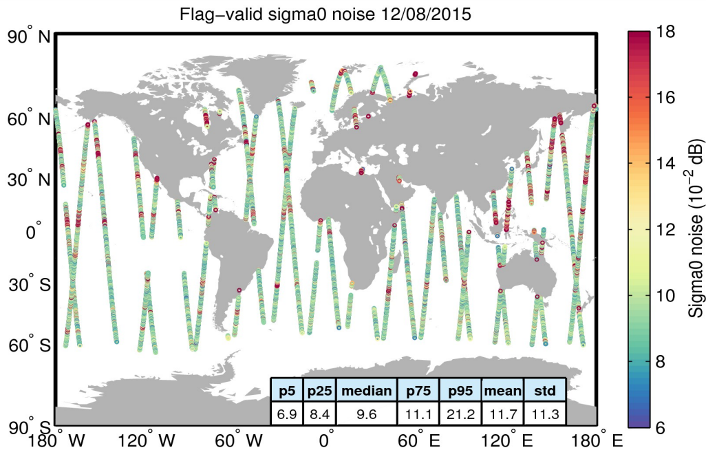
Figure 26. Geographical distribution of flag-valid 20-Hz sigma0 measurement noise over oceans and lakes for 12/08/2015. The statistical values shown in the table refer to the sigma0 noise and are calculated over all measurements shown in the figure.
