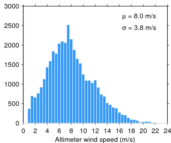
Figure 35. Histogram of science-valid wind over oceans and lakes for 12/08/2015. The mean ( \mu ) and standard deviation ( \sigma ) are also shown. Note that values larger than 24 m/s are excluded from the histogram for the sake of readability but not from the computation of \mu and \sigma .
