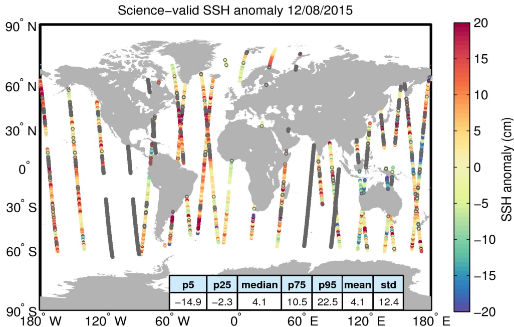
Figure 10. Geographical distribution of science-valid SSH anomaly data over oceans and lakes for 12/08/2015. The statistical values shown in the table refer to the SSH anomaly in cm and are calculated over all measurements shown in the figure. Gray circles denote records that have been rejected based on the editing criteria described in Table 2.
