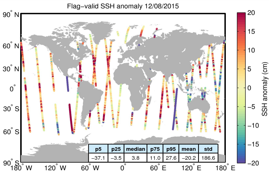
Figure 5. Geographical distribution of flag-valid 1-Hz SSH anomaly data over oceans and lakes for 12/08/2015. The statistical values shown in the table refer to the SSH anomaly in cm and are calculated over all measurements shown in the figure.
