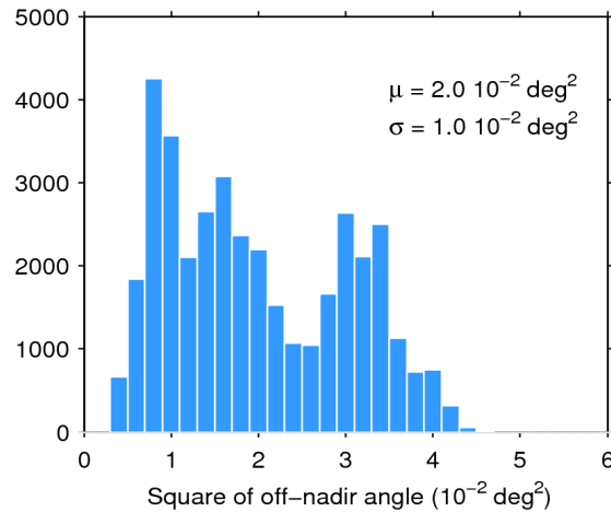
Figure 39. Histogram of flag-valid mispointing over oceans and lakes for 12/08/2015. The mean ( \mu ) and standard deviation ( \sigma ) are also shown. Note that values larger than 6 \cdot 10^{-2} \text{ deg}^2 are excluded from the histogram for the sake of readability but not from the computation of \mu and \sigma .
