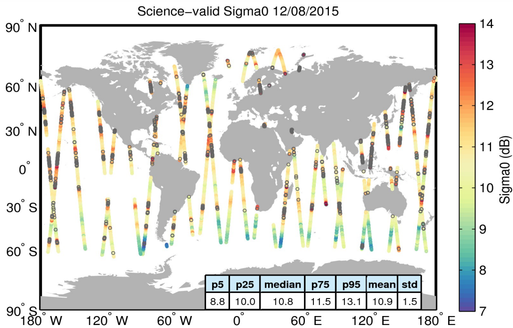
Figure 27. Geographical distribution of science-valid sigma0 data over oceans and lakes for 12/08/2015. The statistical values shown in the table refer to the sigma0 in dB and are calculated over all measurements shown in the figure. Gray circles denote records that have been rejected based on the editing criteria described in Table 4.
