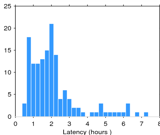
Figure 2. Histogram of the data latency for 12/08/2015. The y-axis denotes the number of files that are made available with a delay of x-hours with respect to the mean time of the records stored in the file.
