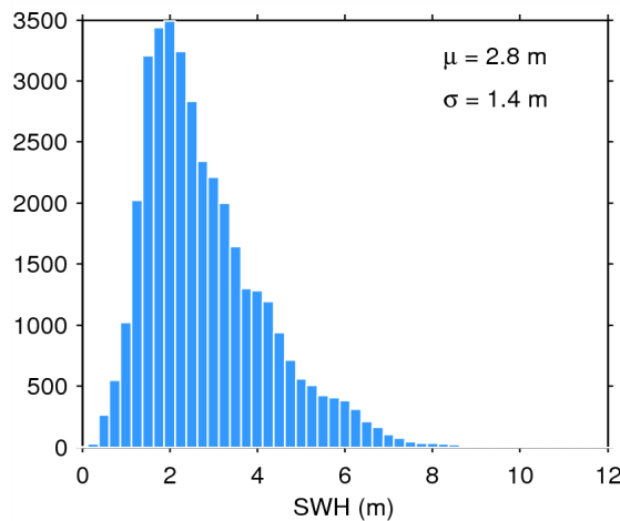
Figure 20. Histogram of science-valid SWH over oceans and lakes for 12/08/2015. The mean ( \mu ) and standard deviation ( \sigma ) are also shown. Note that values larger than 12 m are excluded from the histogram for the sake of readability but not from the computation of \mu and \sigma .
