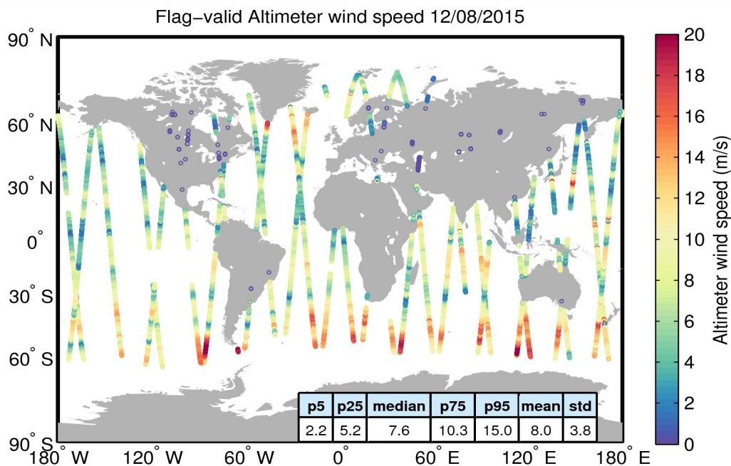
Figure 31. Geographical distribution of flag-valid wind data over oceans and lakes for 12/08/2015. The statistical values shown in the table refer to the wind in m/s and are calculated over all measurements shown in the figure.
