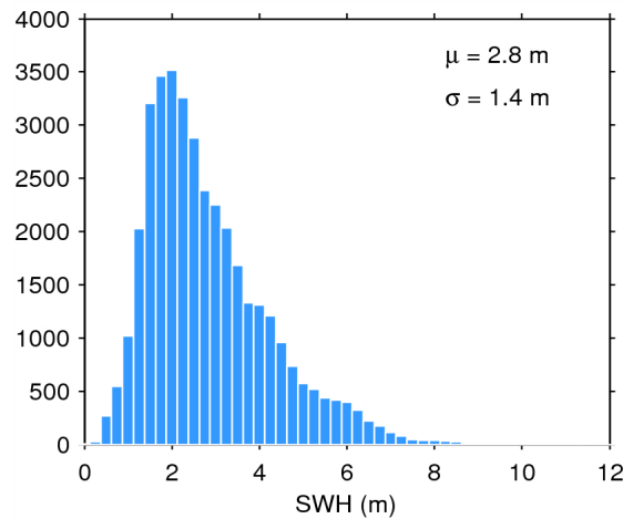
Figure 17. Histogram of flag-valid SWH over oceans and lakes for 12/08/2015. The mean ( \mu ) and standard deviation ( \sigma ) are also shown. Note that values larger than 12 m are excluded from the histogram for the sake of readability but not from the computation of \mu and \sigma .
