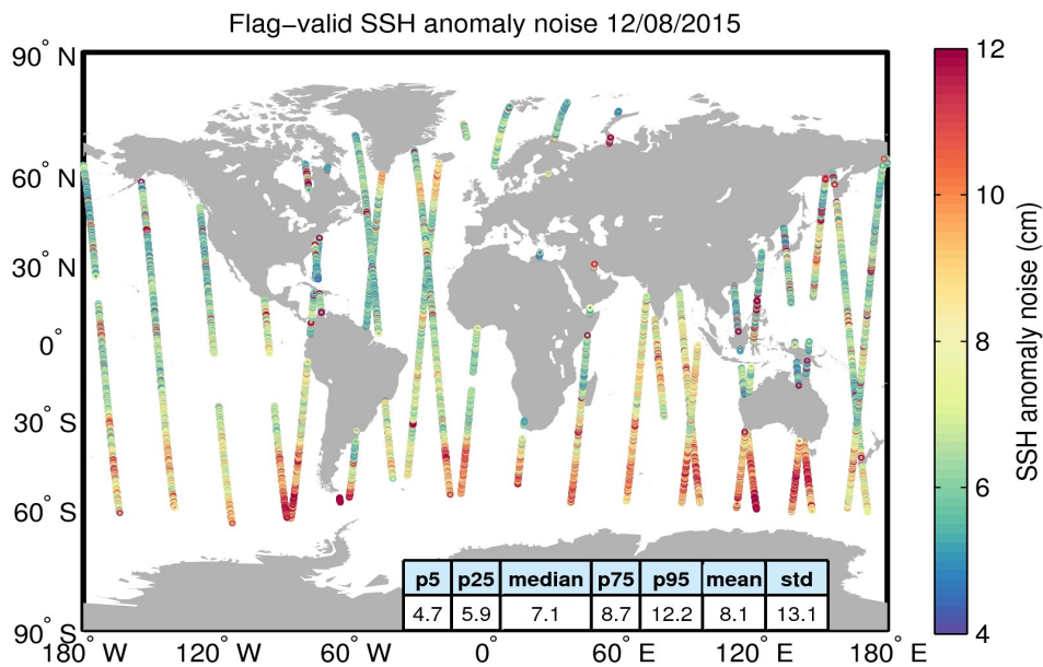
Figure 8. Geographical distribution of flag-valid 20-Hz SSH anomaly measurement noise over oceans and lakes for 12/08/2015. The statistical values shown in the table refer to the SSH anomaly noise and are calculated over all measurements shown in the figure.
