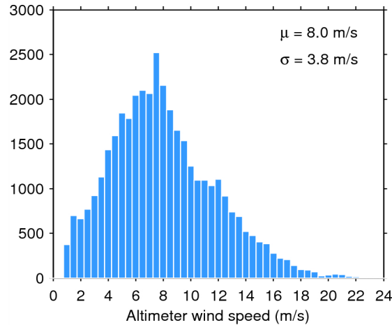
Figure 33. Histogram of flag-valid wind over oceans and lakes for 12/08/2015. The mean ( \mu ) and standard deviation ( \sigma ) are also shown. Note that values larger than 24 m/s are excluded from the histogram for the sake of readability but not from the computation of \mu and \sigma .
