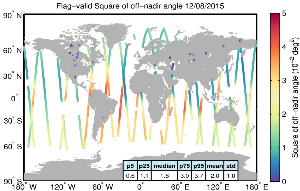
Figure 37. Geographical distribution of flag-valid mispointing data over oceans and lakes for 12/08/2015. The statistical values shown in the table refer to the mispointing in 10^{-2} deg 2 and are calculated over all measurements shown in the figure.
