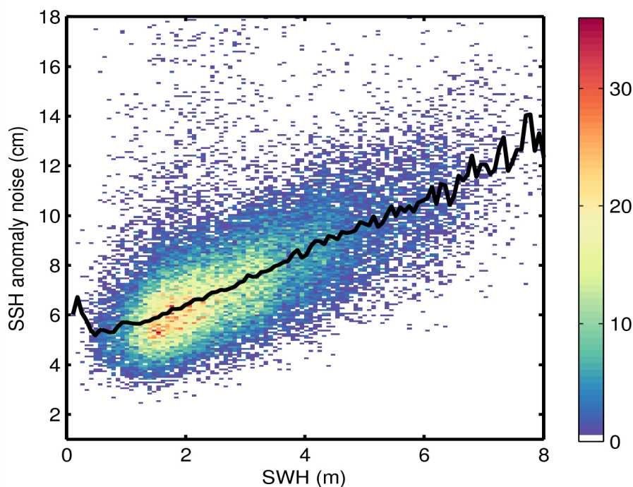
Figure 9. 2D histogram showing flag-valid SSH anomaly noise as a function of SWH for 12/08/2015. The black line denotes the median SSH anomaly as a function of SWH.
