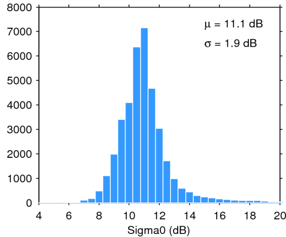
Figure 25. Histogram of flag-valid sigma0 over oceans and lakes for 12/08/2015. The mean ( \mu ) and standard deviation ( \sigma ) are also shown. Note that values outside [4 20] dB are excluded from the histogram for the sake of readability but not from the computation of \mu and \sigma .
