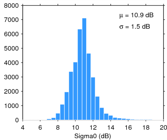
Figure 28. Histogram of science-valid sigma0 over oceans and lakes for 12/08/2015. The mean ( \mu ) and standard deviation ( \sigma ) are also shown. Note that values outside [4 20] dB are excluded from the histogram for the sake of readability but not from the computation of \mu and \sigma .
