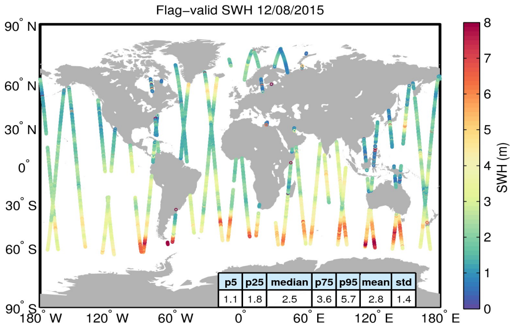
Figure 15. Geographical distribution of flag-valid SWH data over oceans and lakes for 12/08/2015. The statistical values shown in the table refer to the SWH in m and are calculated over all measurements shown in the figure.
