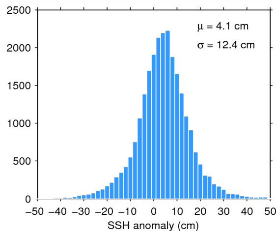
Figure 11. Histogram of science-valid SSH anomaly over oceans and lakes for 12/08/2015. The mean ( \mu ) and standard deviation ( \sigma ) are also shown. Note that values outside [-50 50] cm are excluded from the histogram for the sake of readability but not from the computation of \mu and \sigma .
