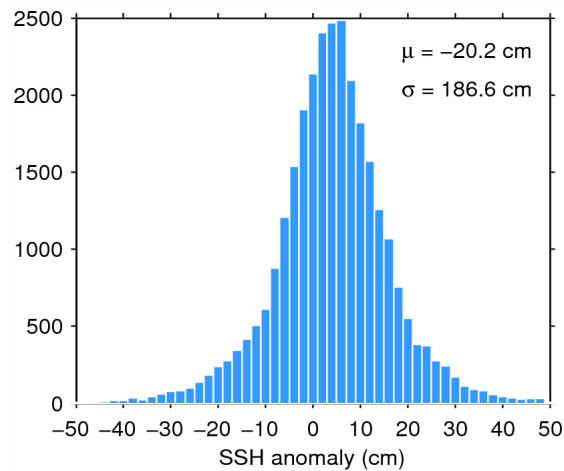
Figure 7. Histogram of flag-valid SSH anomaly over oceans and lakes for 12/08/2015. The mean ( \mu ) and standard deviation ( \sigma ) are also shown. Note that values outside [-50 50] cm are excluded from the histogram for the sake of readability but not from the computation of \mu and \sigma .
