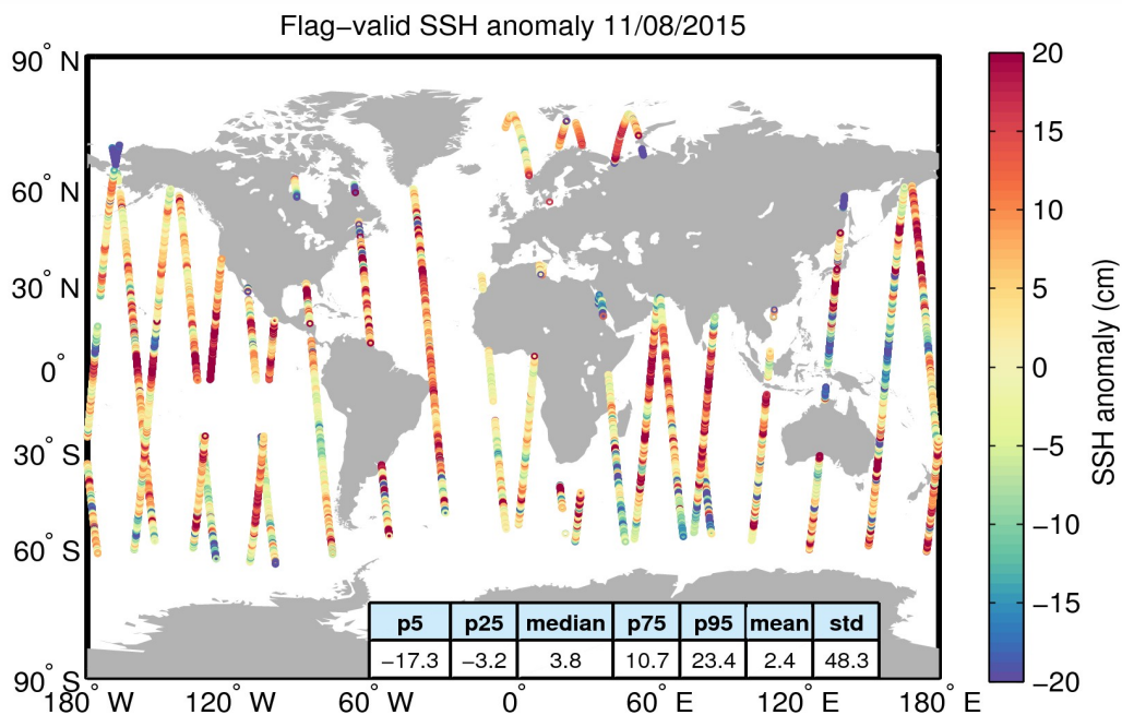
Figure 5. Geographical distribution of flag-valid 1-Hz SSH anomaly data over oceans and lakes for 11/08/2015. The statistical values shown in the table refer to the SSH anomaly in cm and are calculated over all measurements shown in the figure.
