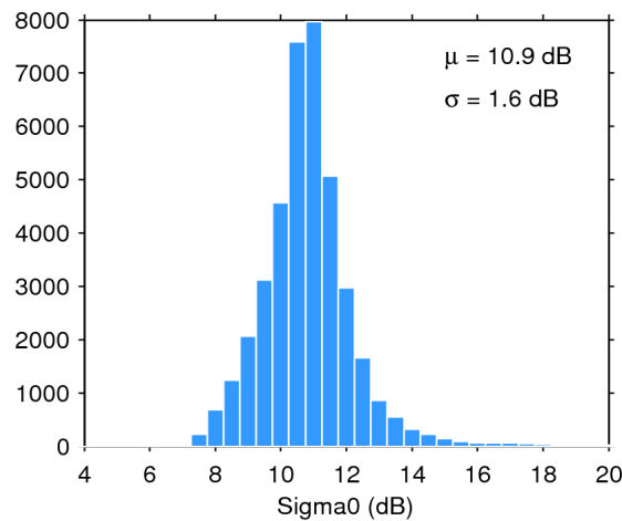
Figure 28. Histogram of science-valid sigma0 over oceans and lakes for 11/08/2015. The mean ( \mu ) and standard deviation ( \sigma ) are also shown. Note that values outside [4 20] dB are excluded from the histogram for the sake of readability but not from the computation of \mu and \sigma .
