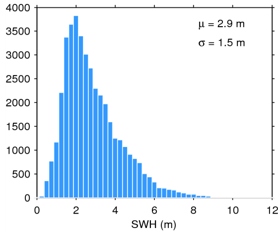
Figure 17. Histogram of flag-valid SWH over oceans and lakes for 11/08/2015. The mean ( \mu ) and standard deviation ( \sigma ) are also shown. Note that values larger than 12 m are excluded from the histogram for the sake of readability but not from the computation of \mu and \sigma .
