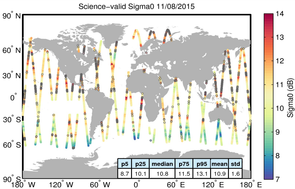
Figure 27. Geographical distribution of science-valid sigma0 data over oceans and lakes for 11/08/2015. The statistical values shown in the table refer to the sigma0 in dB and are calculated over all measurements shown in the figure. Gray circles denote records that have been rejected based on the editing criteria described in Table 4.
