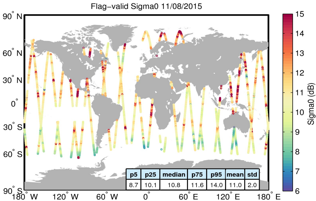
Figure 23. Geographical distribution of flag-valid sigma0 data over oceans and lakes for 11/08/2015. The statistical values shown in the table refer to the sigma0 in dB and are calculated over all measurements shown in the figure.
