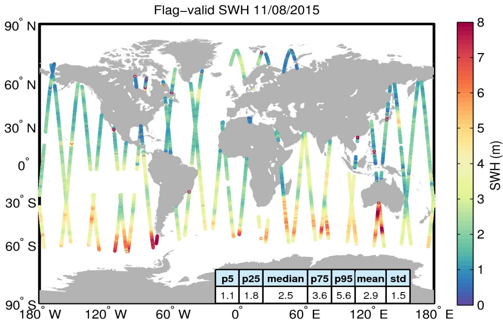
Figure 15. Geographical distribution of flag-valid SWH data over oceans and lakes for 11/08/2015. The statistical values shown in the table refer to the SWH in m and are calculated over all measurements shown in the figure.
