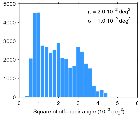
Figure 39. Histogram of flag-valid mispointing over oceans and lakes for 11/08/2015. The mean ( \mu ) and standard deviation ( \sigma ) are also shown. Note that values larger than 6 \cdot 10^{-2} \text{ deg}^2 are excluded from the histogram for the sake of readability but not from the computation of \mu and \sigma .
