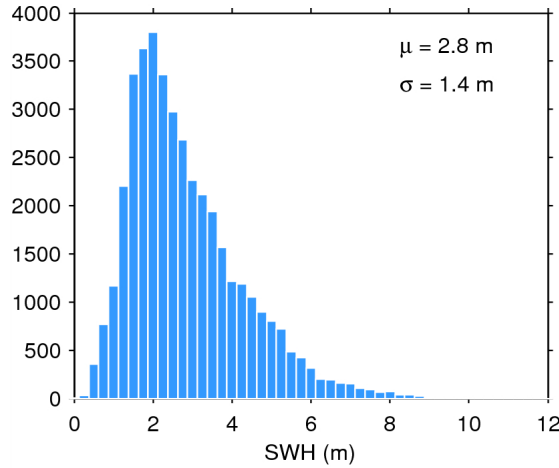
Figure 20. Histogram of science-valid SWH over oceans and lakes for 11/08/2015. The mean ( \mu ) and standard deviation ( \sigma ) are also shown. Note that values larger than 12 m are excluded from the histogram for the sake of readability but not from the computation of \mu and \sigma .
