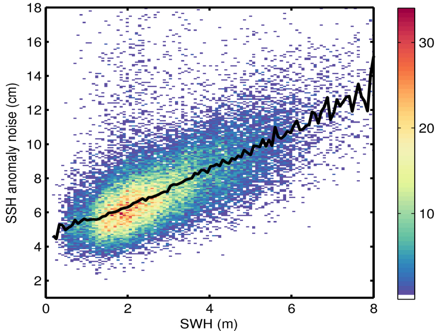
Figure 9. 2D histogram showing flag-valid SSH anomaly noise as a function of SWH for 11/08/2015. The black line denotes the median SSH anomaly as a function of SWH.
