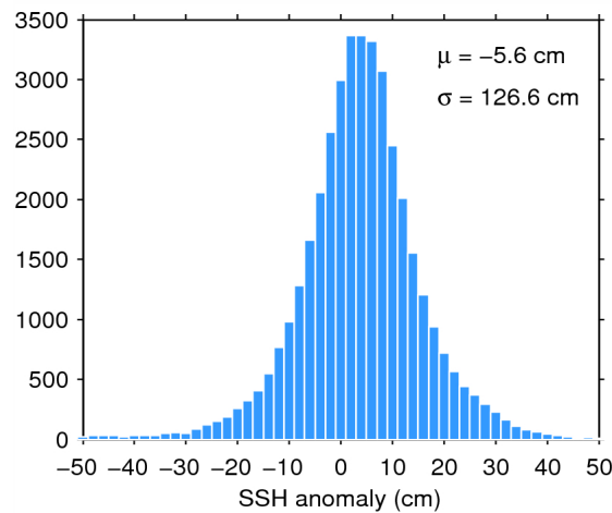
Figure 7. Histogram of flag-valid SSH anomaly over oceans and lakes for 10/08/2015. The mean ( \mu ) and standard deviation ( \sigma ) are also shown. Note that values outside [-50 50] cm are excluded from the histogram for the sake of readability but not from the computation of \mu and \sigma .
