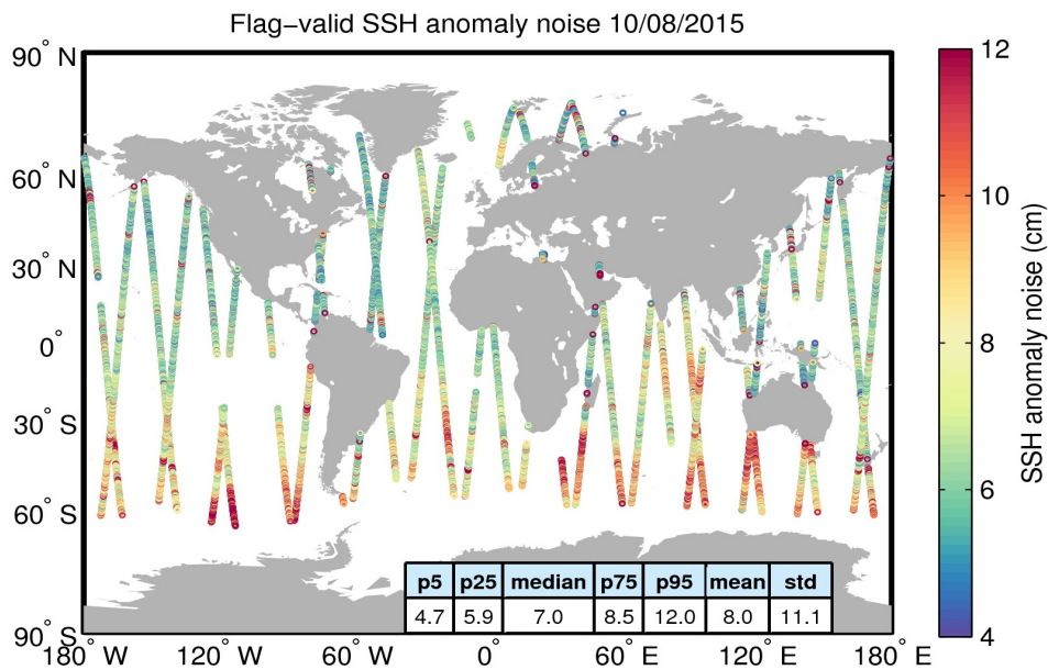
Figure 8. Geographical distribution of flag-valid 20-Hz SSH anomaly measurement noise over oceans and lakes for 10/08/2015. The statistical values shown in the table refer to the SSH anomaly noise and are calculated over all measurements shown in the figure.
