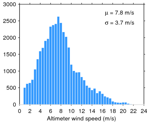
Figure 33. Histogram of flag-valid wind over oceans and lakes for 10/08/2015. The mean ( \mu ) and standard deviation ( \sigma ) are also shown. Note that values larger than 24 m/s are excluded from the histogram for the sake of readability but not from the computation of \mu and \sigma .
