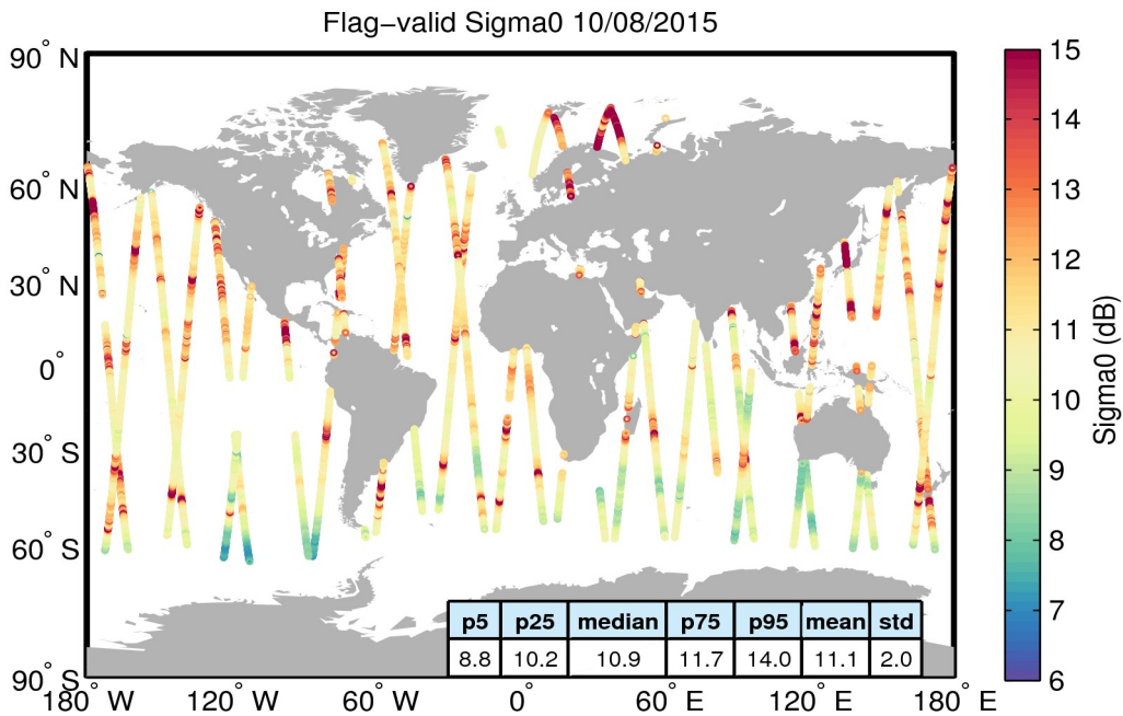
Figure 23. Geographical distribution of flag-valid sigma0 data over oceans and lakes for 10/08/2015. The statistical values shown in the table refer to the sigma0 in dB and are calculated over all measurements shown in the figure.
