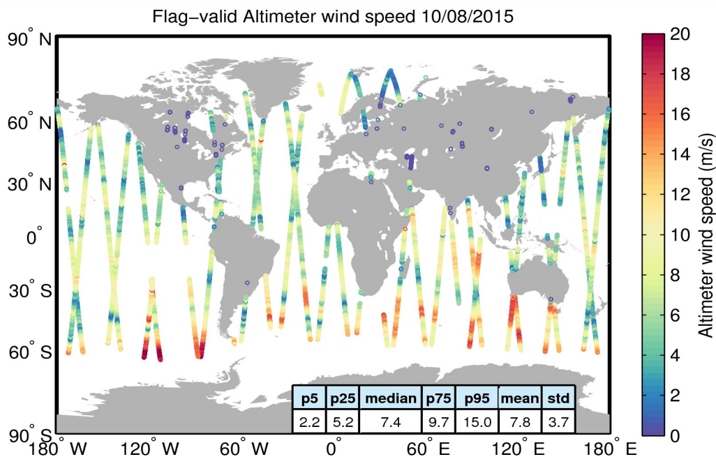
Figure 31. Geographical distribution of flag-valid wind data over oceans and lakes for 10/08/2015. The statistical values shown in the table refer to the wind in m/s and are calculated over all measurements shown in the figure.
