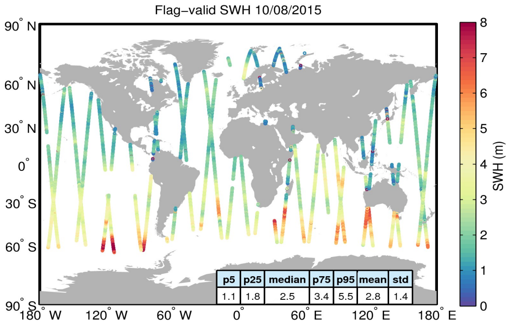
Figure 15. Geographical distribution of flag-valid SWH data over oceans and lakes for 10/08/2015. The statistical values shown in the figure refer to the SWH in m and are calculated over all measurements shown in the figure.
