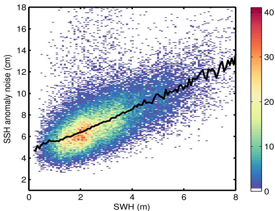
Figure 9. 2D histogram showing flag-valid SSH anomaly noise as a function of SWH for 10/08/2015. The black line denotes the median SSH anomaly as a function of SWH.
