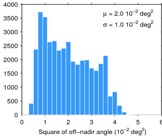
Figure 39. Histogram of flag-valid mispointing over oceans and lakes for 10/08/2015. The mean ( \mu ) and standard deviation ( \sigma ) are also shown. Note that values larger than 6 \cdot 10^{-2} \text{ deg}^2 are excluded from the histogram for the sake of readability but not from the computation of \mu and \sigma .
