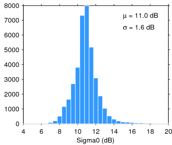
Figure 28. Histogram of science-valid sigma0 over oceans and lakes for 10/08/2015. The mean ( \mu ) and standard deviation ( \sigma ) are also shown. Note that values outside [4 20] dB are excluded from the histogram for the sake of readability but not from the computation of \mu and \sigma .
