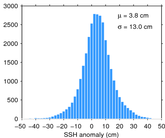
Figure 11. Histogram of science-valid SSH anomaly over oceans and lakes for 10/08/2015. The mean ( \mu ) and standard deviation ( \sigma ) are also shown. Note that values outside [-50 50] cm are excluded from the histogram for the sake of readability but not from the computation of \mu and \sigma .
