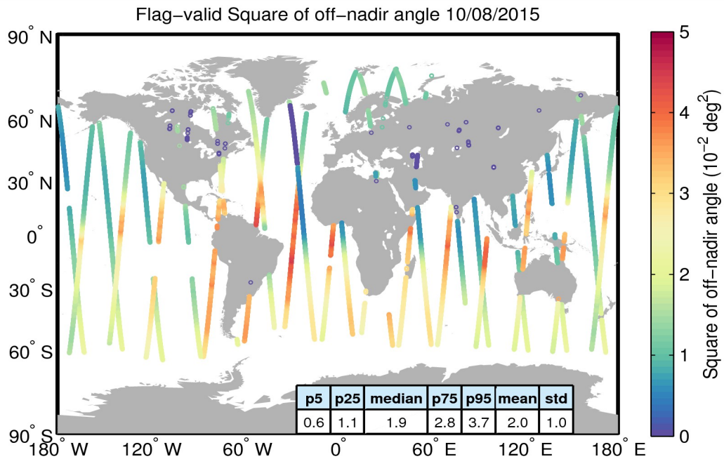
Figure 37. Geographical distribution of flag-valid mispointing data over oceans and lakes for 10/08/2015. The statistical values shown in the table refer to the mispointing in 10^{-2} \text{deg}^2 and are calculated over all measurements shown in the figure.
