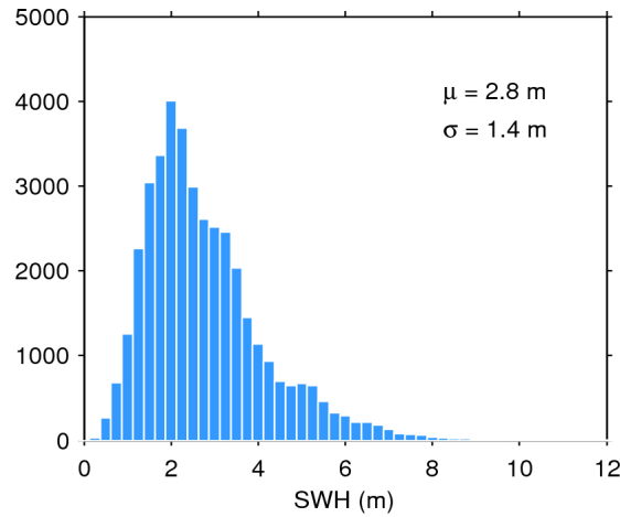
Figure 17. Histogram of flag-valid SWH over oceans and lakes for 10/08/2015. The mean ( \mu ) and standard deviation ( \sigma ) are also shown. Note that values larger than 12 m are excluded from the histogram for the sake of readability but not from the computation of \mu and \sigma .
