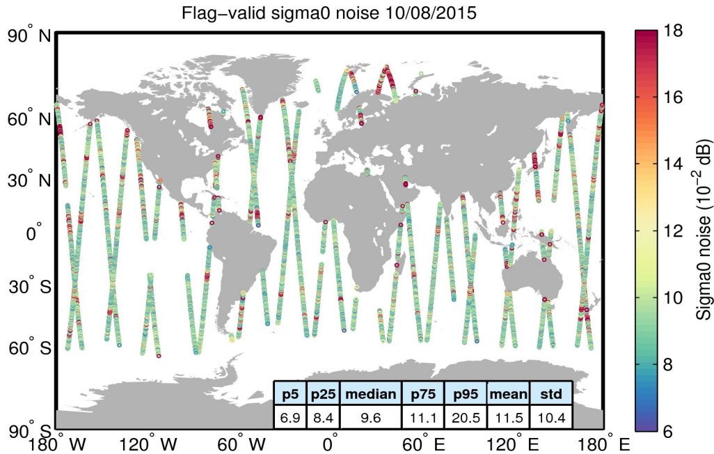
Figure 26. Geographical distribution of flag-valid 20-Hz sigma0 measurement noise over oceans and lakes for 10/08/2015. The statistical values shown in the table refer to the sigma0 noise and are calculated over all measurements shown in the figure.
