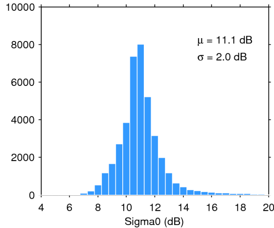
Figure 25. Histogram of flag-valid sigma0 over oceans and lakes for 10/08/2015. The mean ( \mu ) and standard deviation ( \sigma ) are also shown. Note that values outside [4 20] dB are excluded from the histogram for the sake of readability but not from the computation of \mu and \sigma .
