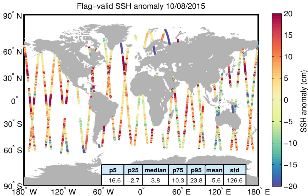
Figure 5. Geographical distribution of flag-valid 1-Hz SSH anomaly data over oceans and lakes for 10/08/2015. The statistical values shown in the table refer to the SSH anomaly in cm and are calculated over all measurements shown in the figure.
