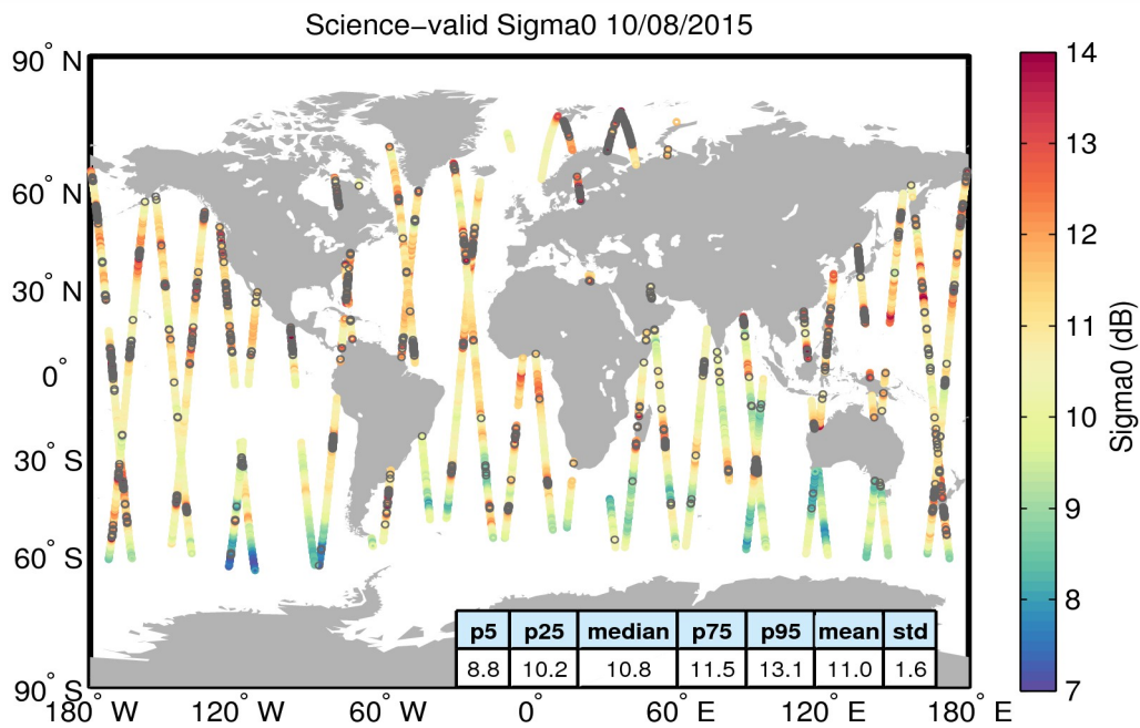
Figure 27. Geographical distribution of science-valid sigma0 data over oceans and lakes for 10/08/2015. The statistical values shown in the table refer to the sigma0 in dB and are calculated over all measurements shown in the figure. Gray circles denote records that have been rejected based on the editing criteria described in Table 4.
