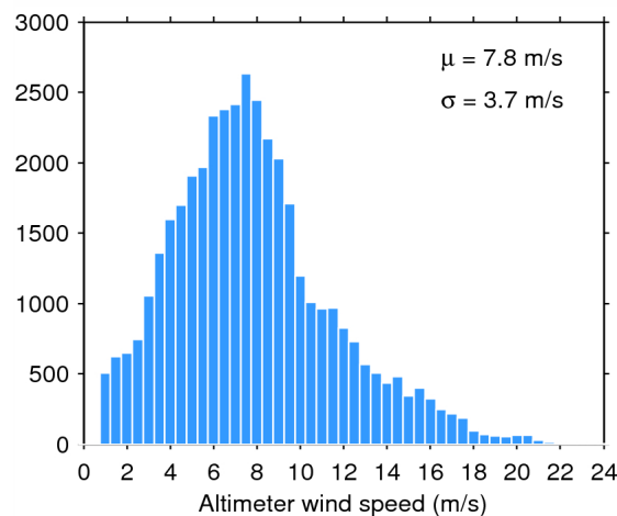
Figure 35. Histogram of science-valid wind over oceans and lakes for 10/08/2015. The mean ( \mu ) and standard deviation ( \sigma ) are also shown. Note that values larger than 24 m/s are excluded from the histogram for the sake of readability but not from the computation of \mu and \sigma .
