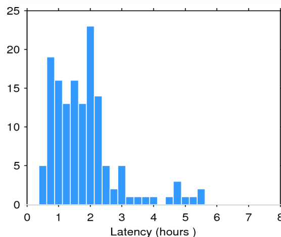
Figure 2. Histogram of the data latency for 10/08/2015. The y-axis denotes the number of files that are made available with a delay of x-hours with respect to the mean time of the records stored in the file.
