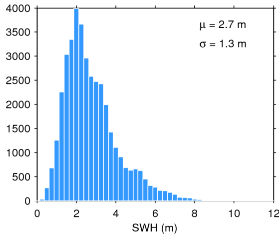
Figure 20. Histogram of science-valid SWH over oceans and lakes for 10/08/2015. The mean ( \mu ) and standard deviation ( \sigma ) are also shown. Note that values larger than 12 m are excluded from the histogram for the sake of readability but not from the computation of \mu and \sigma .
