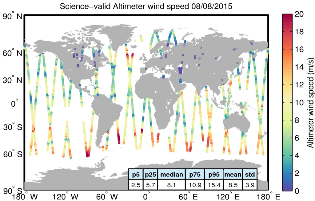
Figure 34. Geographical distribution of science-valid wind data over oceans and lakes for 08/08/2015. The statistical values shown in the table refer to the wind in m/s and are calculated over all measurements shown in the figure. Gray circles denote records that have been rejected based on the editing criteria described in Table 5.
