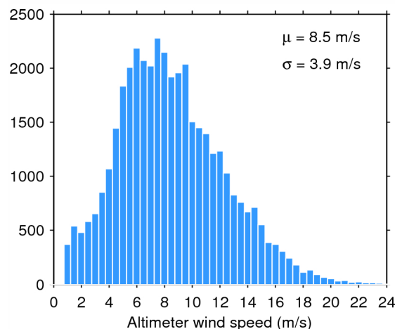
Figure 35. Histogram of science-valid wind over oceans and lakes for 08/08/2015. The mean ( \mu ) and standard deviation ( \sigma ) are also shown. Note that values larger than 24 m/s are excluded from the histogram for the sake of readability but not from the computation of \mu and \sigma .
