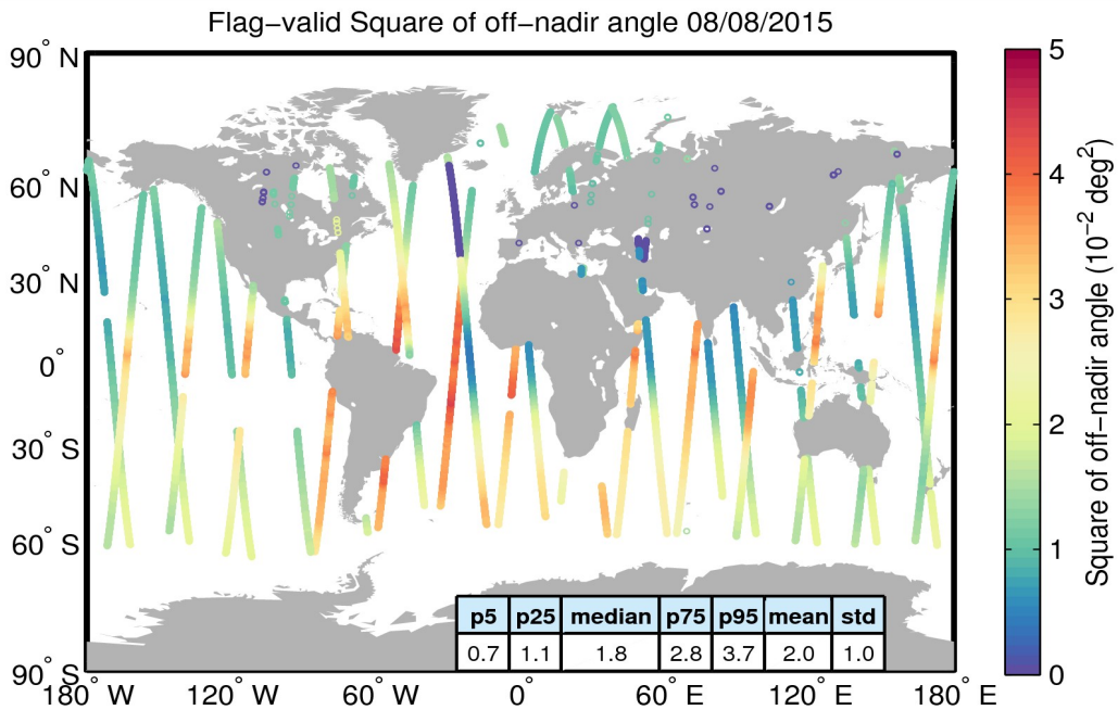
Figure 37. Geographical distribution of flag-valid mispointing data over oceans and lakes for 08/08/2015. The statistical values shown in the table refer to the mispointing in 10^{-2} \text{deg}^2 and are calculated over all measurements shown in the figure.
