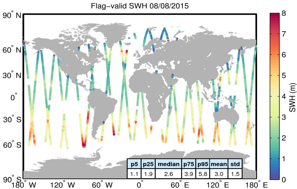
Figure 15. Geographical distribution of flag-valid SWH data over oceans and lakes for 08/08/2015. The statistical values shown in the table refer to the SWH in m and are calculated over all measurements shown in the figure.
