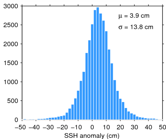
Figure 11. Histogram of science-valid SSH anomaly over oceans and lakes for 08/08/2015. The mean ( \mu ) and standard deviation ( \sigma ) are also shown. Note that values outside [-50 50] cm are excluded from the histogram for the sake of readability but not from the computation of \mu and \sigma .
