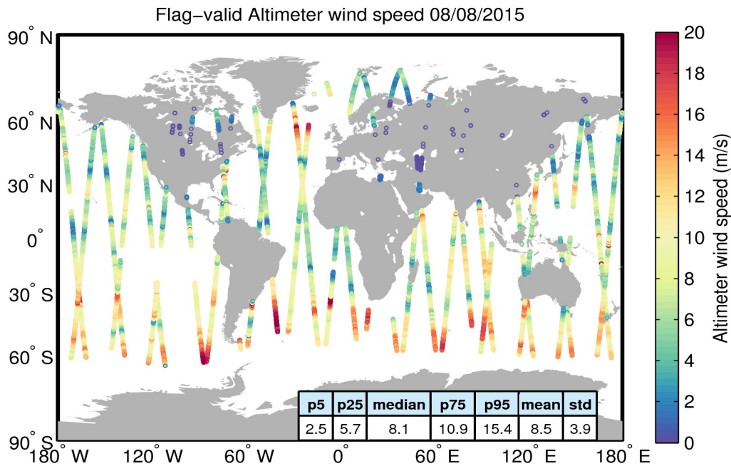
Figure 31. Geographical distribution of flag-valid wind data over oceans and lakes for 08/08/2015. The statistical values shown in the table refer to the wind in m/s and are calculated over all measurements shown in the figure.
