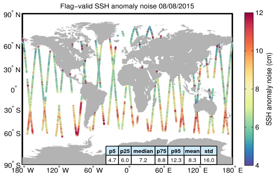
Figure 8. Geographical distribution of flag-valid 20-Hz SSH anomaly measurement noise over oceans and lakes for 08/08/2015. The statistical values shown in the table refer to the SSH anomaly noise and are calculated over all measurements shown in the figure.
