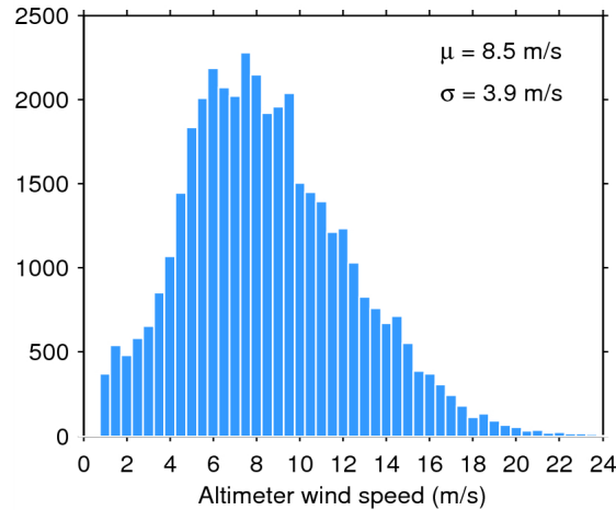
Figure 33. Histogram of flag-valid wind over oceans and lakes for 08/08/2015. The mean ( \mu ) and standard deviation ( \sigma ) are also shown. Note that values larger than 24 m/s are excluded from the histogram for the sake of readability but not from the computation of \mu and \sigma .
