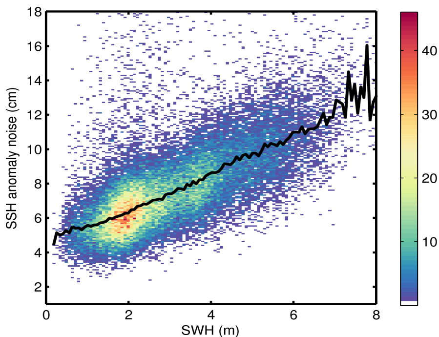
Figure 9. 2D histogram showing flag-valid SSH anomaly noise as a function of SWH for 08/08/2015. The black line denotes the median SSH anomaly as a function of SWH.
