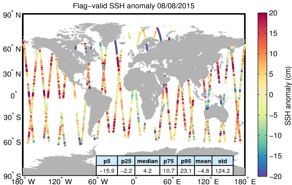
Figure 5. Geographical distribution of flag-valid 1-Hz SSH anomaly data over oceans and lakes for 08/08/2015. The statistical values shown in the table refer to the SSH anomaly in cm and are calculated over all measurements shown in the figure.
