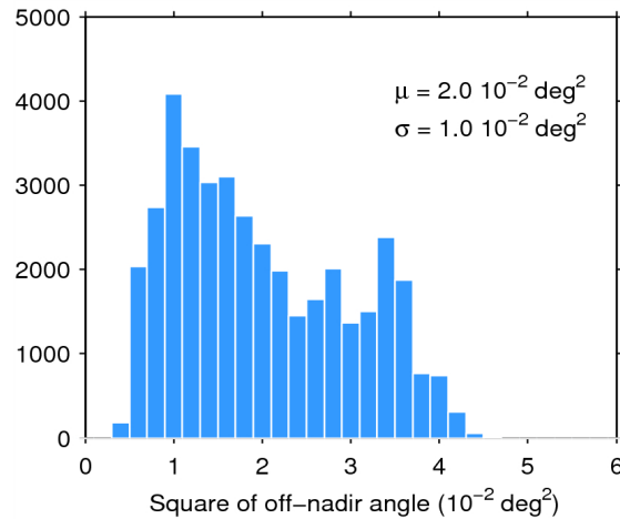
Figure 39. Histogram of flag-valid mispointing over oceans and lakes for 08/08/2015. The mean ( \mu ) and standard deviation ( \sigma ) are also shown. Note that values larger than 6 \cdot 10^{-2} \text{ deg}^2 are excluded from the histogram for the sake of readability but not from the computation of \mu and \sigma .
