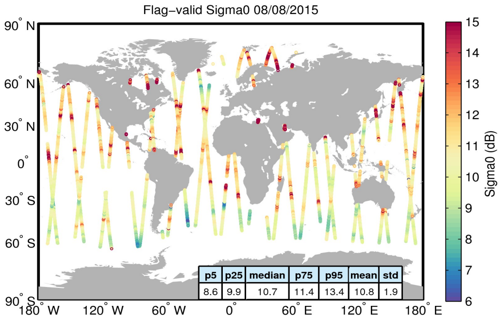
Figure 23. Geographical distribution of flag-valid sigma0 data over oceans and lakes for 08/08/2015. The statistical values shown in the table refer to the sigma0 in dB and are calculated over all measurements shown in the figure.
