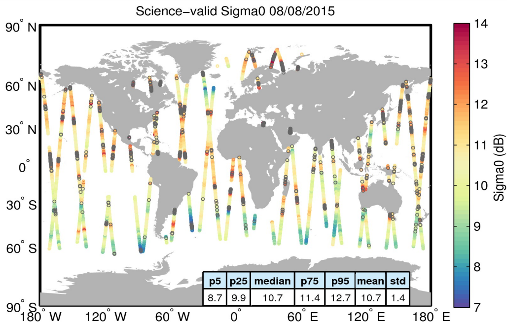
Figure 27. Geographical distribution of science-valid sigma0 data over oceans and lakes for 08/08/2015. The statistical values shown in the table refer to the sigma0 in dB and are calculated over all measurements shown in the figure. Gray circles denote records that have been rejected based on the editing criteria described in Table 4.
