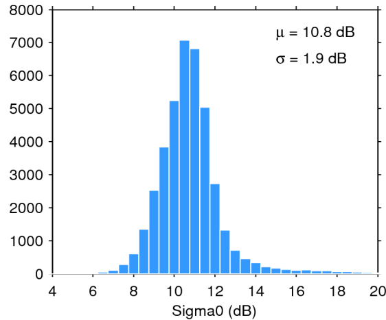
Figure 25. Histogram of flag-valid sigma0 over oceans and lakes for 08/08/2015. The mean ( \mu ) and standard deviation ( \sigma ) are also shown. Note that values outside [4 20] dB are excluded from the histogram for the sake of readability but not from the computation of \mu and \sigma .
