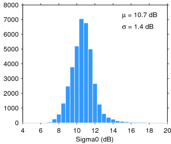
Figure 28. Histogram of science-valid sigma0 over oceans and lakes for 08/08/2015. The mean ( \mu ) and standard deviation ( \sigma ) are also shown. Note that values outside [4 20] dB are excluded from the histogram for the sake of readability but not from the computation of \mu and \sigma .
