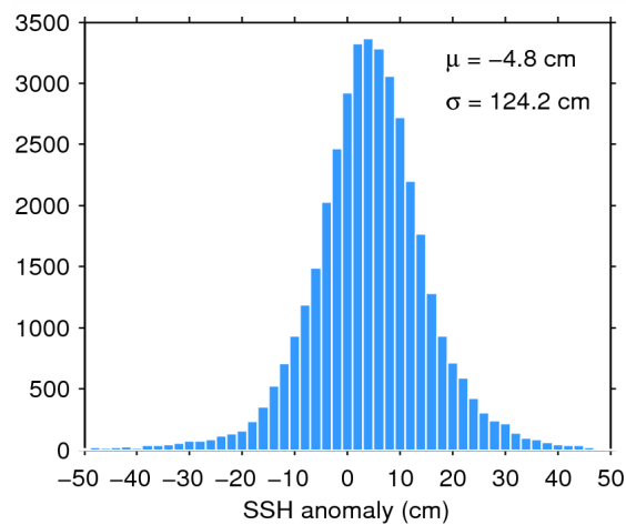
Figure 7. Histogram of flag-valid SSH anomaly over oceans and lakes for 08/08/2015. The mean ( \mu ) and standard deviation ( \sigma ) are also shown. Note that values outside [-50 50] cm are excluded from the histogram for the sake of readability but not from the computation of \mu and \sigma .
