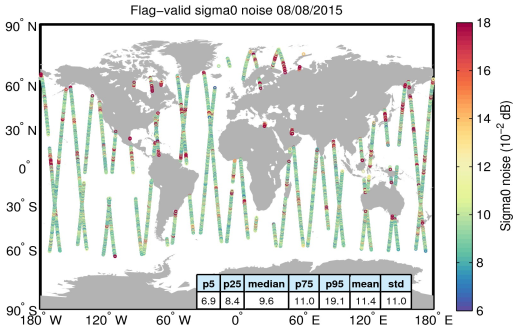
Figure 26. Geographical distribution of flag-valid 20-Hz sigma0 measurement noise over oceans and lakes for 08/08/2015. The statistical values shown in the table refer to the sigma0 noise and are calculated over all measurements shown in the figure.
