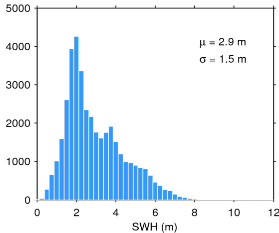
Figure 20. Histogram of science-valid SWH over oceans and lakes for 08/08/2015. The mean ( \mu ) and standard deviation ( \sigma ) are also shown. Note that values larger than 12 m are excluded from the histogram for the sake of readability but not from the computation of \mu and \sigma .
