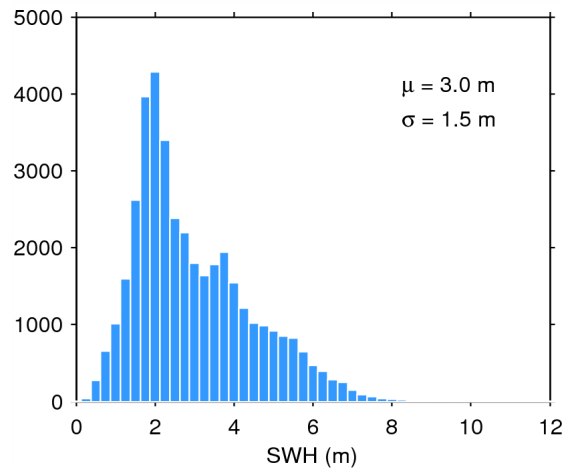
Figure 17. Histogram of flag-valid SWH over oceans and lakes for 08/08/2015. The mean ( \mu ) and standard deviation ( \sigma ) are also shown. Note that values larger than 12 m are excluded from the histogram for the sake of readability but not from the computation of \mu and \sigma .
