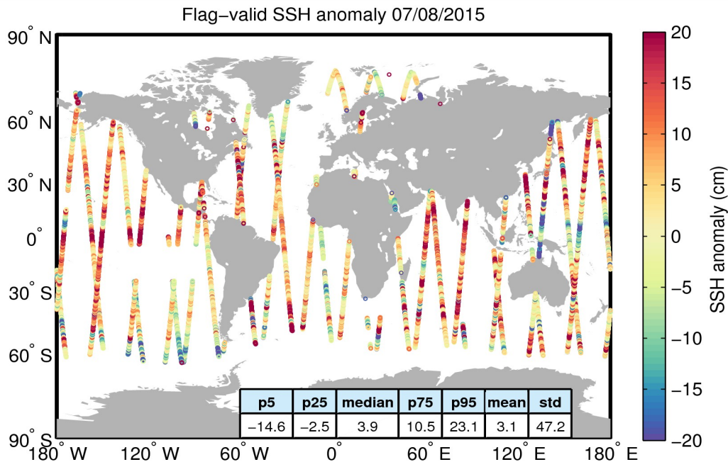
Figure 5. Geographical distribution of flag-valid 1-Hz SSH anomaly data over oceans and lakes for 07/08/2015. The statistical values shown in the table refer to the SSH anomaly in cm and are calculated over all measurements shown in the figure.
