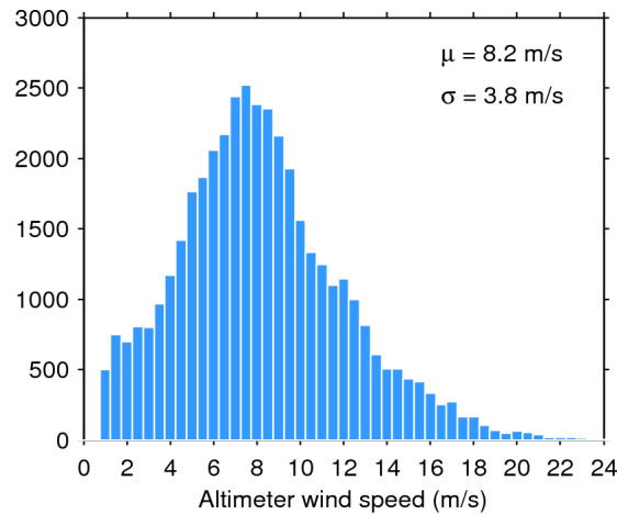
Figure 33. Histogram of flag-valid wind over oceans and lakes for 07/08/2015. The mean ( \mu ) and standard deviation ( \sigma ) are also shown. Note that values larger than 24 m/s are excluded from the histogram for the sake of readability but not from the computation of \mu and \sigma .
