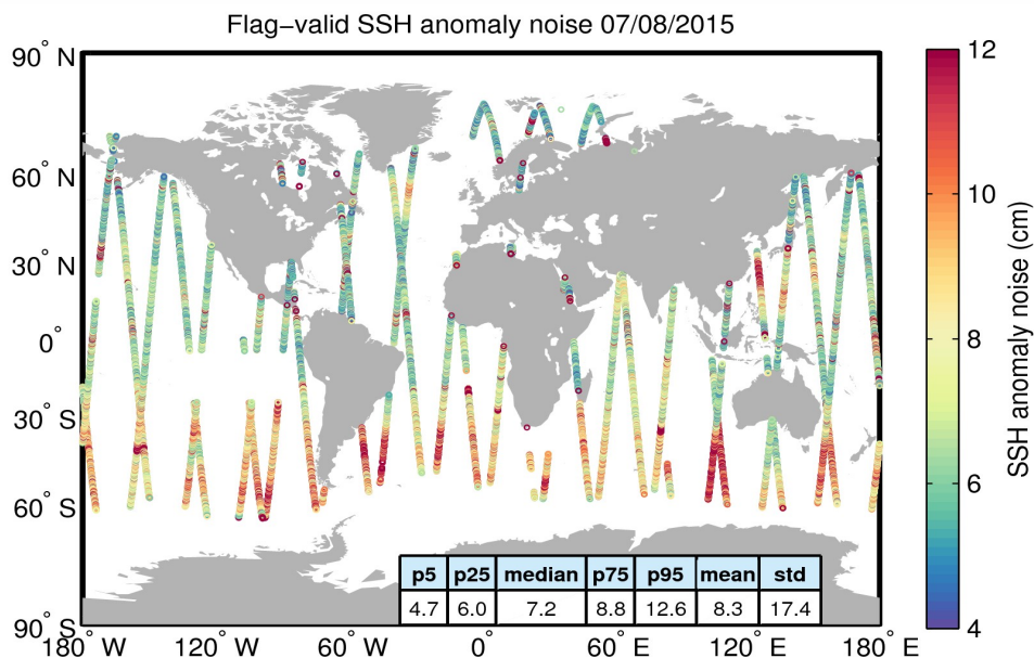
Figure 8. Geographical distribution of flag-valid 20-Hz SSH anomaly measurement noise over oceans and lakes for 07/08/2015. The statistical values shown in the table refer to the SSH anomaly noise and are calculated over all measurements shown in the figure.
