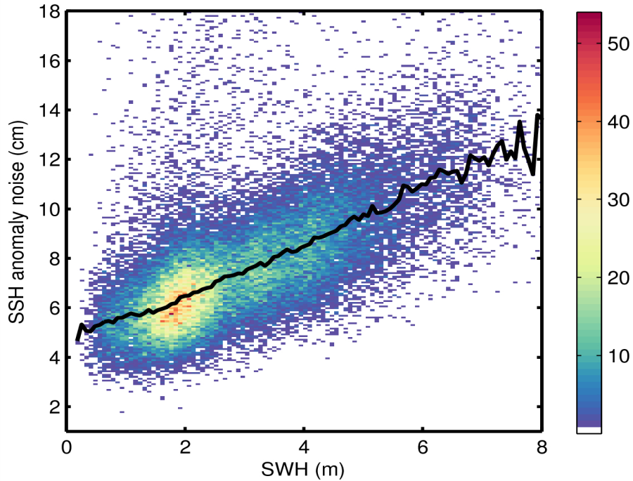
Figure 9. 2D histogram showing flag-valid SSH anomaly noise as a function of SWH for 07/08/2015. The black line denotes the median SSH anomaly as a function of SWH.
