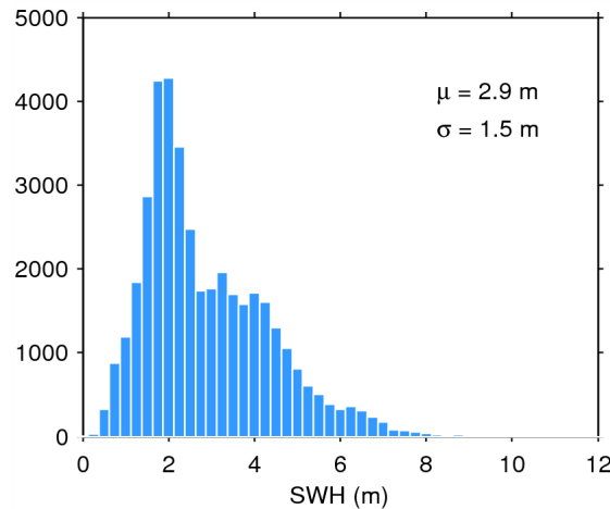
Figure 20. Histogram of science-valid SWH over oceans and lakes for 07/08/2015. The mean ( \mu ) and standard deviation ( \sigma ) are also shown. Note that values larger than 12 m are excluded from the histogram for the sake of readability but not from the computation of \mu and \sigma .
