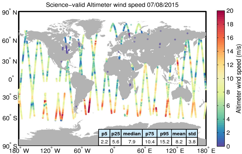
Figure 34. Geographical distribution of science-valid wind data over oceans and lakes for 07/08/2015. The statistical values shown in the table refer to the wind in m/s and are calculated over all measurements shown in the figure. Gray circles denote records that have been rejected based on the editing criteria described in Table 5.
