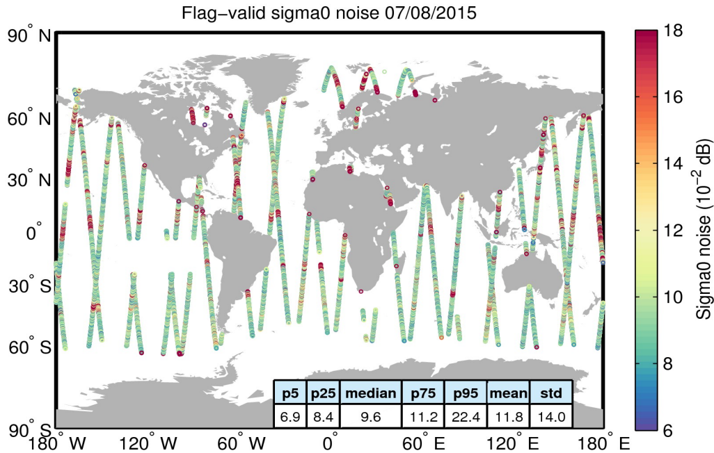
Figure 26. Geographical distribution of flag-valid 20-Hz sigma0 measurement noise over oceans and lakes for 07/08/2015. The statistical values shown in the table refer to the sigma0 noise and are calculated over all measurements shown in the figure.
