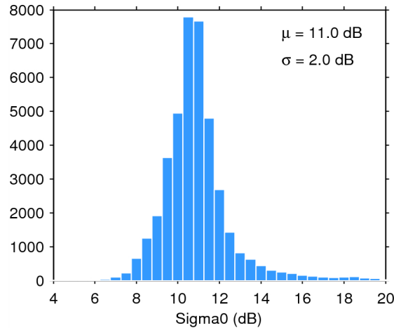
Figure 25. Histogram of flag-valid sigma0 over oceans and lakes for 07/08/2015. The mean ( \mu ) and standard deviation ( \sigma ) are also shown. Note that values outside [4 20] dB are excluded from the histogram for the sake of readability but not from the computation of \mu and \sigma .
