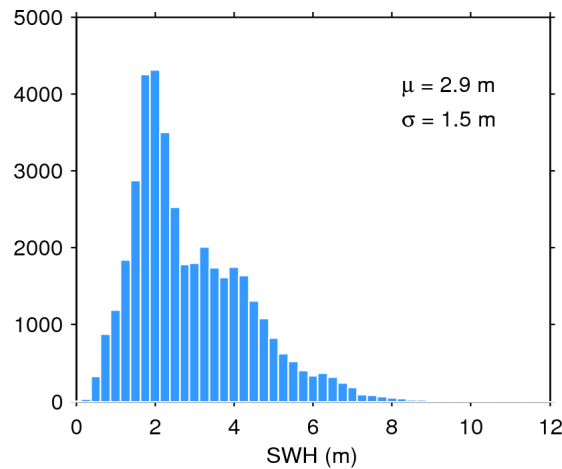
Figure 17. Histogram of flag-valid SWH over oceans and lakes for 07/08/2015. The mean ( \mu ) and standard deviation ( \sigma ) are also shown. Note that values larger than 12 m are excluded from the histogram for the sake of readability but not from the computation of \mu and \sigma .
