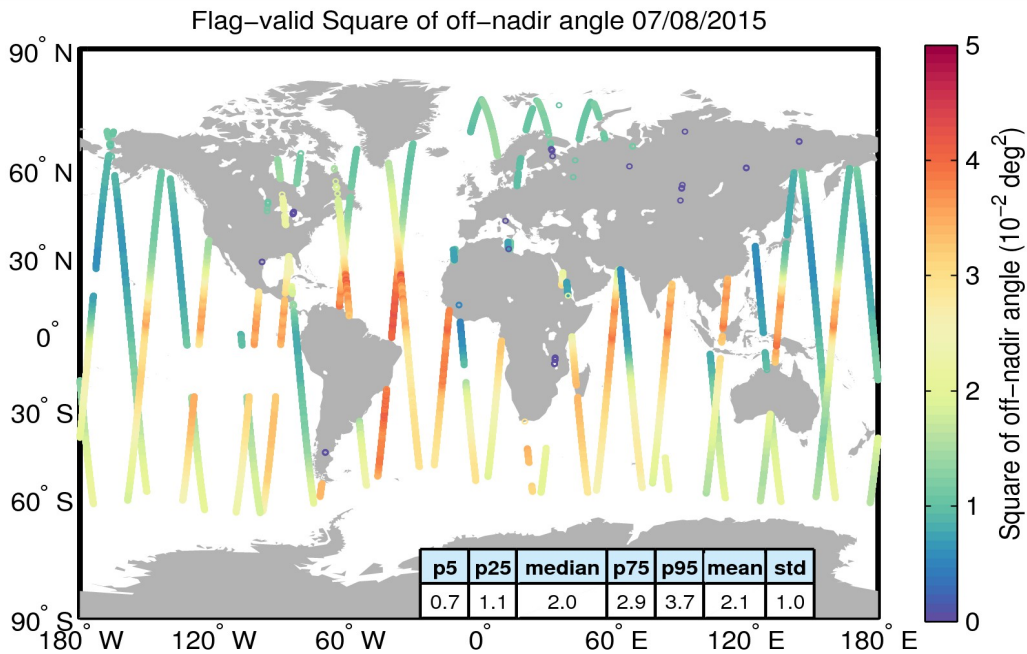
Figure 37. Geographical distribution of flag-valid mispointing data over oceans and lakes for 07/08/2015. The statistical values shown in the table refer to the mispointing in 10^{-2} \text{ deg}^2 and are calculated over all measurements shown in the figure.
