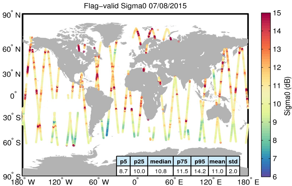
Figure 23. Geographical distribution of flag-valid sigma0 data over oceans and lakes for 07/08/2015. The statistical values shown in the table refer to the sigma0 in dB and are calculated over all measurements shown in the figure.
