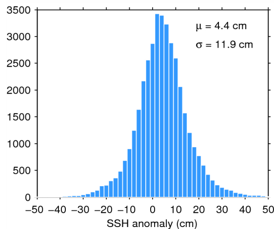
Figure 11. Histogram of science-valid SSH anomaly over oceans and lakes for 07/08/2015. The mean ( \mu ) and standard deviation ( \sigma ) are also shown. Note that values outside [-50 50] cm are excluded from the histogram for the sake of readability but not from the computation of \mu and \sigma .
