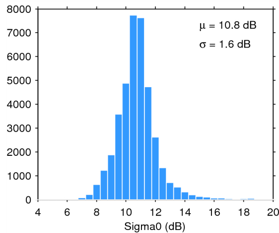
Figure 28. Histogram of science-valid sigma0 over oceans and lakes for 07/08/2015. The mean ( \mu ) and standard deviation ( \sigma ) are also shown. Note that values outside [4 20] dB are excluded from the histogram for the sake of readability but not from the computation of \mu and \sigma .
