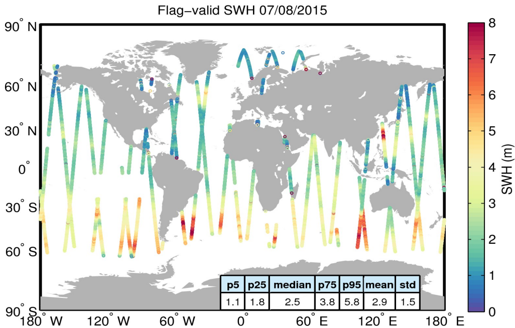
Figure 15. Geographical distribution of flag-valid SWH data over oceans and lakes for 07/08/2015. The statistical values shown in the table refer to the SWH in m and are calculated over all measurements shown in the figure.
