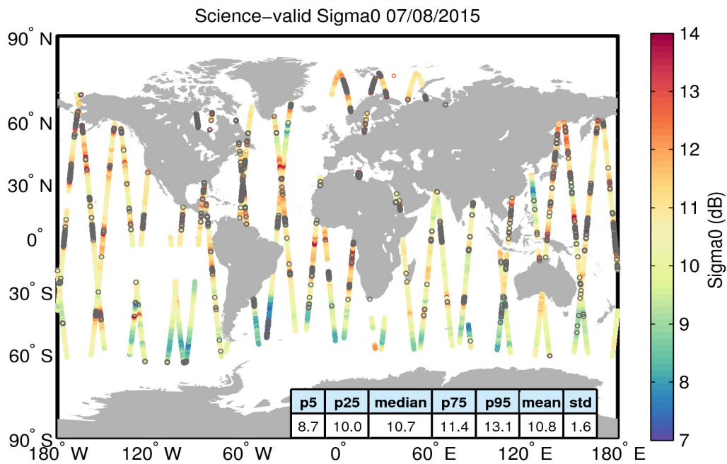
Figure 27. Geographical distribution of science-valid sigma0 data over oceans and lakes for 07/08/2015. The statistical values shown in the table refer to the sigma0 in dB and are calculated over all measurements shown in the figure. Gray circles denote records that have been rejected based on the editing criteria described in Table 4.
