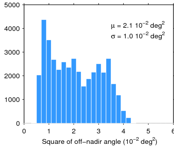
Figure 39. Histogram of flag-valid mispointing over oceans and lakes for 07/08/2015. The mean ( \mu ) and standard deviation ( \sigma ) are also shown. Note that values larger than 6 \cdot 10^{-2} \text{ deg}^2 are excluded from the histogram for the sake of readability but not from the computation of \mu and \sigma .
