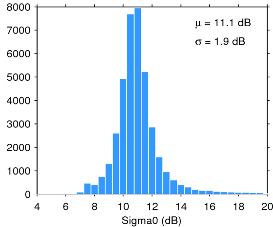
Figure 25. Histogram of flag-valid sigma0 over oceans and lakes for 06/08/2015. The mean ( \mu ) and standard deviation ( \sigma ) are also shown. Note that values outside [4 20] dB are excluded from the histogram for the sake of readability but not from the computation of \mu and \sigma .
