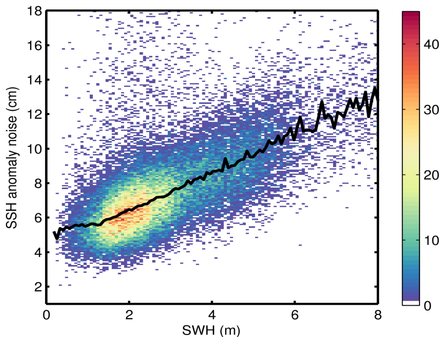
Figure 9. 2D histogram showing flag-valid SSH anomaly noise as a function of SWH for 06/08/2015. The black line denotes the median SSH anomaly as a function of SWH.
