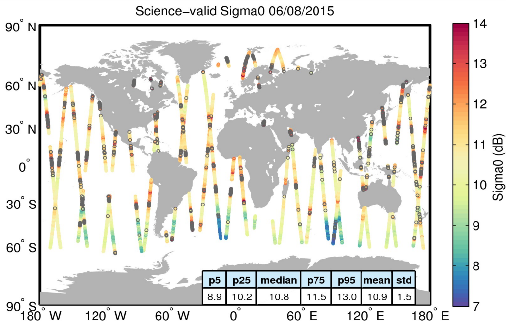
Figure 27. Geographical distribution of science-valid sigma0 data over oceans and lakes for 06/08/2015. The statistical values shown in the table refer to the sigma0 in dB and are calculated over all measurements shown in the figure. Gray circles denote records that have been rejected based on the editing criteria described in Table 4.
