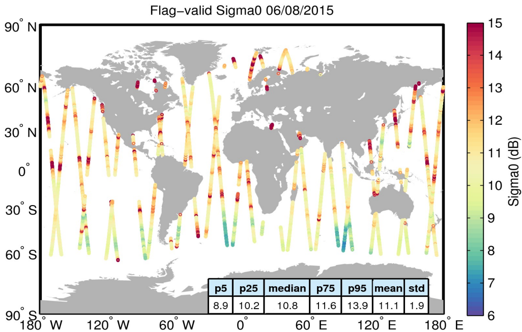
Figure 23. Geographical distribution of flag-valid sigma0 data over oceans and lakes for 06/08/2015. The statistical values shown in the table refer to the sigma0 in dB and are calculated over all measurements shown in the figure.
