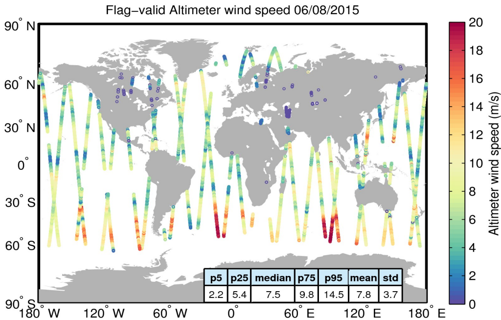
Figure 31. Geographical distribution of flag-valid wind data over oceans and lakes for 06/08/2015. The statistical values shown in the table refer to the wind in m/s and are calculated over all measurements shown in the figure.
