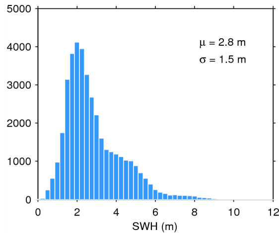
Figure 17. Histogram of flag-valid SWH over oceans and lakes for 06/08/2015. The mean ( \mu ) and standard deviation ( \sigma ) are also shown. Note that values larger than 12 m are excluded from the histogram for the sake of readability but not from the computation of \mu and \sigma .
