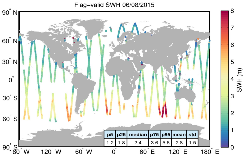
Figure 15. Geographical distribution of flag-valid SWH data over oceans and lakes for 06/08/2015. The statistical values shown in the table refer to the SWH in m and are calculated over all measurements shown in the figure.
