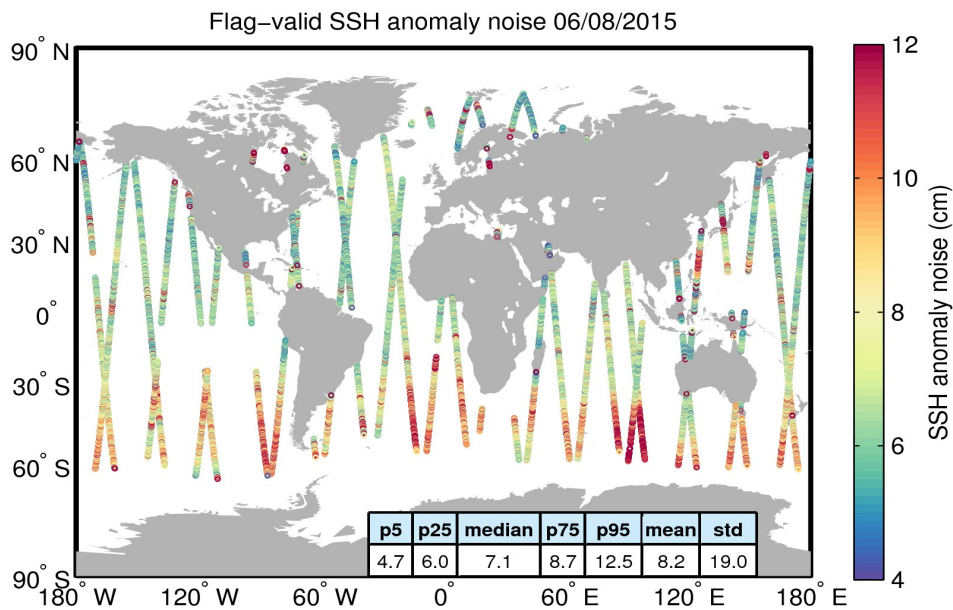
Figure 8. Geographical distribution of flag-valid 20-Hz SSH anomaly measurement noise over oceans and lakes for 06/08/2015. The statistical values shown in the table refer to the SSH anomaly noise and are calculated over all measurements shown in the figure.
