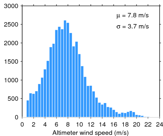
Figure 35. Histogram of science-valid wind over oceans and lakes for 06/08/2015. The mean ( \mu ) and standard deviation ( \sigma ) are also shown. Note that values larger than 24 m/s are excluded from the histogram for the sake of readability but not from the computation of \mu and \sigma .
