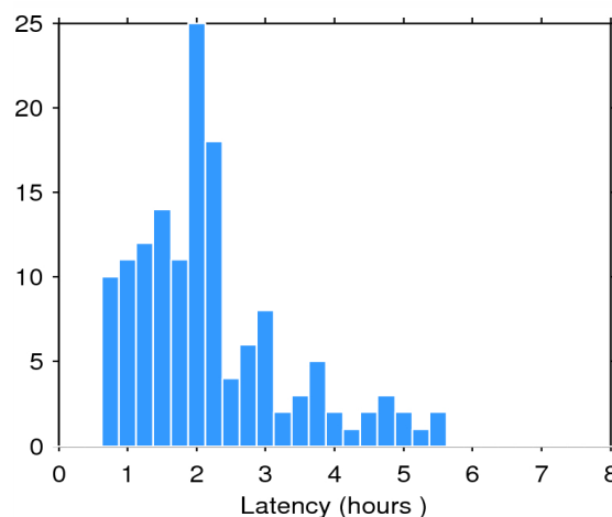
Figure 2. Histogram of the data latency for 06/08/2015. The y-axis denotes the number of files that are made available with a delay of x-hours with respect to the mean time of the records stored in the file.
