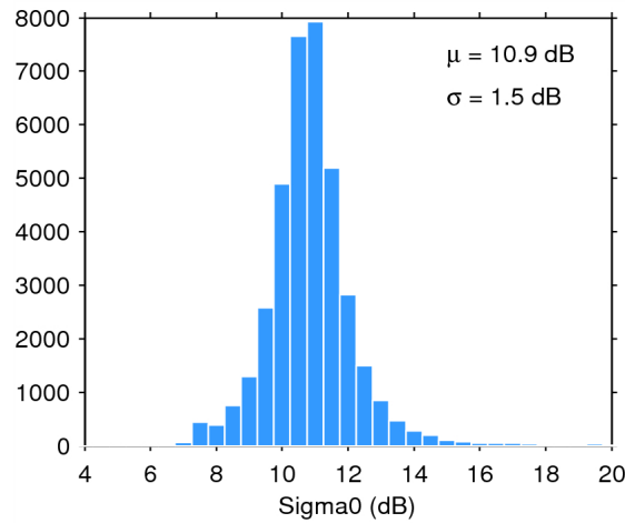
Figure 28. Histogram of science-valid sigma0 over oceans and lakes for 06/08/2015. The mean ( \mu ) and standard deviation ( \sigma ) are also shown. Note that values outside [4 20] dB are excluded from the histogram for the sake of readability but not from the computation of \mu and \sigma .
