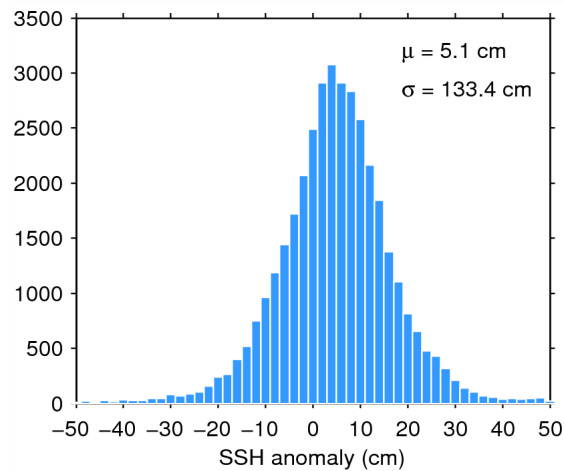
Figure 7. Histogram of flag-valid SSH anomaly over oceans and lakes for 06/08/2015. The mean ( \mu ) and standard deviation ( \sigma ) are also shown. Note that values outside [-50\ 50] cm are excluded from the histogram for the sake of readability but not from the computation of \mu and \sigma .
