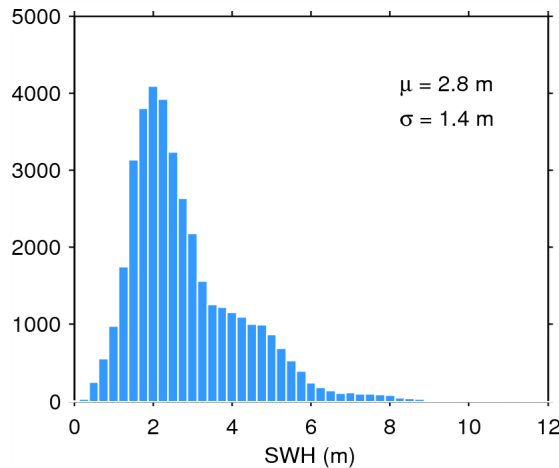
Figure 20. Histogram of science-valid SWH over oceans and lakes for 06/08/2015. The mean ( \mu ) and standard deviation ( \sigma ) are also shown. Note that values larger than 12 m are excluded from the histogram for the sake of readability but not from the computation of \mu and \sigma .
