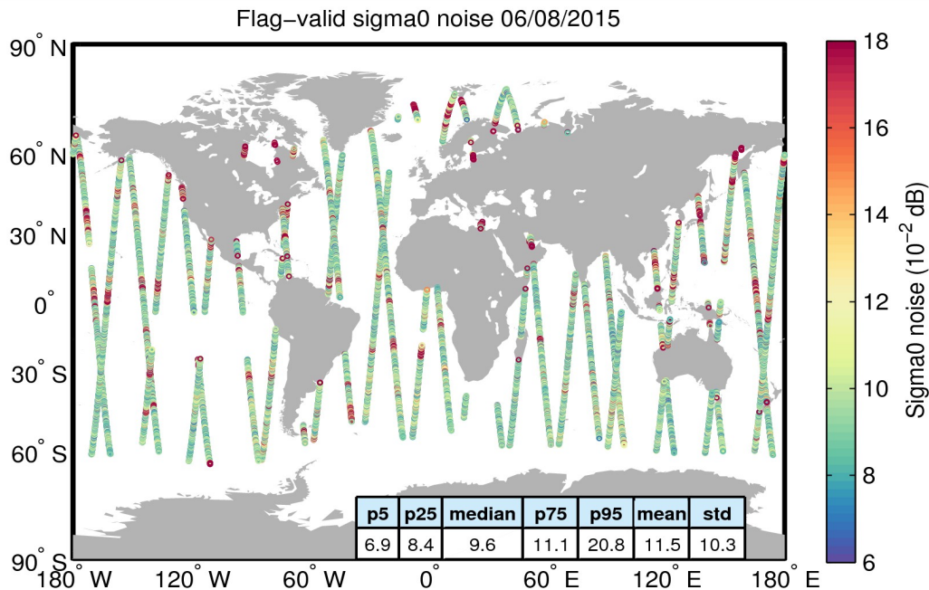
Figure 26. Geographical distribution of flag-valid 20-Hz sigma0 measurement noise over oceans and lakes for 06/08/2015. The statistical values shown in the table refer to the sigma0 noise and are calculated over all measurements shown in the figure.
