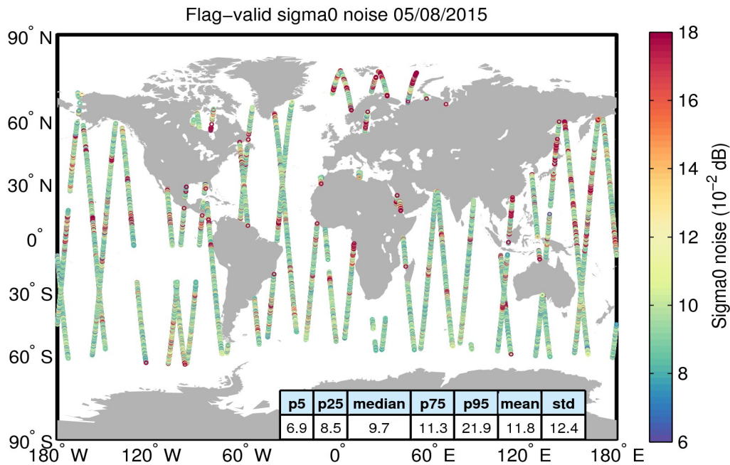
Figure 26. Geographical distribution of flag-valid 20-Hz sigma0 measurement noise over oceans and lakes for 05/08/2015. The statistical values shown in the table refer to the sigma0 noise and are calculated over all measurements shown in the figure.
