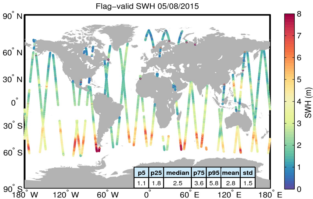
Figure 15. Geographical distribution of flag-valid SWH data over oceans and lakes for 05/08/2015. The statistical values shown in the figure refer to the SWH in m and are calculated over all measurements shown in the figure.
