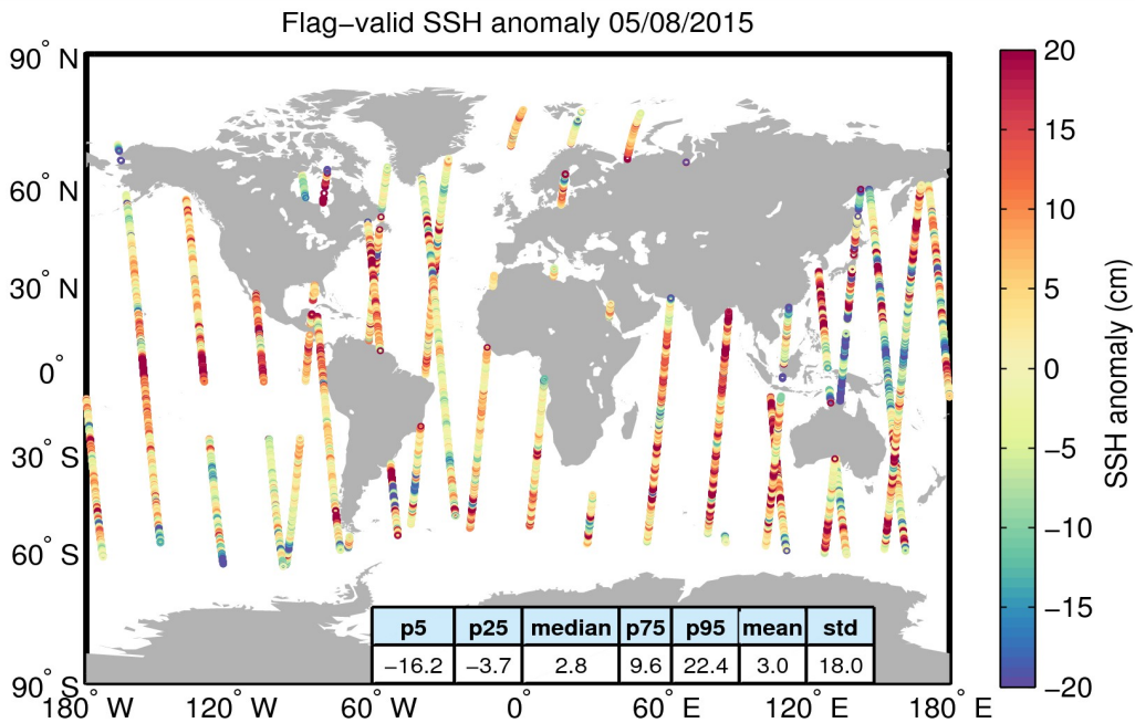
Figure 5. Geographical distribution of flag-valid 1-Hz SSH anomaly data over oceans and lakes for 05/08/2015. The statistical values shown in the table refer to the SSH anomaly in cm and are calculated over all measurements shown in the figure.
