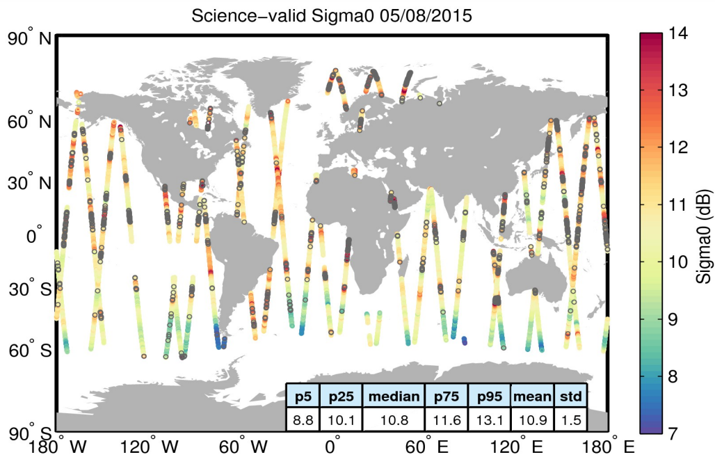
Figure 27. Geographical distribution of science-valid sigma0 data over oceans and lakes for 05/08/2015. The statistical values shown in the table refer to the sigma0 in dB and are calculated over all measurements shown in the figure. Gray circles denote records that have been rejected based on the editing criteria described in Table 4.
