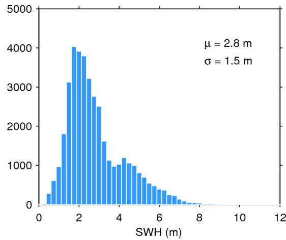
Figure 17. Histogram of flag-valid SWH over oceans and lakes for 05/08/2015. The mean ( \mu ) and standard deviation ( \sigma ) are also shown. Note that values larger than 12 m are excluded from the histogram for the sake of readability but not from the computation of \mu and \sigma .
