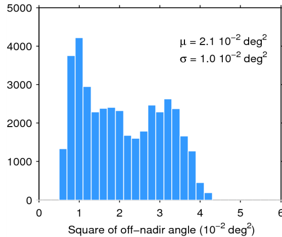
Figure 39. Histogram of flag-valid mispointing over oceans and lakes for 05/08/2015. The mean ( \mu ) and standard deviation ( \sigma ) are also shown. Note that values larger than 6 \cdot 10^{-2} \text{ deg}^2 are excluded from the histogram for the sake of readability but not from the computation of \mu and \sigma .
