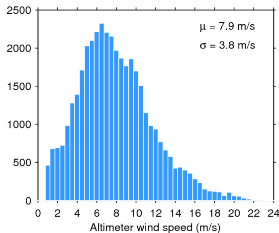
Figure 35. Histogram of science-valid wind over oceans and lakes for 05/08/2015. The mean ( \mu ) and standard deviation ( \sigma ) are also shown. Note that values larger than 24 m/s are excluded from the histogram for the sake of readability but not from the computation of \mu and \sigma .
