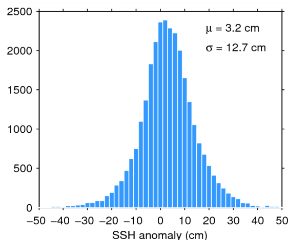
Figure 11. Histogram of science-valid SSH anomaly over oceans and lakes for 05/08/2015. The mean ( \mu ) and standard deviation ( \sigma ) are also shown. Note that values outside [-50 50] cm are excluded from the histogram for the sake of readability but not from the computation of \mu and \sigma .
