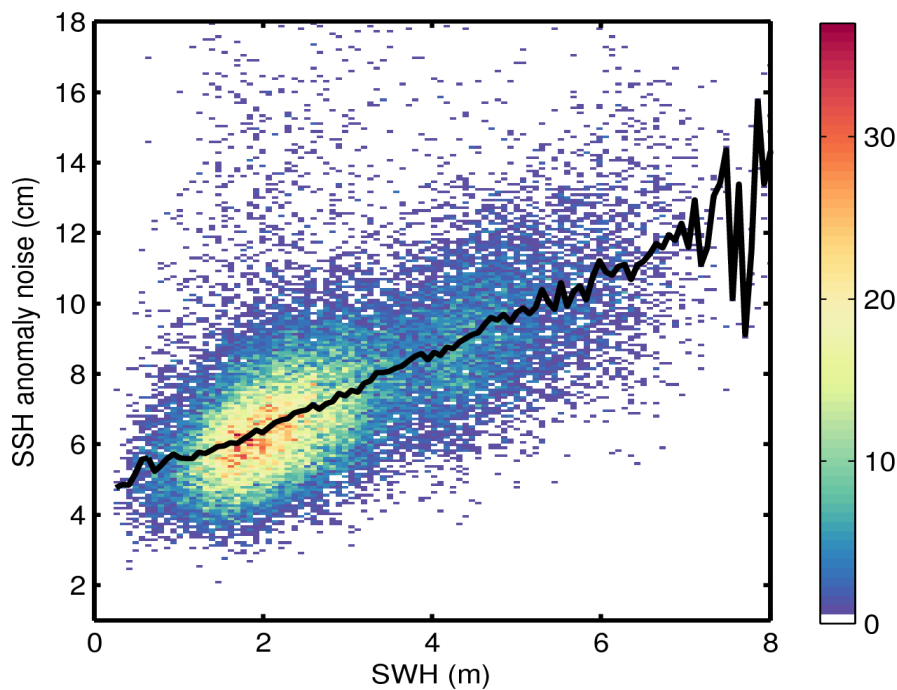
Figure 9. 2D histogram showing flag-valid SSH anomaly noise as a function of SWH for 05/08/2015. The black line denotes the median SSH anomaly as a function of SWH.
