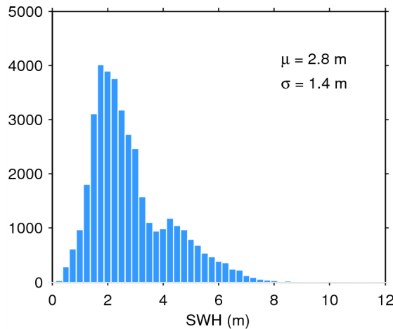
Figure 20. Histogram of science-valid SWH over oceans and lakes for 05/08/2015. The mean ( \mu ) and standard deviation ( \sigma ) are also shown. Note that values larger than 12 m are excluded from the histogram for the sake of readability but not from the computation of \mu and \sigma .
