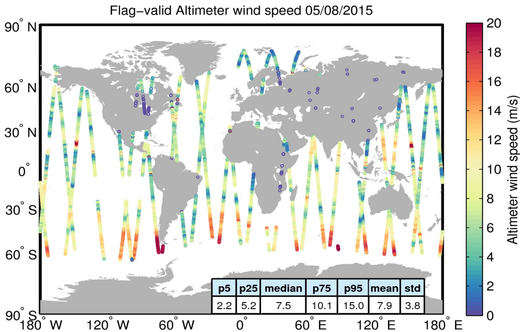
Figure 31. Geographical distribution of flag-valid wind data over oceans and lakes for 05/08/2015. The statistical values shown in the table refer to the wind in m/s and are calculated over all measurements shown in the figure.
