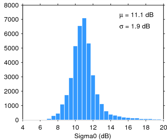
Figure 25. Histogram of flag-valid sigma0 over oceans and lakes for 05/08/2015. The mean ( \mu ) and standard deviation ( \sigma ) are also shown. Note that values outside [4 20] dB are excluded from the histogram for the sake of readability but not from the computation of \mu and \sigma .
