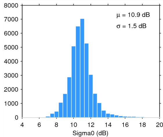
Figure 28. Histogram of science-valid sigma0 over oceans and lakes for 05/08/2015. The mean ( \mu ) and standard deviation ( \sigma ) are also shown. Note that values outside [4 20] dB are excluded from the histogram for the sake of readability but not from the computation of \mu and \sigma .
