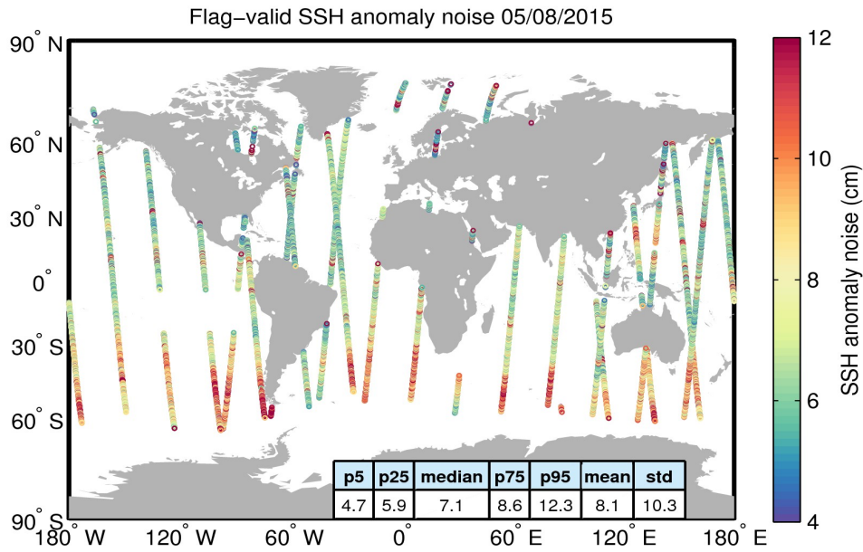
Figure 8. Geographical distribution of flag-valid 20-Hz SSH anomaly measurement noise over oceans and lakes for 05/08/2015. The statistical values shown in the table refer to the SSH anomaly noise and are calculated over all measurements shown in the figure.
