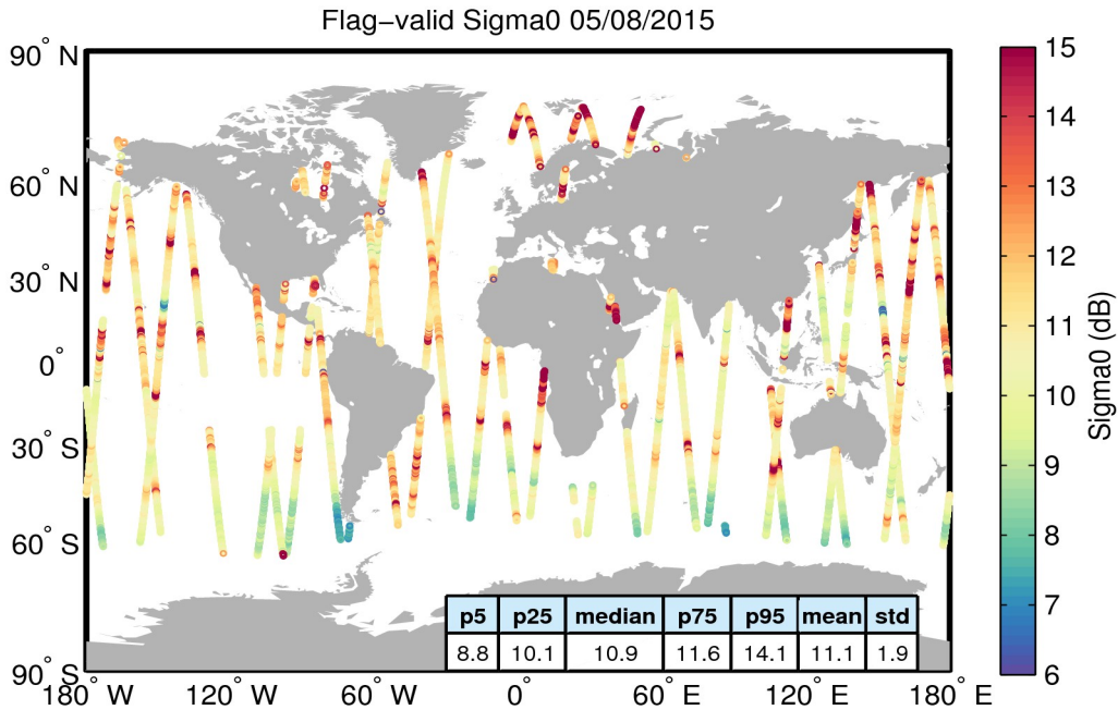
Figure 23. Geographical distribution of flag-valid sigma0 data over oceans and lakes for 05/08/2015. The statistical values shown in the table refer to the sigma0 in dB and are calculated over all measurements shown in the figure.
