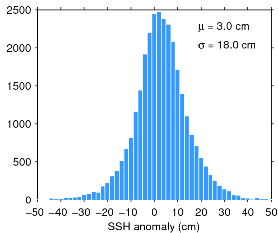
Figure 7. Histogram of flag-valid SSH anomaly over oceans and lakes for 05/08/2015. The mean ( \mu ) and standard deviation ( \sigma ) are also shown. Note that values outside [-50 50] cm are excluded from the histogram for the sake of readability but not from the computation of \mu and \sigma .
