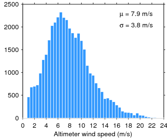
Figure 33. Histogram of flag-valid wind over oceans and lakes for 05/08/2015. The mean ( \mu ) and standard deviation ( \sigma ) are also shown. Note that values larger than 24 m/s are excluded from the histogram for the sake of readability but not from the computation of \mu and \sigma .
