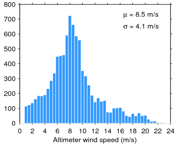
Figure 33. Histogram of flag-valid wind over oceans and lakes for 04/08/2015. The mean ( \mu ) and standard deviation ( \sigma ) are also shown. Note that values larger than 24 m/s are excluded from the histogram for the sake of readability but not from the computation of \mu and \sigma .
