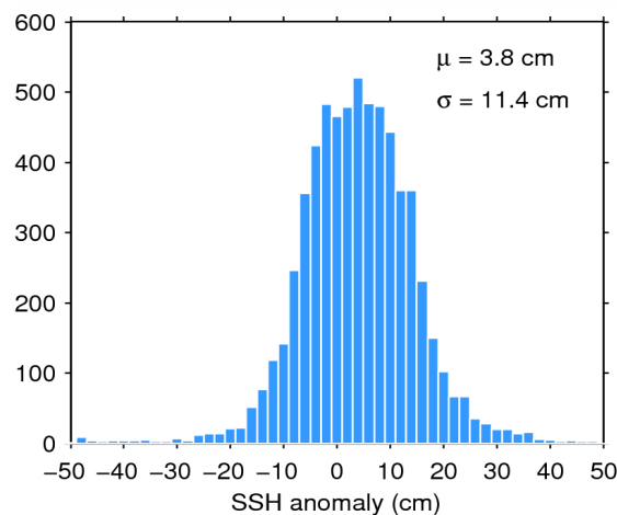
Figure 11. Histogram of science-valid SSH anomaly over oceans and lakes for 04/08/2015. The mean ( \mu ) and standard deviation ( \sigma ) are also shown. Note that values outside [-50 50] cm are excluded from the histogram for the sake of readability but not from the computation of \mu and \sigma .
