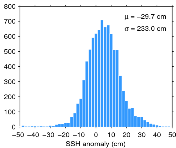
Figure 7. Histogram of flag-valid SSH anomaly over oceans and lakes for 04/08/2015. The mean ( \mu ) and standard deviation ( \sigma ) are also shown. Note that values outside [-50 50] cm are excluded from the histogram for the sake of readability but not from the computation of \mu and \sigma .
