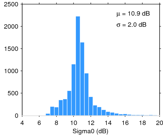
Figure 25. Histogram of flag-valid sigma0 over oceans and lakes for 04/08/2015. The mean ( \mu ) and standard deviation ( \sigma ) are also shown. Note that values outside [4 20] dB are excluded from the histogram for the sake of readability but not from the computation of \mu and \sigma .
