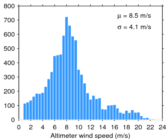
Figure 35. Histogram of science-valid wind over oceans and lakes for 04/08/2015. The mean ( \mu ) and standard deviation ( \sigma ) are also shown. Note that values larger than 24 m/s are excluded from the histogram for the sake of readability but not from the computation of \mu and \sigma .
