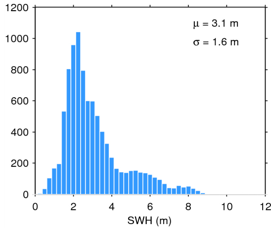
Figure 17. Histogram of flag-valid SWH over oceans and lakes for 04/08/2015. The mean ( \mu ) and standard deviation ( \sigma ) are also shown. Note that values larger than 12 m are excluded from the histogram for the sake of readability but not from the computation of \mu and \sigma .
