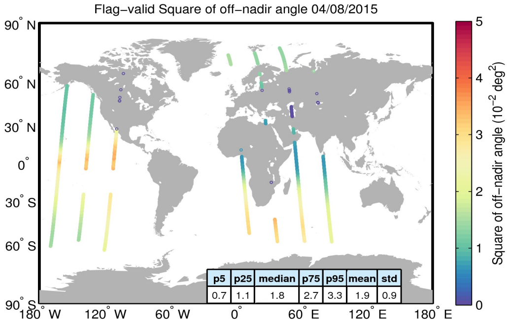
Figure 37. Geographical distribution of flag-valid mispointing data over oceans and lakes for 04/08/2015. The statistical values shown in the table refer to the mispointing in 10^{-2} \text{ deg}^2 and are calculated over all measurements shown in the figure.
