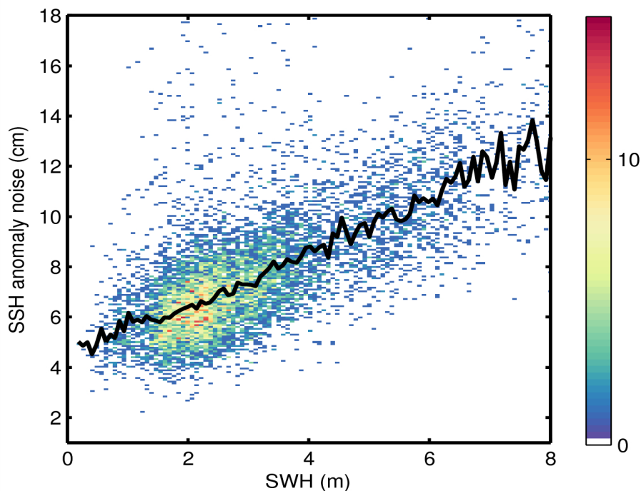
Figure 9. 2D histogram showing flag-valid SSH anomaly noise as a function of SWH for 04/08/2015. The black line denotes the median SSH anomaly as a function of SWH.
