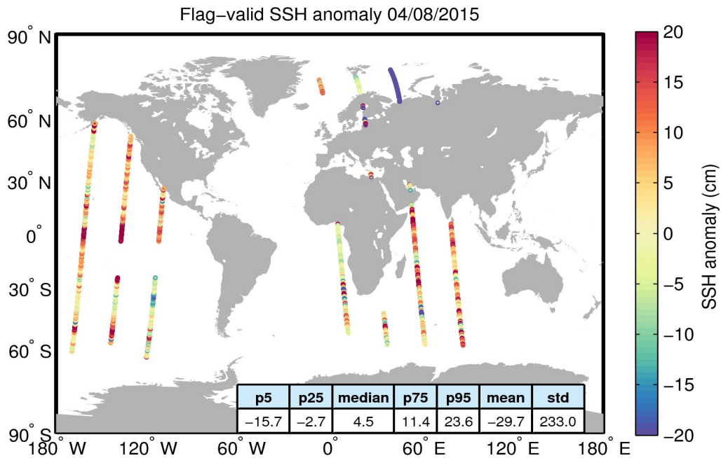
Figure 5. Geographical distribution of flag-valid 1-Hz SSH anomaly data over oceans and lakes for 04/08/2015. The statistical values shown in the table refer to the SSH anomaly in cm and are calculated over all measurements shown in the figure.
