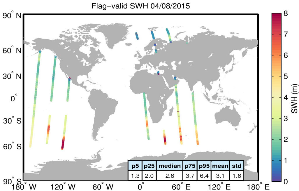
Figure 15. Geographical distribution of flag-valid SWH data over oceans and lakes for 04/08/2015. The statistical values shown in the figure refer to the SWH in m and are calculated over all measurements shown in the figure.
