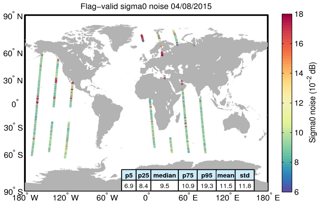
Figure 26. Geographical distribution of flag-valid 20-Hz sigma0 measurement noise over oceans and lakes for 04/08/2015. The statistical values shown in the table refer to the sigma0 noise and are calculated over all measurements shown in the figure.
