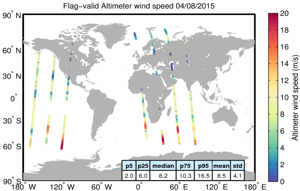
Figure 31. Geographical distribution of flag-valid wind data over oceans and lakes for 04/08/2015. The statistical values shown in the table refer to the wind in m/s and are calculated over all measurements shown in the figure.
