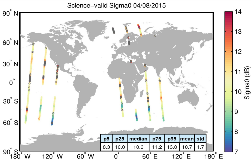
Figure 27. Geographical distribution of science-valid sigma0 data over oceans and lakes for 04/08/2015. The statistical values shown in the table refer to the sigma0 in dB and are calculated over all measurements shown in the figure. Gray circles denote records that have been rejected based on the editing criteria described in Table 4.
