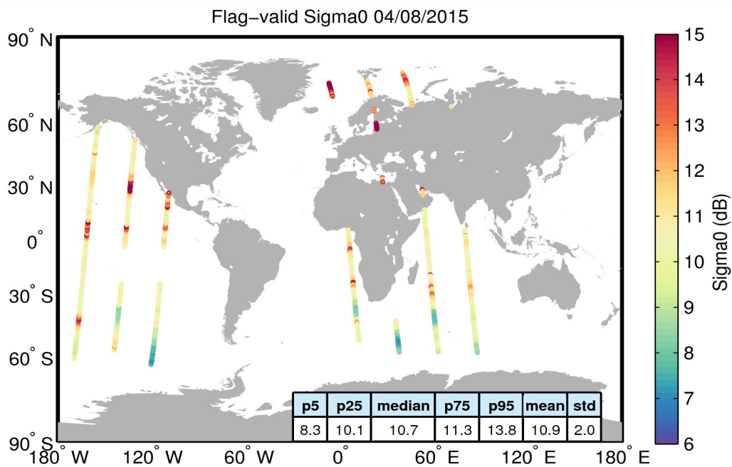
Figure 23. Geographical distribution of flag-valid sigma0 data over oceans and lakes for 04/08/2015. The statistical values shown in the table refer to the sigma0 in dB and are calculated over all measurements shown in the figure.
