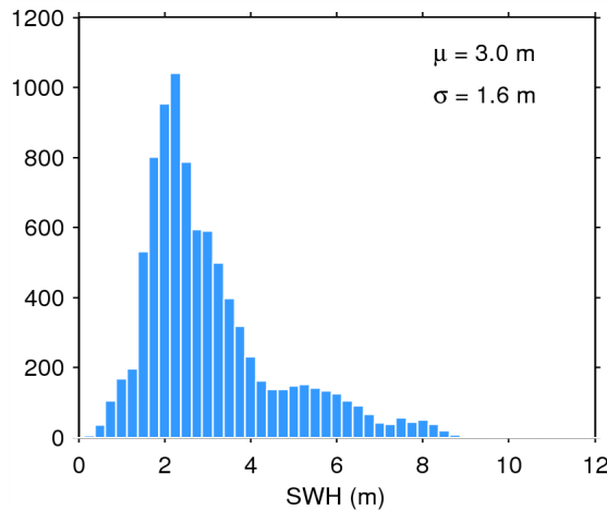
Figure 20. Histogram of science-valid SWH over oceans and lakes for 04/08/2015. The mean ( \mu ) and standard deviation ( \sigma ) are also shown. Note that values larger than 12 m are excluded from the histogram for the sake of readability but not from the computation of \mu and \sigma .
