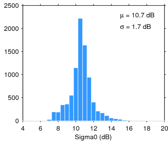
Figure 28. Histogram of science-valid sigma0 over oceans and lakes for 04/08/2015. The mean ( \mu ) and standard deviation ( \sigma ) are also shown. Note that values outside [4 20] dB are excluded from the histogram for the sake of readability but not from the computation of \mu and \sigma .
