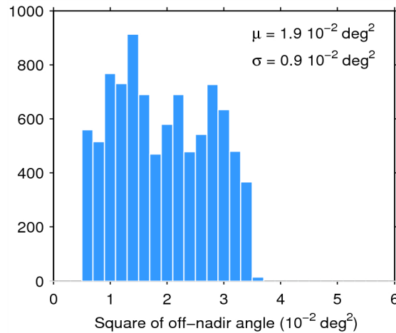
Figure 39. Histogram of flag-valid mispointing over oceans and lakes for 04/08/2015. The mean ( \mu ) and standard deviation ( \sigma ) are also shown. Note that values larger than 6 \cdot 10^{-2} \text{ deg}^2 are excluded from the histogram for the sake of readability but not from the computation of \mu and \sigma .
