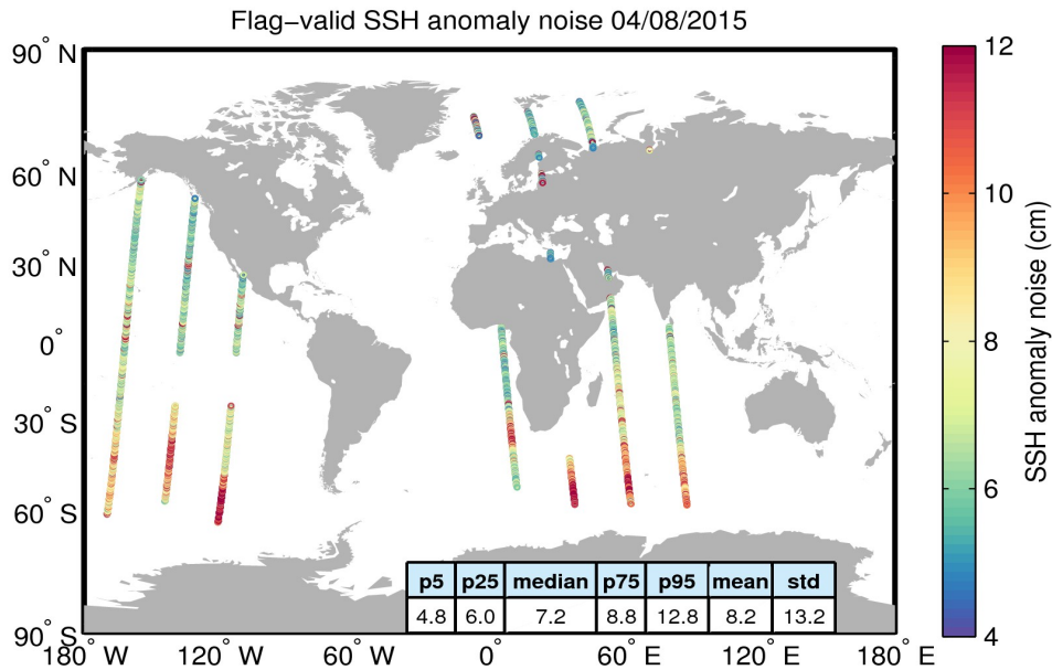
Figure 8. Geographical distribution of flag-valid 20-Hz SSH anomaly measurement noise over oceans and lakes for 04/08/2015. The statistical values shown in the table refer to the SSH anomaly noise and are calculated over all measurements shown in the figure.
