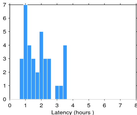
Figure 2. Histogram of the data latency for 04/08/2015. The y-axis denotes the number of files that are made available with a delay of x-hours with respect to the mean time of the records stored in the file.
