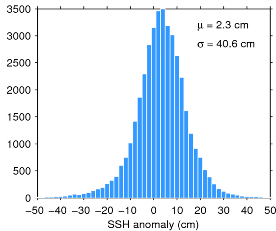
Figure 7. Histogram of flag-valid SSH anomaly over oceans and lakes for 03/08/2015. The mean ( \mu ) and standard deviation ( \sigma ) are also shown. Note that values outside [-50\ 50] cm are excluded from the histogram for the sake of readability but not from the computation of \mu and \sigma .
