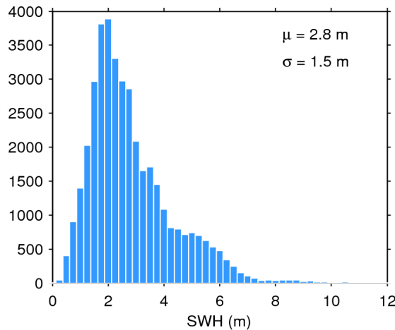
Figure 20. Histogram of science-valid SWH over oceans and lakes for 03/08/2015. The mean ( \mu ) and standard deviation ( \sigma ) are also shown. Note that values larger than 12 m are excluded from the histogram for the sake of readability but not from the computation of \mu and \sigma .
