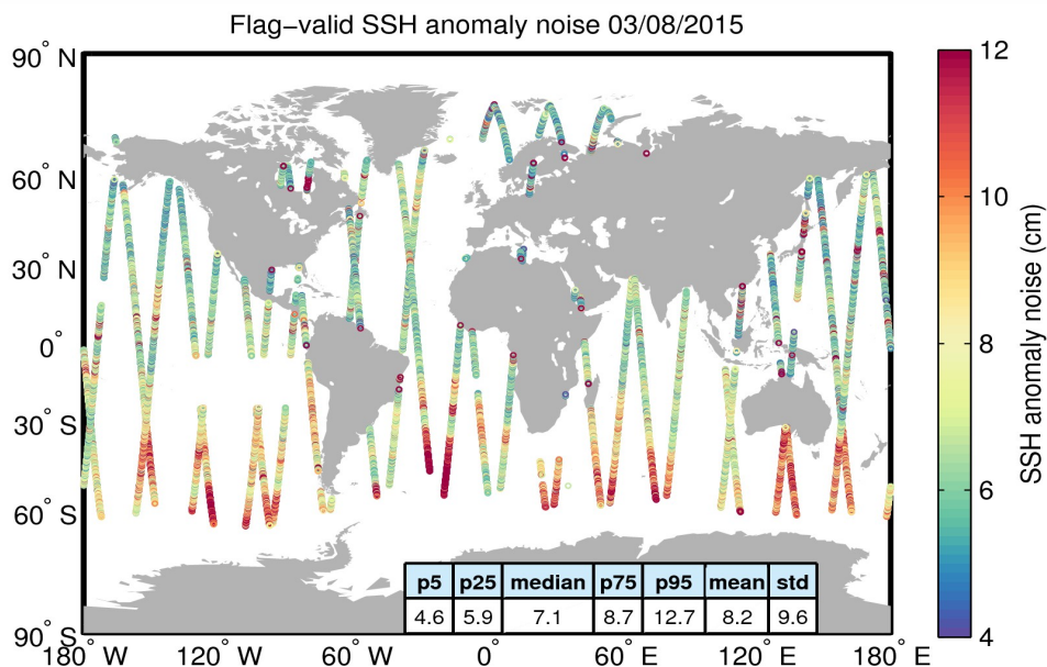
Figure 8. Geographical distribution of flag-valid 20-Hz SSH anomaly measurement noise over oceans and lakes for 03/08/2015. The statistical values shown in the table refer to the SSH anomaly noise and are calculated over all measurements shown in the figure.
