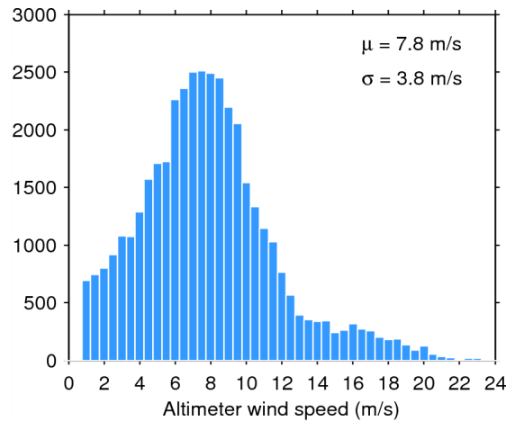
Figure 33. Histogram of flag-valid wind over oceans and lakes for 03/08/2015. The mean ( \mu ) and standard deviation ( \sigma ) are also shown. Note that values larger than 24 m/s are excluded from the histogram for the sake of readability but not from the computation of \mu and \sigma .
