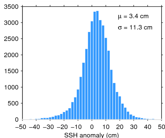
Figure 11. Histogram of science-valid SSH anomaly over oceans and lakes for 03/08/2015. The mean ( \mu ) and standard deviation ( \sigma ) are also shown. Note that values outside [-50 50] cm are excluded from the histogram for the sake of readability but not from the computation of \mu and \sigma .
