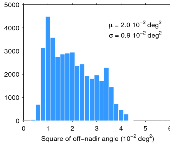
Figure 39. Histogram of flag-valid mispointing over oceans and lakes for 03/08/2015. The mean ( \mu ) and standard deviation ( \sigma ) are also shown. Note that values larger than 6 \cdot 10^{-2} \text{ deg}^2 are excluded from the histogram for the sake of readability but not from the computation of \mu and \sigma .
