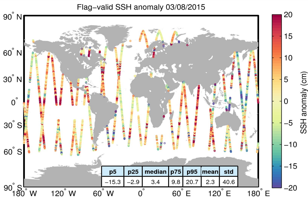
Figure 5. Geographical distribution of flag-valid 1-Hz SSH anomaly data over oceans and lakes for 03/08/2015. The statistical values shown in the table refer to the SSH anomaly in cm and are calculated over all measurements shown in the figure.
