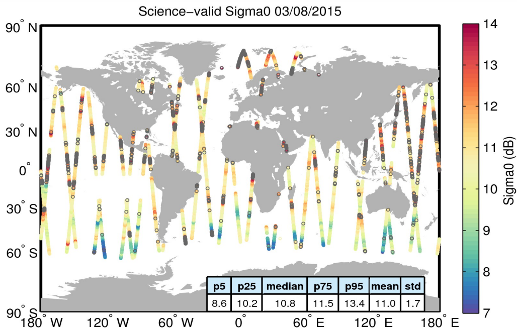
Figure 27. Geographical distribution of science-valid sigma0 data over oceans and lakes for 03/08/2015. The statistical values shown in the table refer to the sigma0 in dB and are calculated over all measurements shown in the figure. Gray circles denote records that have been rejected based on the editing criteria described in Table 4.
