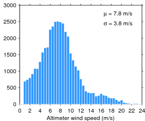
Figure 35. Histogram of science-valid wind over oceans and lakes for 03/08/2015. The mean ( \mu ) and standard deviation ( \sigma ) are also shown. Note that values larger than 24 m/s are excluded from the histogram for the sake of readability but not from the computation of \mu and \sigma .
