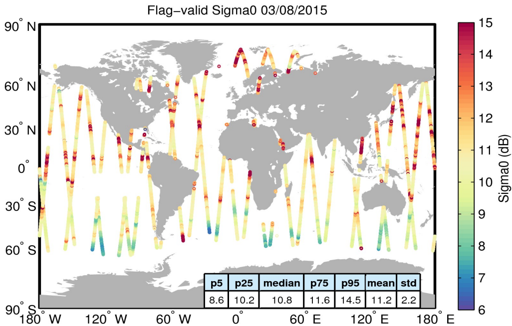
Figure 23. Geographical distribution of flag-valid sigma0 data over oceans and lakes for 03/08/2015. The statistical values shown in the table refer to the sigma0 in dB and are calculated over all measurements shown in the figure.
