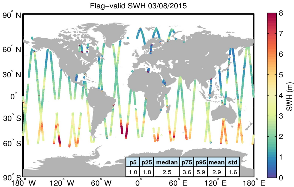
Figure 15. Geographical distribution of flag-valid SWH data over oceans and lakes for 03/08/2015. The statistical values shown in the figure refer to the SWH in m and are calculated over all measurements shown in the figure.
