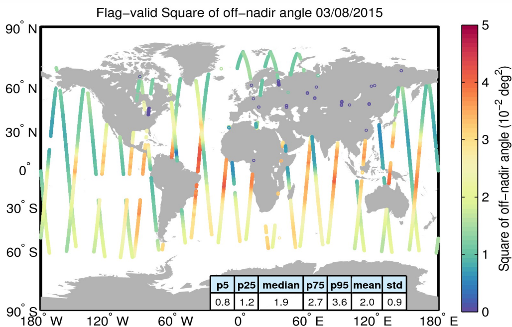
Figure 37. Geographical distribution of flag-valid mispointing data over oceans and lakes for 03/08/2015. The statistical values shown in the table refer to the mispointing in 10^{-2} \text{deg}^2 and are calculated over all measurements shown in the figure.
