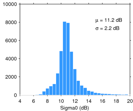
Figure 25. Histogram of flag-valid sigma0 over oceans and lakes for 03/08/2015. The mean ( \mu ) and standard deviation ( \sigma ) are also shown. Note that values outside [4 20] dB are excluded from the histogram for the sake of readability but not from the computation of \mu and \sigma .
