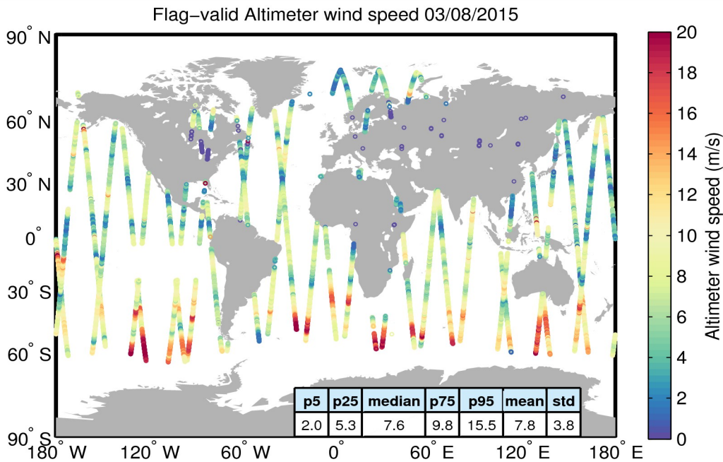
Figure 31. Geographical distribution of flag-valid wind data over oceans and lakes for 03/08/2015. The statistical values shown in the table refer to the wind in m/s and are calculated over all measurements shown in the figure.
