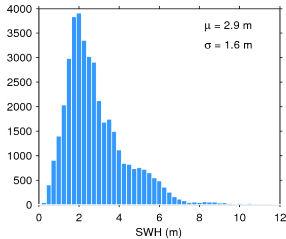
Figure 17. Histogram of flag-valid SWH over oceans and lakes for 03/08/2015. The mean ( \mu ) and standard deviation ( \sigma ) are also shown. Note that values larger than 12 m are excluded from the histogram for the sake of readability but not from the computation of \mu and \sigma .
