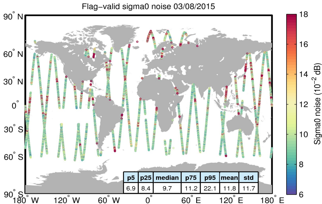
Figure 26. Geographical distribution of flag-valid 20-Hz sigma0 measurement noise over oceans and lakes for 03/08/2015. The statistical values shown in the table refer to the sigma0 noise and are calculated over all measurements shown in the figure.
