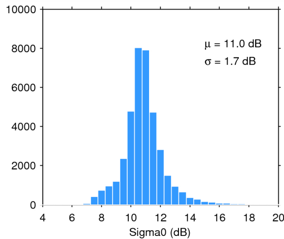
Figure 28. Histogram of science-valid sigma0 over oceans and lakes for 03/08/2015. The mean ( \mu ) and standard deviation ( \sigma ) are also shown. Note that values outside [4 20] dB are excluded from the histogram for the sake of readability but not from the computation of \mu and \sigma .
