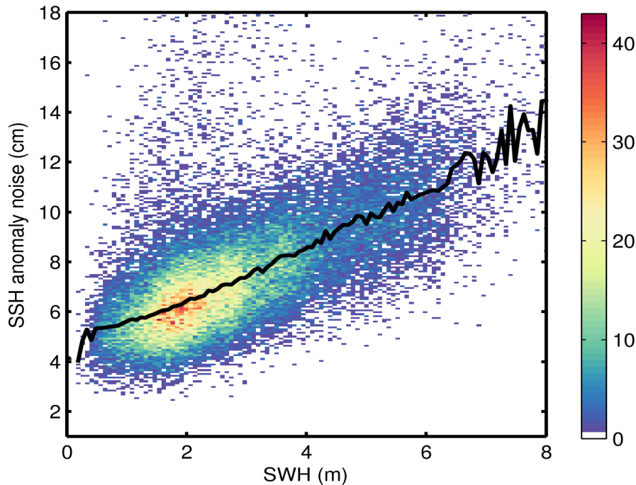
Figure 9. 2D histogram showing flag-valid SSH anomaly noise as a function of SWH for 03/08/2015. The black line denotes the median SSH anomaly as a function of SWH.
