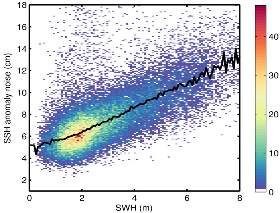
Figure 9. 2D histogram showing flag-valid SSH anomaly noise as a function of SWH for 01/08/2015. The black line denotes the median SSH anomaly as a function of SWH.
