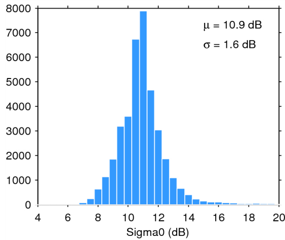
Figure 28. Histogram of science-valid sigma0 over oceans and lakes for 01/08/2015. The mean ( \mu ) and standard deviation ( \sigma ) are also shown. Note that values outside [4 20] dB are excluded from the histogram for the sake of readability but not from the computation of \mu and \sigma .
