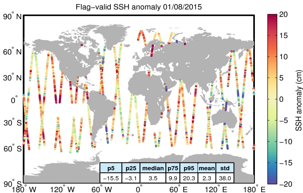
Figure 5. Geographical distribution of flag-valid 1-Hz SSH anomaly data over oceans and lakes for 01/08/2015. The statistical values shown in the table refer to the SSH anomaly in cm and are calculated over all measurements shown in the figure.
