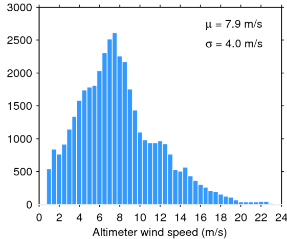
Figure 33. Histogram of flag-valid wind over oceans and lakes for 01/08/2015. The mean ( \mu ) and standard deviation ( \sigma ) are also shown. Note that values larger than 24 m/s are excluded from the histogram for the sake of readability but not from the computation of \mu and \sigma .
