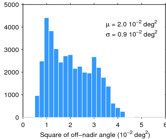
Figure 39. Histogram of flag-valid mispointing over oceans and lakes for 01/08/2015. The mean ( \mu ) and standard deviation ( \sigma ) are also shown. Note that values larger than 6 \cdot 10^{-2} \text{ deg}^2 are excluded from the histogram for the sake of readability but not from the computation of \mu and \sigma .
