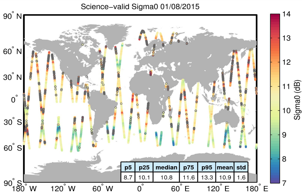
Figure 27. Geographical distribution of science-valid sigma0 data over oceans and lakes for 01/08/2015. The statistical values shown in the table refer to the sigma0 in dB and are calculated over all measurements shown in the figure. Gray circles denote records that have been rejected based on the editing criteria described in Table 4.
