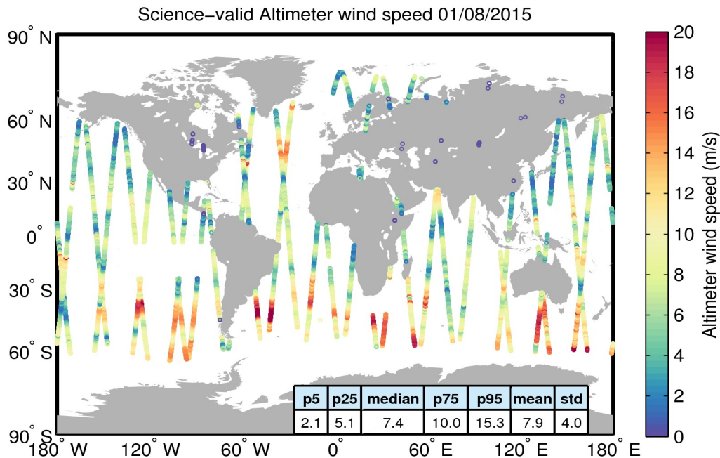
Figure 34. Geographical distribution of science-valid wind data over oceans and lakes for 01/08/2015. The statistical values shown in the table refer to the wind in m/s and are calculated over all measurements shown in the figure. Gray circles denote records that have been rejected based on the editing criteria described in Table 5.
