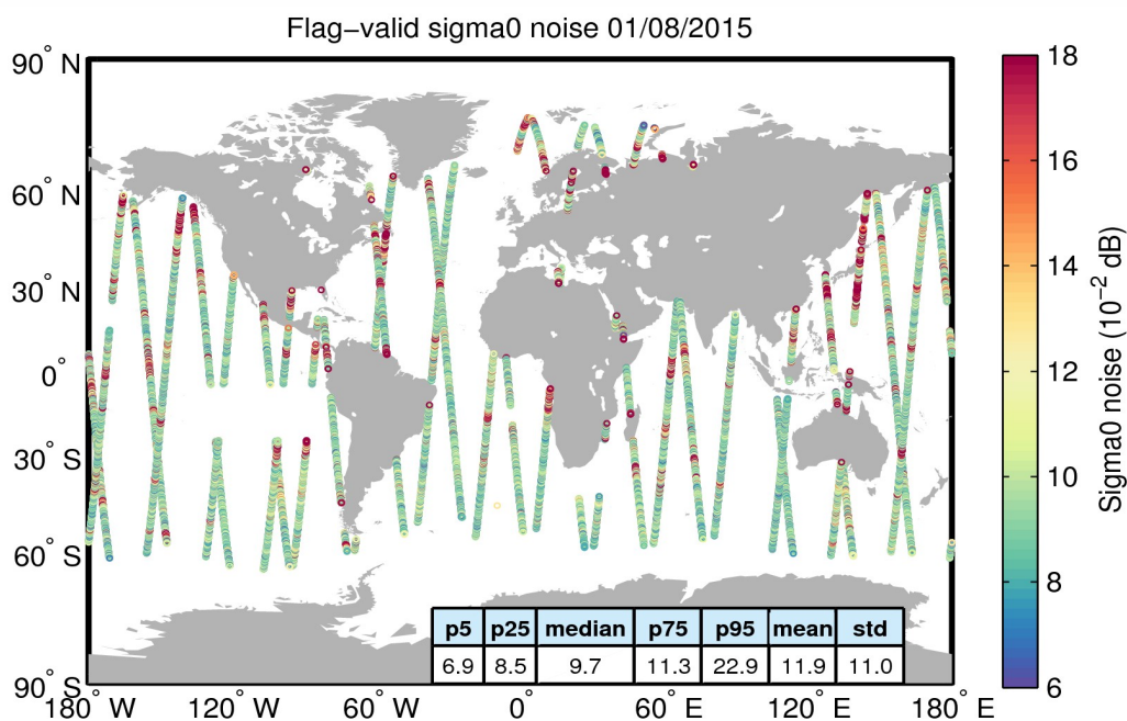
Figure 26. Geographical distribution of flag-valid 20-Hz sigma0 measurement noise over oceans and lakes for 01/08/2015. The statistical values shown in the table refer to the sigma0 noise and are calculated over all measurements shown in the figure.
