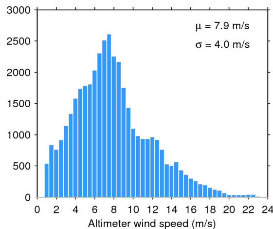
Figure 35. Histogram of science-valid wind over oceans and lakes for 01/08/2015. The mean ( \mu ) and standard deviation ( \sigma ) are also shown. Note that values larger than 24 m/s are excluded from the histogram for the sake of readability but not from the computation of \mu and \sigma .
