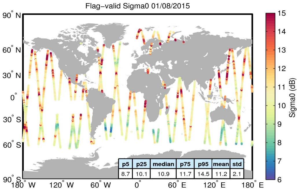
Figure 23. Geographical distribution of flag-valid sigma0 data over oceans and lakes for 01/08/2015. The statistical values shown in the table refer to the sigma0 in dB and are calculated over all measurements shown in the figure.
