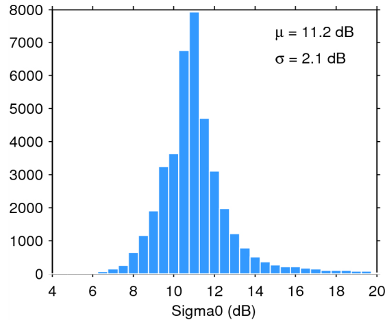
Figure 25. Histogram of flag-valid sigma0 over oceans and lakes for 01/08/2015. The mean ( \mu ) and standard deviation ( \sigma ) are also shown. Note that values outside [4 20] dB are excluded from the histogram for the sake of readability but not from the computation of \mu and \sigma .
