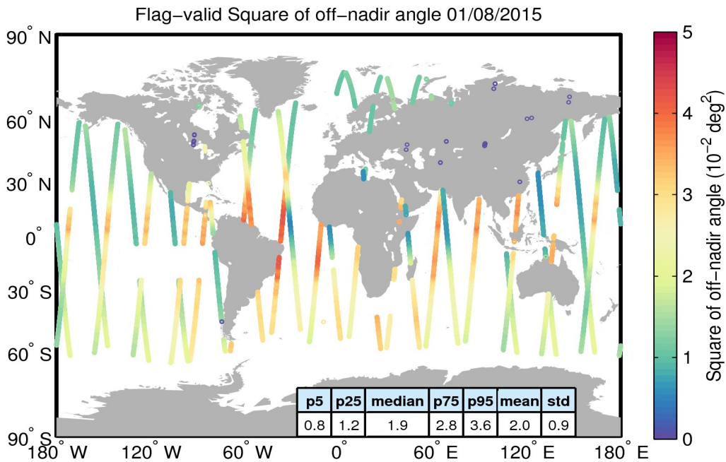
Figure 37. Geographical distribution of flag-valid mispointing data over oceans and lakes for 01/08/2015. The statistical values shown in the table refer to the mispointing in 10^{-2} \text{deg}^2 and are calculated over all measurements shown in the figure.
