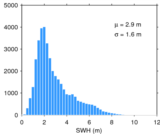
Figure 20. Histogram of science-valid SWH over oceans and lakes for 01/08/2015. The mean ( \mu ) and standard deviation ( \sigma ) are also shown. Note that values larger than 12 m are excluded from the histogram for the sake of readability but not from the computation of \mu and \sigma .
