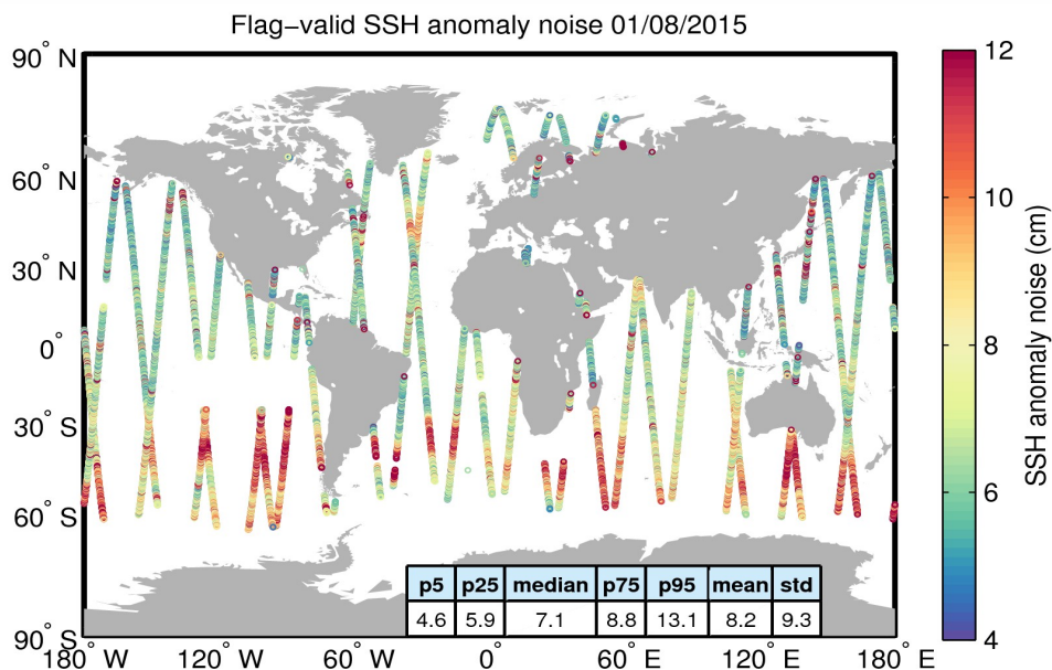
Figure 8. Geographical distribution of flag-valid 20-Hz SSH anomaly measurement noise over oceans and lakes for 01/08/2015. The statistical values shown in the table refer to the SSH anomaly noise and are calculated over all measurements shown in the figure.
