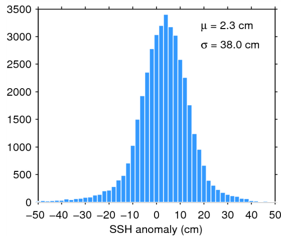
Figure 7. Histogram of flag-valid SSH anomaly over oceans and lakes for 01/08/2015. The mean ( \mu ) and standard deviation ( \sigma ) are also shown. Note that values outside [-50\ 50] cm are excluded from the histogram for the sake of readability but not from the computation of \mu and \sigma .
