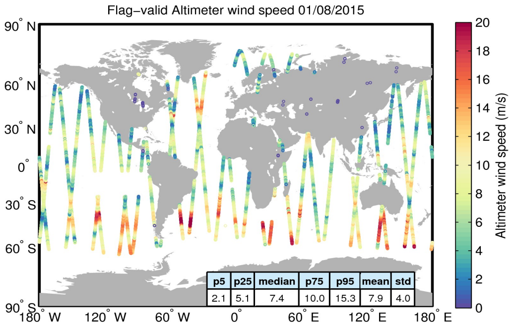
Figure 31. Geographical distribution of flag-valid wind data over oceans and lakes for 01/08/2015. The statistical values shown in the table refer to the wind in m/s and are calculated over all measurements shown in the figure.
