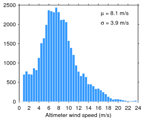
Figure 35. Histogram of science-valid wind over oceans and lakes for 31/07/2015. The mean ( \mu ) and standard deviation ( \sigma ) are also shown. Note that values larger than 24 m/s are excluded from the histogram for the sake of readability but not from the computation of \mu and \sigma .
