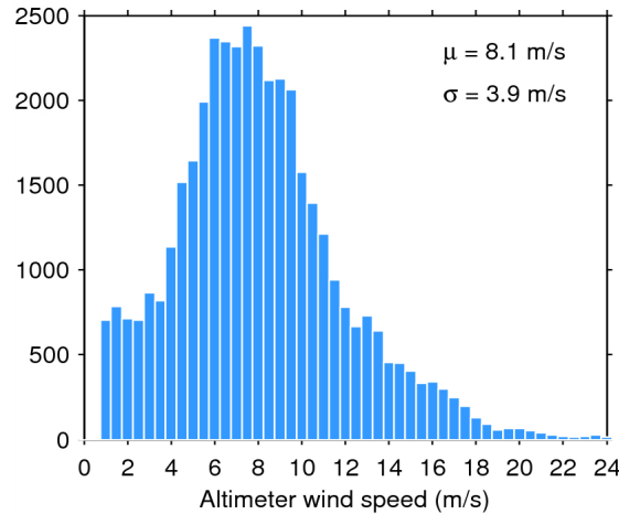
Figure 33. Histogram of flag-valid wind over oceans and lakes for 31/07/2015. The mean ( \mu ) and standard deviation ( \sigma ) are also shown. Note that values larger than 24 m/s are excluded from the histogram for the sake of readability but not from the computation of \mu and \sigma .
