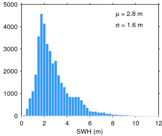
Figure 17. Histogram of flag-valid SWH over oceans and lakes for 31/07/2015. The mean ( \mu ) and standard deviation ( \sigma ) are also shown. Note that values larger than 12 m are excluded from the histogram for the sake of readability but not from the computation of \mu and \sigma .
