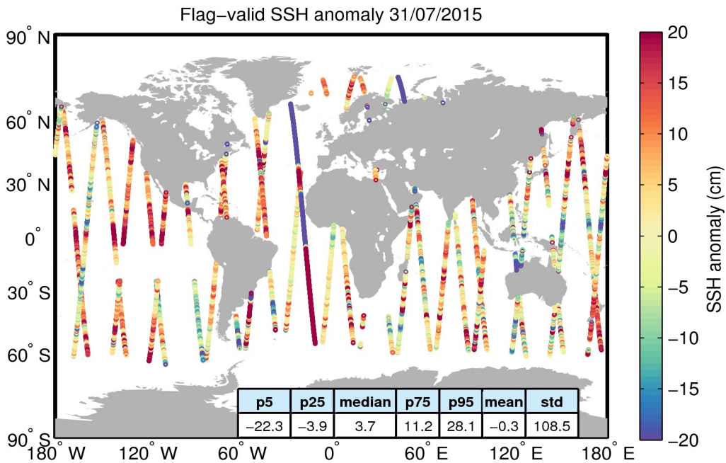
Figure 5. Geographical distribution of flag-valid 1-Hz SSH anomaly data over oceans and lakes for 31/07/2015. The statistical values shown in the table refer to the SSH anomaly in cm and are calculated over all measurements shown in the figure.
