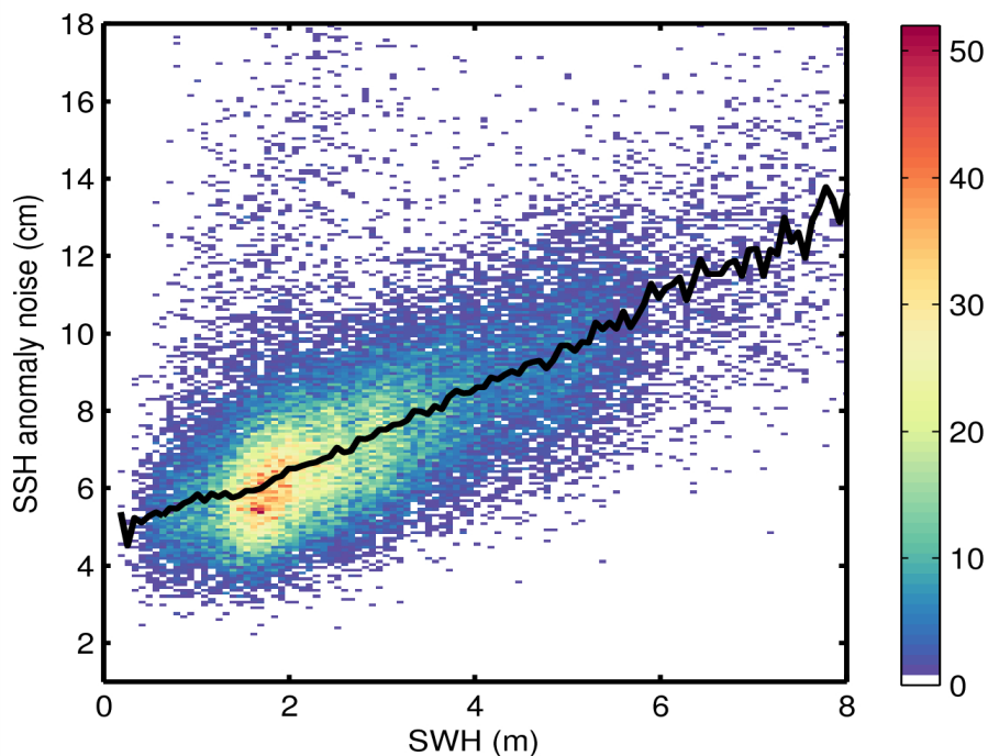
Figure 9. 2D histogram showing flag-valid SSH anomaly noise as a function of SWH for 31/07/2015. The black line denotes the median SSH anomaly as a function of SWH.
