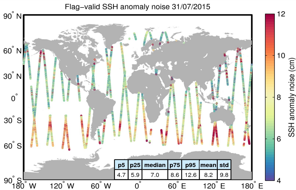
Figure 8. Geographical distribution of flag-valid 20-Hz SSH anomaly measurement noise over oceans and lakes for 31/07/2015. The statistical values shown in the table refer to the SSH anomaly noise and are calculated over all measurements shown in the figure.
