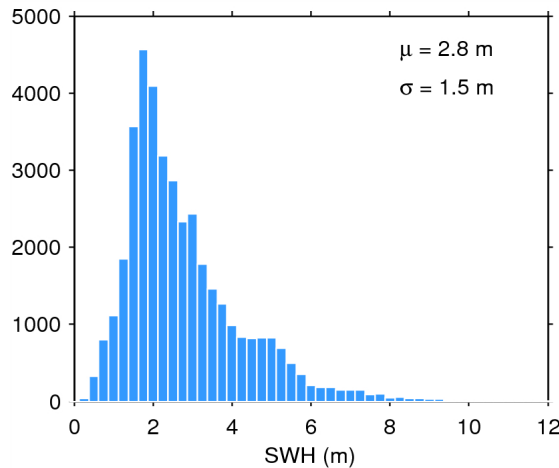
Figure 20. Histogram of science-valid SWH over oceans and lakes for 31/07/2015. The mean ( \mu ) and standard deviation ( \sigma ) are also shown. Note that values larger than 12 m are excluded from the histogram for the sake of readability but not from the computation of \mu and \sigma .
