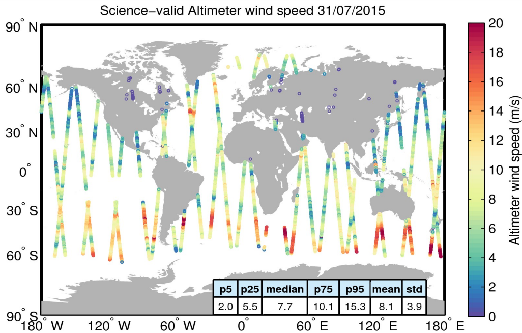
Figure 34. Geographical distribution of science-valid wind data over oceans and lakes for 31/07/2015. The statistical values shown in the table refer to the wind in m/s and are calculated over all measurements shown in the figure. Gray circles denote records that have been rejected based on the editing criteria described in Table 5.
