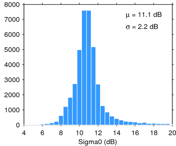
Figure 25. Histogram of flag-valid sigma0 over oceans and lakes for 31/07/2015. The mean ( \mu ) and standard deviation ( \sigma ) are also shown. Note that values outside [4 20] dB are excluded from the histogram for the sake of readability but not from the computation of \mu and \sigma .
