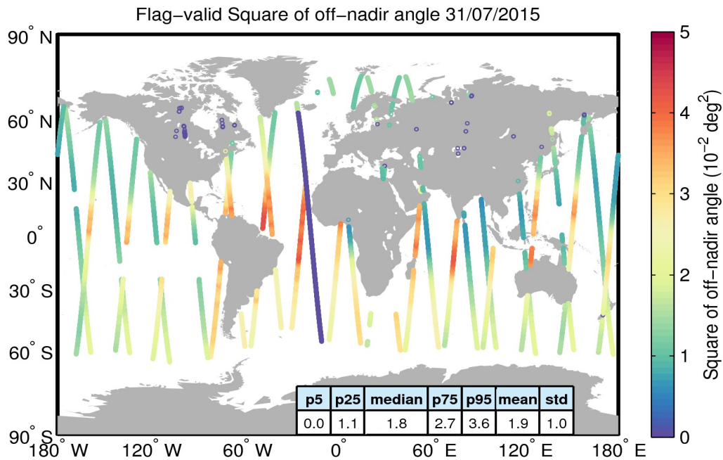
Figure 37. Geographical distribution of flag-valid mispointing data over oceans and lakes for 31/07/2015. The statistical values shown in the table refer to the mispointing in 10^{-2} deg 2 and are calculated over all measurements shown in the figure.
