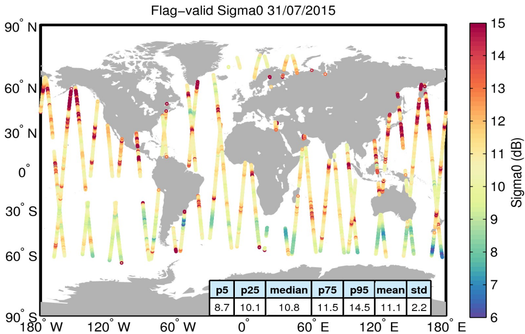
Figure 23. Geographical distribution of flag-valid sigma0 data over oceans and lakes for 31/07/2015. The statistical values shown in the table refer to the sigma0 in dB and are calculated over all measurements shown in the figure.
