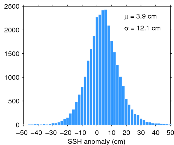
Figure 11. Histogram of science-valid SSH anomaly over oceans and lakes for 31/07/2015. The mean ( \mu ) and standard deviation ( \sigma ) are also shown. Note that values outside [-50 50] cm are excluded from the histogram for the sake of readability but not from the computation of \mu and \sigma .
