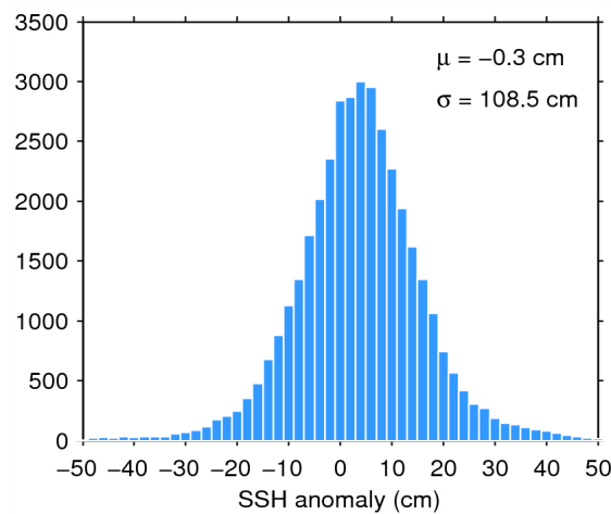
Figure 7. Histogram of flag-valid SSH anomaly over oceans and lakes for 31/07/2015. The mean ( \mu ) and standard deviation ( \sigma ) are also shown. Note that values outside [-50 50] cm are excluded from the histogram for the sake of readability but not from the computation of \mu and \sigma .
