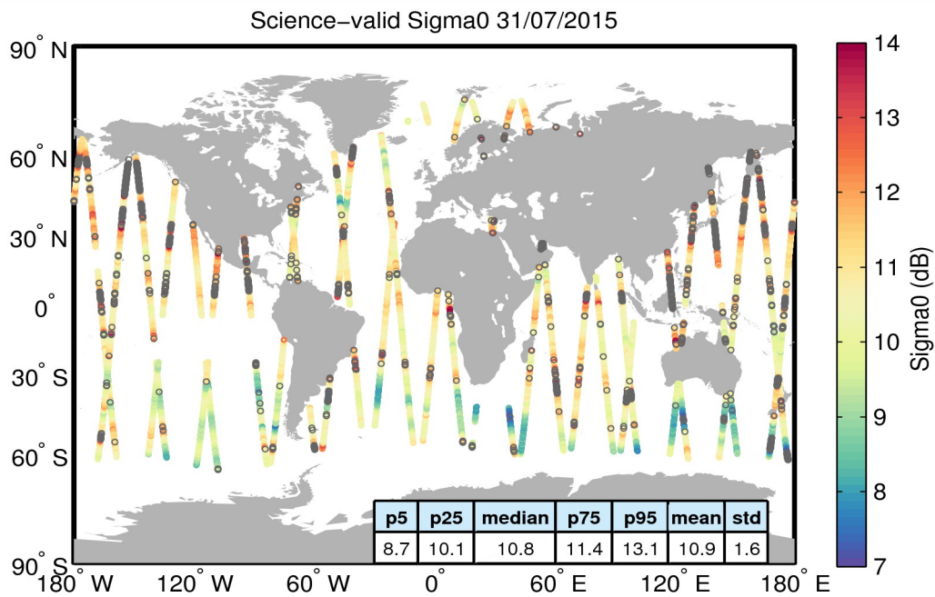
Figure 27. Geographical distribution of science-valid sigma0 data over oceans and lakes for 31/07/2015. The statistical values shown in the table refer to the sigma0 in dB and are calculated over all measurements shown in the figure. Gray circles denote records that have been rejected based on the editing criteria described in Table 4.
