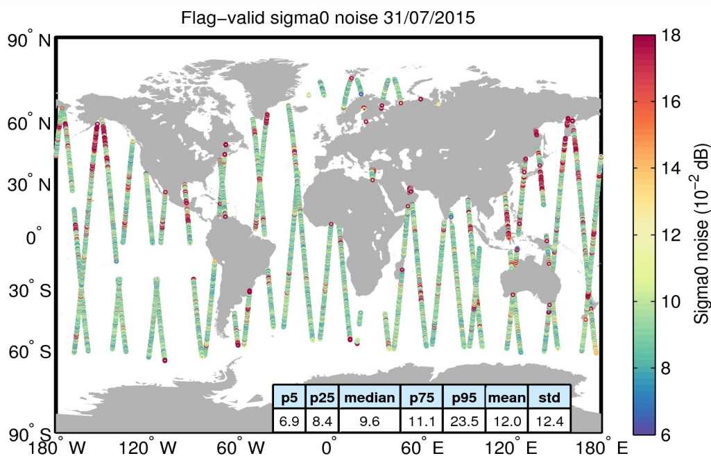
Figure 26. Geographical distribution of flag-valid 20-Hz sigma0 measurement noise over oceans and lakes for 31/07/2015. The statistical values shown in the table refer to the sigma0 noise and are calculated over all measurements shown in the figure.
