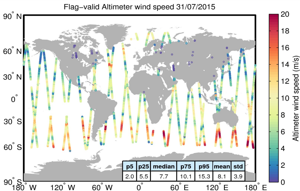
Figure 31. Geographical distribution of flag-valid wind data over oceans and lakes for 31/07/2015. The statistical values shown in the table refer to the wind in m/s and are calculated over all measurements shown in the figure.
