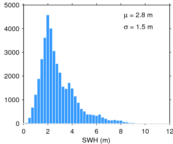
Figure 20. Histogram of science-valid SWH over oceans and lakes for 28/07/2015. The mean ( \mu ) and standard deviation ( \sigma ) are also shown. Note that values larger than 12 m are excluded from the histogram for the sake of readability but not from the computation of \mu and \sigma .
