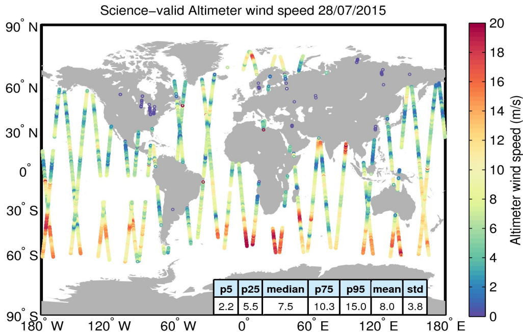
Figure 34. Geographical distribution of science-valid wind data over oceans and lakes for 28/07/2015. The statistical values shown in the table refer to the wind in m/s and are calculated over all measurements shown in the figure. Gray circles denote records that have been rejected based on the editing criteria described in Table 5.
