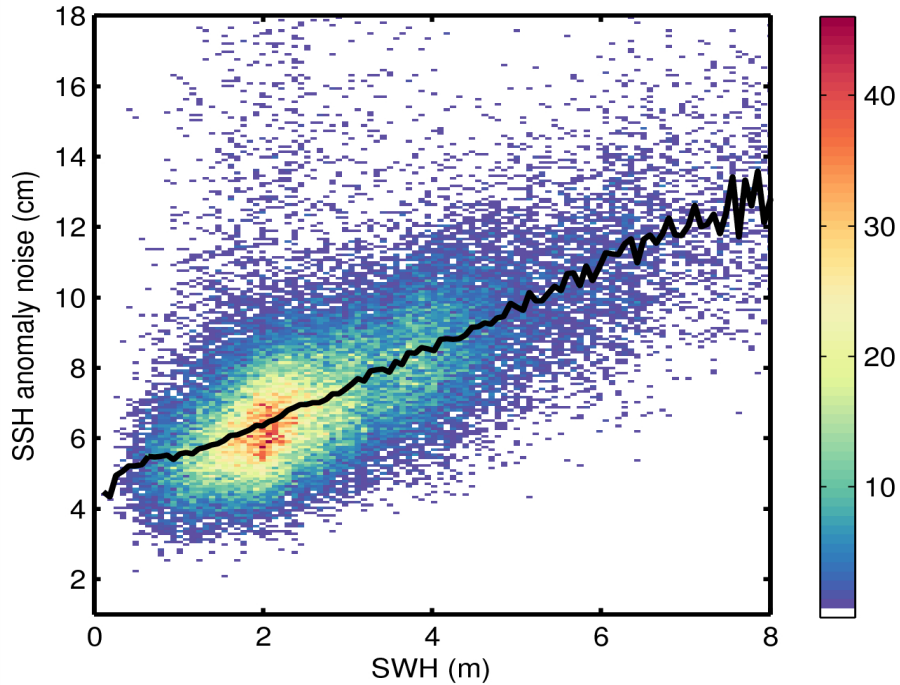
Figure 9. 2D histogram showing flag-valid SSH anomaly noise as a function of SWH for 28/07/2015. The black line denotes the median SSH anomaly as a function of SWH.
