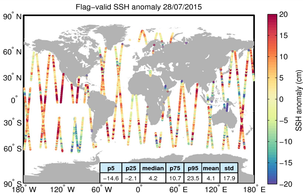
Figure 5. Geographical distribution of flag-valid 1-Hz SSH anomaly data over oceans and lakes for 28/07/2015. The statistical values shown in the table refer to the SSH anomaly in cm and are calculated over all measurements shown in the figure.
