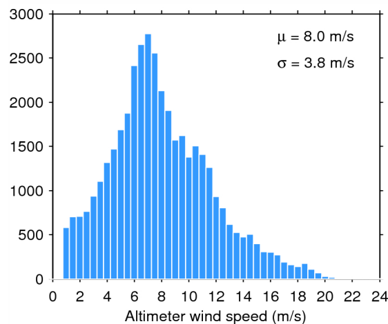
Figure 35. Histogram of science-valid wind over oceans and lakes for 28/07/2015. The mean ( \mu ) and standard deviation ( \sigma ) are also shown. Note that values larger than 24 m/s are excluded from the histogram for the sake of readability but not from the computation of \mu and \sigma .
