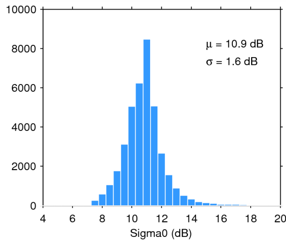
Figure 28. Histogram of science-valid sigma0 over oceans and lakes for 28/07/2015. The mean ( \mu ) and standard deviation ( \sigma ) are also shown. Note that values outside [4 20] dB are excluded from the histogram for the sake of readability but not from the computation of \mu and \sigma .
