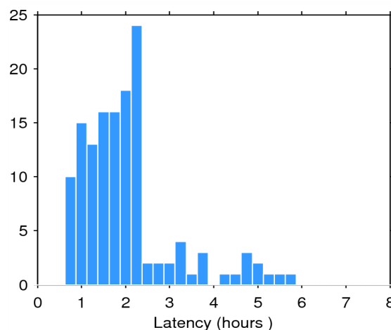
Figure 2. Histogram of the data latency for 28/07/2015. The y-axis denotes the number of files that are made available with a delay of x-hours with respect to the mean time of the records stored in the file.
