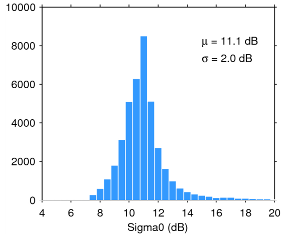
Figure 25. Histogram of flag-valid sigma0 over oceans and lakes for 28/07/2015. The mean ( \mu ) and standard deviation ( \sigma ) are also shown. Note that values outside [4 20] dB are excluded from the histogram for the sake of readability but not from the computation of \mu and \sigma .
