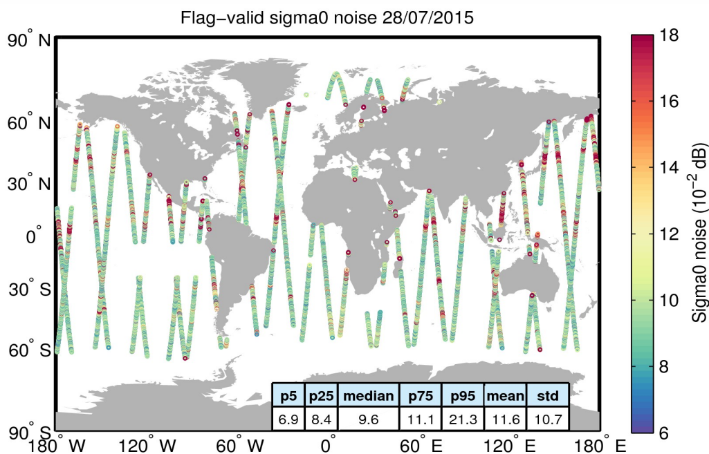
Figure 26. Geographical distribution of flag-valid 20-Hz sigma0 measurement noise over oceans and lakes for 28/07/2015. The statistical values shown in the table refer to the sigma0 noise and are calculated over all measurements shown in the figure.
