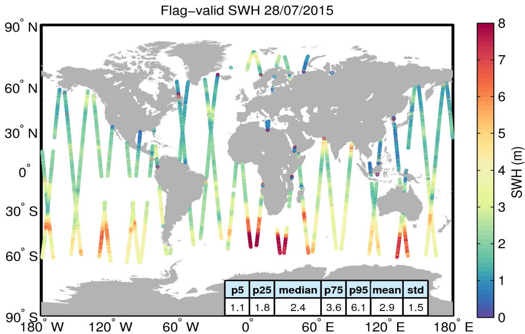
Figure 15. Geographical distribution of flag-valid SWH data over oceans and lakes for 28/07/2015. The statistical values shown in the table refer to the SWH in m and are calculated over all measurements shown in the figure.
