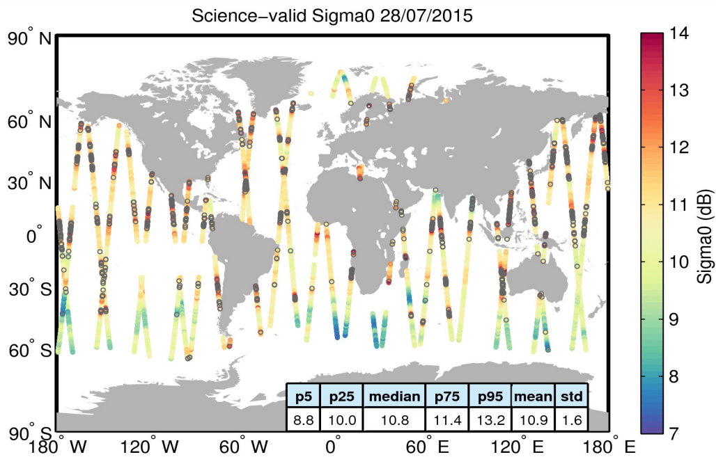
Figure 27. Geographical distribution of science-valid sigma0 data over oceans and lakes for 28/07/2015. The statistical values shown in the table refer to the sigma0 in dB and are calculated over all measurements shown in the figure. Gray circles denote records that have been rejected based on the editing criteria described in Table 4.
