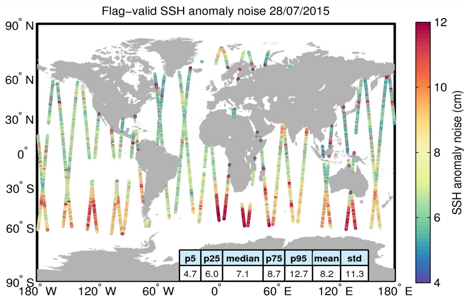
Figure 8. Geographical distribution of flag-valid 20-Hz SSH anomaly measurement noise over oceans and lakes for 28/07/2015. The statistical values shown in the table refer to the SSH anomaly noise and are calculated over all measurements shown in the figure.
