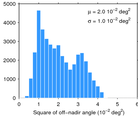
Figure 39. Histogram of flag-valid mispointing over oceans and lakes for 28/07/2015. The mean ( \mu ) and standard deviation ( \sigma ) are also shown. Note that values larger than 6 \cdot 10^{-2} \text{ deg}^2 are excluded from the histogram for the sake of readability but not from the computation of \mu and \sigma .
