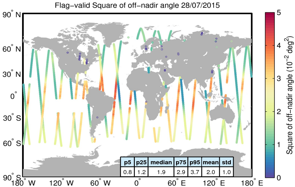
Figure 37. Geographical distribution of flag-valid mispointing data over oceans and lakes for 28/07/2015. The statistical values shown in the table refer to the mispointing in 10^{-2} \text{deg}^2 and are calculated over all measurements shown in the figure.
