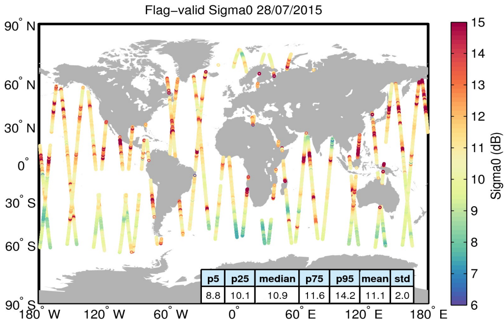
Figure 23. Geographical distribution of flag-valid sigma0 data over oceans and lakes for 28/07/2015. The statistical values shown in the table refer to the sigma0 in dB and are calculated over all measurements shown in the figure.
